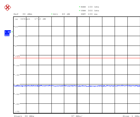
NB-IOT Band 2 CH-High 30MHz~1GHz
