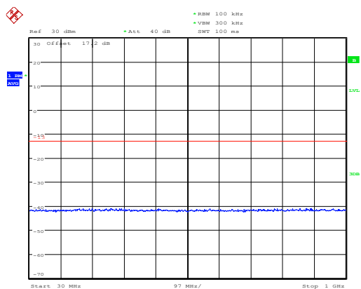
NB-IOT Band 2 CH-Low 30MHz~1GHz
