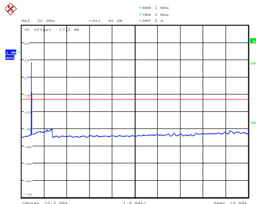
NB-IOT Band 2 CH-Low 1GHz ~20GHz
