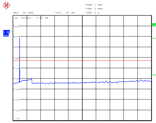
NB-IOT Band 2 CH-High 1GHz ~20GHz
