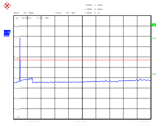
NB-IOT Band 2 CH-Middle 1GHz ~20GHz
