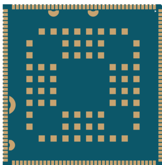
Figure 46: Bottom View of the Module
