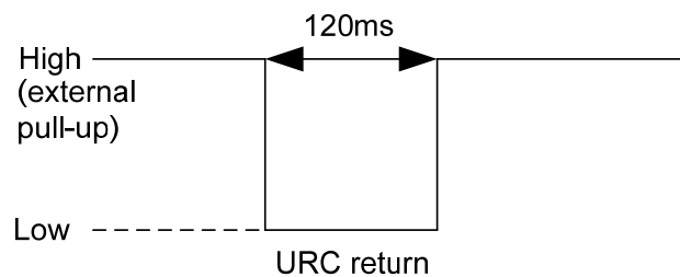
Figure 12: WAKE# Behaviors
