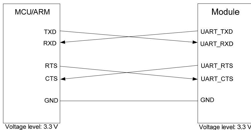
Figure 7: Reference Design of UART Interface
