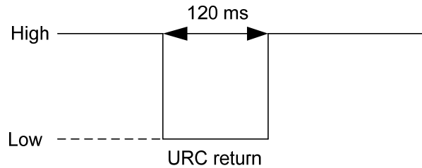
Figure 9: RI Behavior
