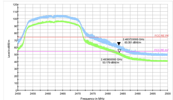
802.11n HT20 -Channel 11 Peak &amp; Average
