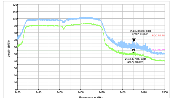
802.11n HT40 -Channel 9 Peak &amp; Average
