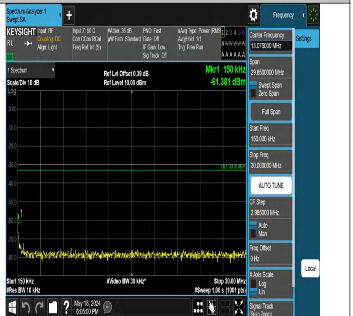
Band2-9538-4-0.15~30MHz-PASS
