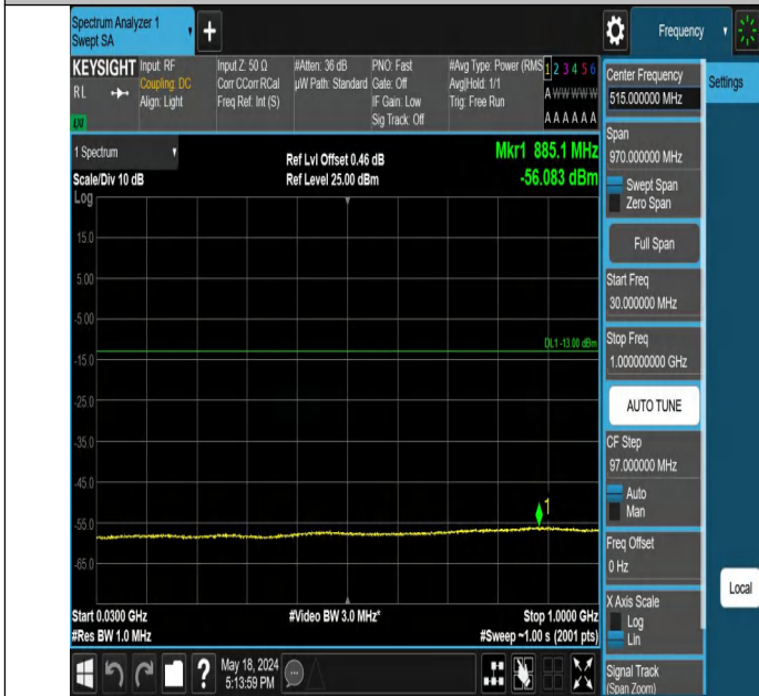
Band2-9262-30~1000MHz-PASS
