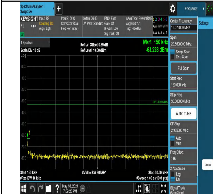
Band2-9262-2-0.15~30MHz-PASS
