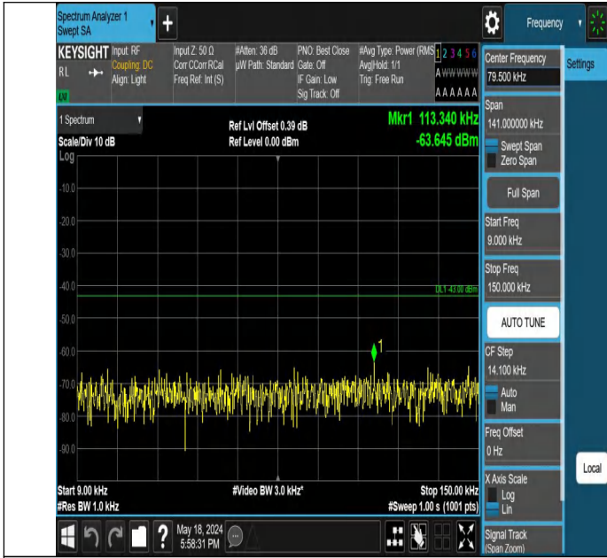
Band2-9538-1-0.009~0.15MHz-PASS
