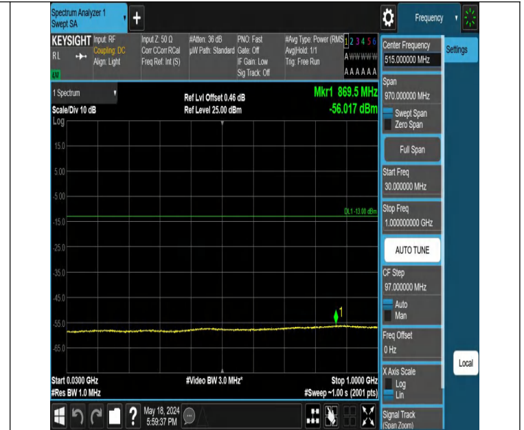
Band2-9262-2-30~1000MHz-PASS
