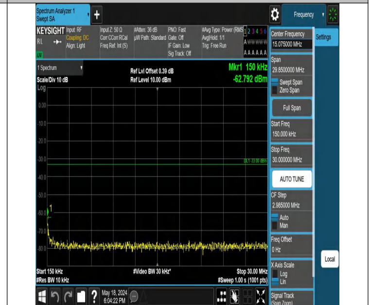
Band2-9400-4-0.15~30MHz-PASS
