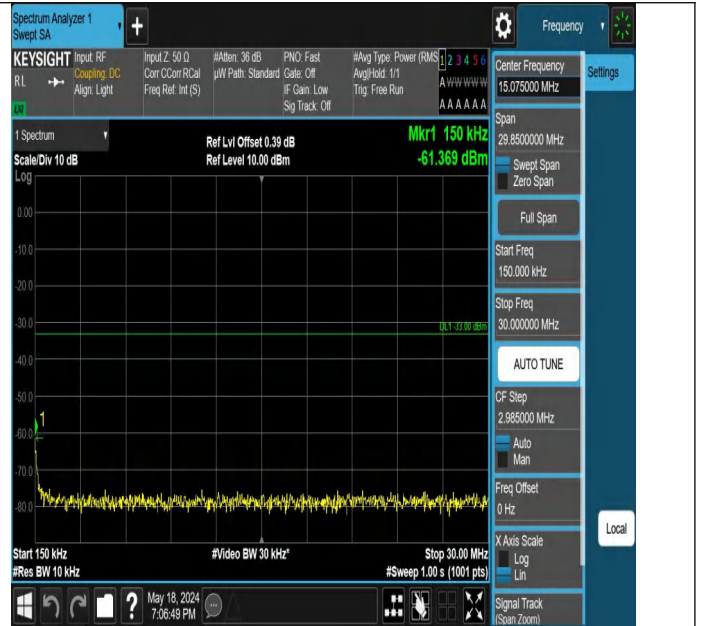
Band2-9262-1-0.15~30MHz-PASS
