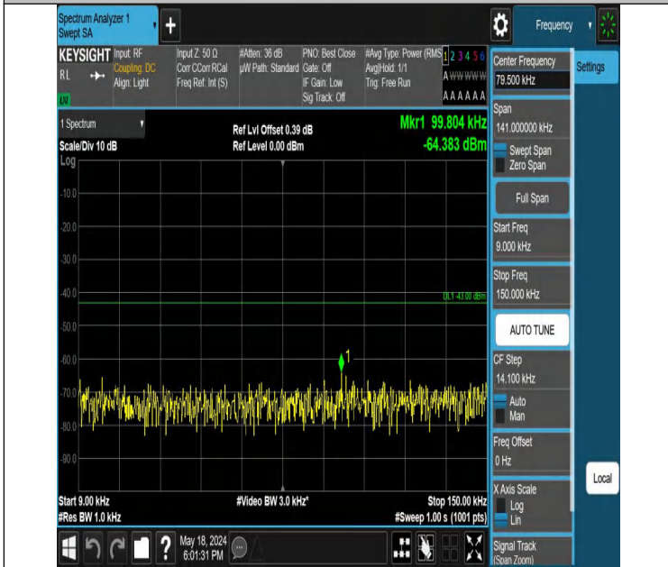
Band2-9262-3-0.009~0.15MHz-PASS
