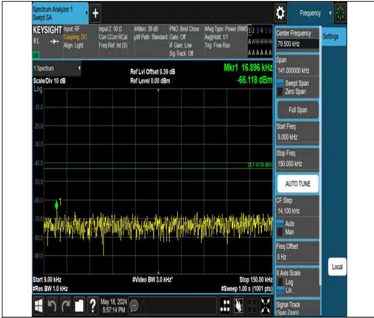
Band2-9262-1-0.009~0.15MHz-PASS
