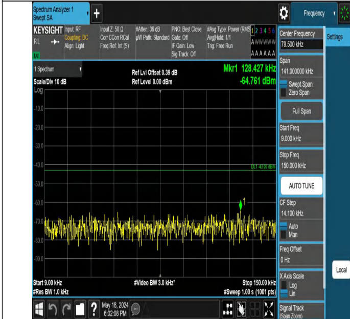
Band2-9400-3-0.009~0.15MHz-PASS
