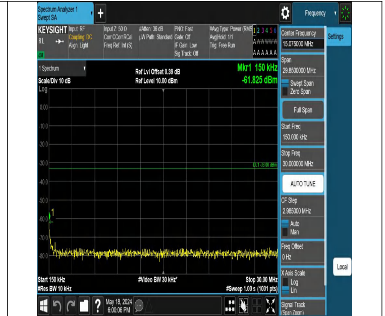
Band2-9400-2-0.15~30MHz-PASS
