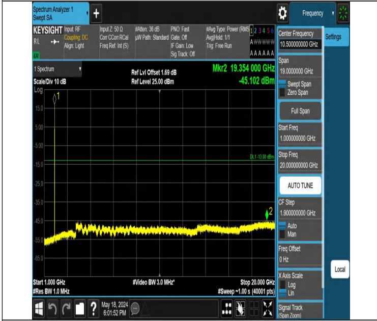
Band2-9262-3-1000~20000MHz-PASS
