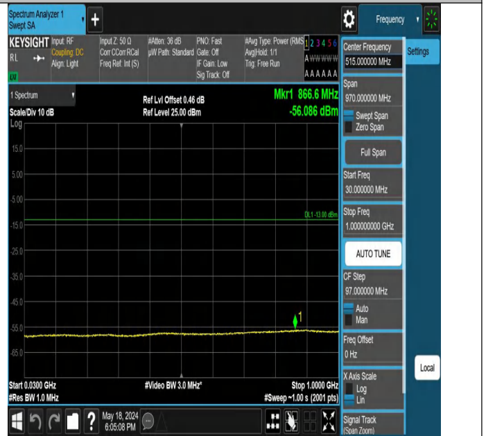
Band2-9538-4-30~1000MHz-PASS
