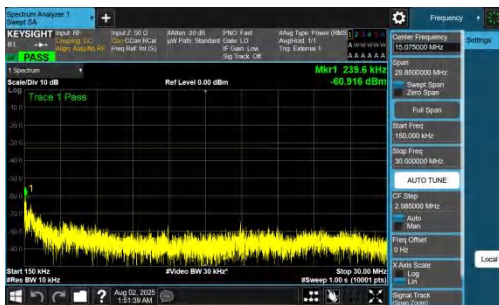
NTNV-DC_7A_n78A-PC2-30-5+60-M+H-QPSK-IDLE-DFT-QPSK-Inner_1RB_Right-0.15-30-PASS
