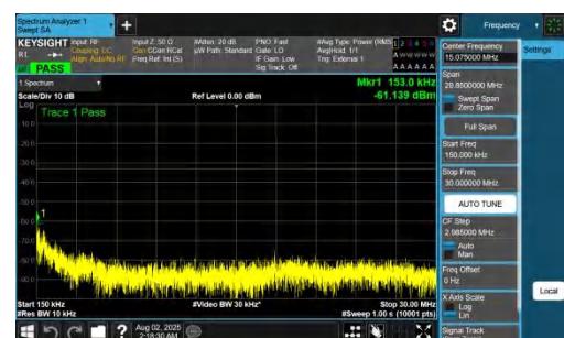
NTNV-DC_7A_n78A-PC2-30-5+70-M+H-QPSK-IDLE-DFT-QPSK-In ner_1RB_Left-0.15-30-PASS
