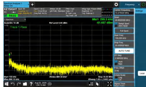
NTNV-DC_7A_n78A-PC2-30-5+70-M+L-QPSK-IDLE-DFT-BPSK-In ner_1RB_Left-0.15-30-PASS
