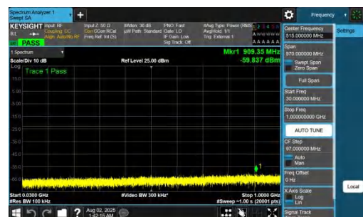
NTNV-DC_7A_n78A-PC2-30-5+60-M+M-QPSK-IDLE-DFT-QPSK-In ner_1RB_Right-30-1000-PASS
