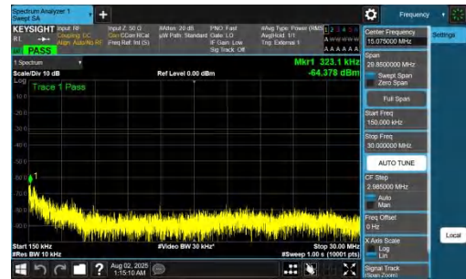
NTNV-DC_7A_n78A-PC2-30-5+50-M+H-QPSK-IDLE-DFT-BPSK-Inner_1RB_Left-0.15-30-PASS
