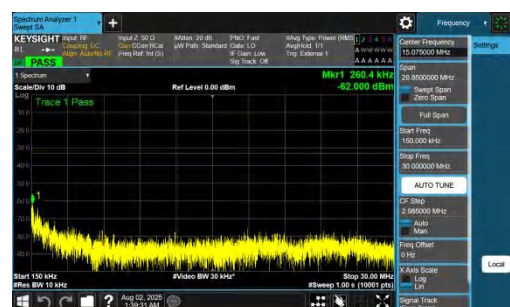
NTNV-DC_7A_n78A-PC2-30-5+60-M+M-QPSK-IDLE-DFT-QPSK-In ner_1RB_Left-0.15-30-PASS
