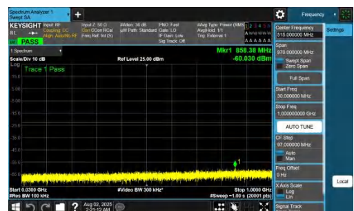
NTNV-DC_7A_n78A-PC2-30-5+70-M+H-QPSK-IDLE-DFT-QPSK-In ner_1RB_Right-30-1000-PASS
