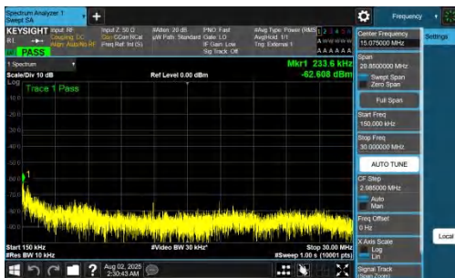
NTNV-DC_7A_n78A-PC2-30-5+80-M+L-QPSK-IDLE-DFT-QPSK-In ner_1RB_Right-0.15-30-PASS
