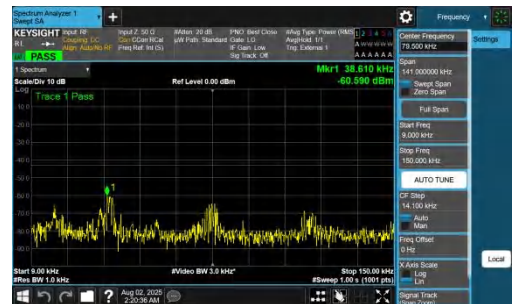
NTNV-DC_7A_n78A-PC2-30-5+70-M+H-QPSK-IDLE-DFT-QPSK-In ner_1RB_Right-0.009-0.15-PASS
