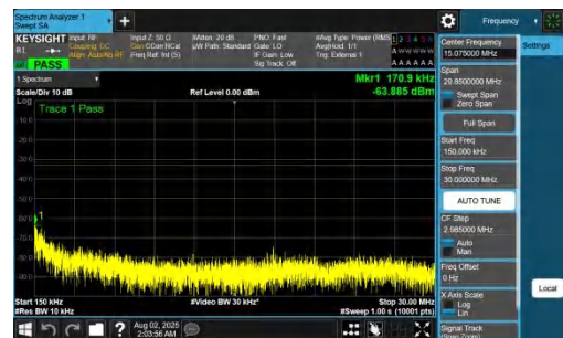
NTNV-DC_7A_n78A-PC2-30-5+70-M+M-QPSK-IDLE-DFT-BPSK-In_ner_1RB_Left-0.15-30-PASS
