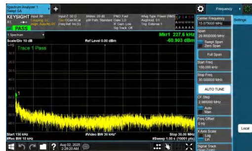
NTNV-DC_7A_n78A-PC2-30-5+80-M+L-QPSK-IDLE-DFT-QPSK-In ner_1RB_Left-0.15-30-PASS
