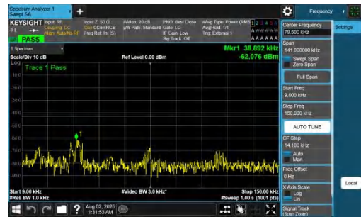
NTNV-DC_7A_n78A-PC2-30-5+60-M+L-QPSK-IDLE-DFT-QPSK-In ner_1RB_Right-0.009-0.15-PASS
