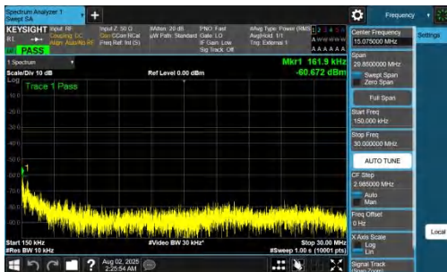
NTNV-DC_7A_n78A-PC2-30-5+80-M+L-QPSK-IDLE-DFT-BPSK-In ner_1RB_Right-0.15-30-PASS
