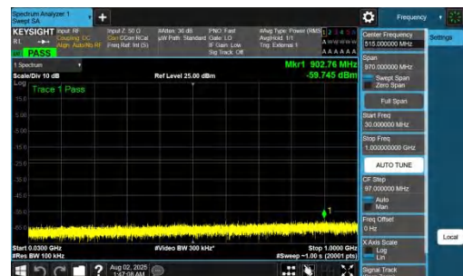
NTNV-DC_7A_n78A-PC2-30-5+60-M+H-QPSK-IDLE-DFT-BPSK-In ner_1RB_Right-30-1000-PASS
