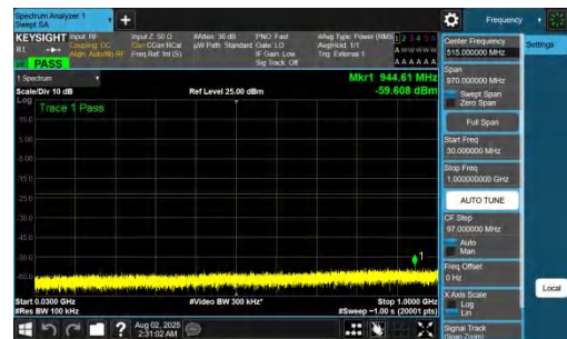
NTNV-DC_7A_n78A-PC2-30-5+80-M+L-QPSK-IDLE-DFT-QPSK-In ner_1RB_Right-30-1000-PASS
