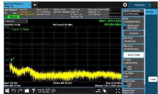
NTNV-DC_7A_n78A-PC2-30-5+70-M+H-QPSK-IDLE-DFT-BPSK-Inner_1RB_Left-0.15-30-PASS
