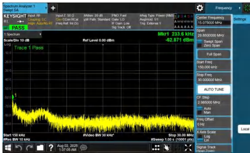
NTNV-DC_7A_n78A-PC2-30-5+60-M+M-QPSK-IDLE-DFT-BPSK-In nner_1RB_Right-0.15-30-PASS
