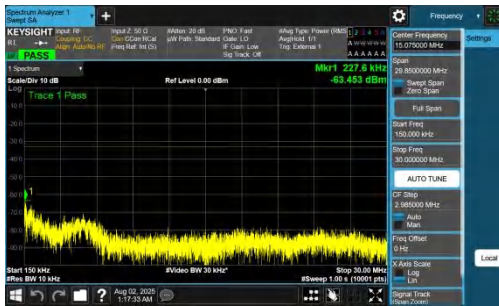
NTNV-DC_7A_n78A-PC2-30-5+50-M+H-QPSK-IDLE-DFT-BPSK-I nner_1RB_Right-0.15-30-PASS
