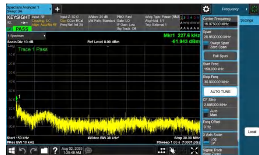
NTNV-DC_7A_n78A-PC2-30-5+60-M+L-QPSK-IDLE-DFT-QPSK-In ner_1RB_Left-0.15-30-PASS
