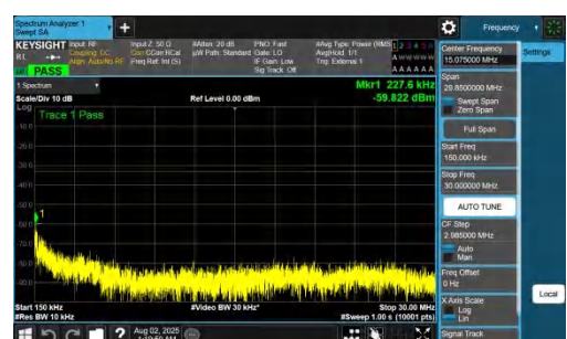
NTNV-DC_7A_n78A-PC2-30-5+50-M+H-QPSK-IDLE-DFT-QPSK-In ner_1RB_Left-0.15-30-PASS
