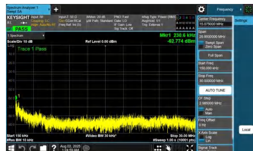
NTNV-DC_7A_n78A-PC2-30-5+60-M+L-QPSK-IDLE-DFT-BPSK-Inner_1RB_Left-0.15-30-PASS
