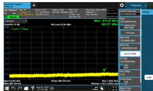
NTNV-DC_7A_n78A-PC2-30-5+70-M+M-QPSK-IDLE-DFT-QPSK-Inner_1RB_Right-30-1000-PASS
