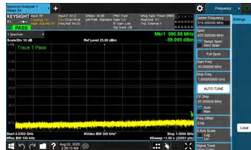
NTNV-DC_7A_n78A-PC2-30-5+80-M+L-QPSK-IDLE-DFT-BPSK-In ner_1RB_Right-30-1000-PASS
