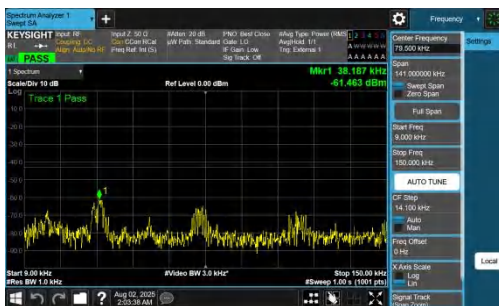
NTNV-DC_7A_n78A-PC2-30-5+70-M+M-QPSK-IDLE-DFT-BPSK-In_ner_1RB_Left-0.009-0.15-PASS
