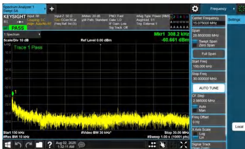
NTNV-DC_7A_n78A-PC2-30-5+60-M+L-QPSK-IDLE-DFT-QPSK-In ner_1RB_Right-0.15-30-PASS
