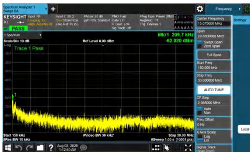
NTNV-DC_7A_n78A-PC2-30-5+50-M+M-QPSK-IDLE-DFT-QPSK-Inner_1RB_Right-0.15-30-PASS
