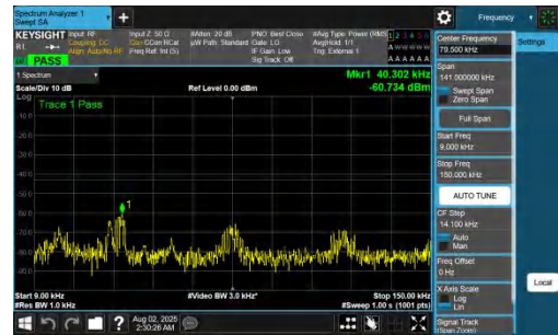
NTNV-DC_7A_n78A-PC2-30-5+80-M+L-QPSK-IDLE-DFT-QPSK-In ner_1RB_Right-0.009-0.15-PASS
