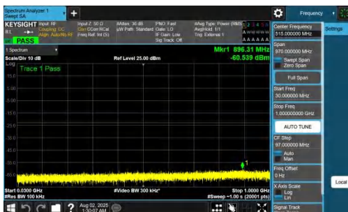
NTNV-DC_7A_n78A-PC2-30-5+60-M+L-QPSK-IDLE-DFT-QPSK-In ner_1RB_Left-30-1000-PASS
