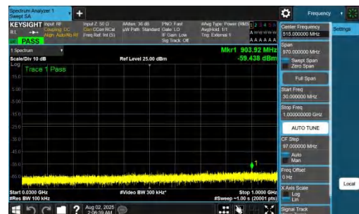
NTNV-DC_7A_n78A-PC2-30-5+70-M+M-QPSK-IDLE-DFT-BPSK-Inner_1RB_Right-30-1000-PASS
