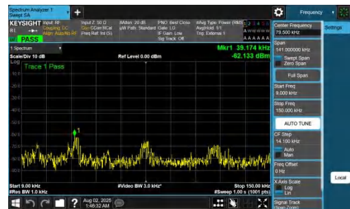
NTNV-DC_7A_n78A-PC2-30-5+60-M+H-QPSK-IDLE-DFT-BPSK-In ner_1RB_Right-0.009-0.15-PASS
