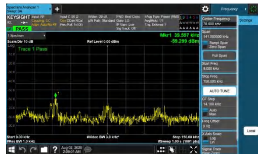
NTNV-DC_7A_n78A-PC2-30-5+70-M+M-QPSK-IDLE-DFT-BPSK-Inner_1RB_Right-0.009-0.15-PASS
