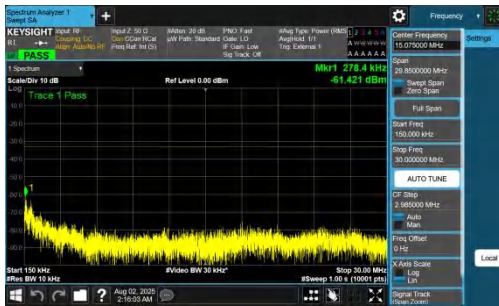
NTNV-DC_7A_n78A-PC2-30-5+70-M+H-QPSK-IDLE-DFT-BPSK-In nner_1RB_Right-0.15-30-PASS
