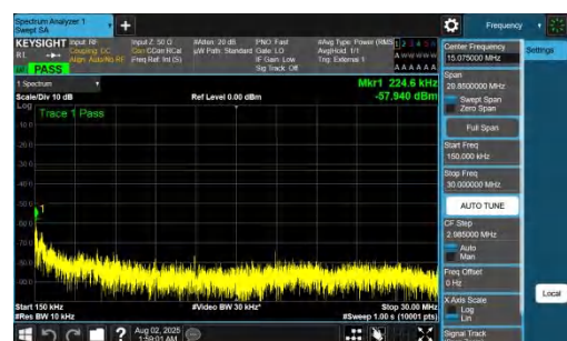
NTNV-DC_7A_n78A-PC2-30-5+70-M+L-QPSK-IDLE-DFT-QPSK-In ner_1RB_Left-0.15-30-PASS
