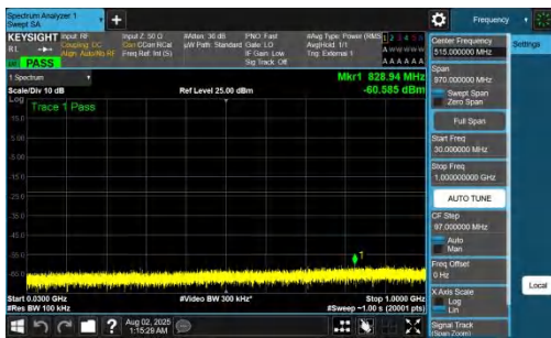
NTNV-DC_7A_n78A-PC2-30-5+50-M+H-QPSK-IDLE-DFT-BPSK-Inner_1RB_Left-30-1000-PASS
