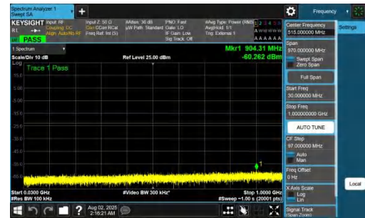
NTNV-DC_7A_n78A-PC2-30-5+70-M+H-QPSK-IDLE-DFT-BPSK-In ner_1RB_Right-30-1000-PASS
