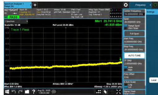
NTNV-DC_7A_n78A-PC2-30-5+50-M+M-QPSK-IDLE-DFT-BPSK-In ner_1RB_Left-6000-26000-PASS
