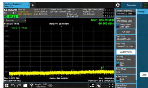
NTNV-DC_7A_n78A-PC2-30-5+60-M+L-QPSK-IDLE-DFT-QPSK-In ner_1RB_Right-30-1000-PASS
