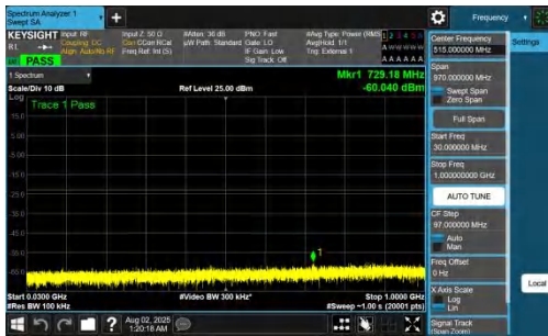
NTNV-DC_7A_n78A-PC2-30-5+50-M+H-QPSK-IDLE-DFT-QPSK-I nner_1RB_Left-30-1000-PASS
