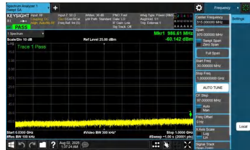
NTNV-DC_7A_n78A-PC2-30-5+60-M+M-QPSK-IDLE-DFT-BPSK-In ner_1RB_Right-30-1000-PASS
