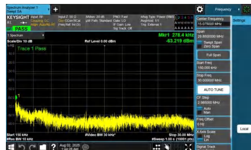
NTNV-DC_7A_n78A-PC2-30-5+60-M+H-QPSK-IDLE-DFT-BPSK-Inner_1RB_Left-0.15-30-PASS
