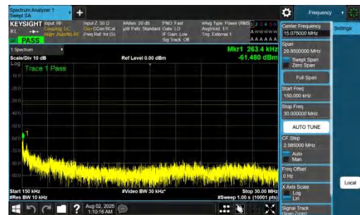
NTNV-DC_7A_n78A-PC2-30-5+50-M+M-QPSK-IDLE-DFT-QPSK-Inner_1RB_Left-0.15-30-PASS
