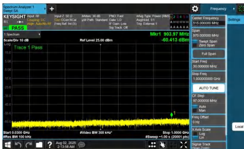
NTNV-DC_7A_n78A-PC2-30-5+70-M+H-QPSK-IDLE-DFT-BPSK-Inner_1RB_Left-30-1000-PASS
