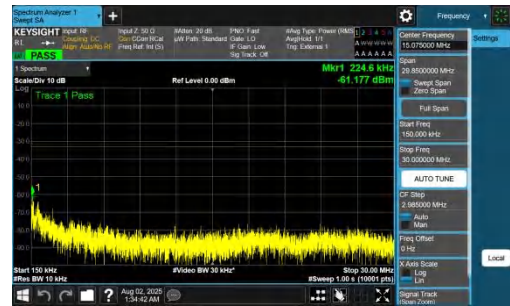
NTNV-DC_7A_n78A-PC2-30-5+60-M+M-QPSK-IDLE-DFT-BPSK-In ner_1RB_Left-0.15-30-PASS
