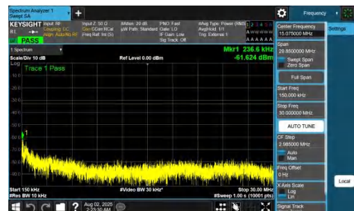
NTNV-DC_7A_n78A-PC2-30-5+80-M+L-QPSK-IDLE-DFT-BPSK-Inner_1RB_Left-0.15-30-PASS
