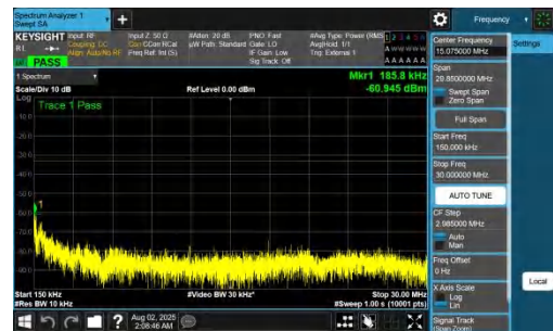
NTVN-DC_7A_n78A-PC2-30-5+70-M+M-QPSK-IDLE-DFT-QPSK-Inner_1RB_Left-0.15-30-PASS
