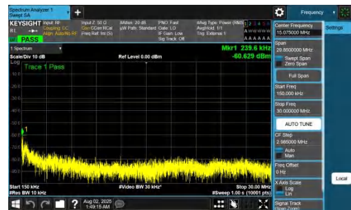
NTNV-DC_7A_n78A-PC2-30-5+60-M+H-QPSK-IDLE-DFT-QPSK-Inner_1RB_Left-0.15-30-PASS
