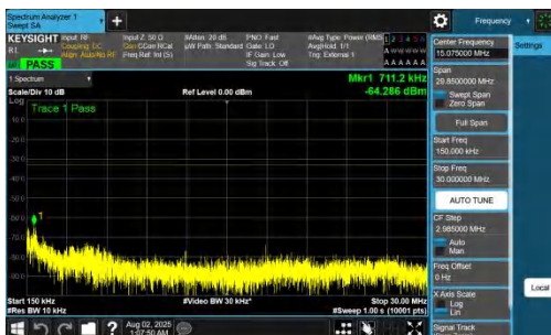
NTNV-DC_7A_n78A-PC2-30-5+50-M+M-QPSK-IDLE-DFT-BPSK-I nner_1RB_Right-0.15-30-PASS
