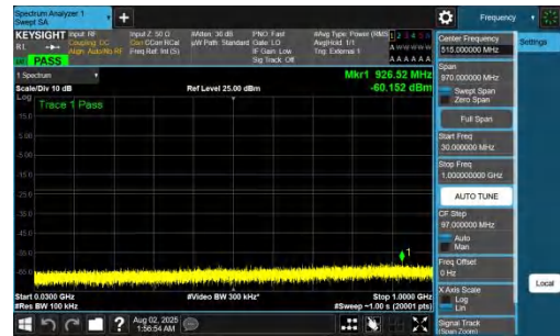
NTNV-DC_7A_n78A-PC2-30-5+70-M+L-QPSK-IDLE-DFT-BPSK-In ner_1RB_Right-30-1000-PASS
