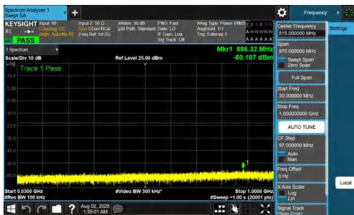
NTNV-DC_7A_n78A-PC2-30-5+60-M+M-QPSK-IDLE-DFT-BPSK-In nner_1RB_Left-30-1000-PASS
