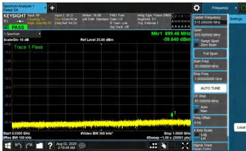
NTNV-DC_7A_n78A-PC2-30-5+70-M+H-QPSK-IDLE-DFT-QPSK-I nner_1RB_Left-30-1000-PASS
