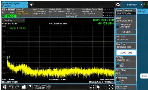
NTNV-DC_7A_n78A-PC2-30-5+70-M+L-QPSK-IDLE-DFT-BPSK-In ner_1RB_Right-0.15-30-PASS
