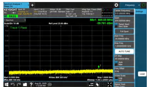
NTNV-DC_7A_n78A-PC2-30-5+50-M+M-QPSK-IDLE-DFT-QPSK-Inner_1RB_Right-30-1000-PASS
