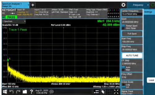
NTNV-DC_7A_n78A-PC2-30-5+30-M+L-QPSK-IDLE-DFT-BPSK-In ner_1RB_Right-0.15-30-PASS
