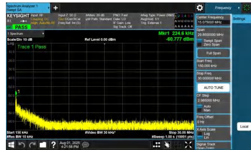
NTVN-DC_7A_n78A-PC2-30-5+40-M+M-QPSK-IDLE-DFT-BPSK-Inner_1RB_Left-0.15-30-PASS
