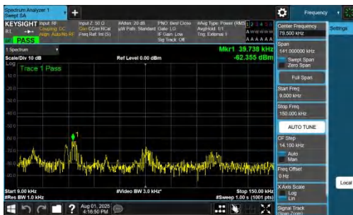
NTNV-DC_7A_n78A-PC2-30-5+40-M+L-QPSK-IDLE-DFT-QPSK-In ner_1RB_Left-0.009-0.15-PASS
