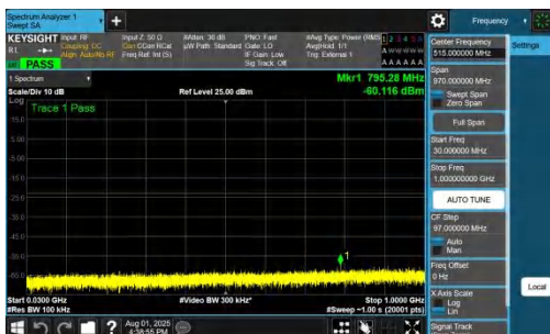
NTNV-DC_7A_n78A-PC2-30-5+40-M+H-QPSK-IDLE-DFT-QPSK-Inner_1RB_Left-30-1000-PASS
