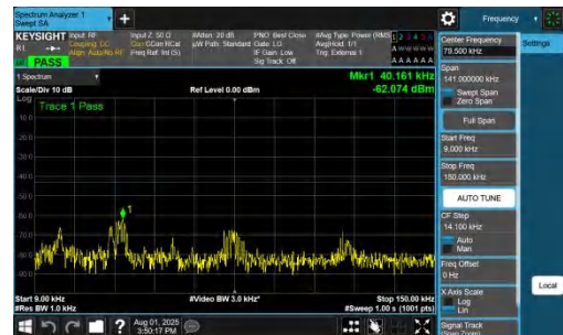
NTNV-DC_7A_n78A-PC2-30-5+30-M+L-QPSK-IDLE-DFT-QPSK-In ner_1RB_Right-0.009-0.15-PASS
