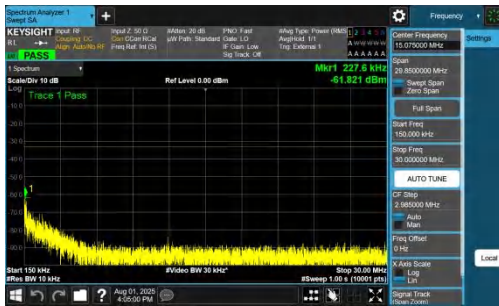
NTVN-DC_7A_n78A-PC2-30-5+30-M+H-QPSK-IDLE-DFT-BPSK-Inner_1RB_Right-0.15-30-PASS
