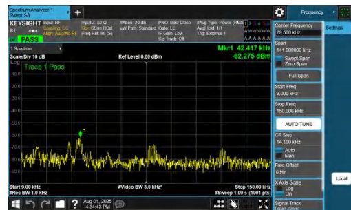
NTNV-DC_7A_n78A-PC2-30-5+40-M+H-QPSK-IDLE-DFT-BPSK-In ner_1RB_Right-0.009-0.15-PASS
