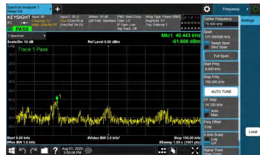
NTVN-DC_7A_n78A-PC2-30-5+30-M+M-QPSK-IDLE-DFT-BPSK-Inner_1RB_Right-0.009-0.15-PASS
