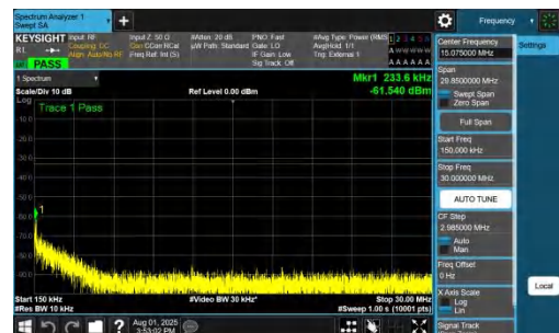
NTNV-DC_7A_n78A-PC2-30-5+30-M+M-QPSK-IDLE-DFT-BPSK-In_ner_1RB_Left-0.15-30-PASS
