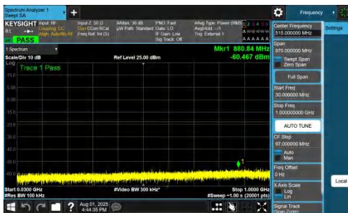
NTNV-DC_7A_n78A-PC2-30-5+50-M+L-QPSK-IDLE-DFT-BPSK-In ner_1RB_Left-30-1000-PASS
