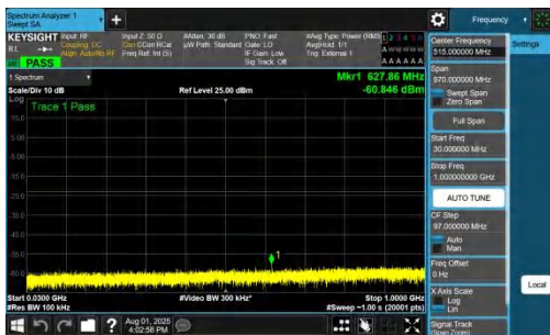
NTNV-DC_7A_n78A-PC2-30-5+30-M+H-QPSK-IDLE-DFT-BPSK-I nner_1RB_Left-30-1000-PASS
