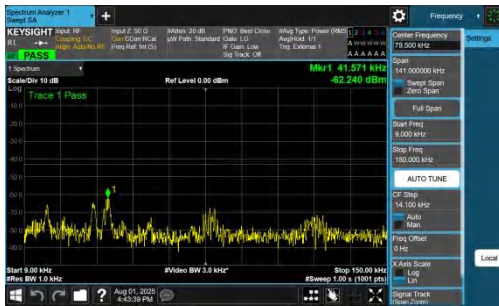
NTNV-DC_7A_n78A-PC2-30-5+50-M+L-QPSK-IDLE-DFT-BPSK-In ner_1RB_Left-0.009-0.15-PASS
