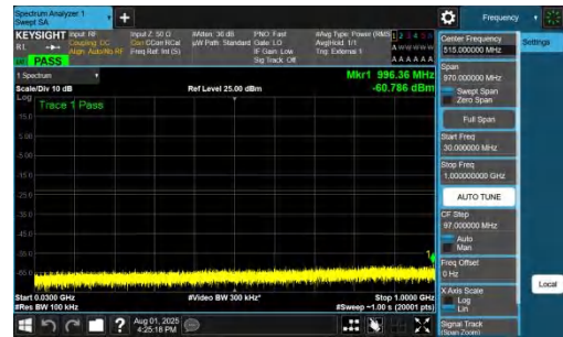
NTNV-DC_7A_n78A-PC2-30-5+40-M+M-QPSK-IDLE-DFT-BPSK-In ner_1RB_Right-30-1000-PASS
