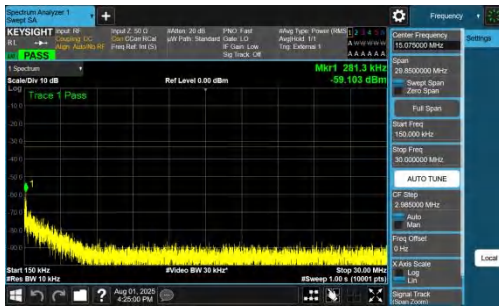
NTNV-DC_7A_n78A-PC2-30-5+40-M+M-QPSK-IDLE-DFT-BPSK-In nner_1RB_Right-0.15-30-PASS
