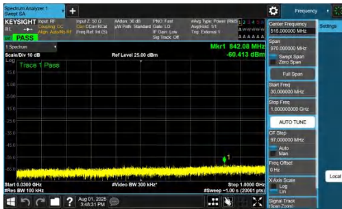
NTNV-DC_7A_n78A-PC2-30-5+30-M+L-QPSK-IDLE-DFT-QPSK-In ner_1RB_Left-30-1000-PASS
