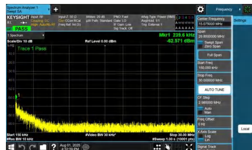
NTNV-DC_7A_n78A-PC2-30-5+40-M+H-QPSK-IDLE-DFT-BPSK-Inner_1RB_Left-0.15-30-PASS
