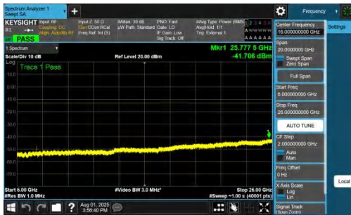
NTNV-DC_7A_n78A-PC2-30-5+30-M+M-QPSK-IDLE-DFT-BPSK-Inner_1RB_Right-6000-26000-PASS
