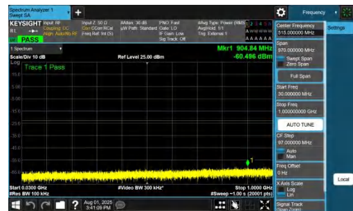
NTNV-DC_7A_n78A-PC2-30-5+25-M+H-QPSK-IDLE-DFT-QPSK-Inner_1RB_Right-30-1000-PASS
