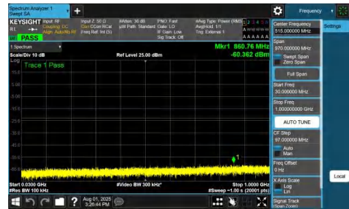
NTNV-DC_7A_n78A-PC2-30-5+25-M+M-QPSK-IDLE-DFT-BPSK-In ner_1RB_Right-30-1000-PASS
