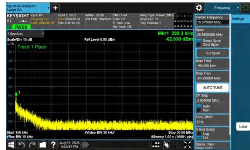
NTNV-DC_7A_n78A-PC2-30-5+50-M+L-QPSK-IDLE-DFT-BPSK-In ner_1RB_Left-0.15-30-PASS
