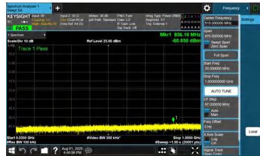
NTNV-DC_7A_n78A-PC2-30-5+50-M+L-QPSK-IDLE-DFT-BPSK-In ner_1RB_Right-30-1000-PASS
