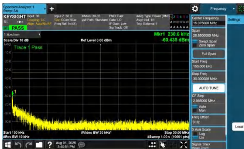
NTNV-DC_7A_n78A-PC2-30-5+25-M+H-QPSK-IDLE-DFT-QPSK-Inner_1RB_Right-0.15-30-PASS
