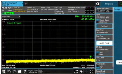
NTNV-DC_7A_n78A-PC2-30-5+40-M+M-QPSK-IDLE-DFT-QPSK-I nner_1RB_Left-30-1000-PASS
