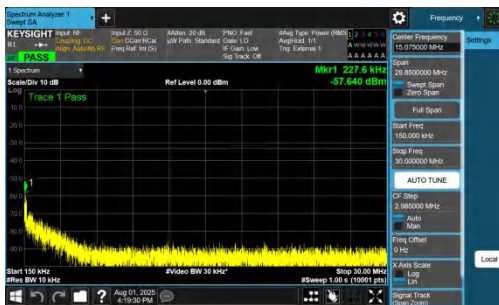
NTNV-DC_7A_n78A-PC2-30-5+40-M+L-QPSK-IDLE-DFT-QPSK-In ner_1RB_Right-0.15-30-PASS
