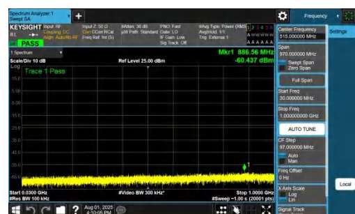
NTNV-DC_7A_n78A-PC2-30-5+30-M+H-QPSK-IDLE-DFT-QPSK-In ner_1RB_Right-30-1000-PASS
