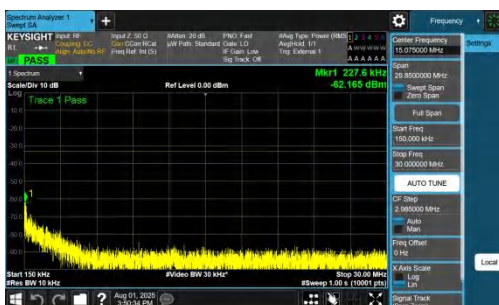
NTNV-DC_7A_n78A-PC2-30-5+30-M+L-QPSK-IDLE-DFT-QPSK-In ner_1RB_Right-0.15-30-PASS
