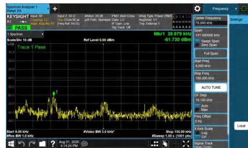
NTNV-DC_7A_n78A-PC2-30-5+40-M+L-QPSK-IDLE-DFT-BPSK-In ner_1RB_Right-0.009-0.15-PASS
