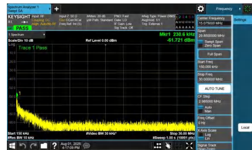
NTNV-DC_7A_n78A-PC2-30-5+40-M+L-QPSK-IDLE-DFT-QPSK-In ner_1RB_Left-0.15-30-PASS
