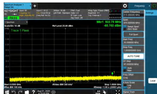
NTNV-DC_7A_n78A-PC2-30-5+40-M+L-QPSK-IDLE-DFT-BPSK-In ner_1RB_Right-30-1000-PASS
