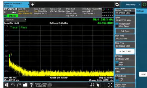
NTNV-DC_7A_n78A-PC2-30-5+30-M+L-QPSK-IDLE-DFT-BPSK-In ner_1RB_Left-0.15-30-PASS
