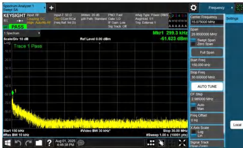
NTNV-DC_7A_n78A-PC2-30-5+50-M+L-QPSK-IDLE-DFT-BPSK-In ner_1RB_Right-0.15-30-PASS
