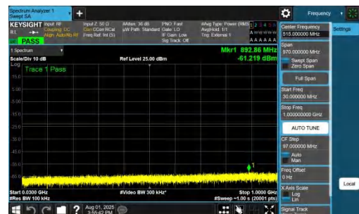
NTVN-DC_7A_n78A-PC2-30-5+30-M+M-QPSK-IDLE-DFT-BPSK-Inner_1RB_Right-30-1000-PASS
