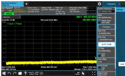
NTNV-DC_7A_n78A-PC2-30-5+50-M+L-QPSK-IDLE-DFT-QPSK-In ner_1RB_Left-30-1000-PASS
