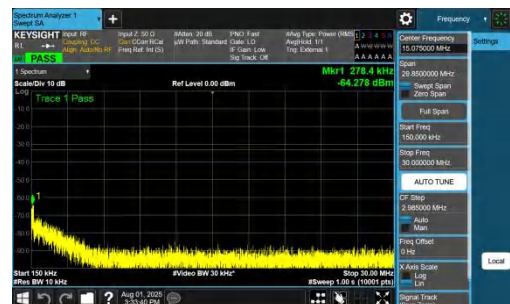
NTNV-DC_7A_n78A-PC2-30-5+25-M+H-QPSK-IDLE-DFT-BPSK-Inner_1RB_Left-0.15-30-PASS
