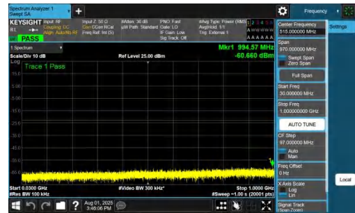
NTNV-DC_7A_n78A-PC2-30-5+30-M+L-QPSK-IDLE-DFT-BPSK-In ner_1RB_Right-30-1000-PASS
