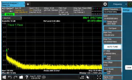
NTNV-DC_7A_n78A-PC2-30-5+25-M+M-QPSK-IDLE-DFT-BPSK-In nner_1RB_Right-0.15-30-PASS
