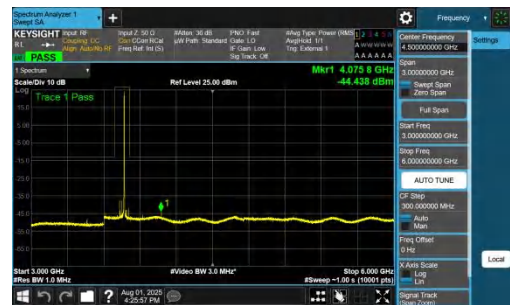
NTNV-DC_7A_n78A-PC2-30-5+40-M+M-QPSK-IDLE-DFT-BPSK-In ner_1RB_Right-3000-6000-PASS
