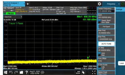
NTVN-DC_7A_n78A-PC2-30-5+30-M+H-QPSK-IDLE-DFT-BPSK-Inner_1RB_Right-30-1000-PASS
