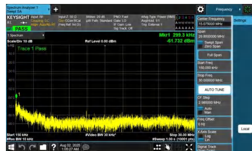
NTNV-DC_7A_n78A-PC2-30-5+50-M+M-QPSK-IDLE-DFT-BPSK-In ner_1RB_Left-0.15-30-PASS
