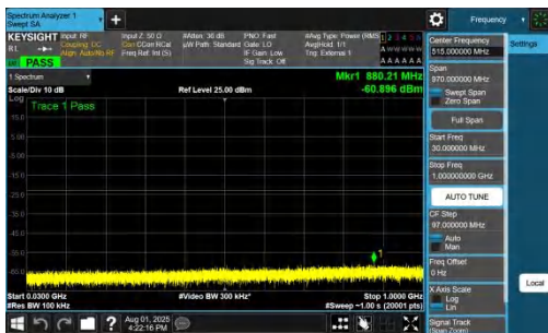
NTVN-DC_7A_n78A-PC2-30-5+40-M+M-QPSK-IDLE-DFT-BPSK-Inner_1RB_Left-30-1000-PASS
