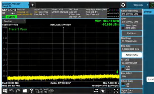
NTNV-DC_7A_n78A-PC2-30-5+30-M+H-QPSK-IDLE-DFT-QPSK-I nner_1RB_Left-30-1000-PASS
