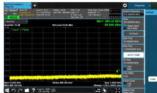
NTNV-DC_7A_n78A-PC2-30-5+40-M+H-QPSK-IDLE-DFT-QPSK-In ner_1RB_Right-30-1000-PASS
