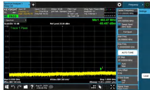
NTNV-DC_7A_n78A-PC2-30-5+10-M+H-QPSK-IDLE-DFT-BPSK-Inner_1RB_Right-30-1000-PASS
