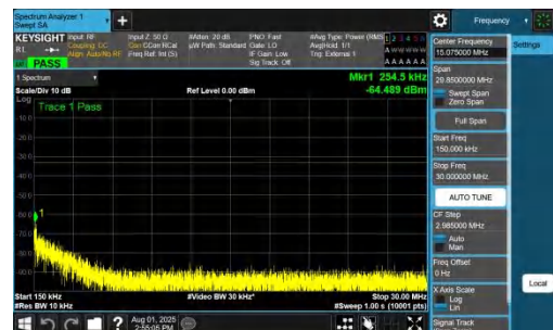
NTNV-DC_7A_n78A-PC2-30-5+20-M+M-QPSK-IDLE-DFT-BPSK-In ner_1RB_Left-0.15-30-PASS
