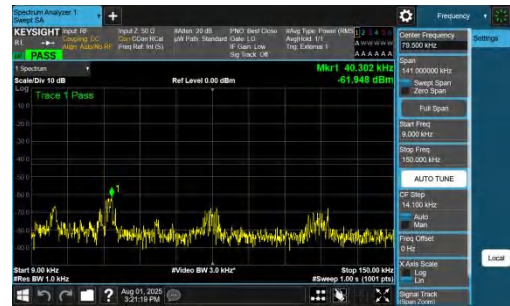
NTNV-DC_7A_n78A-PC2-30-5+25-M+L-QPSK-IDLE-DFT-QPSK-In ner_1RB_Right-0.009-0.15-PASS
