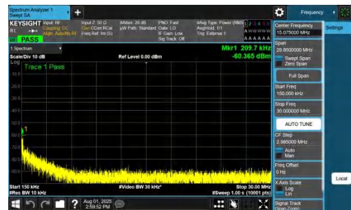
NTNV-DC_7A_n78A-PC2-30-5+20-M+M-QPSK-IDLE-DFT-QPSK-Inner_1RB_Left-0.15-30-PASS
