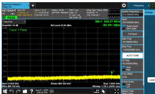
NTNV-DC_7A_n78A-PC2-30-5+20-M+H-QPSK-IDLE-DFT-BPSK-In nner_1RB_Left-30-1000-PASS
