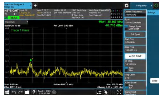
NTNV-DC_7A_n78A-PC2-30-5+15-M+L-QPSK-IDLE-DFT-BPSK-In ner_1RB_Right-0.009-0.15-PASS
