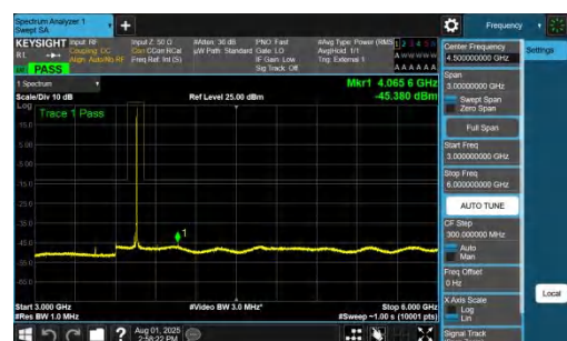
NTVN-DC_7A_n78A-PC2-30-5+20-M+M-QPSK-IDLE-DFT-BPSK-In ner_1RB_Right-3000-6000-PASS
