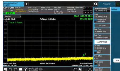
NTNV-DC_7A_n78A-PC2-30-5+15-M+L-QPSK-IDLE-DFT-BPSK-In ner_1RB_Right-30-1000-PASS
