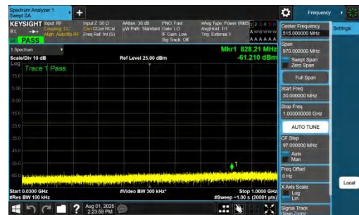
NTNV-DC_7A_n78A-PC2-30-5+15-M+L-QPSK-IDLE-DFT-QPSK-In ner_1RB_Right-30-1000-PASS
