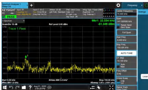
NTNV-DC_7A_n78A-PC2-30-5+10-M+M-QPSK-IDLE-DFT-QPSK-Inner_1RB_Left-0.009-0.15-PASS
