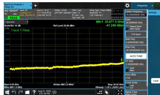
NTNV-DC_7A_n78A-PC2-30-5+20-M+L-QPSK-IDLE-DFT-QPSK-In ner_1RB_Left-6000-26000-PASS
