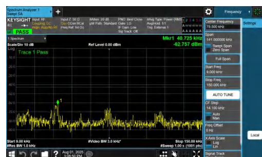
NTNV-DC_7A_n78A-PC2-30-5+20-M+H-QPSK-IDLE-DFT-BPSK-In ner_1RB_Right-0.009-0.15-PASS
