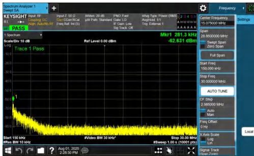
NTNV-DC_7A_n78A-PC2-30-5+15-M+M-QPSK-IDLE-DFT-BPSK-In nner_1RB_Right-0.15-30-PASS
