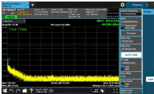
NTNV-DC_7A_n78A-PC2-30-5+10-M+H-QPSK-IDLE-DFT-BPSK-Inner_1RB_Right-0.15-30-PASS
