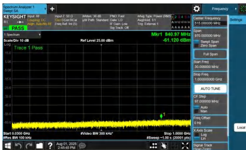
NTNV-DC_7A_n78A-PC2-30-5+20-M+L-QPSK-IDLE-DFT-BPSK-In ner_1RB_Left-30-1000-PASS
