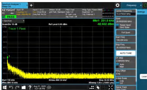
NTNV-DC_7A_n78A-PC2-30-5+25-M+L-QPSK-IDLE-DFT-QPSK-In ner_1RB_Right-0.15-30-PASS
