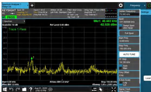
NTNV-DC_7A_n78A-PC2-30-5+15-M+H-QPSK-IDLE-DFT-QPSK-Inner_1RB_Left-0.009-0.15-PASS
