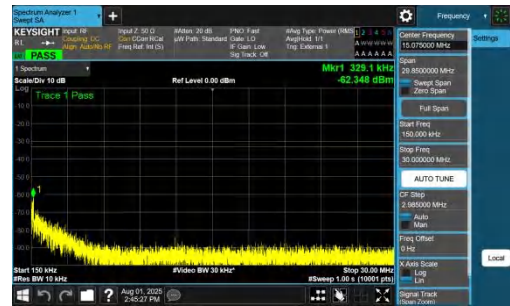
NTNV-DC_7A_n78A-PC2-30-5+20-M+L-QPSK-IDLE-DFT-BPSK-In ner_1RB_Left-0.15-30-PASS
