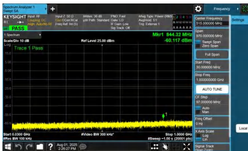
NTVN-DC_7A_n78A-PC2-30-5+15-M+M-QPSK-IDLE-DFT-BPSK-Inner_1RB_Left-30-1000-PASS
