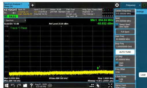
NTNV-DC_7A_n78A-PC2-30-5+25-M+L-QPSK-IDLE-DFT-QPSK-In ner_1RB_Right-30-1000-PASS
