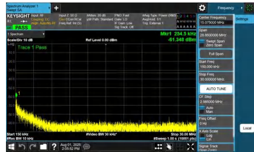
NTNV-DC_7A_n78A-PC2-30-5+10-M+H-QPSK-IDLE-DFT-BPSK-In ner_1RB_Left-0.15-30-PASS
