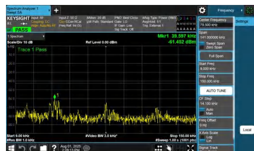
NTVN-DC_7A_n78A-PC2-30-5+15-M+M-QPSK-IDLE-DFT-BPSK-Inner_1RB_Right-0.009-0.15-PASS
