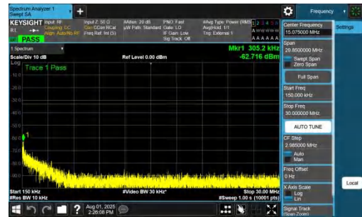
NTVN-DC_7A_n78A-PC2-30-5+15-M+M-QPSK-IDLE-DFT-BPSK-Inner_1RB_Left-0.15-30-PASS
