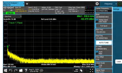
NTNV-DC_7A_n78A-PC2-30-5+20-M+H-QPSK-IDLE-DFT-BPSK-In ner_1RB_Left-0.15-30-PASS
