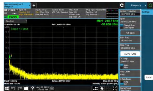
NTNV-DC_7A_n78A-PC2-30-5+25-M+L-QPSK-IDLE-DFT-QPSK-In ner_1RB_Left-0.15-30-PASS
