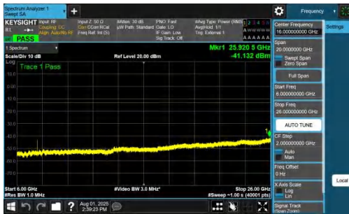
NTNV-DC_7A_n78A-PC2-30-5+15-M+H-QPSK-IDLE-DFT-BPSK-Inner_1RB_Right-6000-26000-PASS
