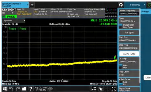
NTNV-DC_7A_n78A-PC2-30-5+10-M+M-QPSK-IDLE-DFT-BPSK-Inner_1RB_Right-6000-26000-PASS
