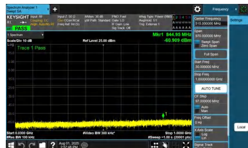
NTVN-DC_7A_n78A-PC2-30-5+20-M+M-QPSK-IDLE-DFT-BPSK-In ner_1RB_Right-30-1000-PASS
