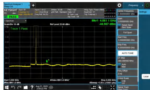
NTNV-DC_7A_n78A-PC2-30-5+10-M+H-QPSK-IDLE-DFT-BPSK-Inner_1RB_Right-3000-6000-PASS
