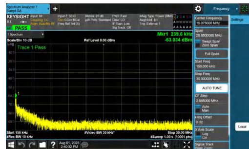
NTNV-DC_7A_n78A-PC2-30-5+15-M+H-QPSK-IDLE-DFT-QPSK-Inner_1RB_Left-0.15-30-PASS
