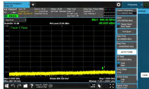
NTNV-DC_7A_n78A-PC2-30-5+20-M+L-QPSK-IDLE-DFT-BPSK-In ner_1RB_Right-30-1000-PASS
