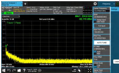
NTNV-DC_7A_n78A-PC2-30-5+20-M+L-QPSK-IDLE-DFT-BPSK-In ner_1RB_Right-0.15-30-PASS
