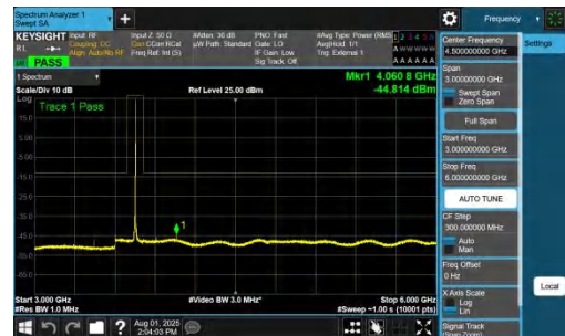
NTNV-DC_7A_n78A-PC2-30-5+10-M+M-QPSK-IDLE-DFT-QPSK-Inner_1RB_Right-3000-6000-PASS
