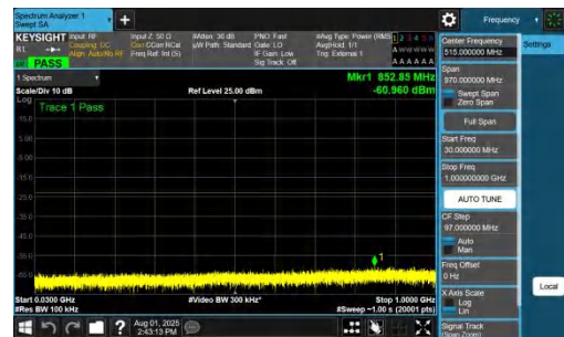
NTV-DC_7A_n78A-PC2-30-5+15-M+H-QPSK-IDLE-DFT-QPSK-Inner_1RB_Right-30-1000-PASS
