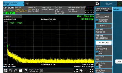
NTVN-DC_7A_n78A-PC2-30-5+25-M+M-QPSK-IDLE-DFT-BPSK-Inner_1RB_Left-0.15-30-PASS
