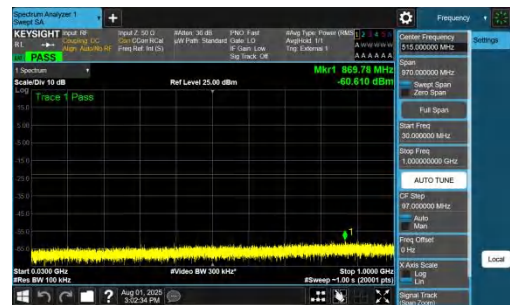
NTNV-DC_7A_n78A-PC2-30-5+20-M+M-QPSK-IDLE-DFT-QPSK-Inner_1RB_Right-30-1000-PASS
