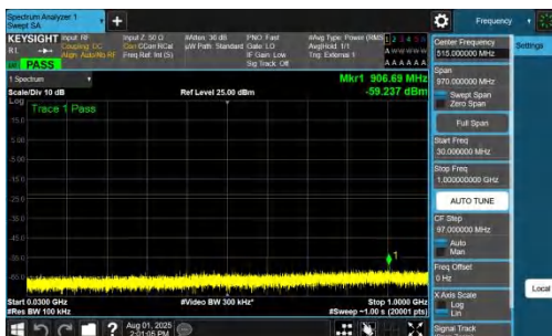
NTNV-DC_7A_n78A-PC2-30-5+10-M+M-QPSK-IDLE-DFT-QPSK-Inner_1RB_Left-30-1000-PASS
