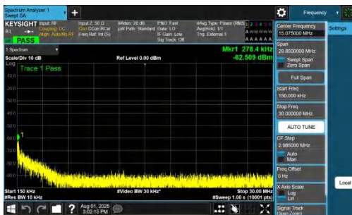
NTNV-DC_7A_n78A-PC2-30-5+20-M+M-QPSK-IDLE-DFT-QPSK-Inner_1RB_Right-0.15-30-PASS
