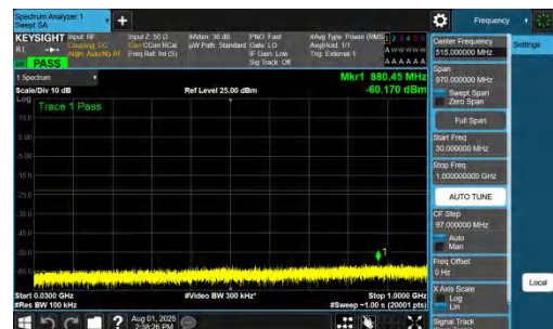
NTNV-DC_7A_n78A-PC2-30-5+15-M+H-QPSK-IDLE-DFT-BPSK-In ner_1RB_Right-30-1000-PASS
