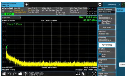
NTNV-DC_7A_n78A-PC2-30-5+15-M+L-QPSK-IDLE-DFT-QPSK-In ner_1RB_Right-0.15-30-PASS
