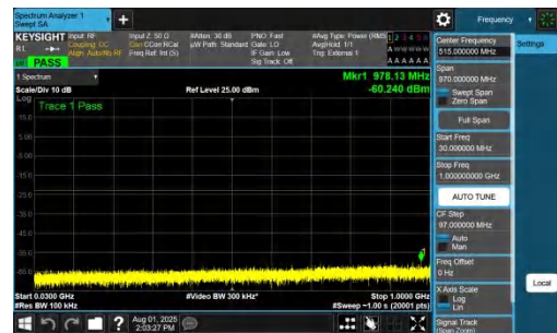
NTNV-DC_7A_n78A-PC2-30-5+10-M+M-QPSK-IDLE-DFT-QPSK-Inner_1RB_Right-30-1000-PASS
