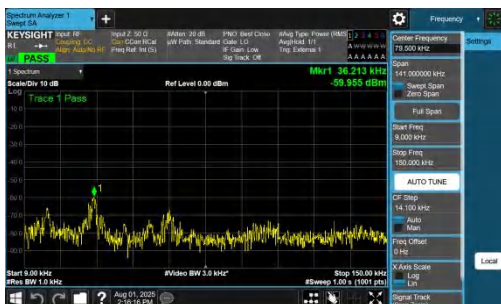
NTNV-DC_7A_n78A-PC2-30-5+15-M+L-QPSK-IDLE-DFT-BPSK-Inner_1RB_Left-0.009-0.15-PASS
