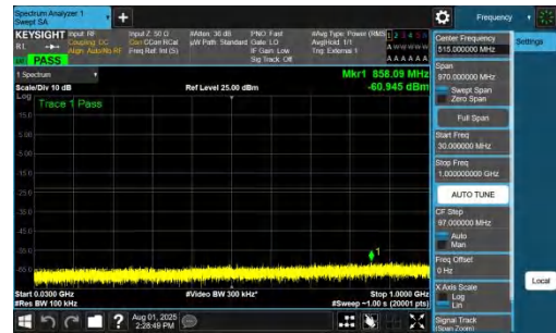
NTNV-DC_7A_n78A-PC2-30-5+15-M+M-QPSK-IDLE-DFT-BPSK-In ner_1RB_Right-30-1000-PASS
