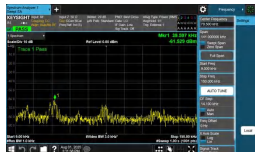
NTNV-DC_7A_n78A-PC2-30-5+20-M+H-QPSK-IDLE-DFT-QPSK-In ner_1RB_Right-0.009-0.15-PASS
