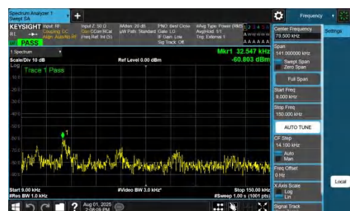
NTNV-DC_7A_n78A-PC2-30-5+10-M+H-QPSK-IDLE-DFT-BPSK-In ner_1RB_Right-0.009-0.15-PASS
