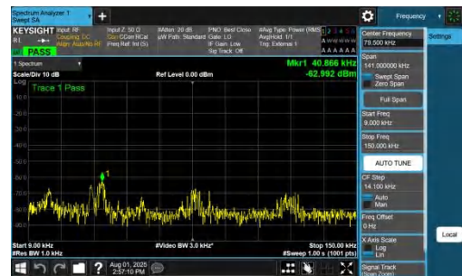
NTVN-DC_7A_n78A-PC2-30-5+20-M+M-QPSK-IDLE-DFT-BPSK-In ner_1RB_Right-0.009-0.15-PASS
