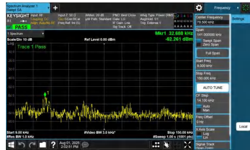
NTNV-DC_7A_n78A-PC2-30-5+10-M+M-QPSK-IDLE-DFT-QPSK-Inner_1RB_Right-0.009-0.15-PASS
