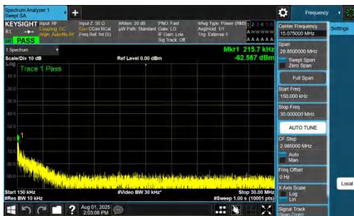
NTNV-DC_7A_n78A-PC2-30-5+10-M+M-QPSK-IDLE-DFT-QPSK-Inner_1RB_Right-0.15-30-PASS
