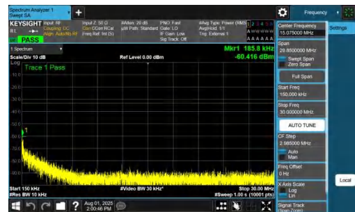
NTNV-DC_7A_n78A-PC2-30-5+10-M+M-QPSK-IDLE-DFT-QPSK-Inner_1RB_Left-0.15-30-PASS
