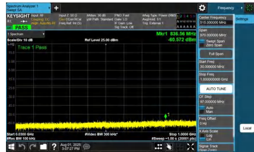
NTNV-DC_7A_n78A-PC2-30-5+20-M+H-QPSK-IDLE-DFT-BPSK-Inner_1RB_Right-30-1000-PASS
