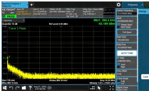
NTNV-DC_7A_n78A-PC2-30-5+20-M+H-QPSK-IDLE-DFT-BPSK-Inner_1RB_Right-0.15-30-PASS
