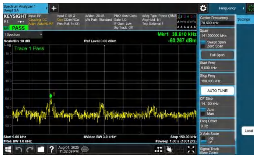
NTNV-DC_7A_n78A-PC2-30-5+90-M+L-QPSK-IDLE-DFT-BPSK-In ner_1RB_Left-0.009-0.15-PASS
