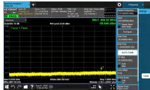
NTVN-DC_7A_n78A-PC2-30-5+90-M+H-QPSK-IDLE-DFT-BPSK-Inner_1RB_Right-30-1000-PASS
