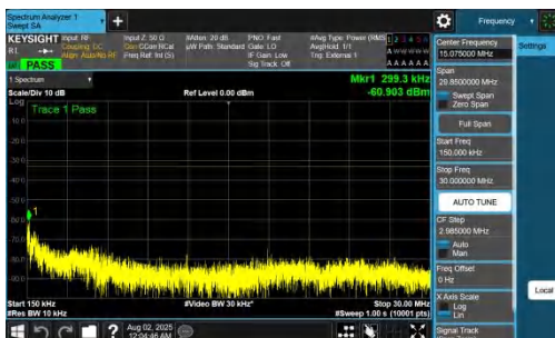
NTNV-DC_7A_n78A-PC2-30-5+100-M+L-QPSK-IDLE-DFT-BPSK-I nner_1RB_Right-0.15-30-PASS
