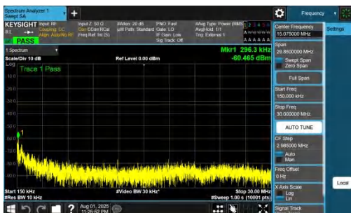
NTNV-DC_7A_n78A-PC2-30-5+80-M+H-QPSK-IDLE-DFT-BPSK-I nner_1RB_Right-0.15-30-PASS
