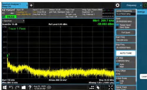
NTNV-DC_7A_n78A-PC2-30-5+100-M+L-QPSK-IDLE-DFT-QPSK-I nner_1RB_Right-0.15-30-PASS
