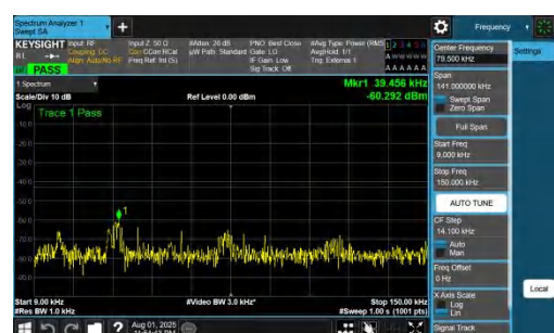
NTNV-DC_7A_n78A-PC2-30-5+90-M+H-QPSK-IDLE-DFT-BPSK-In ner_1RB_Right-0.009-0.15-PASS
