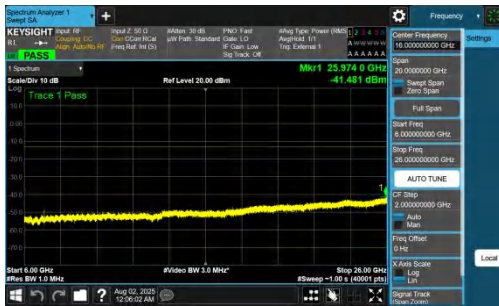
NTNV-DC_7A_n78A-PC2-30-5+100-M+L-QPSK-IDLE-DFT-BPSK-I nner_1RB_Right-6000-26000-PASS
