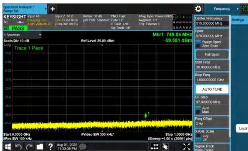
NTNV-DC_7A_n78A-PC2-30-5+90-M+L-QPSK-IDLE-DFT-BPSK-In ner_1RB_Left-30-1000-PASS
