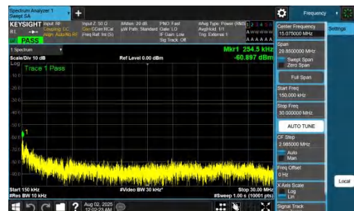
NTNV-DC_7A_n78A-PC2-30-5+100-M+L-QPSK-IDLE-DFT-BPSK-Inner_1RB_Left-0.15-30-PASS
