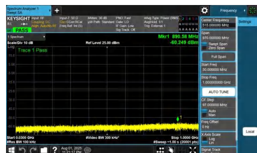
NTNV-DC_7A_n78A-PC2-30-5+80-M+M-QPSK-IDLE-DFT-QPSK-In ner_1RB_Right-30-1000-PASS
