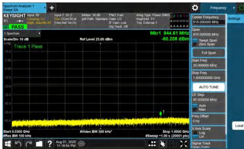
NTNV-DC_7A_n78A-PC2-30-5+80-M+M-QPSK-IDLE-DFT-QPSK-I nner_1RB_Left-30-1000-PASS
