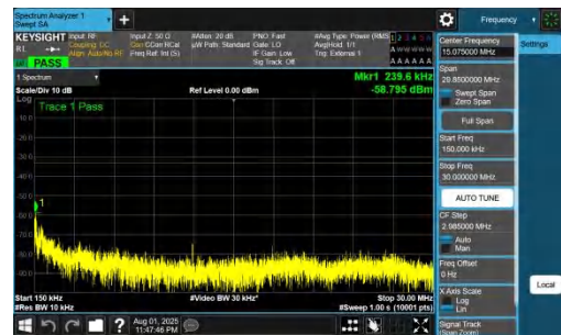
NTVN-DC_7A_n78A-PC2-30-5+90-M+M-QPSK-IDLE-DFT-QPSK-Inner_1RB_Left-0.15-30-PASS
