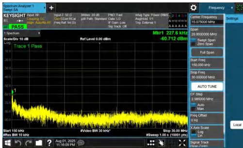
NTNV-DC_7A_n78A-PC2-30-5+80-M+M-QPSK-IDLE-DFT-BPSK-I nner_1RB_Right-0.15-30-PASS
