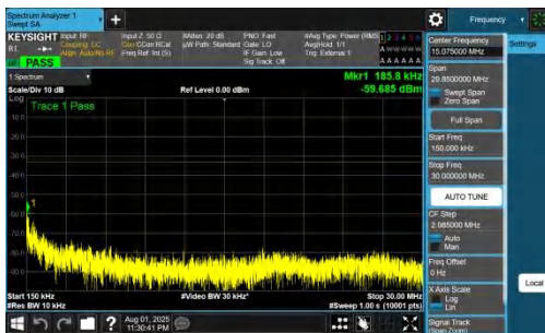
NTNV-DC_7A_n78A-PC2-30-5+80-M+H-QPSK-IDLE-DFT-QPSK-Inner_1RB_Right-0.15-30-PASS
