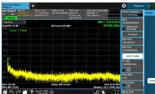
NTNV-DC_7A_n78A-PC2-30-5+90-M+M-QPSK-IDLE-DFT-BPSK-Inner_1RB_Right-0.15-30-PASS
