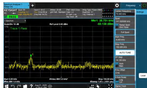
NTNV-DC_7A_n78A-PC2-30-5+80-M+M-QPSK-IDLE-DFT-QPSK-In ner_1RB_Right-0.009-0.15-PASS
