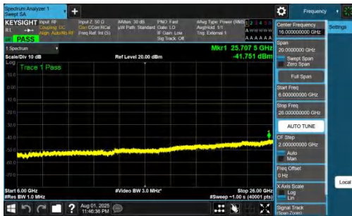
NTVN-DC_7A_n78A-PC2-30-5+90-M+M-QPSK-IDLE-DFT-BPSK-Inner_1RB_Right-6000-26000-PASS
