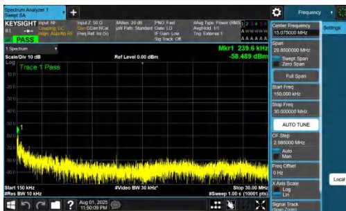
NTNV-DC_7A_n78A-PC2-30-5+90-M+M-QPSK-IDLE-DFT-QPSK-I nner_1RB_Right-0.15-30-PASS
