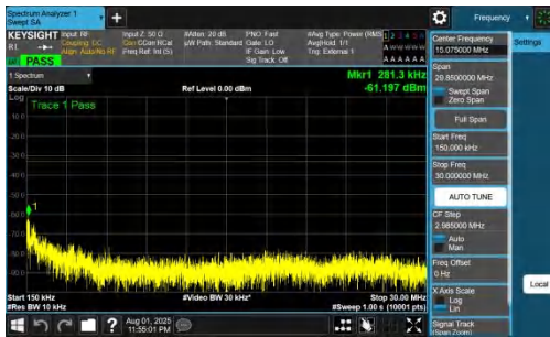
NTVN-DC_7A_n78A-PC2-30-5+90-M+H-QPSK-IDLE-DFT-BPSK-Inner_1RB_Right-0.15-30-PASS
