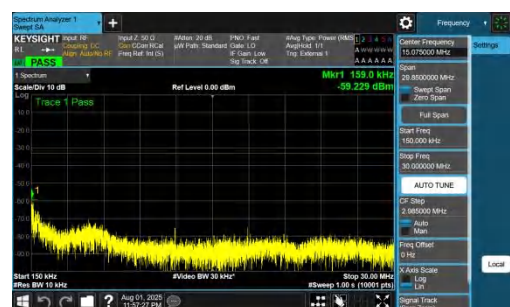
NTVN-DC_7A_n78A-PC2-30-5+90-M+H-QPSK-IDLE-DFT-QPSK-Inner_1RB_Left-0.15-30-PASS
