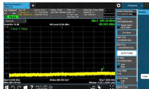
NTNV-DC_7A_n78A-PC2-30-5+90-M+M-QPSK-IDLE-DFT-BPSK-Inner_1RB_Right-30-1000-PASS
