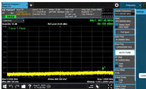
NTNV-DC_7A_n78A-PC2-30-5+80-M+M-QPSK-IDLE-DFT-BPSK-Inner_1RB_Left-30-1000-PASS
