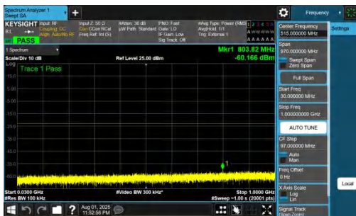
NTNV-DC_7A_n78A-PC2-30-5+90-M+H-QPSK-IDLE-DFT-BPSK-I nner_1RB_Left-30-1000-PASS
