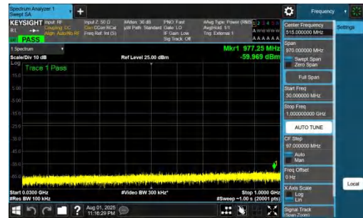
NTNV-DC_7A_n78A-PC2-30-5+80-M+M-QPSK-IDLE-DFT-BPSK-In ner_1RB_Right-30-1000-PASS
