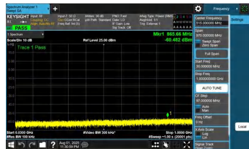
NTNV-DC_7A_n78A-PC2-30-5+80-M+H-QPSK-IDLE-DFT-QPSK-Inner_1RB_Right-30-1000-PASS
