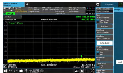
NTNV-DC_7A_n78A-PC2-30-5+100-M+L-QPSK-IDLE-DFT-QPSK-I nner_1RB_Right-30-1000-PASS
