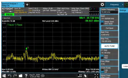
NTVN-DC_7A_n78A-PC2-30-5+90-M+M-QPSK-IDLE-DFT-QPSK-Inner_1RB_Left-0.009-0.15-PASS
