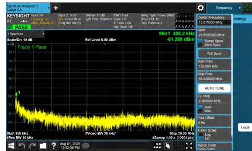
NTNV-DC_7A_n78A-PC2-30-5+90-M+H-QPSK-IDLE-DFT-BPSK-In ner_1RB_Left-0.15-30-PASS
