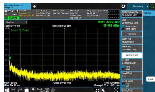
NTNV-DC_7A_n78A-PC2-30-5+80-M+M-QPSK-IDLE-DFT-QPSK-In ner_1RB_Left-0.15-30-PASS
