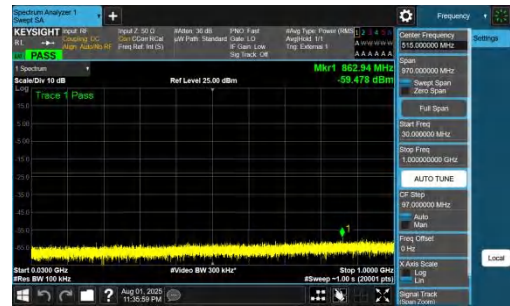
NTNV-DC_7A_n78A-PC2-30-5+90-M+L-QPSK-IDLE-DFT-BPSK-In ner_1RB_Right-30-1000-PASS
