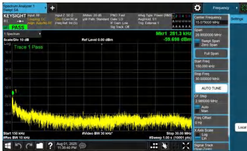
NTNV-DC_7A_n78A-PC2-30-5+90-M+L-QPSK-IDLE-DFT-BPSK-In ner_1RB_Right-0.15-30-PASS
