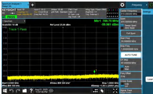
NTNV-DC_7A_n78A-PC2-30-5+90-M+H-QPSK-IDLE-DFT-QPSK-I nner_1RB_Left-30-1000-PASS
