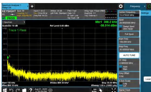
NTNV-DC_7A_n78A-PC2-30-5+80-M+M-QPSK-IDLE-DFT-QPSK-I nner_1RB_Right-0.15-30-PASS
