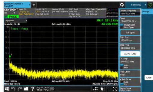
NTNV-DC_7A_n78A-PC2-30-5+90-M+L-QPSK-IDLE-DFT-BPSK-In ner_1RB_Left-0.15-30-PASS
