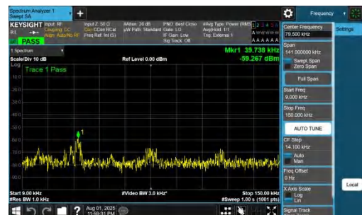
NTNV-DC_7A_n78A-PC2-30-5+90-M+H-QPSK-IDLE-DFT-QPSK-In ner_1RB_Right-0.009-0.15-PASS
