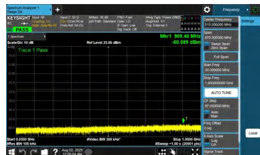
NTNV-DC_7A_n78A-PC2-30-5+100-M+L-QPSK-IDLE-DFT-BPSK-I nner_1RB_Right-30-1000-PASS
