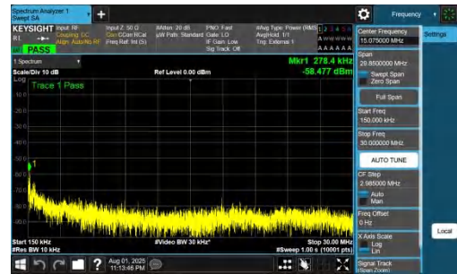
NTNV-DC_7A_n78A-PC2-30-5+80-M+M-QPSK-IDLE-DFT-BPSK-Inner_1RB_Left-0.15-30-PASS
