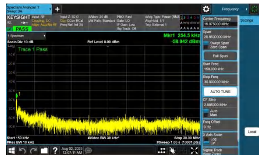
NTNV-DC_7A_n78A-PC2-30-5+100-M+L-QPSK-IDLE-DFT-QPSK-I nner_1RB_Left-0.15-30-PASS
