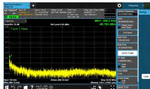
NTNV-DC_7A_n78A-PC2-30-5+90-M+M-QPSK-IDLE-DFT-BPSK-In ner_1RB_Left-0.15-30-PASS
