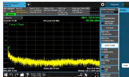
NTNV-DC_7A_n78A-PC2-30-5+80-M+H-QPSK-IDLE-DFT-QPSK-Inner_1RB_Left-0.15-30-PASS
