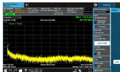
NTNV-DC_7A_n78A-PC2-30-5+90-M+L-QPSK-IDLE-DFT-QPSK-In ner_1RB_Left-0.15-30-PASS
