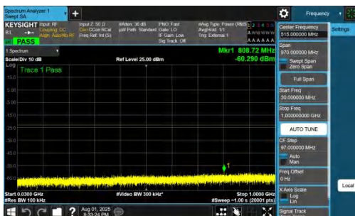
NTNV-DC_7A_n78A-PC2-30-5+25-M+H-QPSK-IDLE-DFT-QPSK-Inner_1RB_Left-30-1000-PASS
