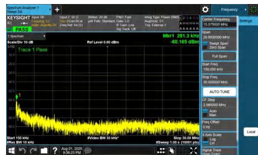
NTNV-DC_7A_n78A-PC2-30-5+50-M+L-QPSK-IDLE-DFT-BPSK-In ner 1RB Left-0.15-30-PASS
