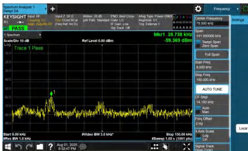
NTNV-DC_7A_n78A-PC2-30-5+25-M+H-QPSK-IDLE-DFT-QPSK-Inner_1RB_Left-0.009-0.15-PASS
