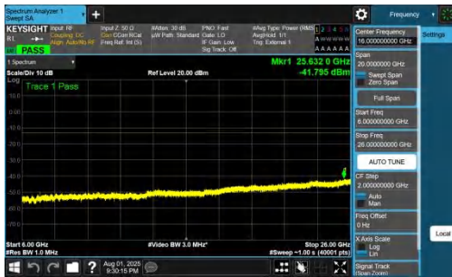
NTNV-DC_7A_n78A-PC2-30-5+40-M+H-QPSK-IDLE-DFT-BPSK-Inner_1RB_Right-6000-26000-PASS
