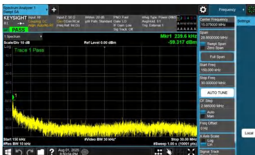
NTVN-DC_7A_n78A-PC2-30-5+30-M+M-QPSK-IDLE-DFT-BPSK-Inner_1RB_Right-0.15-30-PASS
