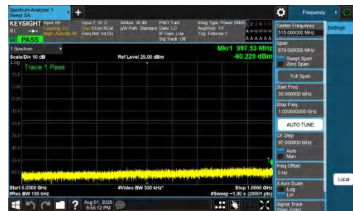
NTNV-DC_7A_n78A-PC2-30-5+30-M+M-QPSK-IDLE-DFT-QPSK-In ner_1RB_Right-30-1000-PASS
