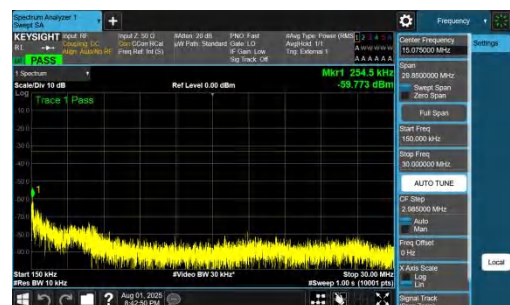
NTNV-DC_7A_n78A-PC2-30-5+30-M+L-QPSK-IDLE-DFT-QPSK-In ner_1RB_Left-0.15-30-PASS
