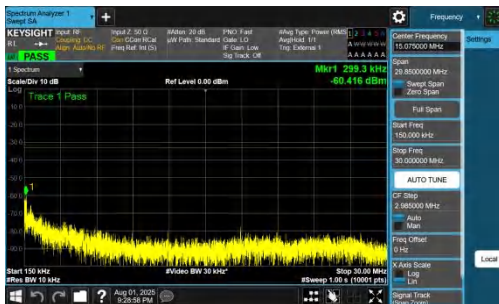
NTNV-DC_7A_n78A-PC2-30-5+40-M+H-QPSK-IDLE-DFT-BPSK-Inner_1RB_Right-0.15-30-PASS
