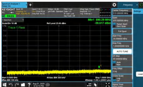
NTNV-DC_7A_n78A-PC2-30-5+40-M+L-QPSK-IDLE-DFT-QPSK-In ner_1RB_Left-30-1000-PASS
