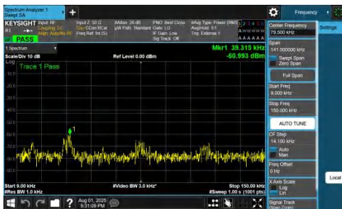
NTNV-DC_7A_n78A-PC2-30-5+40-M+H-QPSK-IDLE-DFT-QPSK-Inner_1RB_Left-0.009-0.15-PASS
