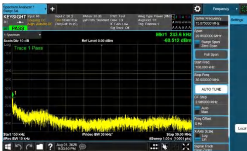
NTNV-DC_7A_n78A-PC2-30-5+40-M+H-QPSK-IDLE-DFT-QPSK-Inner_1RB_Right-0.15-30-PASS
