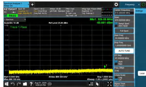
NTNV-DC_7A_n78A-PC2-30-5+30-M+H-QPSK-IDLE-DFT-BPSK-Inner_1RB_Right-30-1000-PASS
