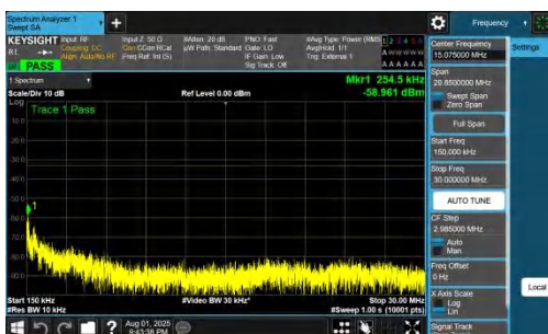
NTNV-DC_7A_n78A-PC2-30-5+50-M+L-QPSK-IDLE-DFT-QPSK-In ner_1RB_Right-0.15-30-PASS
