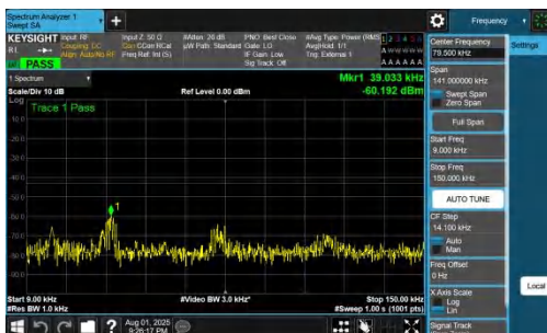
NTNV-DC_7A_n78A-PC2-30-5+40-M+H-QPSK-IDLE-DFT-BPSK-Inner_1RB_Left-0.009-0.15-PASS
