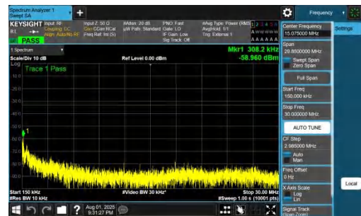
NTNV-DC_7A_n78A-PC2-30-5+40-M+H-QPSK-IDLE-DFT-QPSK-Inner_1RB_Left-0.15-30-PASS
