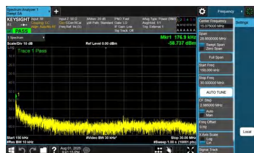
NTNV-DC_7A_n78A-PC2-30-5+50-M+L-QPSK-IDLE-DFT-QPSK-In ner_1RB_Left-0.15-30-PASS
