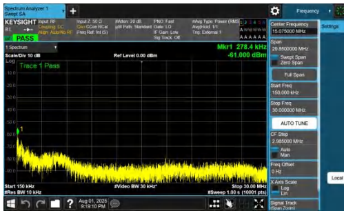
NTNV-DC_7A_n78A-PC2-30-5+40-M+M-QPSK-IDLE-DFT-BPSK-Inner_1RB_Right-0.15-30-PASS
