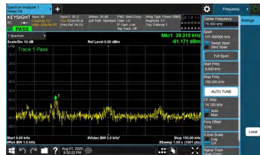
NTNV-DC_7A_n78A-PC2-30-5+25-M+H-QPSK-IDLE-DFT-BPSK-Inner_1RB_Right-0.009-0.15-PASS
