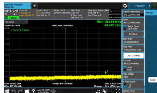
NTNV-DC_7A_n78A-PC2-30-5+25-M+H-QPSK-IDLE-DFT-BPSK-Inner_1RB_Right-30-1000-PASS
