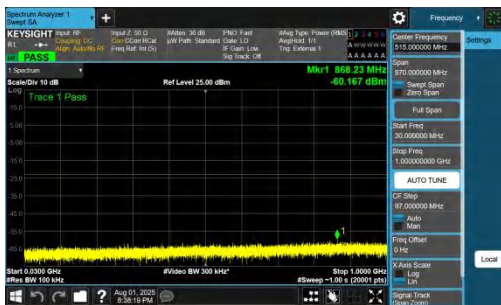
NTNV-DC_7A_n78A-PC2-30-5+30-M+L-QPSK-IDLE-DFT-BPSK-In ner_1RB_Left-30-1000-PASS
