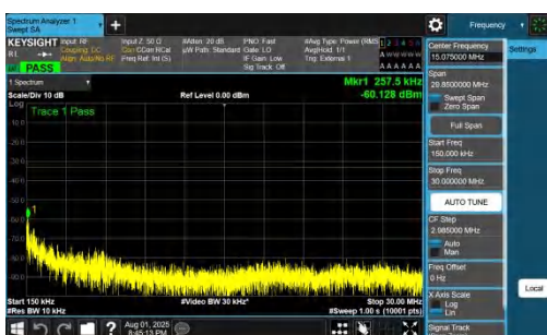
NTNV-DC_7A_n78A-PC2-30-5+30-M+L-QPSK-IDLE-DFT-QPSK-In ner_1RB_Right-0.15-30-PASS
