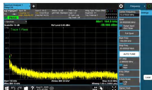
NTNV-DC_7A_n78A-PC2-30-5+40-M+M-QPSK-IDLE-DFT-QPSK-Inner_1RB_Left-0.15-30-PASS
