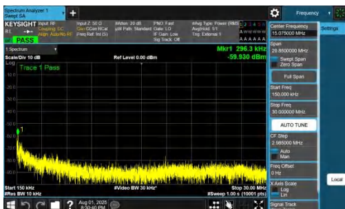
NTNV-DC_7A_n78A-PC2-30-5+25-M+H-QPSK-IDLE-DFT-BPSK-Inner_1RB_Right-0.15-30-PASS
