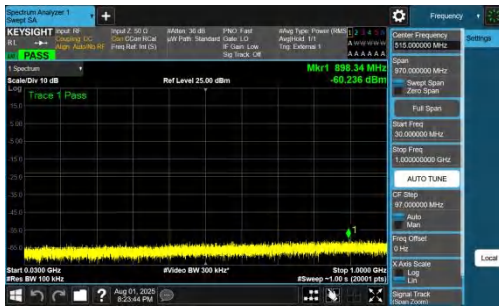
NTNV-DC_7A_n78A-PC2-30-5+25-M+M-QPSK-IDLE-DFT-QPSK-I nner_1RB_Left-30-1000-PASS
