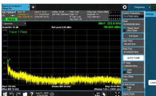
NTNV-DC_7A_n78A-PC2-30-5+40-M+M-QPSK-IDLE-DFT-QPSK-I nner_1RB_Right-0.15-30-PASS
