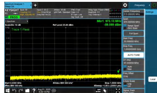
NTNV-DC_7A_n78A-PC2-30-5+40-M+H-QPSK-IDLE-DFT-BPSK-Inner_1RB_Right-30-1000-PASS
