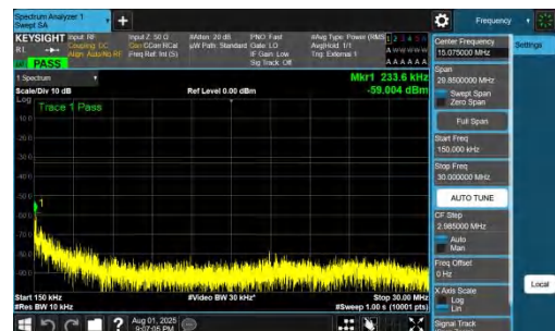
NTNV-DC_7A_n78A-PC2-30-5+40-M+L-QPSK-IDLE-DFT-BPSK-Inner_1RB_Left-0.15-30-PASS
