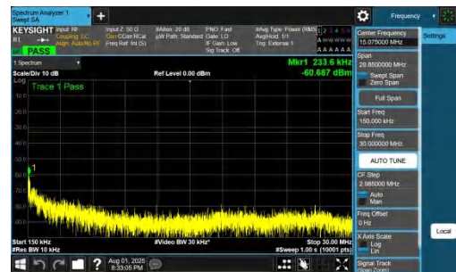
NTNV-DC_7A_n78A-PC2-30-5+25-M+H-QPSK-IDLE-DFT-QPSK-Inner_1RB_Left-0.15-30-PASS
