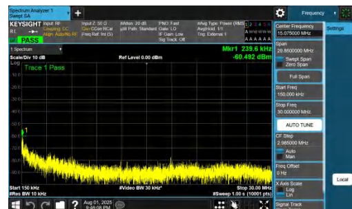
NTNV-DC_7A_n78A-PC2-30-5+50-M+M-QPSK-IDLE-DFT-BPSK-In ner_1RB_Left-0.15-30-PASS
