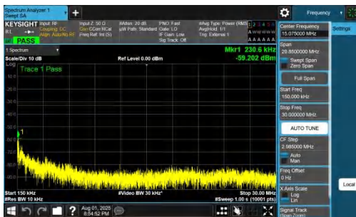
NTNV-DC_7A_n78A-PC2-30-5+30-M+M-QPSK-IDLE-DFT-QPSK-I nner_1RB_Right-0.15-30-PASS
