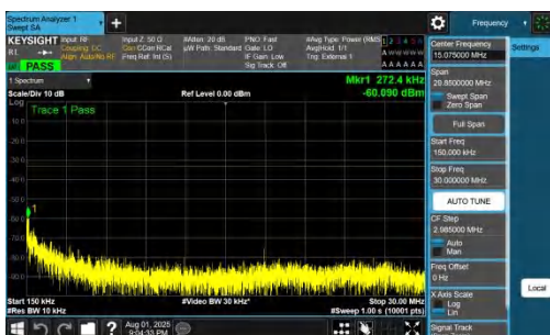
NTNV-DC_7A_n78A-PC2-30-5+30-M+H-QPSK-IDLE-DFT-QPSK-I nner_1RB_Right-0.15-30-PASS
