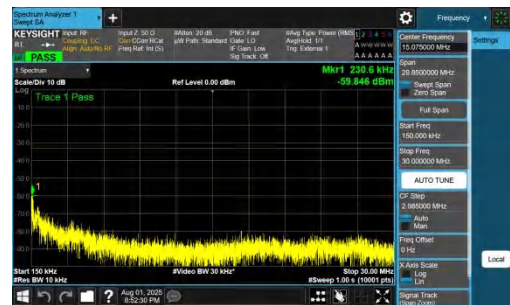
NTNV-DC_7A_n78A-PC2-30-5+30-M+M-QPSK-IDLE-DFT-QPSK-Inner_1RB_Left-0.15-30-PASS
