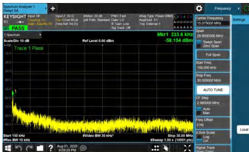
NTNV-DC_7A_n78A-PC2-30-5+40-M+L-QPSK-IDLE-DFT-BPSK-In ner_1RB_Right-0.15-30-PASS
