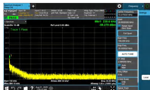
NTNV-DC_7A_n77A-PC2-30-5+100-M+M-QPSK-IDLE-DFT-QPSK-I nner_1RB_Left-0.15-30-PASS
