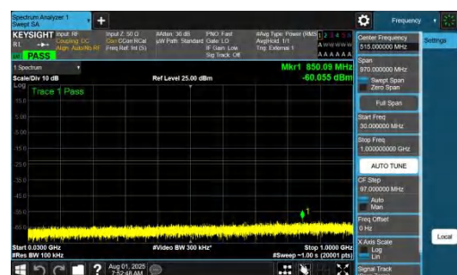
NTNV-DC_7A_n77A-PC2-30-5+100-M+M-QPSK-IDLE-DFT-QPSK-I nner_1RB_Right-30-1000-PASS
