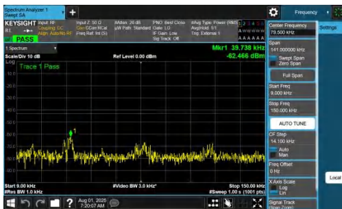
NTVN-DC_7A_n77A-PC2-30-5+90-M+M-QPSK-IDLE-DFT-QPSK-Inner_1RB_Left-0.009-0.15-PASS
