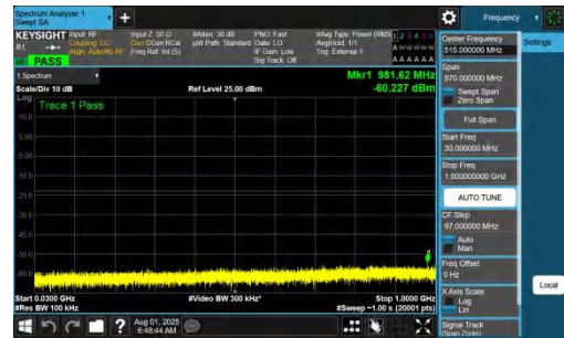
NTNV-DC_7A_n77A-PC2-30-5+80-M+M-QPSK-IDLE-DFT-BPSK-In ner_1RB_Right-30-1000-PASS
