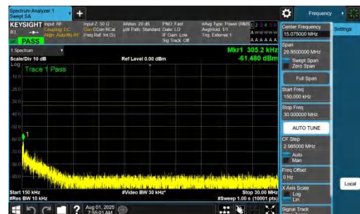
NTNV-DC_7A_n77A-PC2-30-5+100-M+H-QPSK-IDLE-DFT-BPSK-I-nner_1RB_Left-0.15-30-PASS
