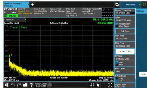
NTNV-DC_7A_n77A-PC2-30-5+100-M+M-QPSK-IDLE-DFT-BPSK-I nner_1RB_Left-0.15-30-PASS
