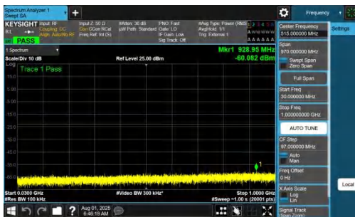
NTNV-DC_7A_n77A-PC2-30-5+80-M+M-QPSK-IDLE-DFT-BPSK-I nner_1RB_Left-30-1000-PASS
