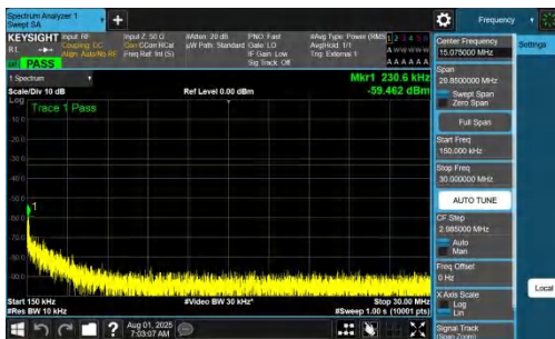
NTNV-DC_7A_n77A-PC2-30-5+80-M+H-QPSK-IDLE-DFT-QPSK-Inner_1RB_Right-0.15-30-PASS
