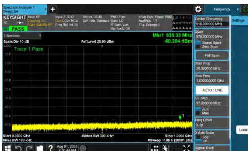
NTVN-DC_7A_n77A-PC2-30-5+90-M+M-QPSK-IDLE-DFT-QPSK-Inner_1RB_Left-30-1000-PASS
