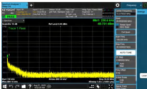
NTNV-DC_7A_n77A-PC2-30-5+100-M+H-QPSK-IDLE-DFT-QPSK-Inner_1RB_Right-0.15-30-PASS
