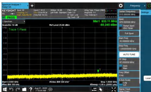
NTNV-DC_7A_n77A-PC2-30-5+90-M+L-QPSK-IDLE-DFT-QPSK-In ner_1RB_Left-30-1000-PASS
