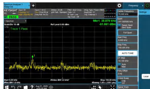
NTNV-DC_7A_n77A-PC2-30-5+80-M+M-QPSK-IDLE-DFT-QPSK-In ner_1RB_Right-0.009-0.15-PASS
