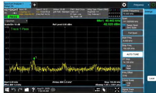
NTNV-DC_7A_n77A-PC2-30-5+80-M+H-QPSK-IDLE-DFT-QPSK-Inner_1RB_Right-0.009-0.15-PASS
