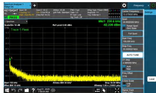
NTNV-DC_7A_n77A-PC2-30-5+100-M+H-QPSK-IDLE-DFT-QPSK-I nner_1RB_Left-0.15-30-PASS
