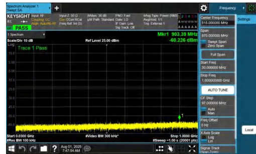
NTNV-DC_7A_n77A-PC2-30-5+100-M+M-QPSK-IDLE-DFT-BPSK-I nner_1RB_Right-30-1000-PASS
