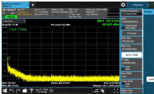
NTNV-DC_7A_n77A-PC2-30-5+100-M+M-QPSK-IDLE-DFT-BPSK- Inner_1RB_Right-0.15-30-PASS
