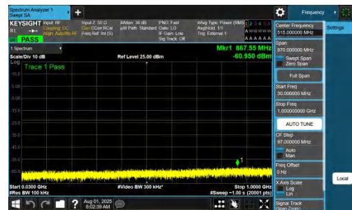
NTNV-DC_7A_n77A-PC2-30-5+100-M+H-QPSK-IDLE-DFT-QPSK-I-nner_1RB_Right-30-1000-PASS
