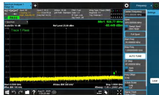
NTNV-DC_7A_n77A-PC2-30-5+80-M+H-QPSK-IDLE-DFT-QPSK-Inner_1RB_Right-30-1000-PASS
