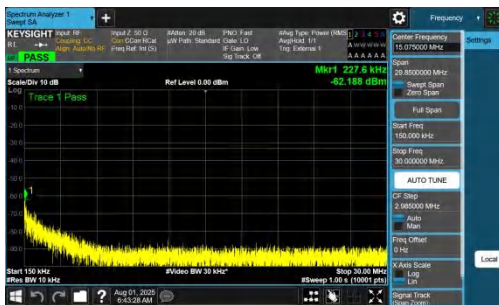
NTNV-DC_7A_n77A-PC2-30-5+80-M+L-QPSK-IDLE-DFT-QPSK-In ner_1RB_Right-0.15-30-PASS
