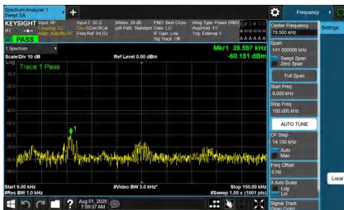
NTNV-DC_7A_n77A-PC2-30-5+100-M+H-QPSK-IDLE-DFT-QPSK- Inner_1RB_Left-0.009-0.15-PASS
