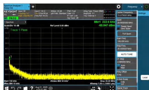
NTNV-DC_7A_n77A-PC2-30-5+30-M+H-QPSK-IDLE-DFT-QPSK-In ner_1RB_Left-0.15-30-PASS
