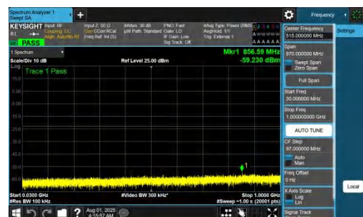
NTNV-DC_7A_n77A-PC2-30-5+30-M+L-QPSK-IDLE-DFT-QPSK-In ner_1RB_Right-30-1000-PASS
