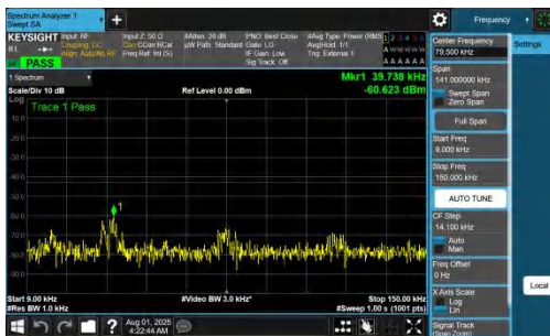
NTNV-DC_7A_n77A-PC2-30-5+30-M+M-QPSK-IDLE-DFT-QPSK-Inner_1RB_Left-0.009-0.15-PASS
