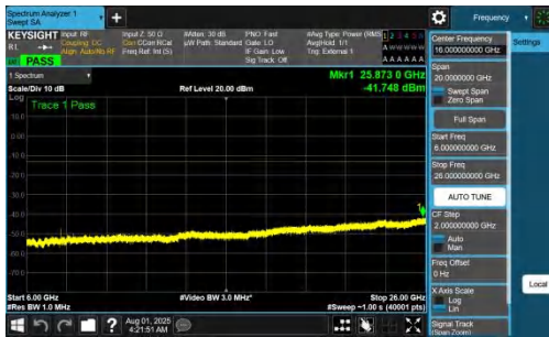
NTNV-DC_7A_n77A-PC2-30-5+30-M+M-QPSK-IDLE-DFT-BPSK-Inner_1RB_Right-6000-26000-PASS
