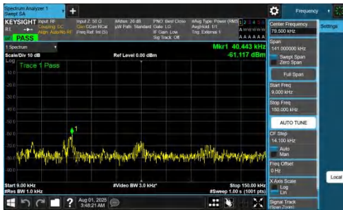
NTVN-DC_7A_n77A-PC2-30-5+25-M+M-QPSK-IDLE-DFT-BPSK-Inner_1RB_Left-0.009-0.15-PASS
