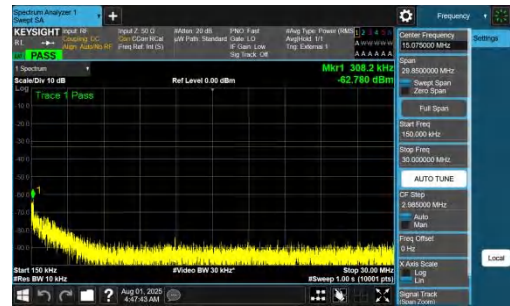
NTNV-DC_7A_n77A-PC2-30-5+40-M+M-QPSK-IDLE-DFT-BPSK-In ner_1RB_Left-0.15-30-PASS
