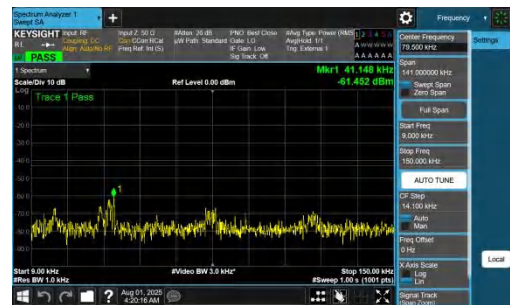
NTVN-DC_7A_n77A-PC2-30-5+30-M+M-QPSK-IDLE-DFT-BPSK-Inner_1RB_Right-0.009-0.15-PASS
