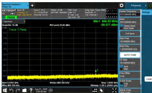
NTVN-DC_7A_n77A-PC2-30-5+25-M+M-QPSK-IDLE-DFT-BPSK-Inner_1RB_Left-30-1000-PASS
