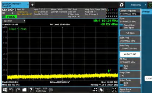
NTNV-DC_7A_n77A-PC2-30-5+25-M+M-QPSK-IDLE-DFT-QPSK-Inner_1RB_Left-30-1000-PASS
