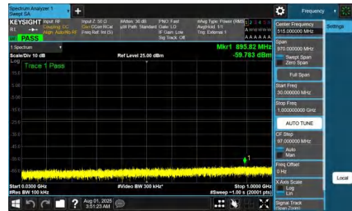
NTNV-DC_7A_n77A-PC2-30-5+25-M+M-QPSK-IDLE-DFT-BPSK-In ner_1RB_Right-30-1000-PASS
