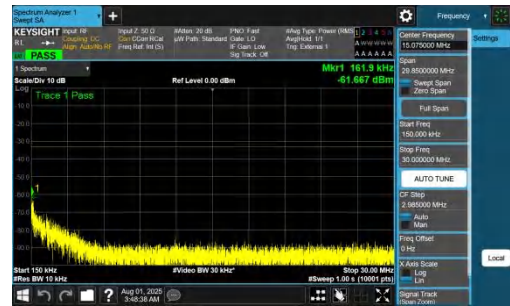
NTVN-DC_7A_n77A-PC2-30-5+25-M+M-QPSK-IDLE-DFT-BPSK-Inner_1RB_Left-0.15-30-PASS
