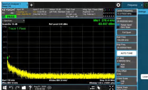
NTNV-DC_7A_n77A-PC2-30-5+40-M+H-QPSK-IDLE-DFT-BPSK-Inner_1RB_Right-0.15-30-PASS
