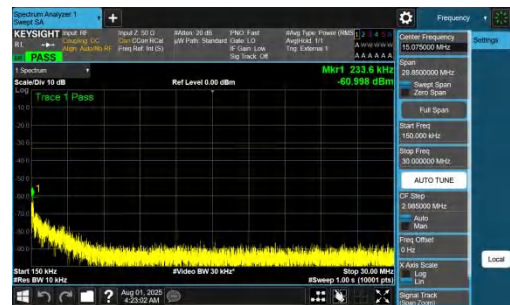
NTNV-DC_7A_n77A-PC2-30-5+30-M+M-QPSK-IDLE-DFT-QPSK-Inner_1RB_Left-0.15-30-PASS
