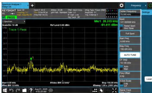
NTNV-DC_7A_n77A-PC2-30-5+40-M+L-QPSK-IDLE-DFT-QPSK-In ner_1RB_Left-0.009-0.15-PASS
