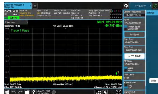
NTVN-DC_7A_n77A-PC2-30-5+30-M+M-QPSK-IDLE-DFT-BPSK-Inner_1RB_Right-30-1000-PASS
