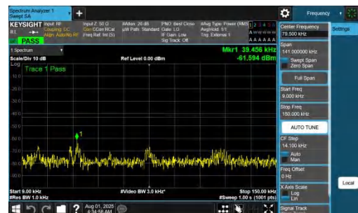
NTNV-DC_7A_n77A-PC2-30-5+30-M+H-QPSK-IDLE-DFT-QPSK-In ner_1RB_Right-0.009-0.15-PASS
