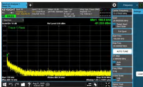
NTNV-DC_7A_n77A-PC2-30-5+25-M+H-QPSK-IDLE-DFT-QPSK-Inner_1RB_Right-0.15-30-PASS
