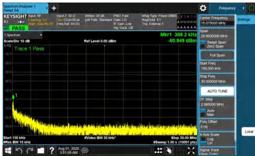
NTNV-DC_7A_n77A-PC2-30-5+25-M+M-QPSK-IDLE-DFT-BPSK-In nner_1RB_Right-0.15-30-PASS
