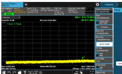
NTNV-DC_7A_n77A-PC2-30-5+40-M+H-QPSK-IDLE-DFT-QPSK-Inner_1RB_Left-30-1000-PASS
