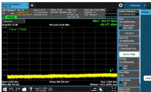
NTNV-DC_7A_n77A-PC2-30-5+50-M+L-QPSK-IDLE-DFT-BPSK-In ner_1RB_Left-30-1000-PASS
