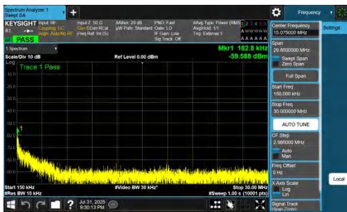
NTNV-DC_7A_n77A-PC2-30-5+50-M+M-QPSK-IDLE-DFT-QPSK-I nner_1RB_Right-0.15-30-PASS
