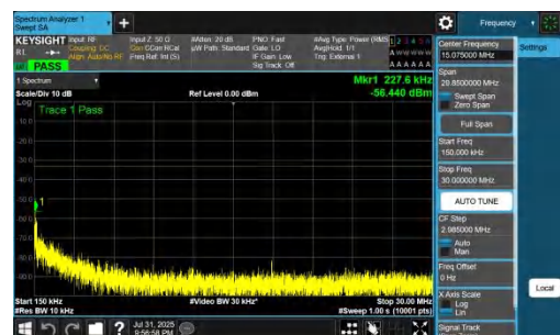
NTNV-DC_7A_n77A-PC2-30-5+60-M+M-QPSK-IDLE-DFT-QPSK-In ner_1RB_Left-0.15-30-PASS
