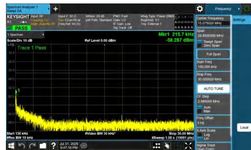
NTNV-DC_7A_n77A-PC2-30-5+60-M+L-QPSK-IDLE-DFT-QPSK-In ner_1RB_Left-0.15-30-PASS
