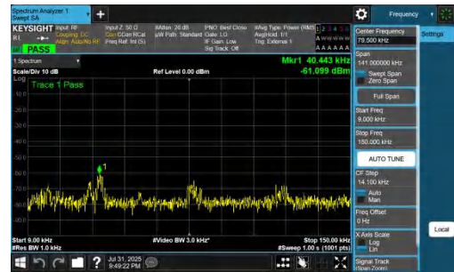
NTNV-DC_7A_n77A-PC2-30-5+60-M+L-QPSK-IDLE-DFT-QPSK-In_ner_1RB_Right-0.009-0.15-PASS
