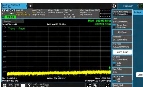
NTNV-DC_7A_n77A-PC2-30-5+70-M+M-QPSK-IDLE-DFT-BPSK-In ner_1RB_Left-30-1000-PASS
