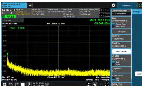
NTVN-DC_7A_n77A-PC2-30-5+70-M+M-QPSK-IDLE-DFT-BPSK-Inner_1RB_Right-0.15-30-PASS
