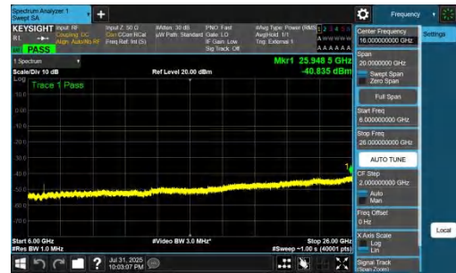
NTNV-DC_7A_n77A-PC2-30-5+60-M+H-QPSK-IDLE-DFT-BPSK-In ner_1RB_Left-6000-26000-PASS
