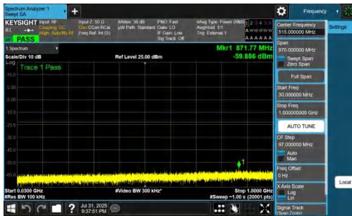
NTNV-DC_7A_n77A-PC2-30-5+50-M+H-QPSK-IDLE-DFT-QPSK-I nner_1RB_Left-30-1000-PASS
