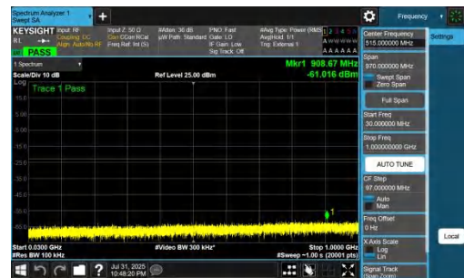
NTNV-DC_7A_n77A-PC2-30-5+80-M+L-QPSK-IDLE-DFT-QPSK-In ner_1RB_Right-30-1000-PASS
