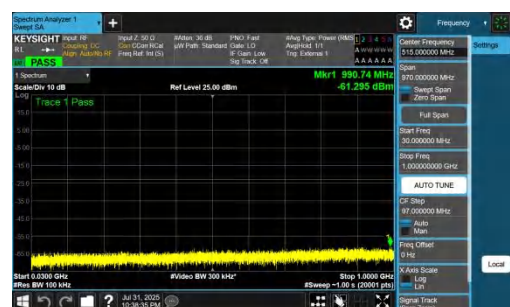
NTNV-DC_7A_n77A-PC2-30-5+70-M+H-QPSK-IDLE-DFT-QPSK-Inner_1RB_Right-30-1000-PASS
