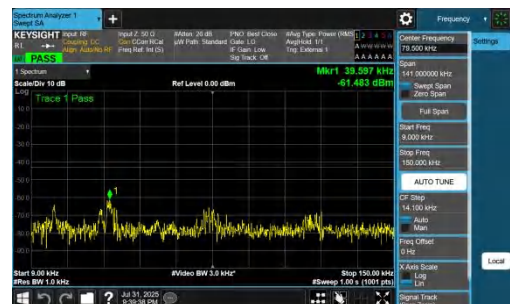
NTNV-DC_7A_n77A-PC2-30-5+50-M+H-QPSK-IDLE-DFT-QPSK-In ner_1RB_Right-0.009-0.15-PASS
