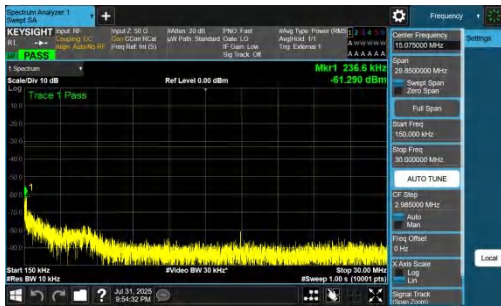
NTNV-DC_7A_n77A-PC2-30-5+60-M+M-QPSK-IDLE-DFT-BPSK-I nner_1RB_Right-0.15-30-PASS
