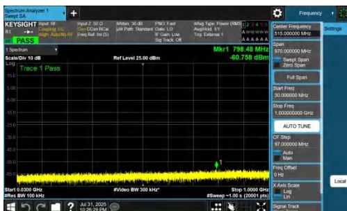
NTNV-DC_7A_n77A-PC2-30-5+70-M+M-QPSK-IDLE-DFT-QPSK-Inner_1RB_Left-30-1000-PASS
