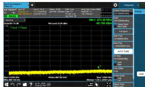
NTNV-DC_7A_n77A-PC2-30-5+70-M+M-QPSK-IDLE-DFT-QPSK-Inner_1RB_Right-30-1000-PASS
