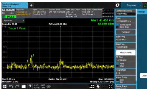
NTNV-DC_7A_n77A-PC2-30-5+80-M+L-QPSK-IDLE-DFT-QPSK-In ner_1RB_Left-0.009-0.15-PASS
