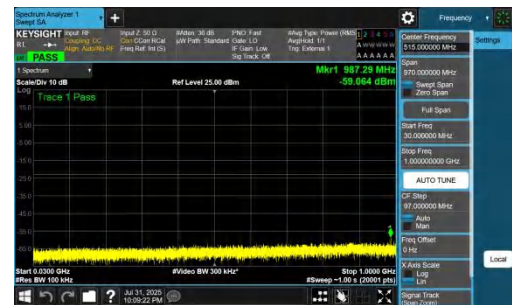
NTNV-DC_7A_n77A-PC2-30-5+60-M+H-QPSK-IDLE-DFT-QPSK-Inner_1RB_Right-30-1000-PASS
