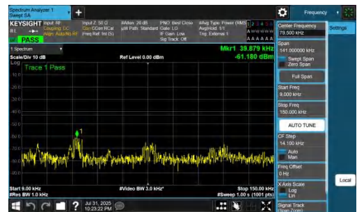
NTVN-DC_7A_n77A-PC2-30-5+70-M+M-QPSK-IDLE-DFT-BPSK-Inner_1RB_Right-0.009-0.15-PASS
