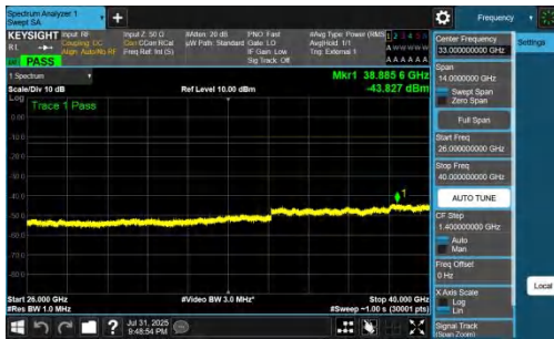
NTNV-DC_7A_n77A-PC2-30-5+60-M+L-QPSK-IDLE-DFT-QPSK-In_ner_1RB_Left-26000-40000-PASS
