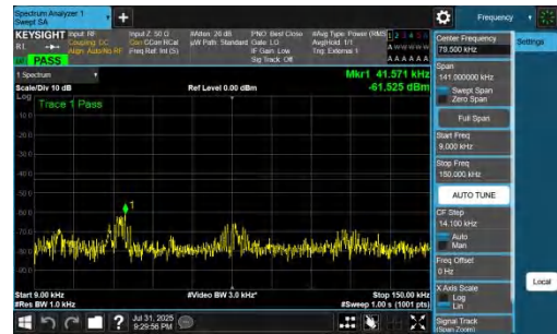
NTNV-DC_7A_n77A-PC2-30-5+50-M+M-QPSK-IDLE-DFT-QPSK-In ner_1RB_Right-0.009-0.15-PASS
