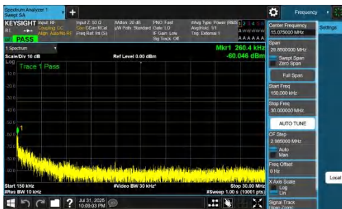
NTNV-DC_7A_n77A-PC2-30-5+60-M+H-QPSK-IDLE-DFT-QPSK-Inner_1RB_Right-0.15-30-PASS
