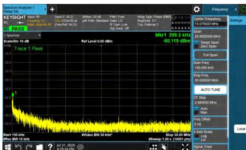
NTNV-DC_7A_n77A-PC2-30-5+50-M+M-QPSK-IDLE-DFT-BPSK-Inner_1RB_Right-0.15-30-PASS
