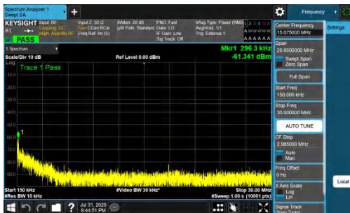
NTNV-DC_7A_n77A-PC2-30-5+60-M+L-QPSK-IDLE-DFT-BPSK-In ner_1RB_Right-0.15-30-PASS
