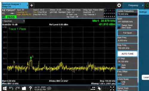
NTNV-DC_7A_n77A-PC2-30-5+70-M+M-QPSK-IDLE-DFT-QPSK-Inner_1RB_Left-0.009-0.15-PASS
