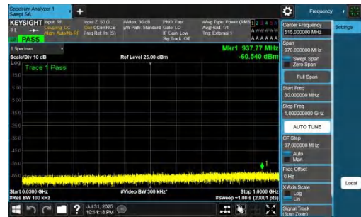
NTNV-DC_7A_n77A-PC2-30-5+70-M+L-QPSK-IDLE-DFT-BPSK-In ner_1RB_Right-30-1000-PASS
