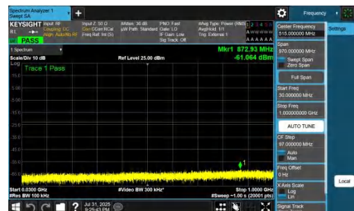
NTNV-DC_7A_n77A-PC2-30-5+50-M+M-QPSK-IDLE-DFT-BPSK-Inner_1RB_Right-30-1000-PASS
