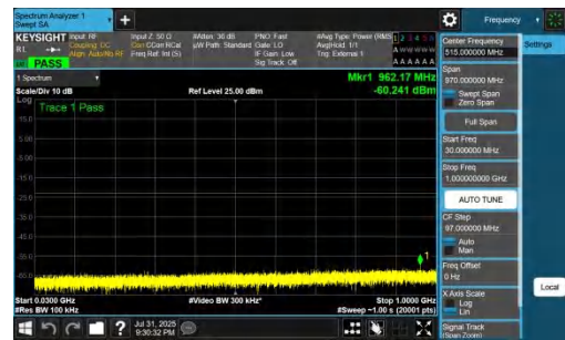
NTNV-DC_7A_n77A-PC2-30-5+50-M+M-QPSK-IDLE-DFT-QPSK-In ner_1RB_Right-30-1000-PASS
