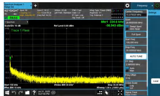
NTNV-DC_7A_n77A-PC2-30-5+50-M+M-QPSK-IDLE-DFT-QPSK-Inner_1RB_Left-0.15-30-PASS
