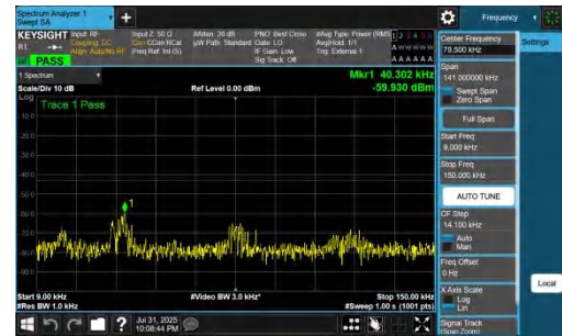
NTNV-DC_7A_n77A-PC2-30-5+60-M+H-QPSK-IDLE-DFT-QPSK-Inner_1RB_Right-0.009-0.15-PASS
