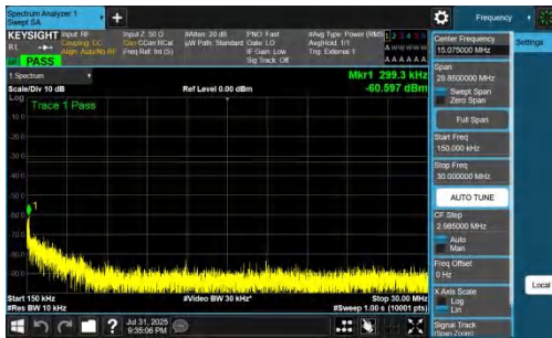
NTNV-DC_7A_n77A-PC2-30-5+50-M+H-QPSK-IDLE-DFT-BPSK-In nner_1RB_Right-0.15-30-PASS
