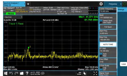
NTNV-DC_7A_n77A-PC2-30-5+80-M+L-QPSK-IDLE-DFT-QPSK-In ner_1RB_Right-0.009-0.15-PASS
