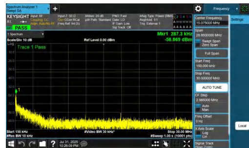
NTNV-DC_7A_n77A-PC2-30-5+70-M+M-QPSK-IDLE-DFT-QPSK-Inner_1RB_Left-0.15-30-PASS
