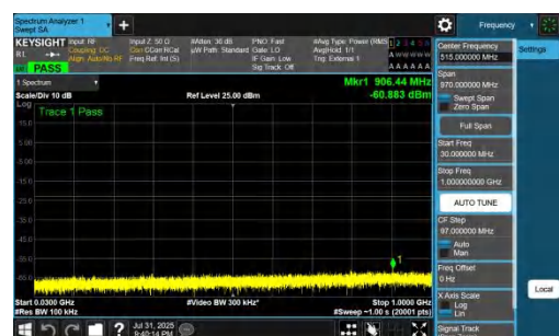
NTNV-DC_7A_n77A-PC2-30-5+50-M+H-QPSK-IDLE-DFT-QPSK-In ner_1RB_Right-30-1000-PASS
