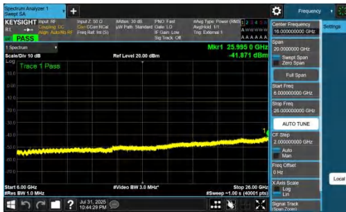
NTNV-DC_7A_n77A-PC2-30-5+80-M+L-QPSK-IDLE-DFT-BPSK-In ner_1RB_Right-6000-26000-PASS
