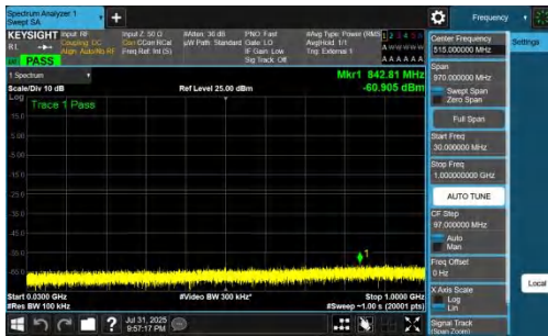
NTNV-DC_7A_n77A-PC2-30-5+60-M+M-QPSK-IDLE-DFT-QPSK-I nner_1RB_Left-30-1000-PASS
