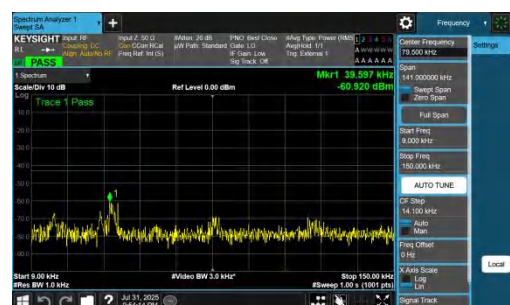
NTNV-DC_7A_n77A-PC2-30-5+60-M+M-QPSK-IDLE-DFT-BPSK-In ner_1RB_Right-0.009-0.15-PASS
