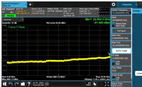
NTNV-DC_7A_n77A-PC2-30-5+70-M+M-QPSK-IDLE-DFT-BPSK-Inner_1RB_Right-6000-26000-PASS
