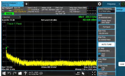
NTNV-DC_7A_n77A-PC2-30-5+70-M+L-QPSK-IDLE-DFT-BPSK-In ner_1RB_Right-0.15-30-PASS
