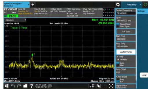
NTNV-DC_7A_n77A-PC2-30-5+70-M+M-QPSK-IDLE-DFT-QPSK-Inner_1RB_Right-0.009-0.15-PASS
