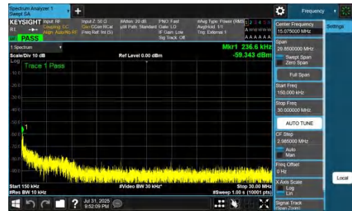
NTNV-DC_7A_n77A-PC2-30-5+60-M+M-QPSK-IDLE-DFT-BPSK-In ner_1RB_Left-0.15-30-PASS
