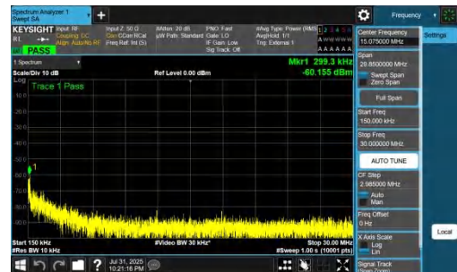
NTNV-DC_7A_n77A-PC2-30-5+70-M+M-QPSK-IDLE-DFT-BPSK-In ner_1RB_Left-0.15-30-PASS
