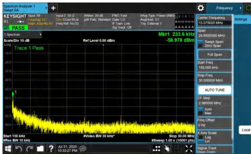
NTNV-DC_7A_n77A-PC2-30-5+70-M+H-QPSK-IDLE-DFT-BPSK-Inner_1RB_Right-0.15-30-PASS
