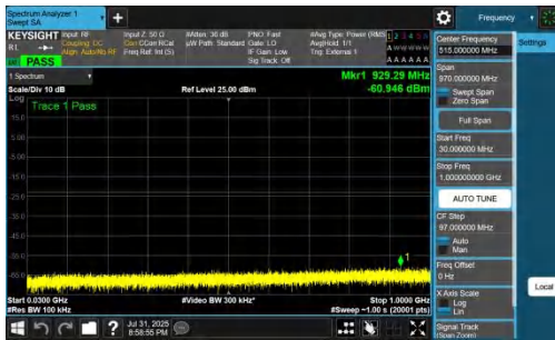
NTNV-DC_7A_n77A-PC2-30-5+40-M+M-QPSK-IDLE-DFT-QPSK-I nner_1RB_Left-30-1000-PASS
