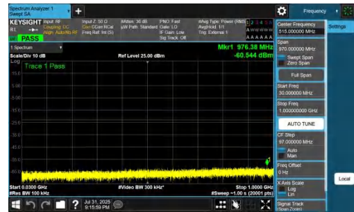
NTNV-DC_7A_n77A-PC2-30-5+50-M+L-QPSK-IDLE-DFT-BPSK-In ner_1RB_Right-30-1000-PASS
