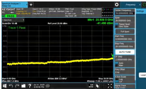
NTNV-DC_7A_n77A-PC2-30-5+25-M+H-QPSK-IDLE-DFT-BPSK-Inner_1RB_Right-6000-26000-PASS
