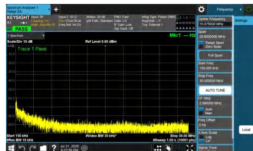
NTNV-DC_7A_n77A-PC2-30-5+50-M+M-QPSK-IDLE-DFT-BPSK-In_ner_1RB_Left-0.15-30-PASS
