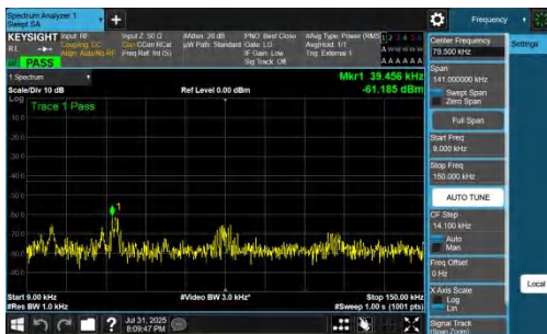
NTNV-DC_7A_n77A-PC2-30-5+25-M+H-QPSK-IDLE-DFT-QPSK-Inner_1RB_Left-0.009-0.15-PASS
