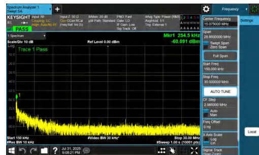
NTNV-DC_7A_n77A-PC2-30-5+40-M+H-QPSK-IDLE-DFT-QPSK-Inner_1RB_Left-0.15-30-PASS
