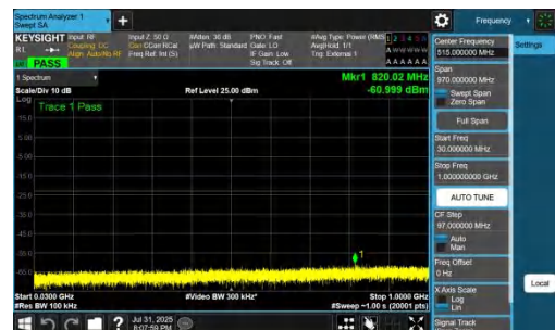
NTNV-DC_7A_n77A-PC2-30-5+25-M+H-QPSK-IDLE-DFT-BPSK-In ner_1RB_Right-30-1000-PASS
