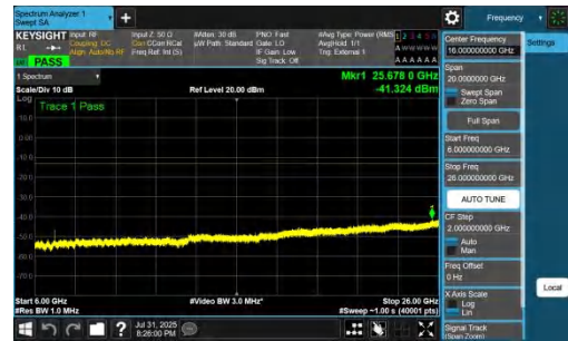
NTNV-DC_7A_n77A-PC2-30-5+30-M+M-QPSK-IDLE-DFT-BPSK-Inner_1RB_Left-6000-26000-PASS
