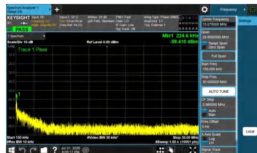
NTNV-DC_7A_n77A-PC2-30-5+25-M+H-QPSK-IDLE-DFT-BPSK-Inner_1RB_Left-0.15-30-PASS
