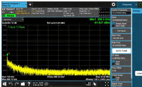
NTNV-DC_7A_n77A-PC2-30-5+30-M+H-QPSK-IDLE-DFT-BPSK-Inner_1RB_Right-0.15-30-PASS
