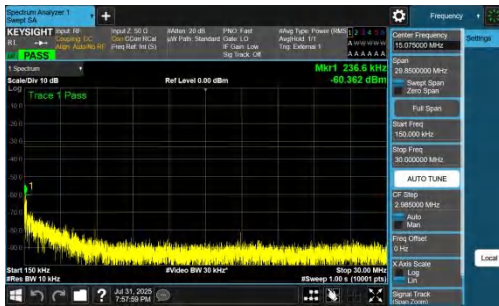
NTVN-DC_7A_n77A-PC2-30-5+25-M+M-QPSK-IDLE-DFT-BPSK-Inner_1RB_Right-0.15-30-PASS
