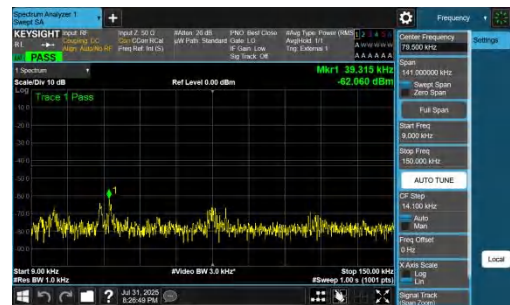
NTNV-DC_7A_n77A-PC2-30-5+30-M+M-QPSK-IDLE-DFT-BPSK-Inner_1RB_Right-0.009-0.15-PASS
