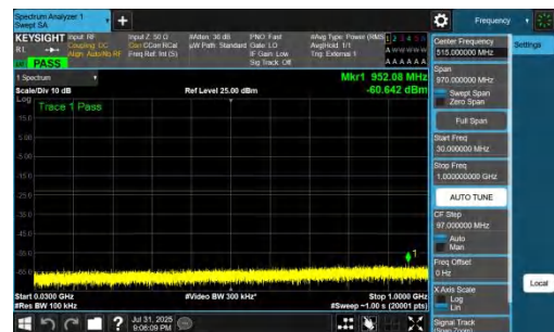
NTNV-DC_7A_n77A-PC2-30-5+40-M+H-QPSK-IDLE-DFT-BPSK-In ner_1RB_Right-30-1000-PASS
