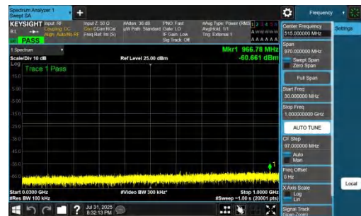
NTNV-DC_7A_n77A-PC2-30-5+30-M+M-QPSK-IDLE-DFT-QPSK-Inner_1RB_Right-30-1000-PASS
