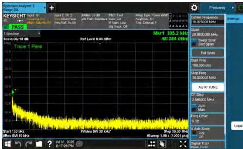
NTNV-DC_7A_n77A-PC2-30-5+30-M+L-QPSK-IDLE-DFT-BPSK-In ner_1RB_Right-0.15-30-PASS
