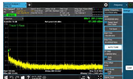
NTVN-DC_7A_n77A-PC2-30-5+40-M+L-QPSK-IDLE-DFT-BPSK-Inner_1RB_Left-0.15-30-PASS
