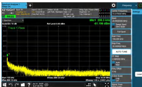
NTNV-DC_7A_n77A-PC2-30-5+30-M+M-QPSK-IDLE-DFT-BPSK-Inner_1RB_Right-0.15-30-PASS
