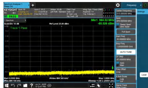
NTNV-DC_7A_n77A-PC2-30-5+25-M+H-QPSK-IDLE-DFT-QPSK-Inner_1RB_Right-30-1000-PASS
