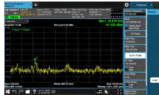
NTNV-DC_7A_n77A-PC2-30-5+40-M+H-QPSK-IDLE-DFT-QPSK-Inner_1RB_Right-0.009-0.15-PASS
