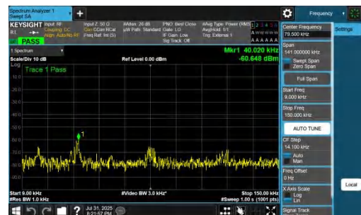
NTNV-DC_7A_n77A-PC2-30-5+30-M+L-QPSK-IDLE-DFT-QPSK-In ner_1RB_Right-0.009-0.15-PASS
