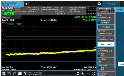
NTNV-DC_7A_n77A-PC2-30-5+40-M+H-QPSK-IDLE-DFT-BPSK-Inner_1RB_Right-6000-26000-PASS
