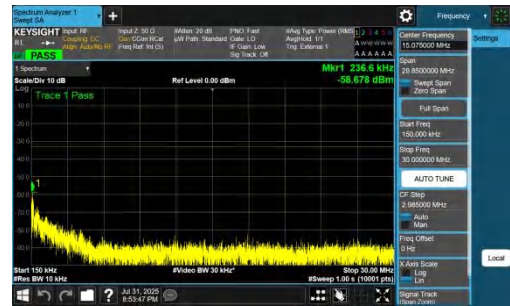
NTVN-DC_7A_n77A-PC2-30-5+40-M+M-QPSK-IDLE-DFT-BPSK-Inner_1RB_Left-0.15-30-PASS
