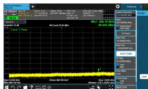
NTNV-DC_7A_n77A-PC2-30-5+25-M+M-QPSK-IDLE-DFT-QPSK-In ner_1RB_Right-30-1000-PASS
