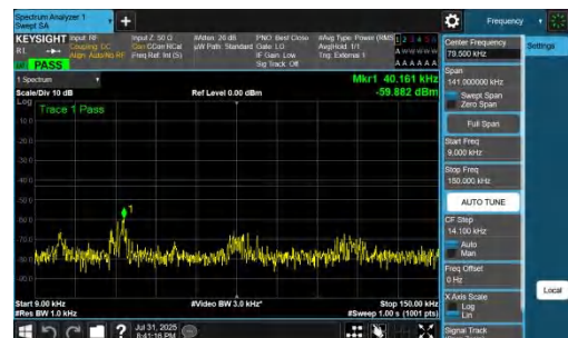
NTVN-DC_7A_n77A-PC2-30-5+30-M+H-QPSK-IDLE-DFT-QPSK-Inner_1RB_Right-0.009-0.15-PASS
