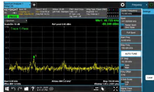
NTNV-DC_7A_n77A-PC2-30-5+30-M+M-QPSK-IDLE-DFT-QPSK-Inner_1RB_Right-0.009-0.15-PASS
