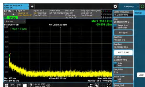
NTVN-DC_7A_n77A-PC2-30-5+25-M+M-QPSK-IDLE-DFT-QPSK-Inner_1RB_Left-0.15-30-PASS
