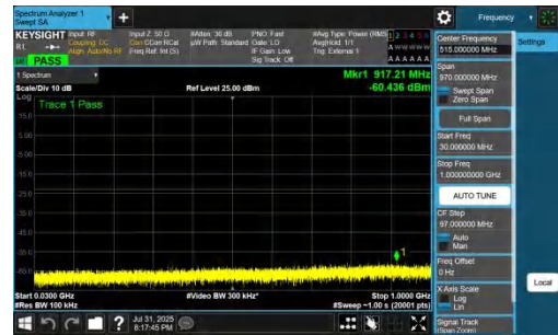
NTNV-DC_7A_n77A-PC2-30-5+30-M+L-QPSK-IDLE-DFT-BPSK-In ner_1RB_Right-30-1000-PASS
