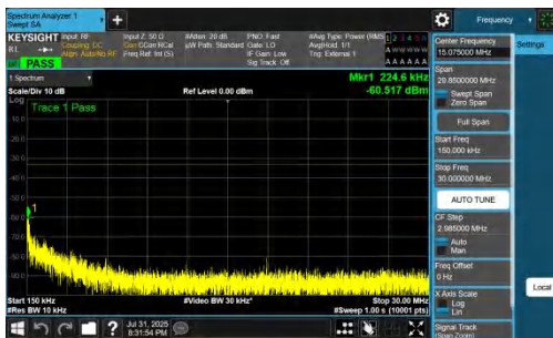
NTNV-DC_7A_n77A-PC2-30-5+30-M+M-QPSK-IDLE-DFT-QPSK-Inner_1RB_Right-0.15-30-PASS
