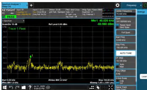
NTNV-DC_7A_n77A-PC2-30-5+40-M+H-QPSK-IDLE-DFT-QPSK-Inner_1RB_Left-0.009-0.15-PASS
