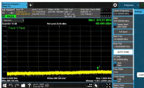
NTNV-DC_7A_n77A-PC2-30-5+30-M+H-QPSK-IDLE-DFT-BPSK-Inner_1RB_Left-30-1000-PASS
