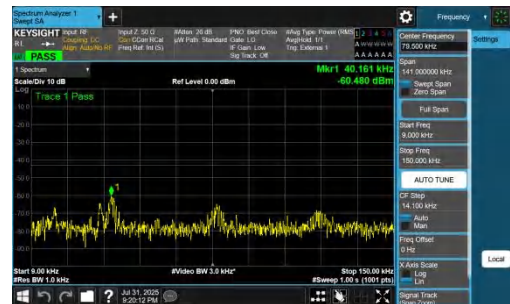
NTNV-DC_7A_n77A-PC2-30-5+50-M+L-QPSK-IDLE-DFT-QPSK-In ner_1RB_Right-0.009-0.15-PASS
