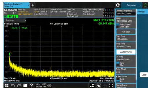
NTNV-DC_7A_n77A-PC2-30-5+40-M+L-QPSK-IDLE-DFT-QPSK-In ner_1RB_Left-0.15-30-PASS
