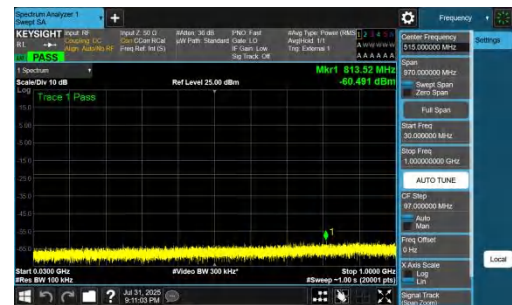
NTNV-DC_7A_n77A-PC2-30-5+40-M+H-QPSK-IDLE-DFT-QPSK-Inner_1RB_Right-30-1000-PASS
