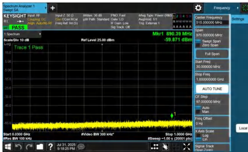
NTNV-DC_7A_n77A-PC2-30-5+50-M+L-QPSK-IDLE-DFT-QPSK-In ner_1RB_Left-30-1000-PASS
