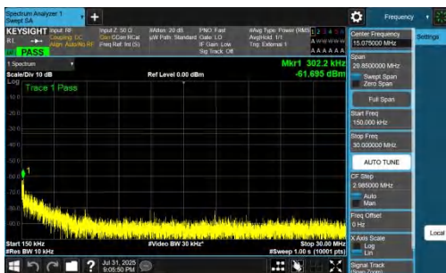
NTNV-DC_7A_n77A-PC2-30-5+40-M+H-QPSK-IDLE-DFT-BPSK-I nner_1RB_Right-0.15-30-PASS
