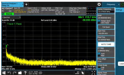
NTNV-DC_7A_n77A-PC2-30-5+40-M+L-QPSK-IDLE-DFT-QPSK-In ner_1RB_Right-0.15-30-PASS
