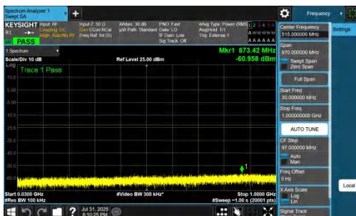
NTNV-DC_7A_n77A-PC2-30-5+25-M+H-QPSK-IDLE-DFT-QPSK-Inner_1RB_Left-30-1000-PASS
