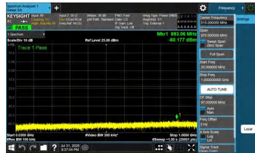
NTNV-DC_7A_n77A-PC2-30-5+30-M+H-QPSK-IDLE-DFT-BPSK-Inner_1RB_Right-30-1000-PASS
