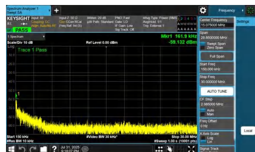
NTNV-DC_7A_n77A-PC2-30-5+50-M+L-QPSK-IDLE-DFT-QPSK-In ner_1RB_Left-0.15-30-PASS
