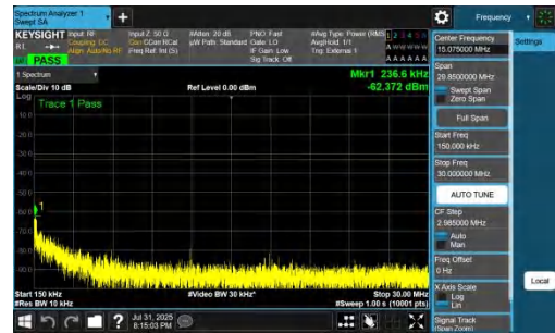
NTNV-DC_7A_n77A-PC2-30-5+30-M+L-QPSK-IDLE-DFT-BPSK-In ner_1RB_Left-0.15-30-PASS
