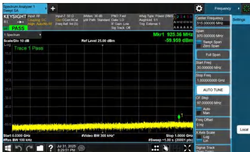
NTNV-DC_7A_n77A-PC2-30-5+30-M+M-QPSK-IDLE-DFT-QPSK-Inner_1RB_Left-30-1000-PASS
