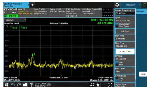
NTNV-DC_7A_n77A-PC2-30-5+40-M+M-QPSK-IDLE-DFT-QPSK-In ner_1RB_Right-0.009-0.15-PASS
