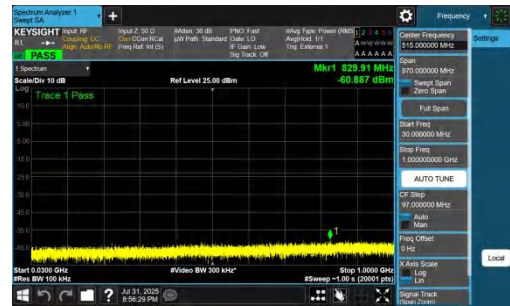
NTNV-DC_7A_n77A-PC2-30-5+40-M+M-QPSK-IDLE-DFT-BPSK-In ner_1RB_Right-30-1000-PASS
