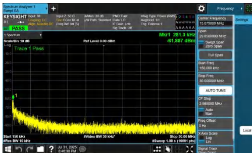
NTNV-DC_7A_n77A-PC2-30-5+40-M+L-QPSK-IDLE-DFT-BPSK-In ner_1RB_Right-0.15-30-PASS
