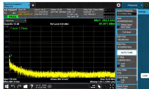
NTNV-DC_7A_n77A-PC2-30-5+25-M+H-QPSK-IDLE-DFT-QPSK-Inner_1RB_Left-0.15-30-PASS
