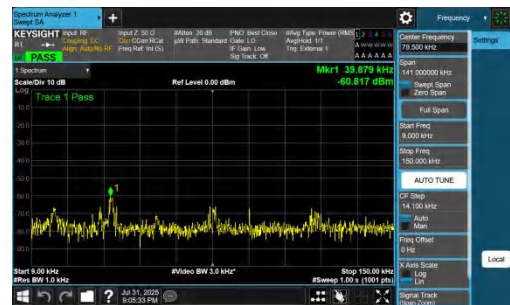
NTNV-DC_7A_n77A-PC2-30-5+40-M+H-QPSK-IDLE-DFT-BPSK-In ner_1RB_Right-0.009-0.15-PASS
