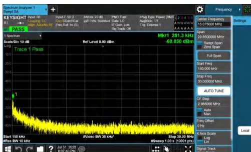
NTNV-DC_7A_n77A-PC2-30-5+25-M+H-QPSK-IDLE-DFT-BPSK-I nner_1RB_Right-0.15-30-PASS
