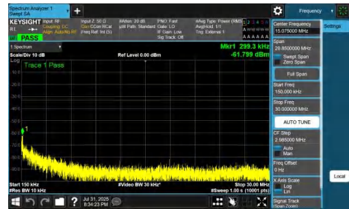
NTNV-DC_7A_n77A-PC2-30-5+30-M+H-QPSK-IDLE-DFT-BPSK-Inner_1RB_Left-0.15-30-PASS
