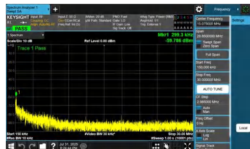
NTNV-DC_7A_n77A-PC2-30-5+30-M+M-QPSK-IDLE-DFT-BPSK-In ner_1RB_Left-0.15-30-PASS
