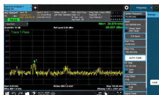
NTVN-DC_7A_n77A-PC2-30-5+40-M+M-QPSK-IDLE-DFT-BPSK-Inner_1RB_Right-0.009-0.15-PASS
