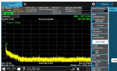
NTNV-DC_7A_n77A-PC2-30-5+40-M+H-QPSK-IDLE-DFT-QPSK-Inner_1RB_Right-0.15-30-PASS
