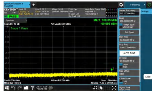
NTVN-DC_7A_n77A-PC2-30-5+25-M+M-QPSK-IDLE-DFT-BPSK-Inner_1RB_Right-30-1000-PASS
