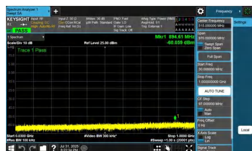
NTNV-DC_7A_n77A-PC2-30-5+30-M+L-QPSK-IDLE-DFT-QPSK-In ner_1RB_Right-30-1000-PASS
