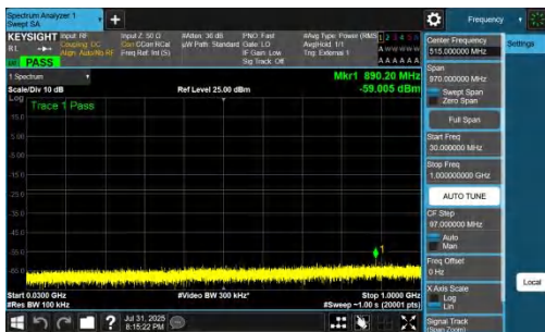
NTNV-DC_7A_n77A-PC2-30-5+30-M+L-QPSK-IDLE-DFT-BPSK-In ner_1RB_Left-30-1000-PASS
