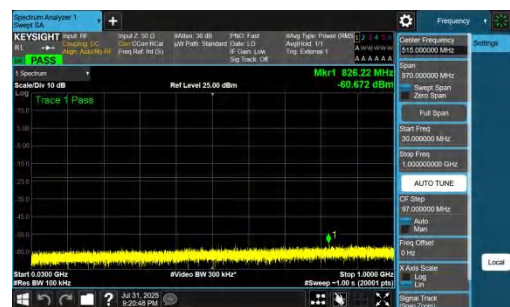
NTNV-DC_7A_n77A-PC2-30-5+50-M+L-QPSK-IDLE-DFT-QPSK-In ner_1RB_Right-30-1000-PASS
