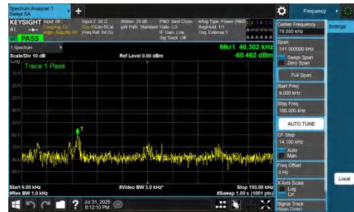
NTNV-DC_7A_n77A-PC2-30-5+25-M+H-QPSK-IDLE-DFT-QPSK-Inner_1RB_Right-0.009-0.15-PASS
