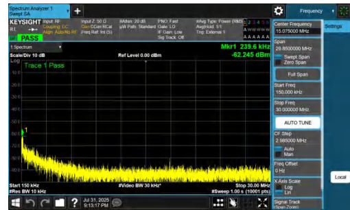
NTNV-DC_7A_n77A-PC2-30-5+50-M+L-QPSK-IDLE-DFT-BPSK-In ner_1RB_Left-0.15-30-PASS
