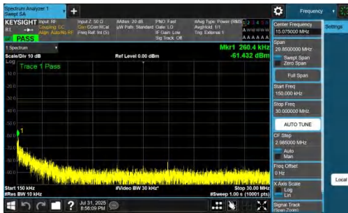
NTNV-DC_7A_n77A-PC2-30-5+40-M+M-QPSK-IDLE-DFT-BPSK-I nner_1RB_Right-0.15-30-PASS
