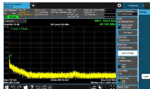
NTNV-DC_7A_n77A-PC2-30-5+15-M+H-QPSK-IDLE-DFT-BPSK-Inner_1RB_Left-0.15-30-PASS
