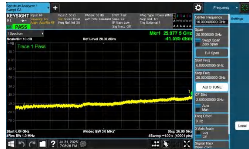
NTNV-DC_7A_n77A-PC2-30-5+15-M+H-QPSK-IDLE-DFT-BPSK-In ner_1RB_Left-6000-26000-PASS
