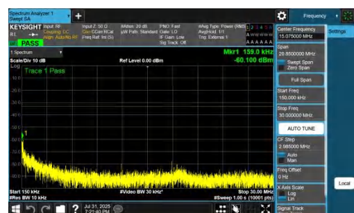
NTNV-DC_7A_n77A-PC2-30-5+20-M+L-QPSK-IDLE-DFT-QPSK-In ner_1RB_Left-0.15-30-PASS
