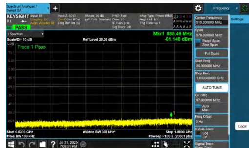
NTNV-DC_7A_n77A-PC2-30-5+15-M+H-QPSK-IDLE-DFT-BPSK-In ner_1RB_Right-30-1000-PASS
