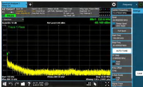
NTNV-DC_7A_n77A-PC2-30-5+10-M+H-QPSK-IDLE-DFT-BPSK-In nner_1RB_Right-0.15-30-PASS
