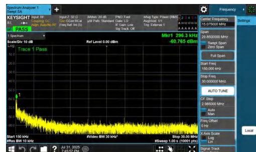
NTNV-DC_7A_n77A-PC2-30-5+25-M+L-QPSK-IDLE-DFT-BPSK-Inner_1RB_Left-0.15-30-PASS
