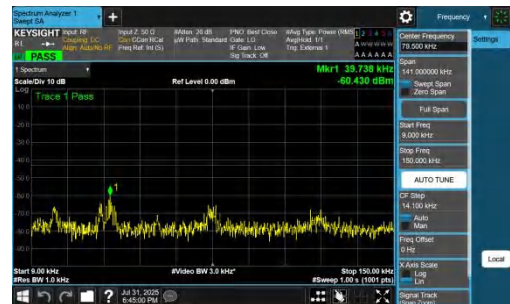
NTNV-DC_7A_n77A-PC2-30-5+10-M+H-QPSK-IDLE-DFT-QPSK-In ner_1RB_Right-0.009-0.15-PASS
