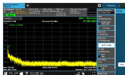
NTNV-DC_7A_n77A-PC2-30-5+20-M+H-QPSK-IDLE-DFT-QPSK-In ner_1RB_Left-0.15-30-PASS
