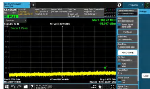
NTNV-DC_7A_n77A-PC2-30-5+15-M+L-QPSK-IDLE-DFT-BPSK-In ner_1RB_Right-30-1000-PASS
