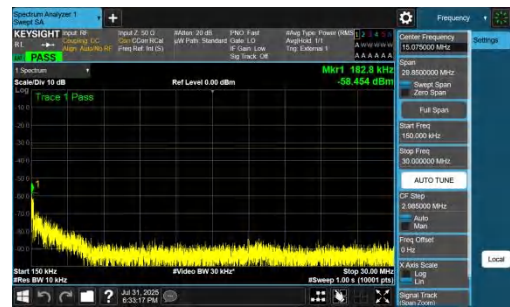
NTNV-DC_7A_n77A-PC2-30-5+10-M+M-QPSK-IDLE-DFT-QPSK-Inner_1RB_Left-0.15-30-PASS
