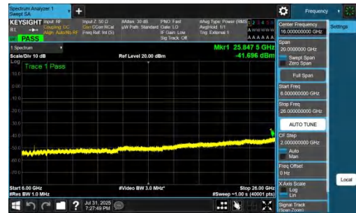
NTVN-DC_7A_n77A-PC2-30-5+20-M+M-QPSK-IDLE-DFT-BPSK-Inner_1RB_Left-6000-26000-PASS
