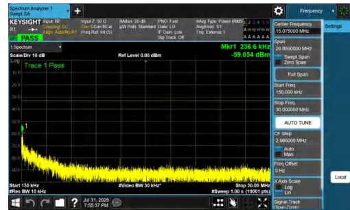
NTNV-DC_7A_n77A-PC2-30-5+25-M+M-QPSK-IDLE-DFT-BPSK-In ner_1RB_Left-0.15-30-PASS
