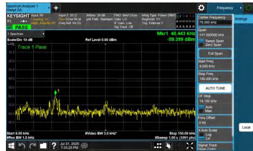
NTNV-DC_7A_n77A-PC2-30-5+20-M+M-QPSK-IDLE-DFT-QPSK-Inner_1RB_Right-0.009-0.15-PASS
