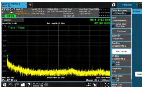
NTNV-DC_7A_n77A-PC2-30-5+15-M+H-QPSK-IDLE-DFT-BPSK-I nner_1RB_Right-0.15-30-PASS
