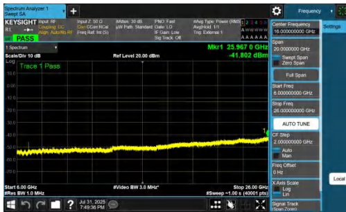
NTNV-DC_7A_n77A-PC2-30-5+25-M+L-QPSK-IDLE-DFT-BPSK-In ner_1RB_Right-6000-26000-PASS
