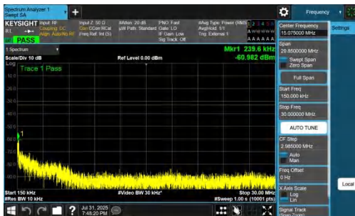
NTNV-DC_7A_n77A-PC2-30-5+25-M+L-QPSK-IDLE-DFT-BPSK-In ner_1RB_Right-0.15-30-PASS
