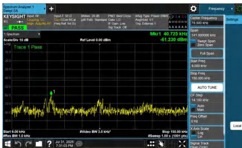
NTNV-DC_7A_n77A-PC2-30-5+20-M+M-QPSK-IDLE-DFT-QPSK-Inner_1RB_Left-0.009-0.15-PASS
