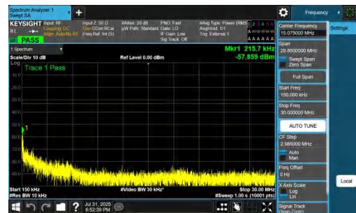
NTNV-DC_7A_n77A-PC2-30-5+15-M+L-QPSK-IDLE-DFT-QPSK-In ner_1RB_Left-0.15-30-PASS
