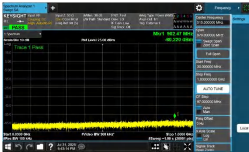
NTNV-DC_7A_n77A-PC2-30-5+10-M+H-QPSK-IDLE-DFT-QPSK-I nner_1RB_Left-30-1000-PASS
