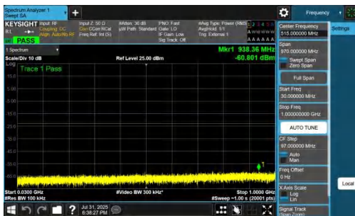
NTNV-DC_7A_n77A-PC2-30-5+10-M+H-QPSK-IDLE-DFT-BPSK-Inner_1RB_Left-30-1000-PASS
