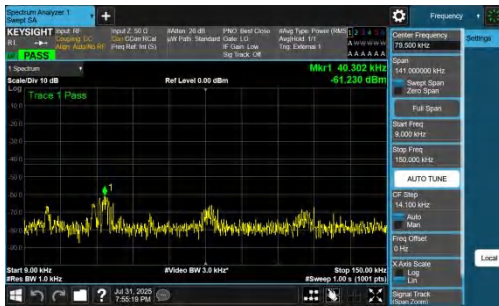
NTNV-DC_7A_n77A-PC2-30-5+25-M+M-QPSK-IDLE-DFT-BPSK-In nner_1RB_Left-0.009-0.15-PASS
