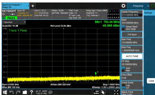
NTNV-DC_7A_n77A-PC2-30-5+15-M+M-QPSK-IDLE-DFT-QPSK-I nner 1RB Left-30-1000-PASS
