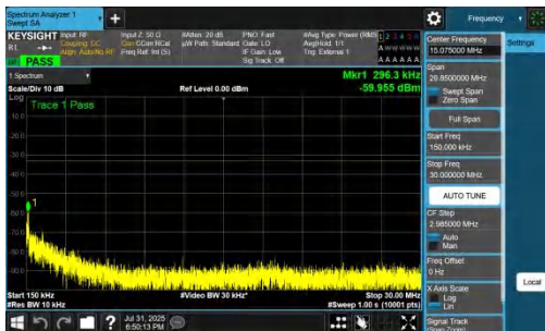
NTNV-DC_7A_n77A-PC2-30-5+15-M+L-QPSK-IDLE-DFT-BPSK-In ner_1RB_Right-0.15-30-PASS
