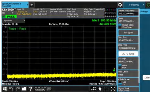
NTNV-DC_7A_n77A-PC2-30-5+20-M+L-QPSK-IDLE-DFT-QPSK-In ner_1RB_Left-30-1000-PASS
