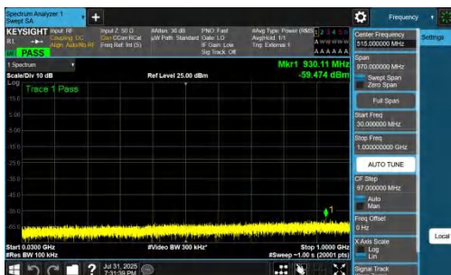
NTNV-DC_7A_n77A-PC2-30-5+20-M+M-QPSK-IDLE-DFT-QPSK-Inner_1RB_Left-30-1000-PASS
