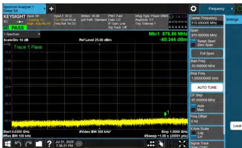
NTNV-DC_7A_n77A-PC2-30-5+20-M+H-QPSK-IDLE-DFT-BPSK-Inner_1RB_Left-30-1000-PASS
