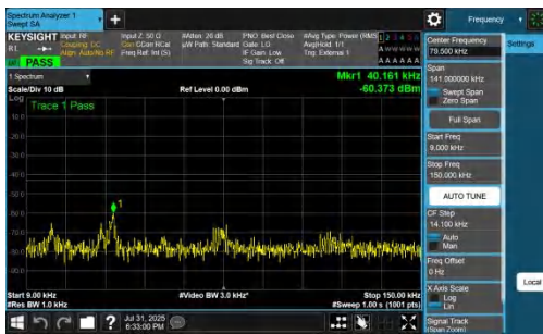
NTNV-DC_7A_n77A-PC2-30-5+10-M+M-QPSK-IDLE-DFT-QPSK-Inner_1RB_Left-0.009-0.15-PASS
