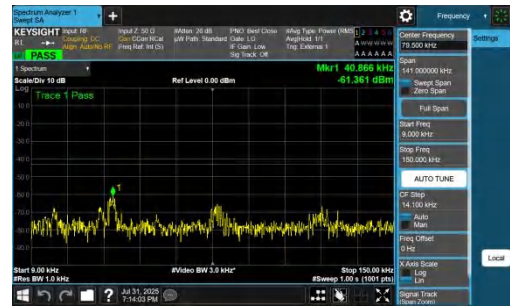
NTNV-DC_7A_n77A-PC2-30-5+15-M+H-QPSK-IDLE-DFT-QPSK-Inner_1RB_Right-0.009-0.15-PASS
