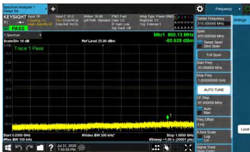
NTNV-DC_7A_n77A-PC2-30-5+25-M+M-QPSK-IDLE-DFT-BPSK-In nner_1RB_Left-30-1000-PASS
