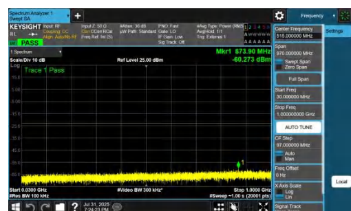
NTNV-DC_7A_n77A-PC2-30-5+20-M+L-QPSK-IDLE-DFT-QPSK-In ner_1RB_Right-30-1000-PASS
