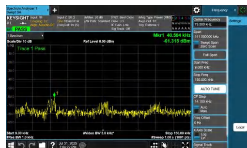
NTNV-DC_7A_n77A-PC2-30-5+15-M+M-QPSK-IDLE-DFT-QPSK-In ner 1RB Right-0.009-0.15-PASS
