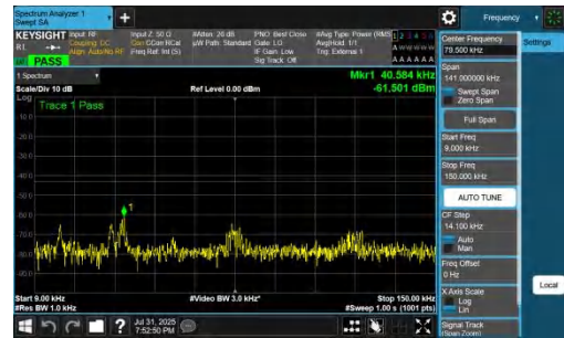
NTNV-DC_7A_n77A-PC2-30-5+25-M+L-QPSK-IDLE-DFT-QPSK-In_ner_1RB_Right-0.009-0.15-PASS
