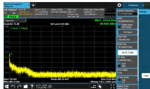
NTNV-DC_7A_n77A-PC2-30-5+20-M+M-QPSK-IDLE-DFT-QPSK-Inner_1RB_Left-0.15-30-PASS
