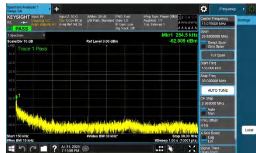
NTNV-DC_7A_n77A-PC2-30-5+15-M+H-QPSK-IDLE-DFT-QPSK-Inner_1RB_Left-0.15-30-PASS
