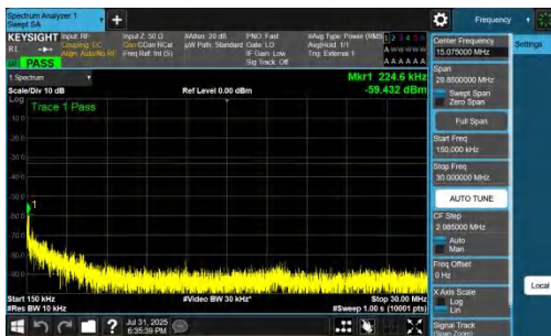
NTNV-DC_7A_n77A-PC2-30-5+10-M+M-QPSK-IDLE-DFT-QPSK-I nner_1RB_Right-0.15-30-PASS
