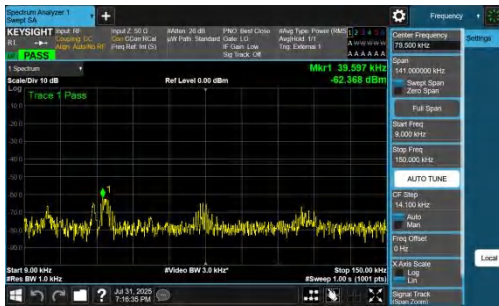
NTNV-DC_7A_n77A-PC2-30-5+20-M+L-QPSK-IDLE-DFT-BPSK-In ner_1RB_Left-0.009-0.15-PASS
