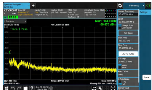
NTNV-n77(3700-3980)-PC2-30-70-M-DFT-BPSK-Inner_1RB_Left-0.15 -30-PASS
