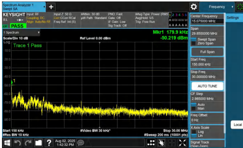
NTNV-n77(3700-3980)-PC2-30-70-L-DFT-BPSK-Inner_1RB_Right-0.15-30-PASS
