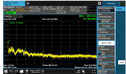
NTNV-n77(3700-3980)-PC2-30-70-H-DFT-BPSK-Inner_1RB_Left-0.15- 30-PASS
