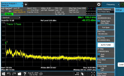
NTNV-n77(3700-3980)-PC2-30-60-H-DFT-QPSK-Inner_1RB_Right-0.15 30-30-PASS
