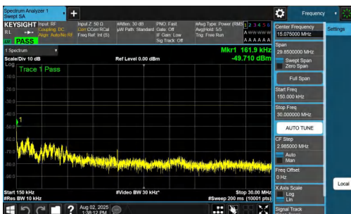
NTNV-n77(3700-3980)-PC2-30-60-H-DFT-BPSK-Inner_1RB_Right-0. 15-30-PASS
