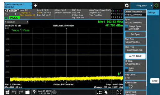
NTNV-n77(3700-3980)-PC2-30-60-H-DFT-QPSK-Inner_1RB_Right-30.30 1000-PASS
