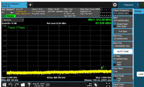
NTNV-n77(3700-3980)-PC2-30-60-L-DFT-QPSK-Inner_1RB_Left-3000-1000-PASS
