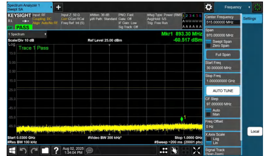
NTNV-n77(3700-3980)-PC2-30-60-M-DFT-BPSK-Inner_1RB_Right-30-1000-PASS
