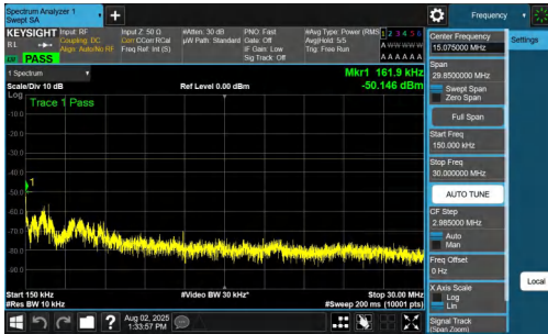
NTNV-n77(3700-3980)-PC2-30-60-M-DFT-BPSK-Inner_1RB_Right-0.15-30-PASS
