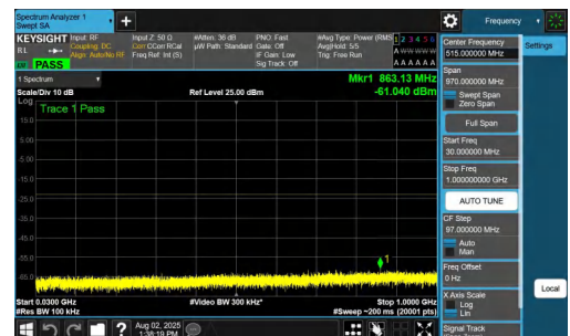
NTNV-n77(3700-3980)-PC2-30-60-H-DFT-BPSK-Inner_1RB_Right-30- 1000-PASS
