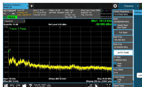
NTNV-n77(3700-3980)-PC2-30-70-L-DFT-BPSK-Inner_1RB_Left-0.15-30-PASS
