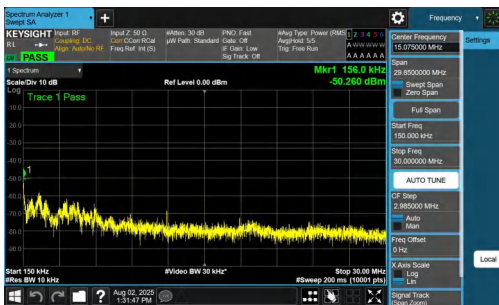
NTNV-n77(3700-3980)-PC2-30-60-L-DFT-QPSK-Inner_1RB_Right-0. 15-30-PASS
