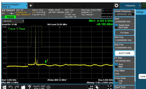
NTNV-n77(3700-3980)-PC2-30-60-M-DFT-BPSK-Inner_1RB_Left-300 0-6000-PASS
