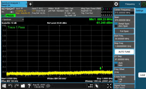
NTNV-n77(3700-3980)-PC2-30-60-M-DFT-QPSK-Inner_1RB_Left-30-1000-PASS
