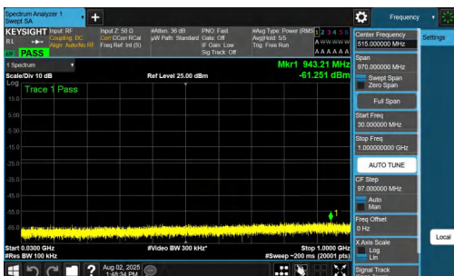
NTNV-n77(3700-3980)-PC2-30-70-M-DFT-QPSK-Inner_1RB_Left-30-1000-PASS
