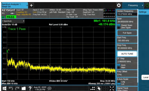
NTNV-n77(3700-3980)-PC2-30-70-M-DFT-QPSK-Inner_1RB_Right-0.15-30-PASS
