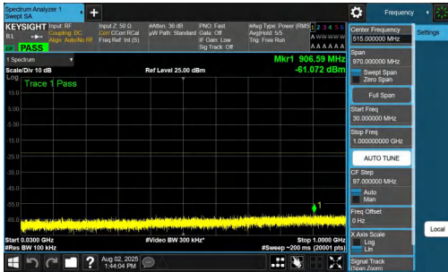
NTNV-n77(3700-3980)-PC2-30-70-L-DFT-QPSK-Inner_1RB_Left-30-1000-PASS
