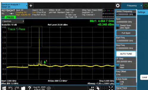
NTNV-n77(3700-3980)-PC2-30-70-H-DFT-BPSK-Inner_1RB_Left-300 0-6000-PASS
