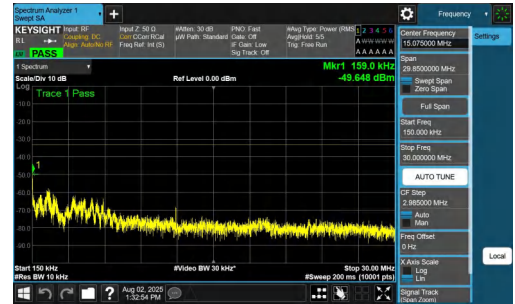
NTNV-n77(3700-3980)-PC2-30-60-M-DFT-BPSK-Inner_1RB_Left-0.15 -30-PASS
