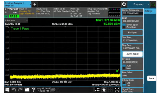
NTNV-n77(3700-3980)-PC2-30-70-L-DFT-BPSK-Inner_1RB_Right-30-1000-PASS
