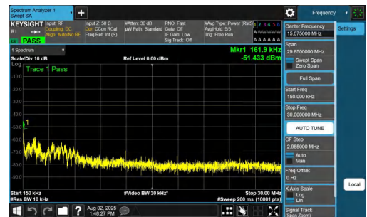
NTNV-n77(3700-3980)-PC2-30-70-M-DFT-QPSK-Inner_1RB_Left-0.15-30-PASS
