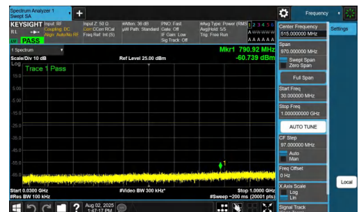
NTNV-n77(3700-3980)-PC2-30-70-M-DFT-BPSK-Inner_1RB_Right-30- 1000-PASS
