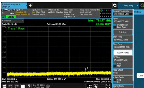
NTNV-n77(3700-3980)-PC2-30-60-H-DFT-QPSK-Inner_1RB_Left-30-1000-PASS
