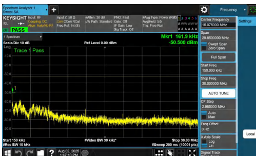
NTNV-n77(3700-3980)-PC2-30-70-M-DFT-BPSK-Inner_1RB_Right-0. 15-30-PASS
