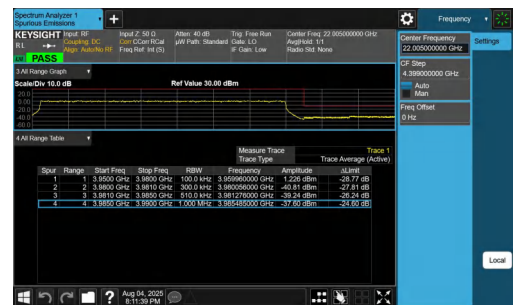
NTNV-n77(3700-3980)-PC2-30-30-H-DFT-QPSK-Outer_Full-PASS
