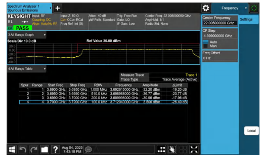
NTNV-n77(3700-3980)-PC2-30-20-L-DFT-BPSK-Outer_Full-PASS
