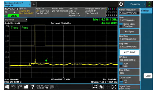
NTNV-n77(3700-3980)-PC2-30-10-L-DFT-QPSK-Inner_1RB_Right-300 0-6000-PASS
