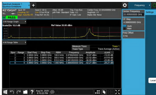
NTNV-n77(3700-3980)-PC2-30-30-H-DFT-BPSK-Edge_1RB_Right-PASS
