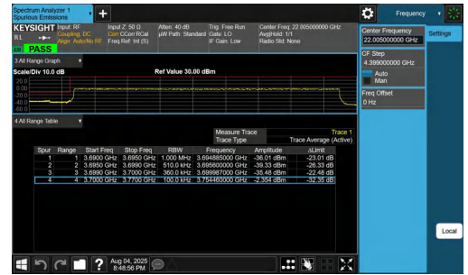
NTNV-n77(3700-3980)-PC2-30-70-L-DFT-QPSK-Outer_Full-PASS
