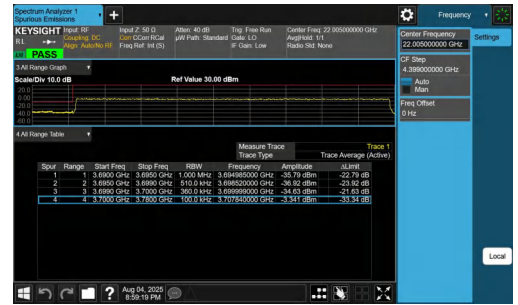
NTNV-n77(3700-3980)-PC2-30-80-L-DFT-QPSK-Outer_Full-PASS
