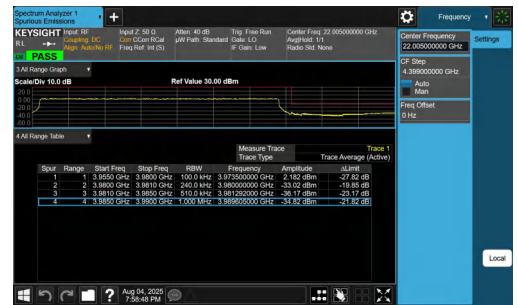
NTNV-n77(3700-3980)-PC2-30-25-H-DFT-BPSK-Outer_Full-PASS
