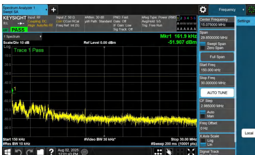
NTNV-n77(3700-3980)-PC2-30-10-M-DFT-BPSK-Inner_1RB_Right-0. 15-30-PASS
