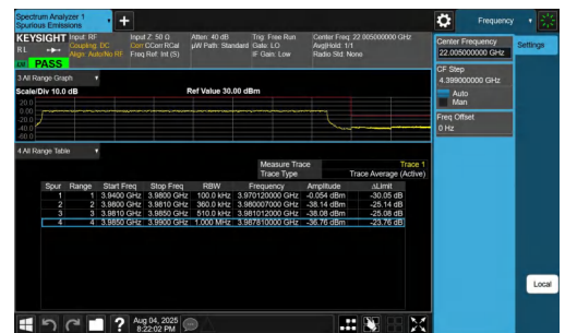
NTNV-n77(3700-3980)-PC2-30-40-H-DFT-QPSK-Outer_Full-PASS
