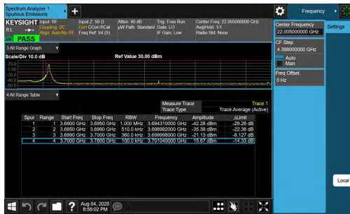
NTNV-n77(3700-3980)-PC2-30-80-L-DFT-BPSK-Edge_1RB_Left-PASS
