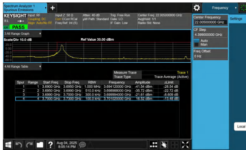
NTNV-n77(3700-3980)-PC2-30-30-L-DFT-BPSK-Edge_1RB_Left-PASS
