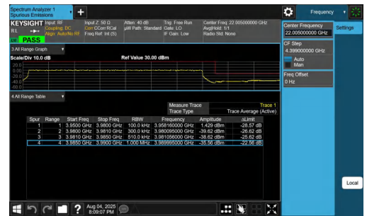
NTNV-n77(3700-3980)-PC2-30-30-H-DFT-BPSK-Outer_Full-PASS
