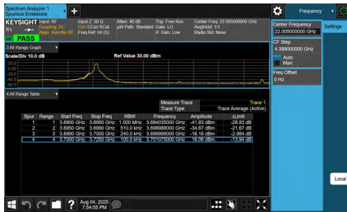
NTNV-n77(3700-3980)-PC2-30-25-L-DFT-BPSK-Edge_1RB_Left-PASS
