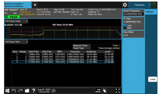
NTNV-n77(3700-3980)-PC2-30-25-L-DFT-BPSK-Outer_Full-PASS
