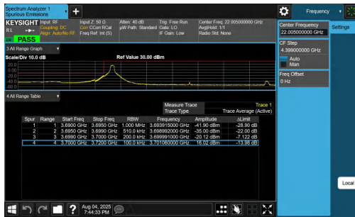
NTNV-n77(3700-3980)-PC2-30-20-L-DFT-BPSK-Edge_1RB_Left-PASS
