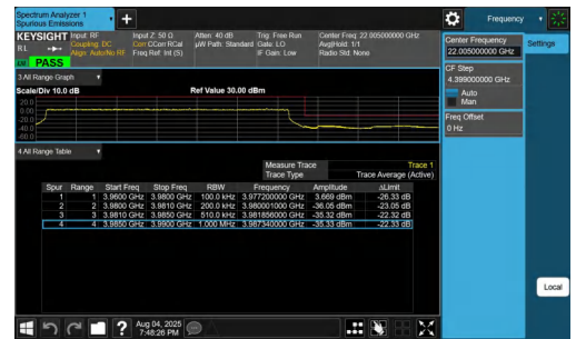
NTNV-n77(3700-3980)-PC2-30-20-H-DFT-BPSK-Outer_Full-PASS
