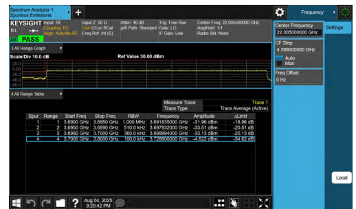
NTNV-n77(3700-3980)-PC2-30-100-L-DFT-QPSK-Outer_Full-PASS S
