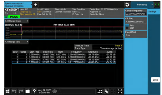
NTNV-n77(3700-3980)-PC2-30-90-L-DFT-QPSK-Outer_Full-PASS
