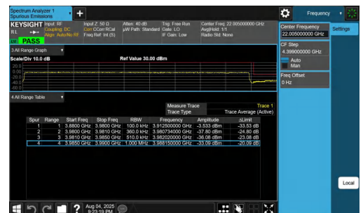
NTNV-n77(3700-3980)-PC2-30-100-H-DFT-BPSK-Outer_Full-PAS S
