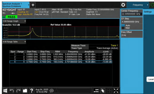
NTNV-n77(3700-3980)-PC2-30-40-L-DFT-BPSK-Edge_1RB_Left-PASS
