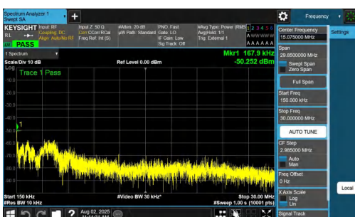
NTNV-n77(3700-3980)-PC2-30-10-L-DFT-QPSK-Inner_1RB_Right-0.15-30-PASS
