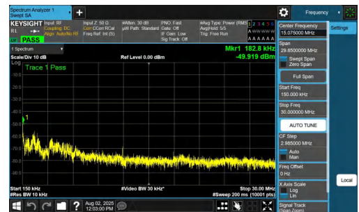
NTVN-n77(3700-3980)-PC2-30-10-M-DFT-QPSK-Inner_1RB_Left-0.15-30-PASS
