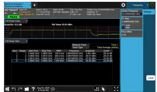
NTNV-n77(3700-3980)-PC2-30-40-H-DFT-BPSK-Outer_Full-PASS
