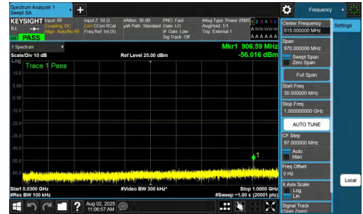
NTVN-n77(3700-3980)-PC2-30-10-L-DFT-BPSK-Inner_1RB_Right-30-1000-PASS
