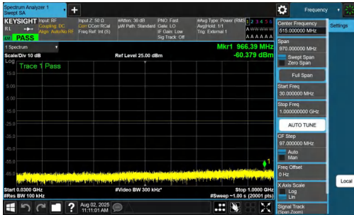
NTNV-n77(3700-3980)-PC2-30-10-L-DFT-QPSK-Inner_1RB_Left-30-1000-PASS
