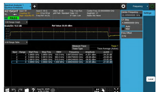
NTNV-n77(3700-3980)-PC2-30-100-H-DFT-QPSK-Outer_Full-PAS S
