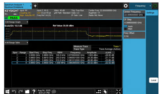
NTNV-n77(3700-3980)-PC2-30-25-H-DFT-QPSK-Outer_Full-PASS
