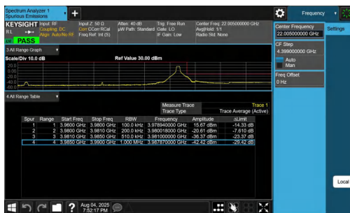
NTNV-n77(3700-3980)-PC2-30-20-H-DFT-QPSK-Edge_1RB_Right-PASS
