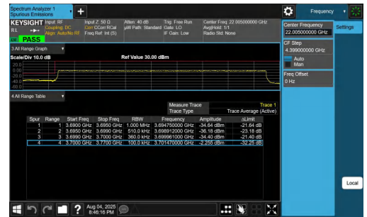
NTNV-n77(3700-3980)-PC2-30-70-L-DFT-BPSK-Outer_Full-PASS
