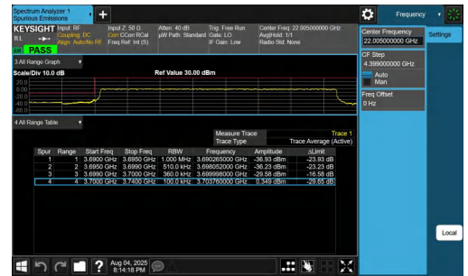
NTNV-n77(3700-3980)-PC2-30-40-L-DFT-BPSK-Outer_Full-PASS
