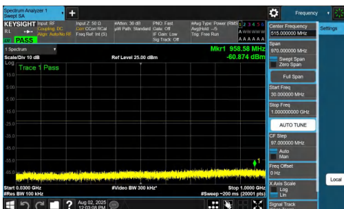
NTVN-n77(3700-3980)-PC2-30-10-M-DFT-QPSK-Inner_1RB_Left-30-1000-PASS
