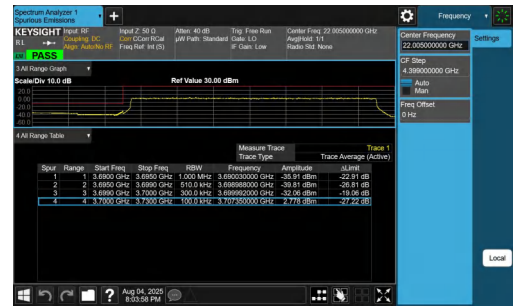
NTNV-n77(3700-3980)-PC2-30-30-L-DFT-BPSK-Outer_Full-PASS
