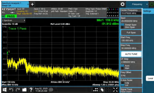
NTVN-n77(3700-3980)-PC2-30-10-L-DFT-BPSK-Inner_1RB_Right-0.15-30-PASS
