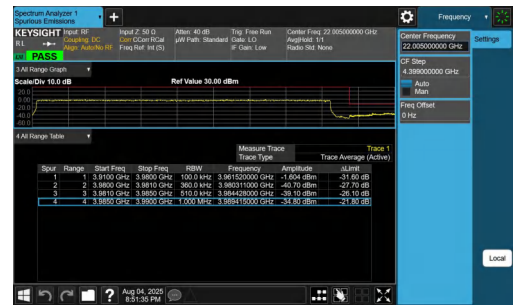
NTNV-n77(3700-3980)-PC2-30-70-H-DFT-BPSK-Outer_Full-PASS
