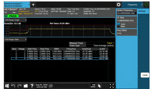
NTNV-n77(3700-3980)-PC2-30-50-L-DFT-BPSK-Outer_Full-PASS
