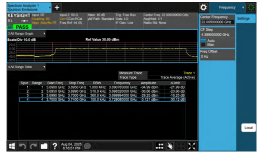
NTNV-n77(3700-3980)-PC2-30-40-L-DFT-QPSK-Outer_Full-PASS
