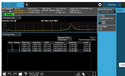
NTNV-n77(3700-3980)-PC2-30-30-H-DFT-QPSK-Edge_1RB_Right-PASS
