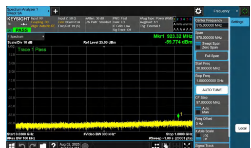
NTNV-n77(3700-3980)-PC2-30-10-L-DFT-QPSK-Inner_1RB_Right-30-1000-PASS
