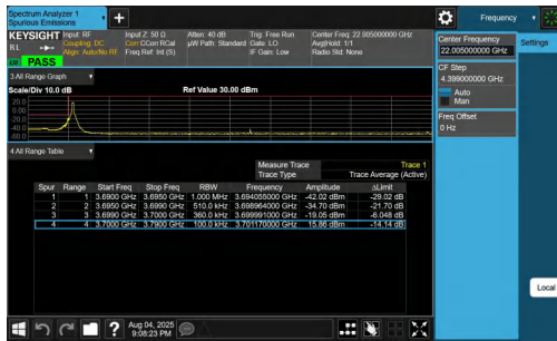
NTNV-n77(3700-3980)-PC2-30-90-L-DFT-BPSK-Edge_1RB_Left-PASS
