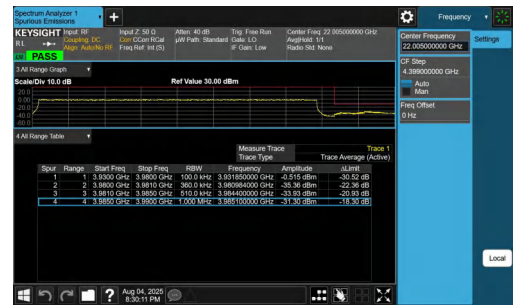
NTNV-n77(3700-3980)-PC2-30-50-H-DFT-BPSK-Outer_Full-PASS
