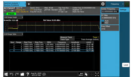
NTNV-n77(3700-3980)-PC2-30-90-L-DFT-BPSK-Outer_Full-PASS
