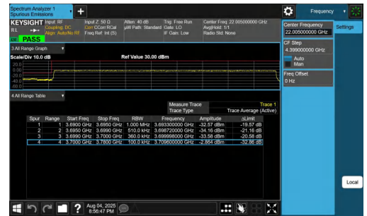
NTNV-n77(3700-3980)-PC2-30-80-L-DFT-BPSK-Outer_Full-PASS
