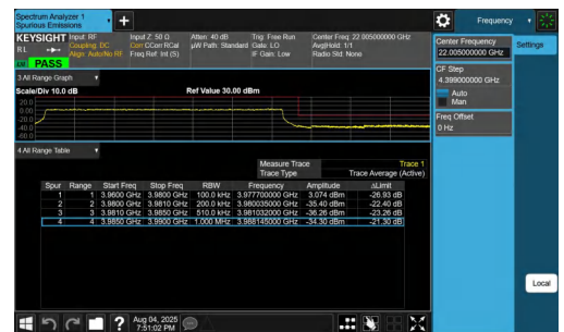
NTNV-n77(3700-3980)-PC2-30-20-H-DFT-QPSK-Outer_Full-PASS
