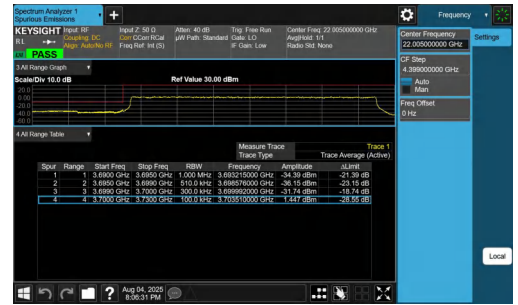
NTNV-n77(3700-3980)-PC2-30-30-L-DFT-QPSK-Outer_Full-PASS
