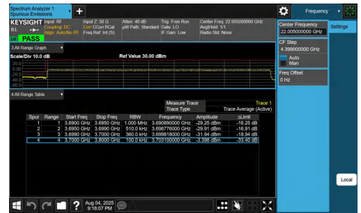
NTNV-n77(3700-3980)-PC2-30-100-L-DFT-BPSK-Outer_Full-PASS S
