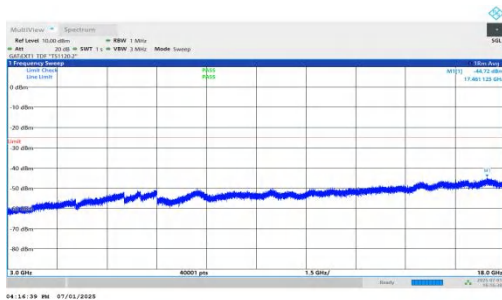
NTNV-n41-PC2-30-30-L-DFT-BPSK-Inner_1RB_Right-3000-1800 0-PASS
