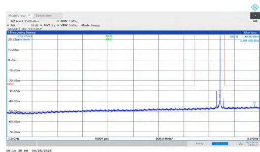
NTNV-n41-PC2-30-30-H-DFT-QPSK-Inner_1RB_Right-1000-3000- -PASS
