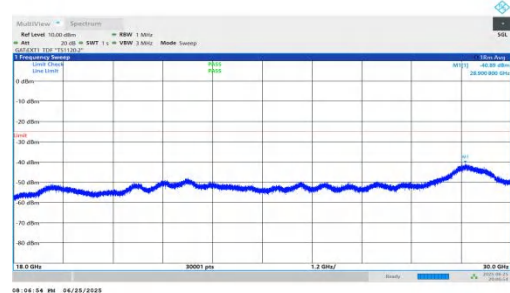
NTNV-n41-PC2-30-30-H-DFT-BPSK-Inner_1RB_Left-18000-30000-PASS 0-PASS
