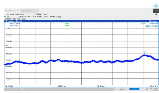
NTNV-n41-PC2-30-25-H-DFT-QPSK-Inner_1RB_Right-18000-30000-PASS
