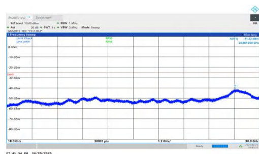
NTVN-n41-PC2-30-25-L-DFT-QPSK-Inner_1RB_Right-18000-30000 00-PASS
