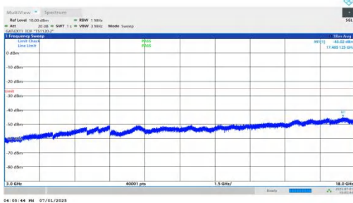
NTNV-n41-PC2-30-20-L-DFT-BPSK-Inner_1RB_Right-3000-18000-PASS
