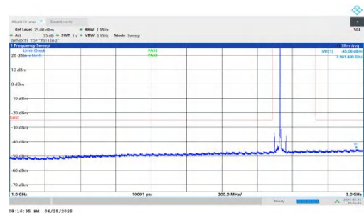
NTVN-n41-PC2-30-35-L-DFT-QPSK-Inner_1RB_Right-1000-3000-P PASS
