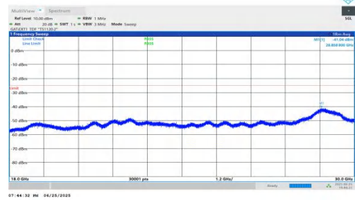
NTNV-n41-PC2-30-25-M-DFT-BPSK-Inner_1RB_Right-18000-3000-PASS
