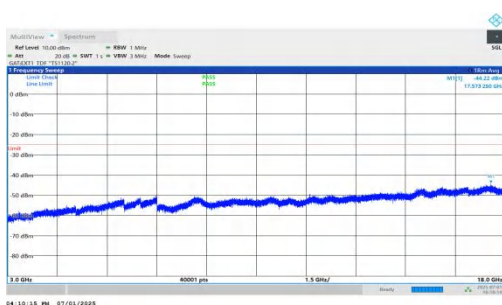
NTNV-n41-PC2-30-20-H-DFT-QPSK-Inner_1RB_Right-3000-18000-PASS
