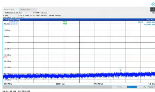
NTNV-n41-PC2-30-30-M-DFT-QPSK-Inner_1RB_Right-30-1000- PASS
