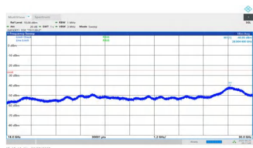
NTVN-n41-PC2-30-35-L-DFT-QPSK-Inner_1RB_Right-18000-3000 00-PASS
