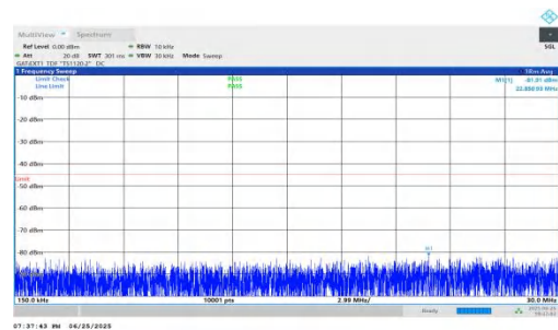
NTNV-n41-PC2-30-25-L-DFT-BPSK-Inner_1RB_Right-0.15-30-PA SS
