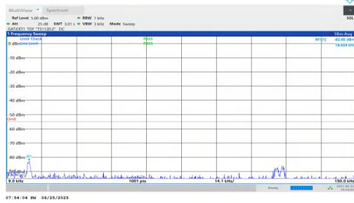
NTNV-n41-PC2-30-30-L-DFT-BPSK-Inner_1RB_Left-0.009-0.15-PASS
