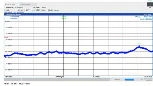
NTVN-n41-PC2-30-35-L-DFT-QPSK-Inner_1RB_Left-18000-3000 0-PASS
