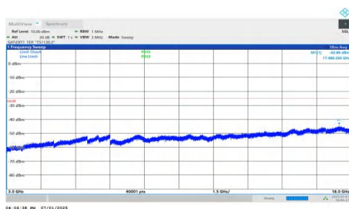
NTVN-n41-PC2-30-20-L-DFT-QPSK-Inner_1RB_Right-3000-180 00-PASS
