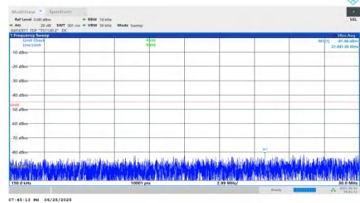
NTNV-n41-PC2-30-25-M-DFT-QPSK-Inner_1RB_Left-0.15-30-PASS
