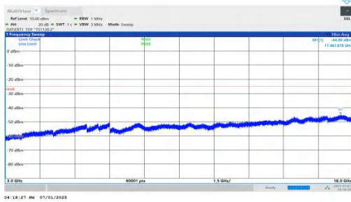
NTNV-n41-PC2-30-30-M-DFT-BPSK-Inner_1RB_Right-3000-18000-PASS
