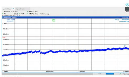
NTNV-n41-PC2-30-30-H-DFT-QPSK-Inner_1RB_Right-3000-180 00-PASS
