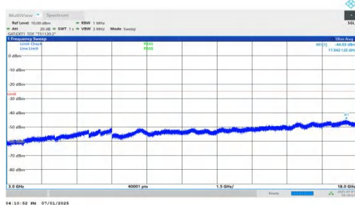
NTNV-n41-PC2-30-25-L-DFT-BPSK-Inner_1RB_Left-3000-18000 -PASS
