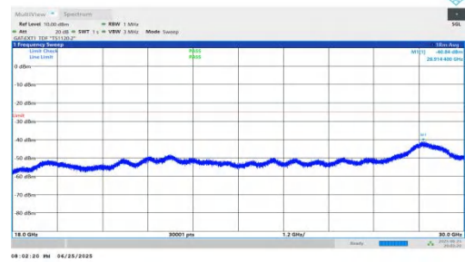
NTNV-n41-PC2-30-30-M-DFT-BPSK-Inner_1RB_Right-18000-300-PASS
