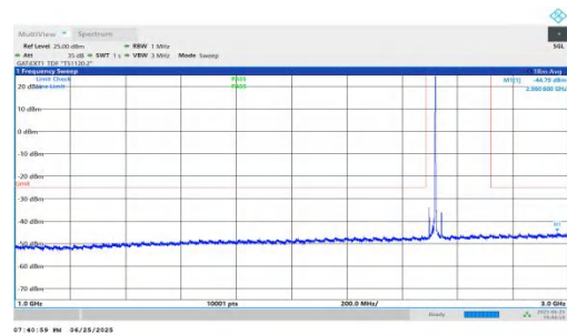
NTVN-n41-PC2-30-25-L-DFT-QPSK-Inner_1RB_Right-1000-3000-P PASS
