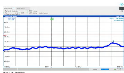
NTVN-n41-PC2-30-30-L-DFT-QPSK-Inner_1RB_Right-18000-3000 00-PASS
