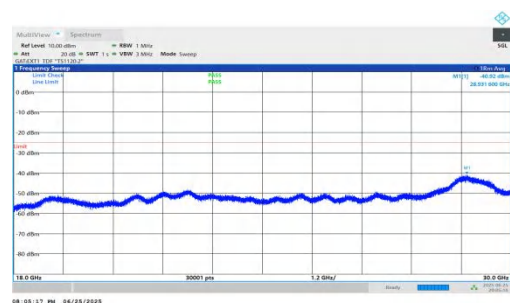
NTNV-n41-PC2-30-30-M-DFT-QPSK-Inner_1RB_Right-18000-3000- 00-PASS
