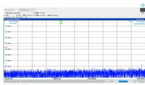
NTNV-n41-PC2-30-20-M-DFT-BPSK-Inner_1RB_Right-0.15-30-PASS
