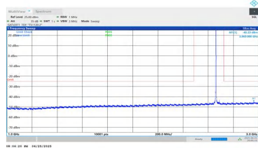
NTNV-n41-PC2-30-30-H-DFT-BPSK-Inner_1RB_Left-1000-3000-PASS ASS
