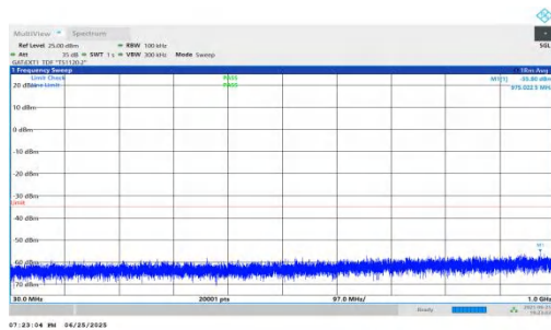
NTVN-n41-PC2-30-20-L-DFT-QPSK-Inner_1RB_Right-30-1000-P ASS
