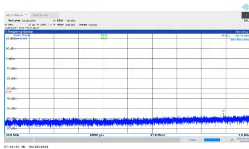
NTVN-n41-PC2-30-25-L-DFT-QPSK-Inner_1RB_Right-30-1000-P ASS
