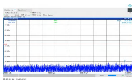
NTNV-n41-PC2-30-35-M-DFT-BPSK-Inner_1RB_Right-0.15-30-PASS
