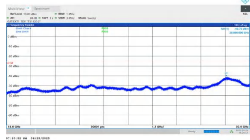
NTNV-n41-PC2-30-20-L-DFT-BPSK-Inner_1RB_Right-18000-3000-PASS
