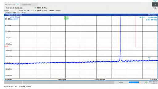
NTNV-n41-PC2-30-20-L-DFT-BPSK-Inner_1RB_Right-1000-3000-PASS
