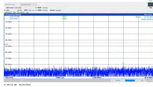
NTNV-n41-PC2-30-25-H-DFT-BPSK-Inner_1RB_Left-0.15-30-PASS
