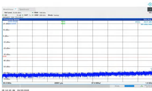
NTVN-n41-PC2-30-35-L-DFT-QPSK-Inner_1RB_Right-30-1000-P ASS
