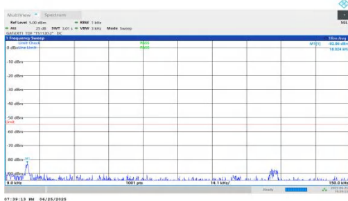
NTNV-n41-PC2-30-25-L-DFT-QPSK-Inner_1RB_Left-0.009-0.15-PASS
