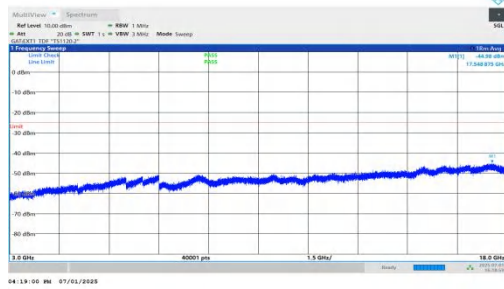
NTNV-n41-PC2-30-30-M-DFT-QPSK-Inner_1RB_Left-3000-1800 0-PASS
