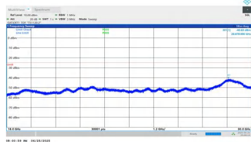
NTNV-n41-PC2-30-30-M-DFT-BPSK-Inner_1RB_Left-18000-30000-PASS
