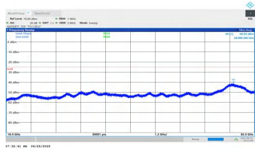
NTVN-n41-PC2-30-20-H-DFT-BPSK-Inner_1RB_Right-18000-300 00-PASS
