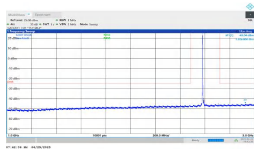
NTNV-n41-PC2-30-25-M-DFT-BPSK-Inner_1RB_Left-1000-3000-PASS
