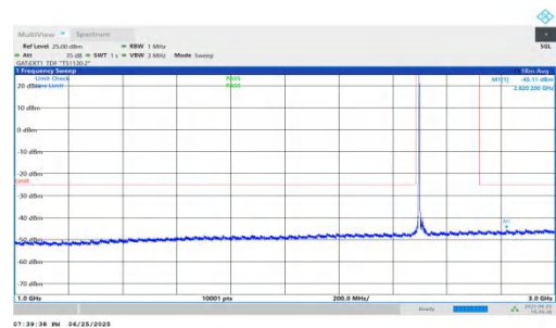
NTNV-n41-PC2-30-25-L-DFT-QPSK-Inner_1RB_Left-1000-3000-PASS
