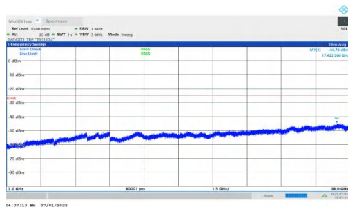
NTNV-n41-PC2-30-20-M-DFT-BPSK-Inner_1RB_Left-3000-18000-PASS
