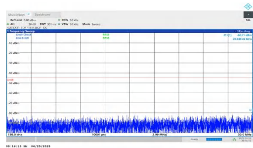
NTVN-n41-PC2-30-35-L-DFT-QPSK-Inner_1RB_Right-0.15-30-PA SS
