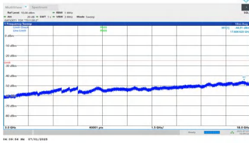
NTNV-n41-PC2-30-20-H-DFT-QPSK-Inner_1RB_Left-3000-1800 0-PASS
