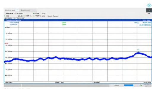
NTNV-n41-PC2-30-30-H-DFT-QPSK-Inner_1RB_Right-18000-300 00-PASS
