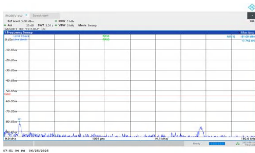
NTVN-n41-PC2-30-25-H-DFT-QPSK-Inner_1RB_Left-0.009-0.15- PASS
