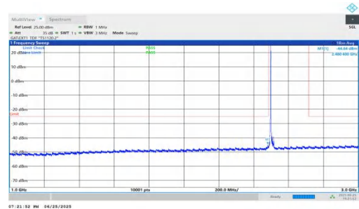
NTNV-n41-PC2-30-20-L-DFT-QPSK-Inner_1RB_Left-1000-3000-PASS
