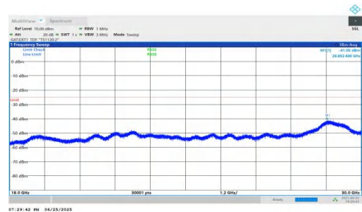
NTNV-n41-PC2-30-20-M-DFT-QPSK-Inner_1RB_Right-18000-30000- 00-PASS
