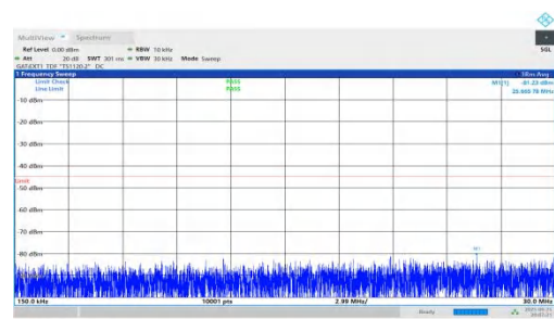
NTNV-n41-PC2-30-30-H-DFT-BPSK-Inner_1RB_Right-0.15-30-PASS SS
