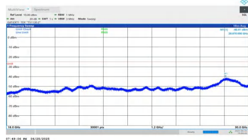
NTNV-n41-PC2-30-25-H-DFT-BPSK-Inner_1RB_Left-18000-30000-PASS
