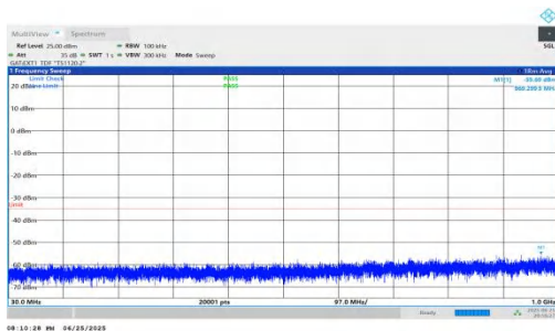
NTNV-n41-PC2-30-30-H-DFT-QPSK-Inner_1RB_Right-30-1000- PASS
