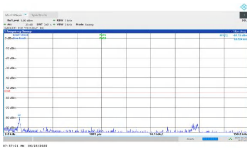
NTNV-n41-PC2-30-30-L-DFT-QPSK-Inner_1RB_Left-0.009-0.15- PASS
