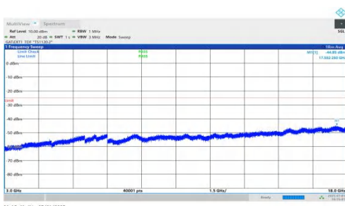
NTNV-n41-PC2-30-25-H-DFT-QPSK-Inner_1RB_Right-3000-18000-PASS
