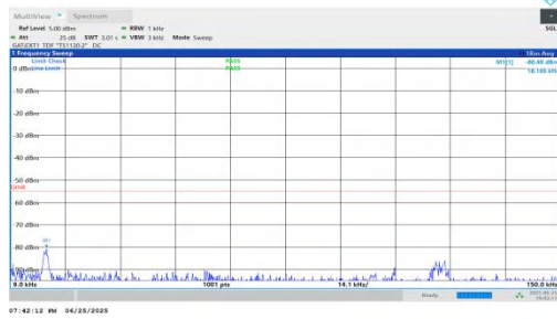
NTNV-n41-PC2-30-25-M-DFT-BPSK-Inner_1RB_Left-0.009-0.15-PASS
