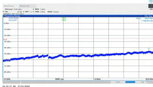
NTNV-n41-PC2-30-30-M-DFT-BPSK-Inner_1RB_Left-3000-18000-PASS
