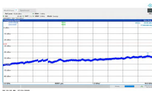
NTNV-n41-PC2-30-30-M-DFT-QPSK-Inner_1RB_Right-3000-18000- 00-PASS
