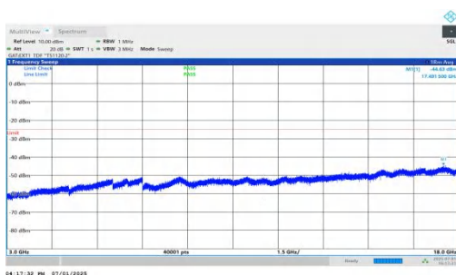
NTVN-n41-PC2-30-30-L-DFT-QPSK-Inner_1RB_Right-3000-18000 00-PASS
