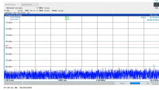
NTNV-n41-PC2-30-20-M-DFT-BPSK-Inner_1RB_Left-0.15-30-PASS
