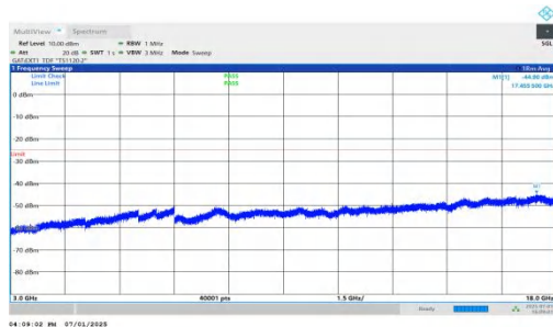
NTNV-n41-PC2-30-20-H-DFT-BPSK-Inner_1RB_Left-3000-18000-PASS 0-PASS
