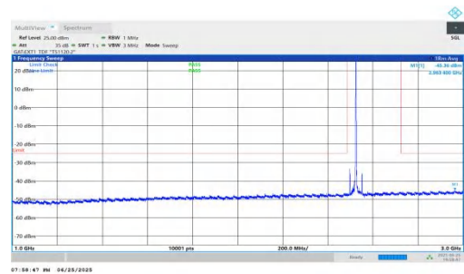
NTVN-n41-PC2-30-30-L-DFT-QPSK-Inner_1RB_Right-1000-3000-P PASS
