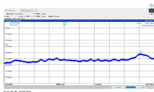
NTVN-n41-PC2-30-20-L-DFT-QPSK-Inner_1RB_Right-18000-300 00-PASS
