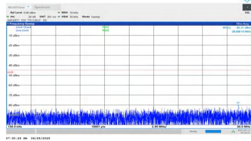
NTNV-n41-PC2-30-20-H-DFT-BPSK-Inner_1RB_Left-0.15-30-PAS S
