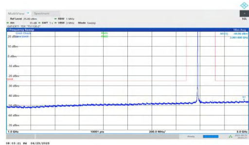
NTNV-n41-PC2-30-30-M-DFT-QPSK-Inner_1RB_Left-1000-3000-PASS
