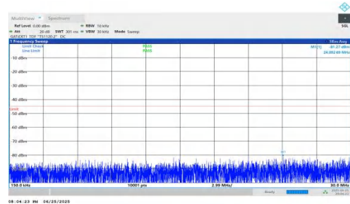
NTNV-n41-PC2-30-30-M-DFT-QPSK-Inner_1RB_Right-0.15-30-P ASS
