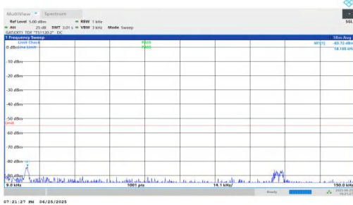
NTNV-n41-PC2-30-20-L-DFT-QPSK-Inner_1RB_Left-0.009-0.15-PASS
