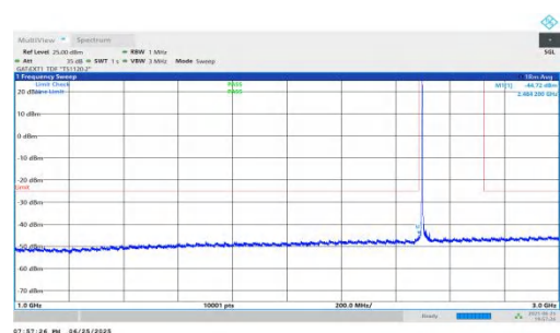
NTNV-n41-PC2-30-30-L-DFT-QPSK-Inner_1RB_Left-1000-3000-P ASS
