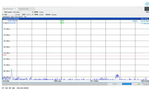
NTNV-n41-PC2-30-20-H-DFT-QPSK-Inner_1RB_Right-0.009-0.1 5-PASS
