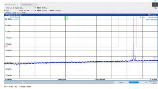
NTVN-n41-PC2-30-25-H-DFT-BPSK-Inner_1RB_Right-1000-3000 -PASS
