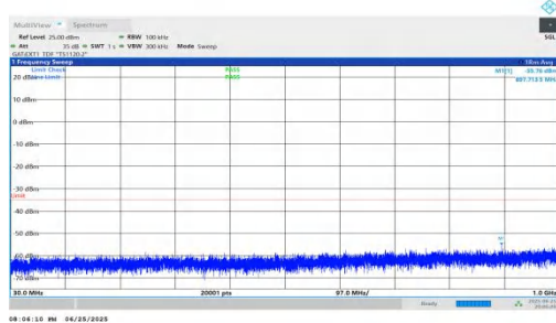
NTNV-n41-PC2-30-30-H-DFT-BPSK-Inner_1RB_Left-30-1000-PASS SS
