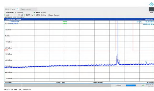
NTVN-n41-PC2-30-20-L-DFT-QPSK-Inner_1RB_Right-1000-3000- PASS
