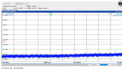
NTNV-n41-PC2-30-30-L-DFT-BPSK-Inner_1RB_Right-30-1000-P ASS
