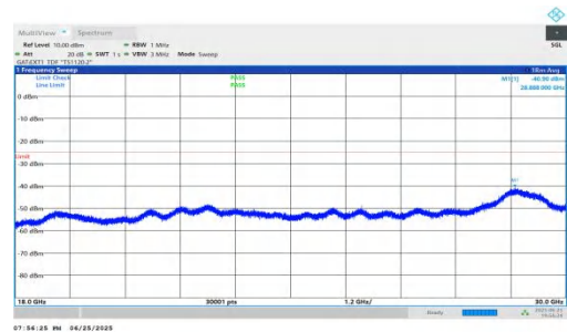
NTNV-n41-PC2-30-30-L-DFT-BPSK-Inner_1RB_Right-18000-300 00-PASS
