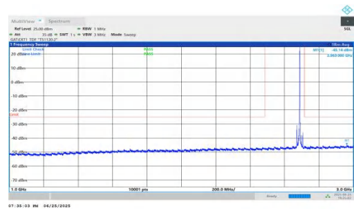
NTNV-n41-PC2-30-20-H-DFT-QPSK-Inner_1RB_Right-1000-3000-PASS
