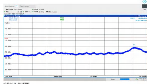
NTNV-n41-PC2-30-25-L-DFT-BPSK-Inner_1RB_Left-18000-30000 -PASS
