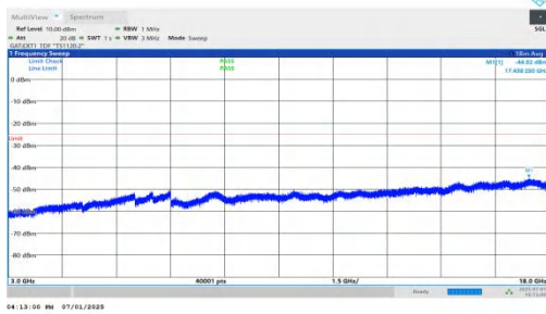
NTNV-n41-PC2-30-25-M-DFT-BPSK-Inner_1RB_Right-3000-18000-PASS
