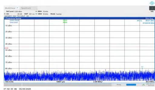
NTNV-n41-PC2-30-25-H-DFT-QPSK-Inner_1RB_Right-0.15-30-PA SS
