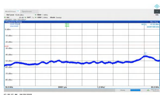
NTNV-n41-PC2-30-20-H-DFT-QPSK-Inner_1RB_Right-18000-30000-PASS
