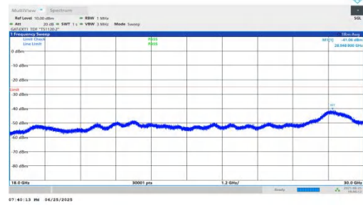
NTVN-n41-PC2-30-25-L-DFT-QPSK-Inner_1RB_Left-18000-3000 0-PASS
