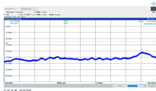
NTNV-n41-PC2-30-20-H-DFT-BPSK-Inner_1RB_Left-18000-30000-PASS 0-PASS
