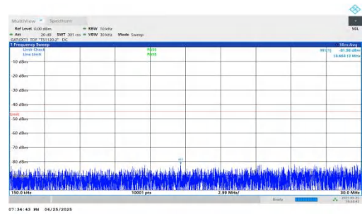
NTNV-n41-PC2-30-20-H-DFT-QPSK-Inner_1RB_Right-0.15-30-PA SS
