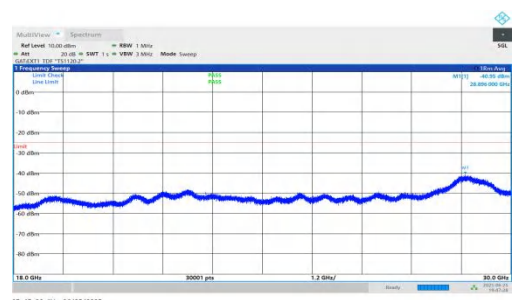
NTNV-n41-PC2-30-25-M-DFT-QPSK-Inner_1RB_Right-18000-3000 00-PASS
