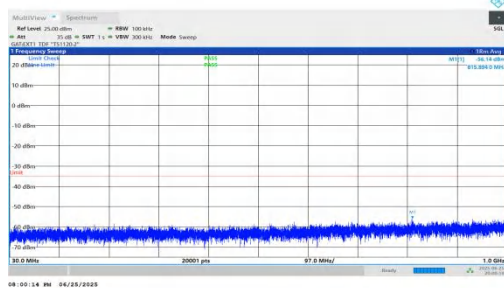
NTNV-n41-PC2-30-30-M-DFT-BPSK-Inner_1RB_Left-30-1000-PASS
