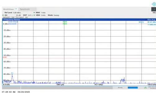
NTNV-n41-PC2-30-20-M-DFT-QPSK-Inner_1RB_Right-0.009-0.1 5-PASS
