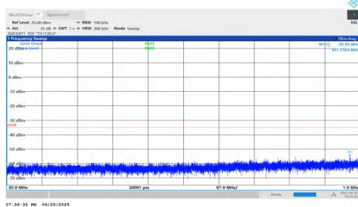
NTNV-n41-PC2-30-25-L-DFT-BPSK-Inner_1RB_Left-30-1000-PA SS
