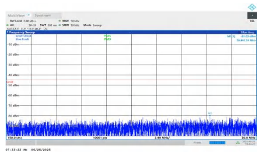
NTVN-n41-PC2-30-20-H-DFT-QPSK-Inner_1RB_Left-0.15-30-PAS S
