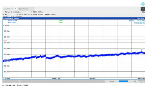
NTNV-n41-PC2-30-35-L-DFT-BPSK-Inner_1RB_Left-3000-18000-PASS
