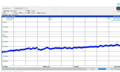
NTNV-n41-PC2-30-25-M-DFT-QPSK-Inner_1RB_Right-3000-1800 00-PASS
