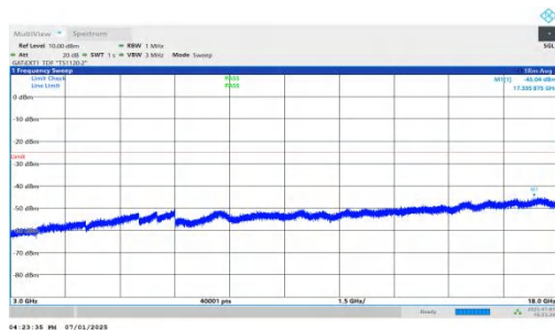
NTNV-n41-PC2-30-35-M-DFT-BPSK-Inner_1RB_Left-3000-18000-PASS
