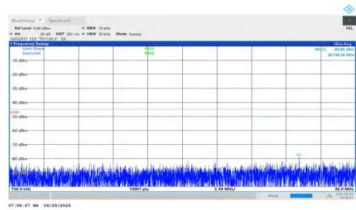
NTVN-n41-PC2-30-30-L-DFT-QPSK-Inner_1RB_Right-0.15-30-PA SS
