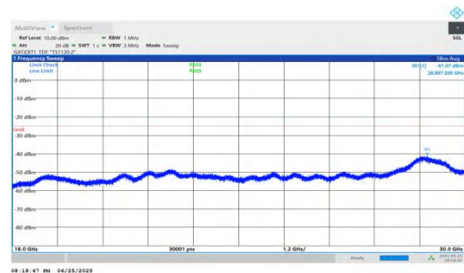
NTNV-n41-PC2-30-35-M-DFT-BPSK-Inner_1RB_Left-18000-30000-PASS
