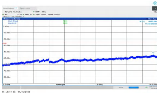
NTVN-n41-PC2-30-25-H-DFT-BPSK-Inner_1RB_Right-3000-180 00-PASS
