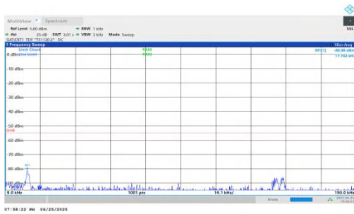
NTVN-n41-PC2-30-30-L-DFT-QPSK-Inner_1RB_Right-0.009-0.1 5-PASS
