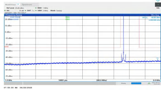
NTNV-n41-PC2-30-30-L-DFT-BPSK-Inner_1RB_Right-1000-3000-P PASS
