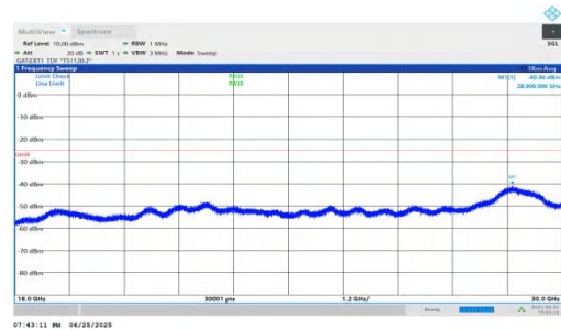
NTNV-n41-PC2-30-25-M-DFT-BPSK-Inner_1RB_Left-18000-30000-PASS
