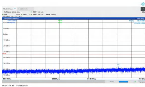
NTNV-n41-PC2-30-20-H-DFT-QPSK-Inner_1RB_Right-30-1000-PASS
