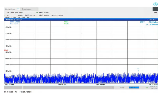
NTNV-n41-PC2-30-30-L-DFT-BPSK-Inner_1RB_Right-0.15-30-PASS
