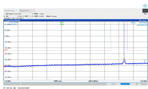
NTVN-n41-PC2-30-20-H-DFT-QPSK-Inner_1RB_Left-1000-3000- PASS
