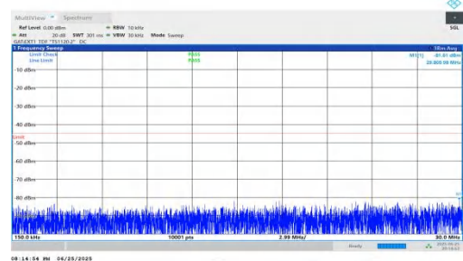
NTNV-n41-PC2-30-35-L-DFT-QPSK-Inner_1RB_Left-0.15-30-PASS
