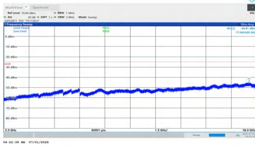
NTVN-n41-PC2-30-35-L-DFT-QPSK-Inner_1RB_Left-3000-18000 -PASS
