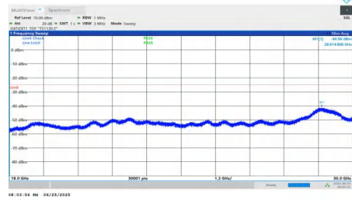
NTNV-n41-PC2-30-30-M-DFT-QPSK-Inner_1RB_Left-18000-3000 0-PASS
