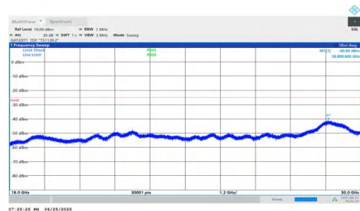
NTNV-n41-PC2-30-20-M-DFT-BPSK-Inner_1RB_Left-18000-30000-PASS
