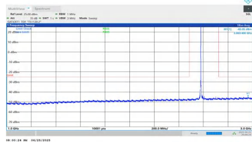
NTNV-n41-PC2-30-30-M-DFT-BPSK-Inner_1RB_Left-1000-3000-PASS
