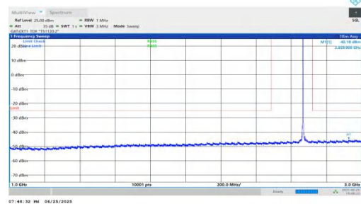
NTNV-n41-PC2-30-25-H-DFT-BPSK-Inner_1RB_Left-1000-3000-PASS
