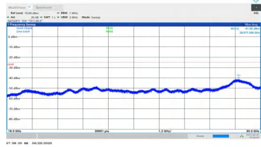
NTVN-n41-PC2-30-30-L-DFT-QPSK-Inner_1RB_Left-18000-3000 0-PASS
