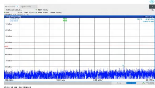
NTNV-n41-PC2-30-25-L-DFT-QPSK-Inner_1RB_Left-0.15-30-PASS
