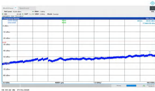
NTVN-n41-PC2-30-20-H-DFT-BPSK-Inner_1RB_Right-3000-180 00-PASS
