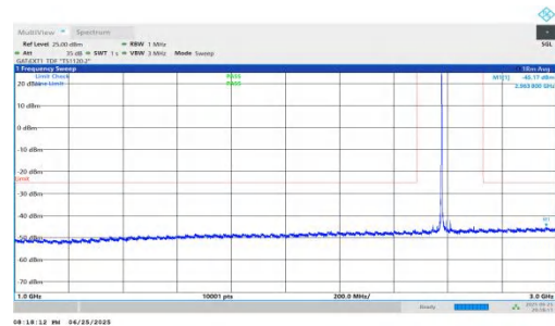
NTNV-n41-PC2-30-35-M-DFT-BPSK-Inner_1RB_Left-1000-3000-PASS
