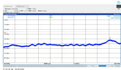
NTVN-n41-PC2-30-25-H-DFT-BPSK-Inner_1RB_Right-18000-300 00-PASS
