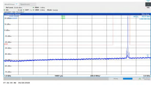
NTVN-n41-PC2-30-20-H-DFT-BPSK-Inner_1RB_Right-1000-3000 -PASS
