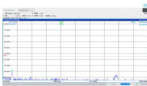
NTNV-n41-PC2-30-30-H-DFT-BPSK-Inner_1RB_Right-0.009-0.15-PASS 5-PASS
