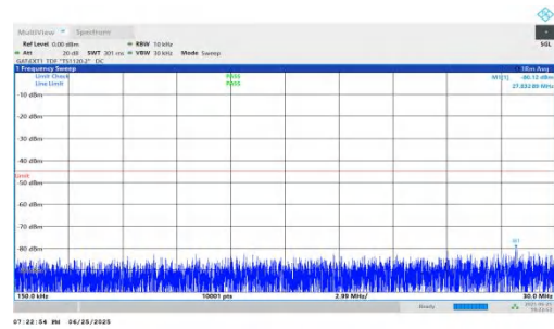
NTVN-n41-PC2-30-20-L-DFT-QPSK-Inner_1RB_Right-0.15-30-PA SS
