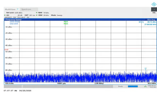
NTNV-n41-PC2-30-30-L-DFT-QPSK-Inner_1RB_Left-0.15-30-PAS S
