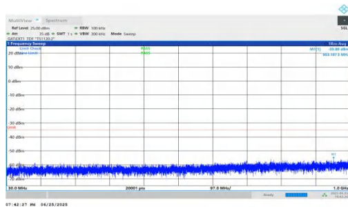
NTNV-n41-PC2-30-25-M-DFT-BPSK-Inner_1RB_Left-30-1000-PASS
