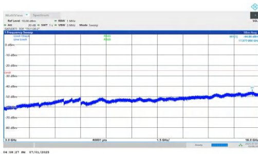
NTNV-n41-PC2-30-20-M-DFT-QPSK-Inner_1RB_Right-3000-18000- 00-PASS
