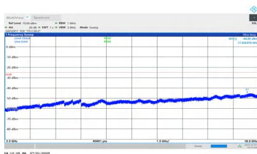
NTVN-n41-PC2-30-25-L-DFT-QPSK-Inner_1RB_Right-3000-18000 00-PASS
