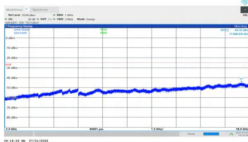
NTNV-n41-PC2-30-25-H-DFT-BPSK-Inner_1RB_Left-3000-18000-PASS
