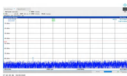
NTNV-n41-PC2-30-25-M-DFT-BPSK-Inner_1RB_Right-0.15-30-PASS
