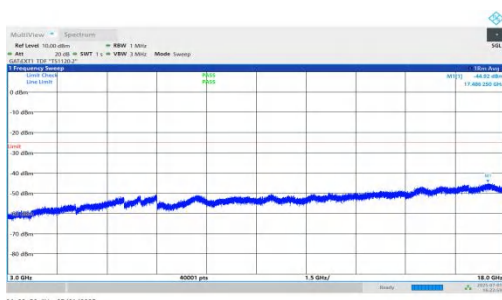
NTVN-n41-PC2-30-35-L-DFT-QPSK-Inner_1RB_Right-3000-18000 00-PASS
