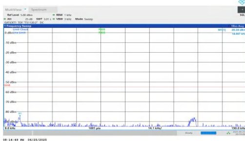
NTNV-n41-PC2-30-35-L-DFT-QPSK-Inner_1RB_Left-0.009-0.15-PASS
