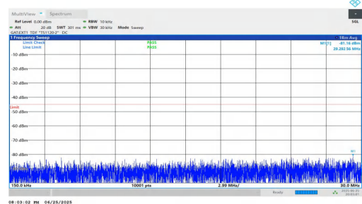
NTNV-n41-PC2-30-30-M-DFT-QPSK-Inner_1RB_Left-0.15-30-PASS
