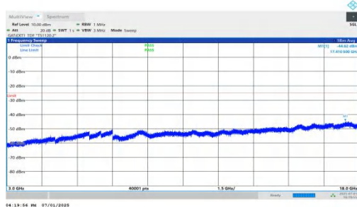
NTNV-n41-PC2-30-30-H-DFT-BPSK-Inner_1RB_Left-3000-18000-PASS 0-PASS
