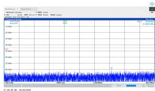
NTNV-n41-PC2-30-20-M-DFT-QPSK-Inner_1RB_Right-0.15-30-P ASS
