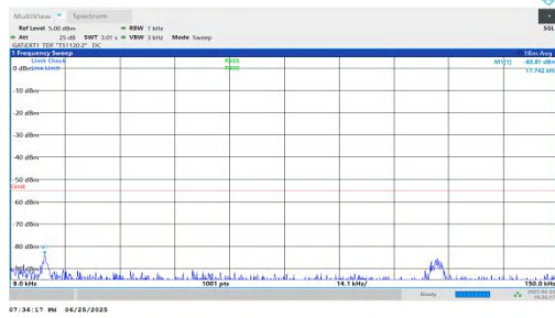
NTNV-n41-PC2-30-25-L-DFT-BPSK-Inner_1RB_Left-0.009-0.15- PASS
