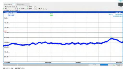
NTNV-n41-PC2-30-35-L-DFT-BPSK-Inner_1RB_Right-18000-30000-PASS
