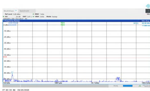
NTNV-n41-PC2-30-25-M-DFT-BPSK-Inner_1RB_Right-0.009-0.15-5-PASS
