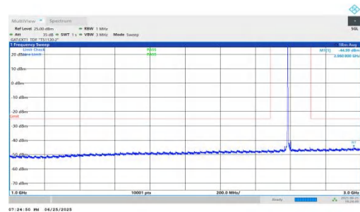
NTNV-n41-PC2-30-20-M-DFT-BPSK-Inner_1RB_Left-1000-3000-PASS
