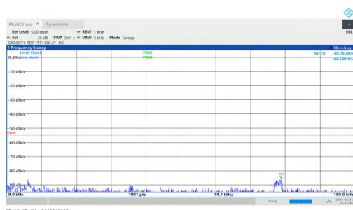
NTNV-n41-PC2-30-20-M-DFT-BPSK-Inner_1RB_Right-0.009-0.15-PASS
