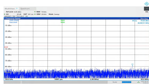
NTNV-n41-PC2-30-25-H-DFT-BPSK-Inner_1RB_Right-0.15-30-PASS
