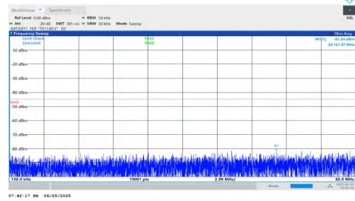
NTNV-n41-PC2-30-25-M-DFT-BPSK-Inner_1RB_Left-0.15-30-PASS
