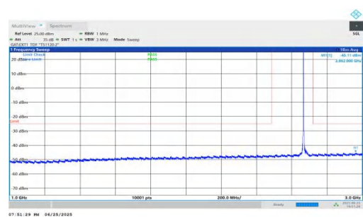
NTVN-n41-PC2-30-25-H-DFT-QPSK-Inner_1RB_Left-1000-3000- PASS
