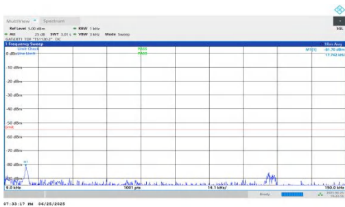
NTVN-n41-PC2-30-20-H-DFT-QPSK-Inner_1RB_Left-0.009-0.15- PASS
