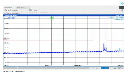
NTNV-n41-PC2-30-25-H-DFT-QPSK-Inner_1RB_Right-1000-3000-PASS
