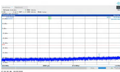
NTNV-n41-PC2-30-25-H-DFT-QPSK-Inner_1RB_Right-30-1000-PASS
