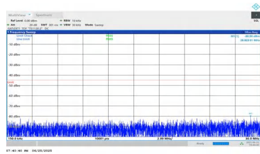
NTVN-n41-PC2-30-25-L-DFT-QPSK-Inner_1RB_Right-0.15-30-PA SS
