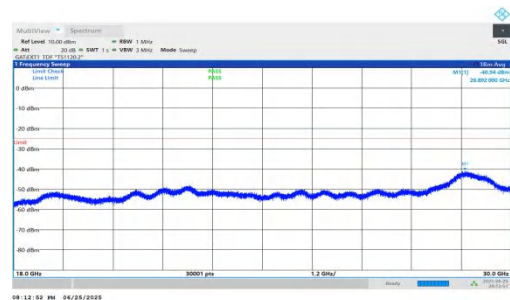
NTNV-n41-PC2-30-35-L-DFT-BPSK-Inner_1RB_Left-18000-30000-PASS
