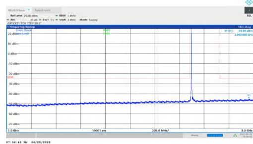
NTNV-n41-PC2-30-25-L-DFT-BPSK-Inner_1RB_Left-1000-3000-P ASS
