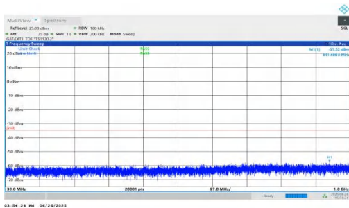
NTNV-n38-PC3-30-10-H-DFT-BPSK-Inner_1RB_Left-30-1000-PASS
