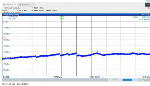
NTNV-n38-PC3-30-20-L-DFT-BPSK-Inner_1RB_Right-3000-12000-PASS
