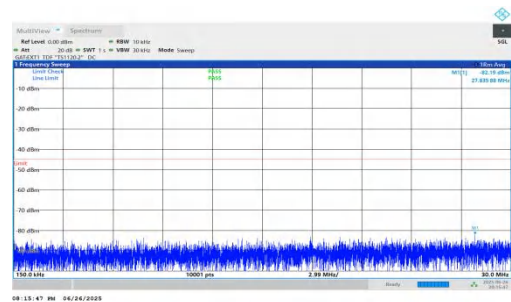
NTNV-n38-PC3-30-25-H-DFT-QPSK-Inner_1RB_Left-0.15-30-PAS S
