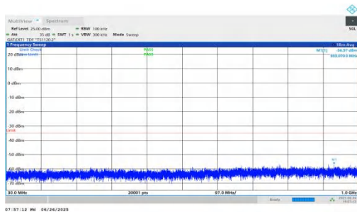
NTNV-n38-PC3-30-25-L-DFT-BPSK-Inner_1RB_Left-30-1000-PA SS
