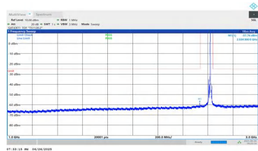
NTNV-n38-PC3-30-15-H-DFT-QPSK-Inner_1RB_Right-1000-3000 -PASS
