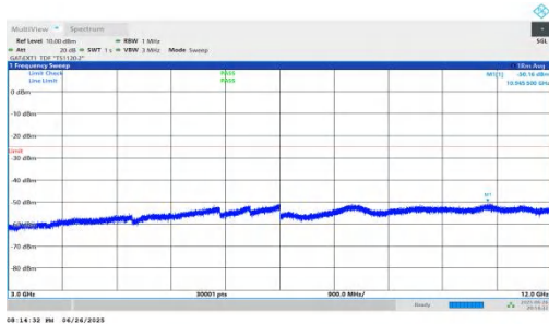
NTNV-n38-PC3-30-25-H-DFT-BPSK-Inner_1RB_Right-3000-120 00-PASS
