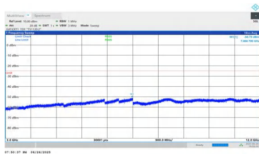
NTNV-n38-PC3-30-20-H-DFT-BPSK-Inner_1RB_Left-3000-12000-PASS
