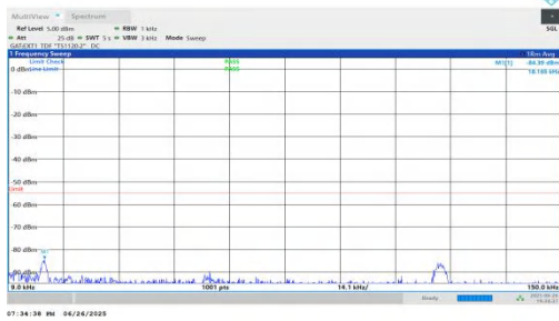
NTNV-n38-PC3-30-20-L-DFT-BPSK-Inner_1RB_Left-0.009-0.15-PASS
