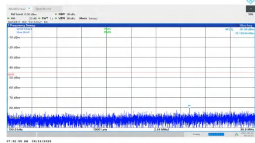
NTNV-n38-PC3-30-15-H-DFT-QPSK-Inner_1RB_Right-0.15-30-PA SS
