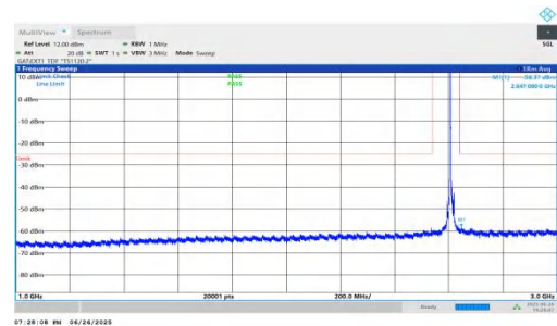
NTNV-n38-PC3-30-15-H-DFT-BPSK-Inner_1RB_Left-1000-3000-PASS
