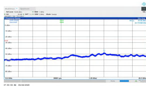
NTNV-n38-PC3-30-20-H-DFT-BPSK-Inner_1RB_Left-12000-26500-PASS
