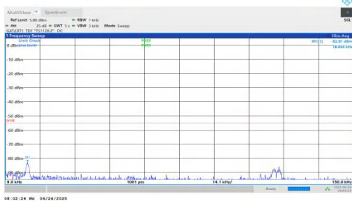
NTNV-n38-PC3-30-25-L-DFT-QPSK-Inner_1RB_Right-0.009-0.1 5-PASS
