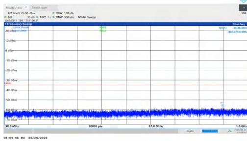
NTNV-n38-PC3-30-25-M-DFT-BPSK-Inner_1RB_Left-30-1000-PASS
