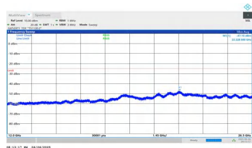
NTNV-n38-PC3-30-25-H-DFT-BPSK-Inner_1RB_Left-12000-26500-PASS
