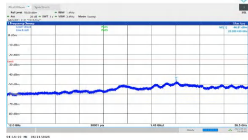
NTNV-n38-PC3-30-15-M-DFT-QPSK-Inner_1RB_Left-12000-2650 0-PASS
