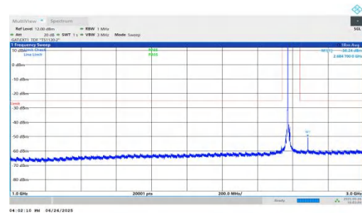
NTNV-n38-PC3-30-15-L-DFT-BPSK-Inner_1RB_Left-1000-3000-PASS
