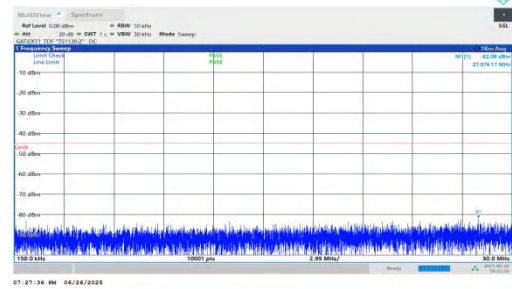
NTNV-n38-PC3-30-15-H-DFT-BPSK-Inner_1RB_Left-0.15-30-PAS
