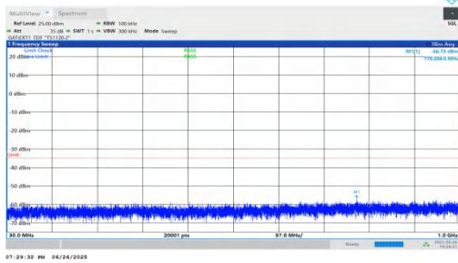
NTNV-n38-PC3-30-15-H-DFT-BPSK-Inner_1RB_Right-30-1000-P ASS
