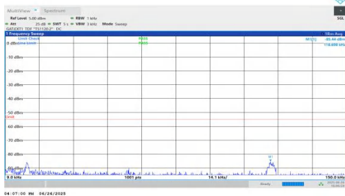
NTNV-n38-PC3-30-15-L-DFT-QPSK-Inner_1RB_Right-0.009-0.1 5-PASS
