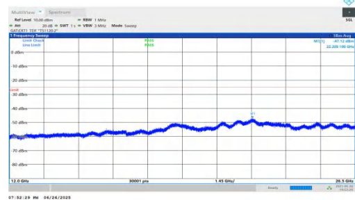
NTNV-n38-PC3-30-20-H-DFT-BPSK-Inner_1RB_Right-12000-26500-PASS
