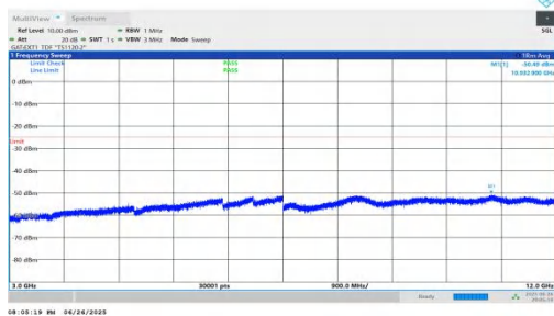
NTNV-n38-PC3-30-25-M-DFT-BPSK-Inner_1RB_Left-3000-12000-PASS
