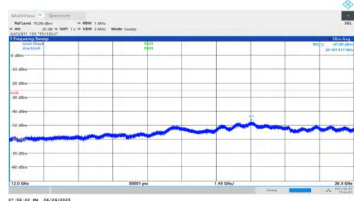
NTNV-n38-PC3-30-20-H-DFT-QPSK-Inner_1RB_Right-12000-265 00-PASS
