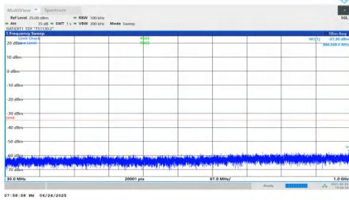
NTNV-n38-PC3-30-25-L-DFT-BPSK-Inner_1RB_Right-30-1000-P ASS
