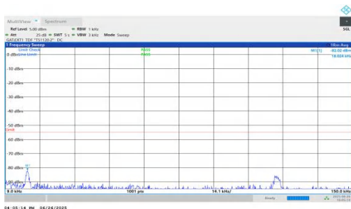
NTNV-n38-PC3-30-15-L-DFT-QPSK-Inner_1RB_Left-0.009-0.15- PASS
