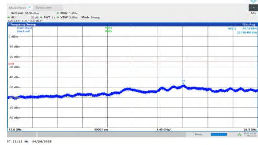
NTNV-n38-PC3-30-15-H-DFT-QPSK-Inner_1RB_Left-12000-2650 0-PASS
