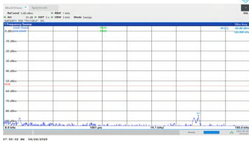
NTNV-n38-PC3-30-20-H-DFT-QPSK-Inner_1RB_Right-0.009-0.1 5-PASS
