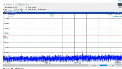
NTNV-n38-PC3-30-20-H-DFT-QPSK-Inner_1RB_Left-0.15-30-PASS
