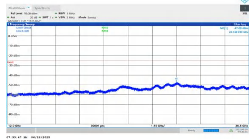
NTNV-n38-PC3-30-15-H-DFT-QPSK-Inner_1RB_Right-12000-265 00-PASS
