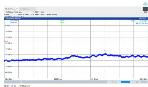
NTNV-n38-PC3-30-30-L-DFT-BPSK-Inner_1RB_Left-12000-26500-PASS
