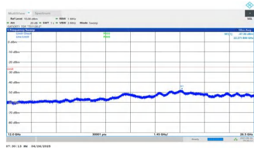
NTNV-n38-PC3-30-15-H-DFT-BPSK-Inner_1RB_Right-12000-26500-PASS
