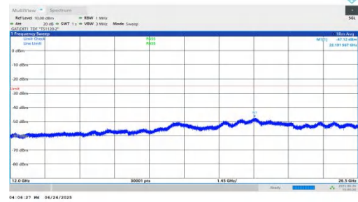
NTNV-n38-PC3-30-15-L-DFT-QPSK-Inner_1RB_Left-12000-2650 0-PASS
