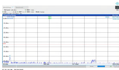
NTNV-n38-PC3-30-20-H-DFT-BPSK-Inner_1RB_Right-0.009-0.15-PASS
