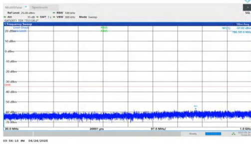
NTNV-n38-PC3-30-10-H-DFT-BPSK-Inner_1RB_Right-30-1000-P ASS
