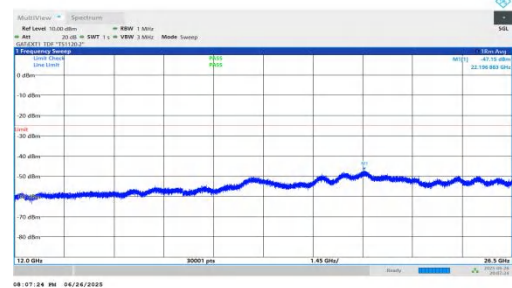
NTNV-n38-PC3-30-25-M-DFT-BPSK-Inner_1RB_Right-12000-26500-PASS
