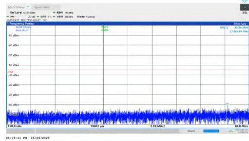
NTNV-n38-PC3-30-15-M-DFT-BPSK-Inner_1RB_Left-0.15-30-PASS
