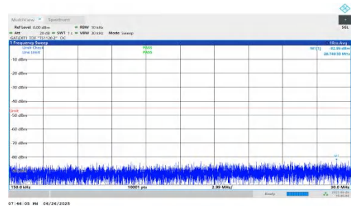
NTNV-n38-PC3-30-20-M-DFT-QPSK-Inner_1RB_Left-0.15-30-PASS
