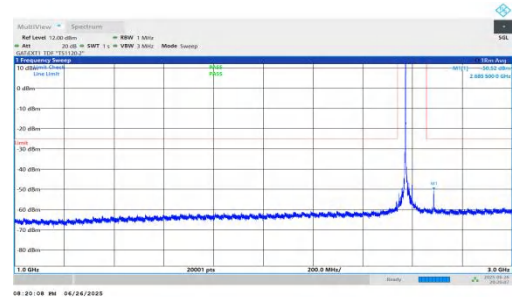
NTNV-n38-PC3-30-30-L-DFT-BPSK-Inner_1RB_Left-1000-3000-PASS
