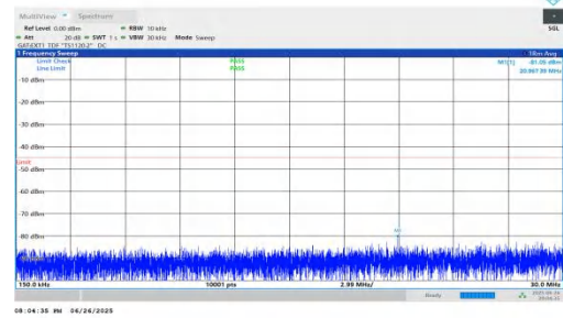
NTNV-n38-PC3-30-25-M-DFT-BPSK-Inner_1RB_Left-0.15-30-PASS
