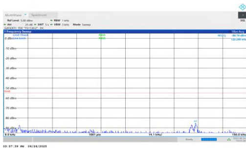
NTNV-n38-PC3-30-10-H-DFT-QPSK-Inner_1RB_Left-0.009-0.15-PASS
