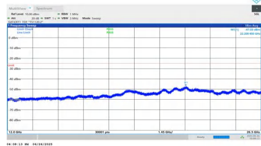
NTNV-n38-PC3-30-15-L-DFT-QPSK-Inner_1RB_Right-12000-265 00-PASS
