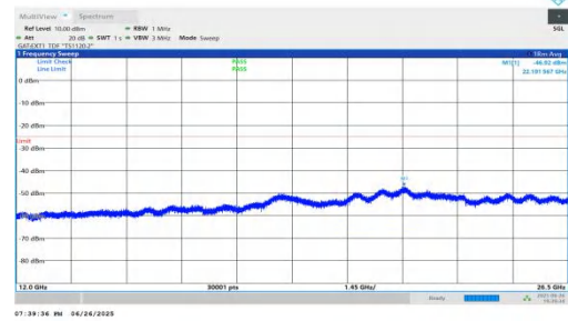
NTNV-n38-PC3-30-20-L-DFT-QPSK-Inner_1RB_Left-12000-2650 0-PASS
