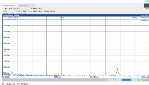
NTNV-n38-PC3-30-25-M-DFT-BPSK-Inner_1RB_Right-0.009-0.15-PASS
