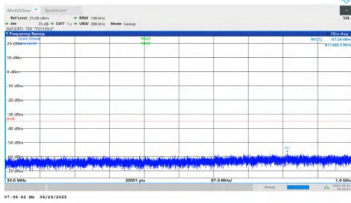
NTNV-n38-PC3-30-20-L-DFT-BPSK-Inner_1RB_Right-30-1000-P ASS
