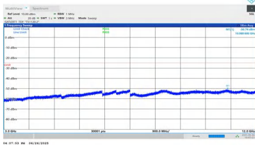
NTNV-n38-PC3-30-15-L-DFT-QPSK-Inner_1RB_Right-3000-120 00-PASS
