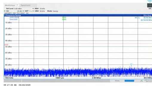
NTNV-n38-PC3-30-25-H-DFT-QPSK-Inner_1RB_Right-0.15-30-PA SS
