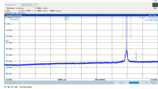
NTNV-n38-PC3-30-20-M-DFT-BPSK-Inner_1RB_Left-1000-3000-PASS
