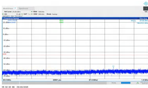
NTNV-n38-PC3-30-25-L-DFT-QPSK-Inner_1RB_Right-30-1000-P ASS
