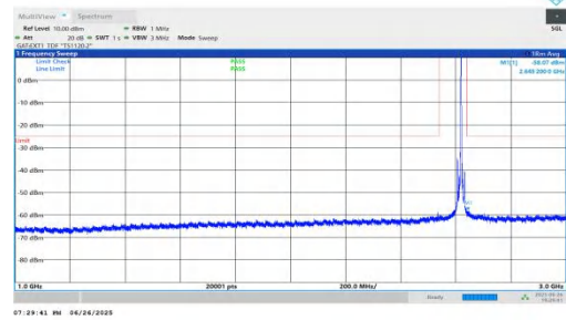
NTNV-n38-PC3-30-15-H-DFT-BPSK-Inner_1RB_Right-1000-3000-PASS
