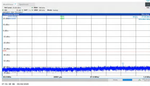
NTNV-n38-PC3-30-20-H-DFT-BPSK-Inner_1RB_Right-30-1000-P ASS
