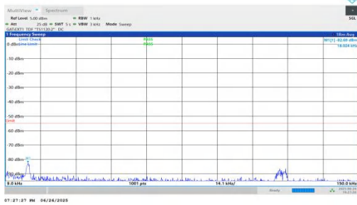
NTNV-n38-PC3-30-15-H-DFT-BPSK-Inner_1RB_Left-0.009-0.15-PASS
