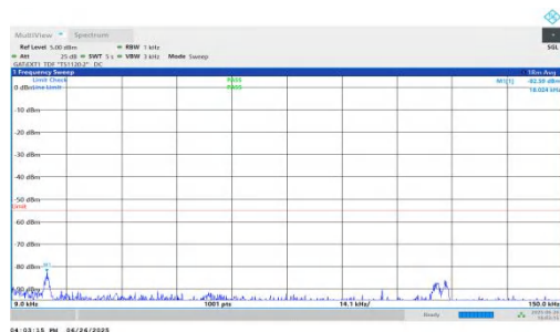
NTNV-n38-PC3-30-15-L-DFT-BPSK-Inner_1RB_Right-0.009-0.15-PASS
