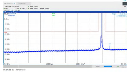
NTNV-n38-PC3-30-20-L-DFT-BPSK-Inner_1RB_Right-1000-3000-PASS
