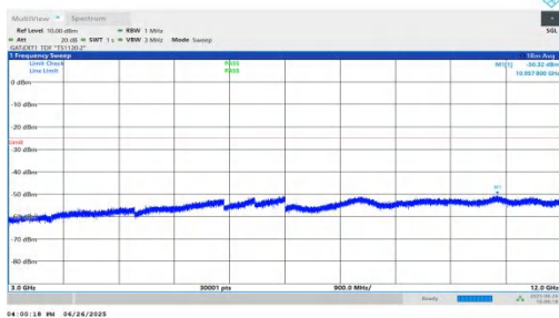
NTNV-n38-PC3-30-10-H-DFT-QPSK-Inner_1RB_Right-3000-120 00-PASS
