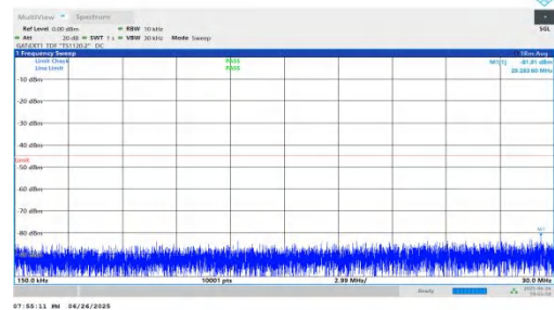
NTNV-n38-PC3-30-20-H-DFT-QPSK-Inner_1RB_Right-0.15-30-PA SS
