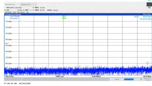
NTNV-n38-PC3-30-20-M-DFT-BPSK-Inner_1RB_Left-0.15-30-PASS
