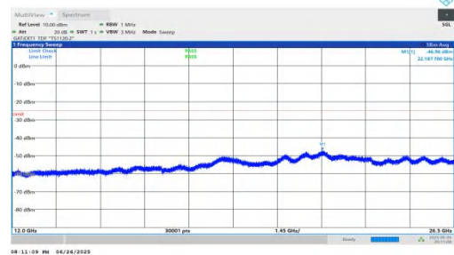
NTNV-n38-PC3-30-25-M-DFT-QPSK-Inner_1RB_Right-12000-26500- 00-PASS
