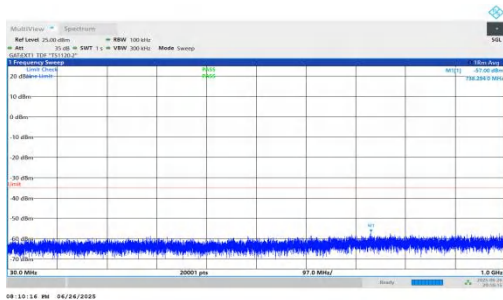
NTNV-n38-PC3-30-25-M-DFT-QPSK-Inner_1RB_Right-30-1000- PASS
