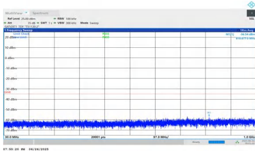
NTNV-n38-PC3-30-20-H-DFT-QPSK-Inner_1RB_Right-30-1000- PASS
