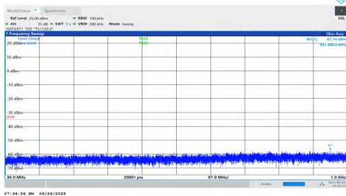
NTNV-n38-PC3-30-20-L-DFT-BPSK-Inner_1RB_Left-30-1000-PASS
