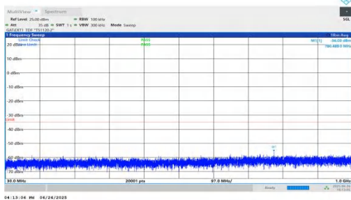
NTNV-n38-PC3-30-15-M-DFT-QPSK-Inner_1RB_Left-30-1000-PASS
