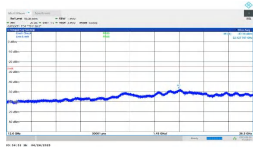
NTNV-n38-PC3-30-10-H-DFT-BPSK-Inner_1RB_Right-12000-26500-PASS
