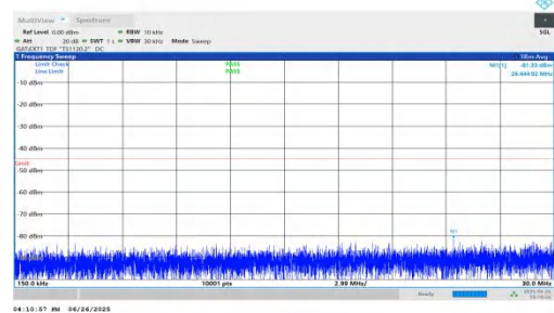
NTNV-n38-PC3-30-15-M-DFT-BPSK-Inner_1RB_Right-0.15-30-PASS
