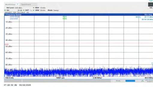
NTNV-n38-PC3-30-20-H-DFT-BPSK-Inner_1RB_Left-0.15-30-PAS
