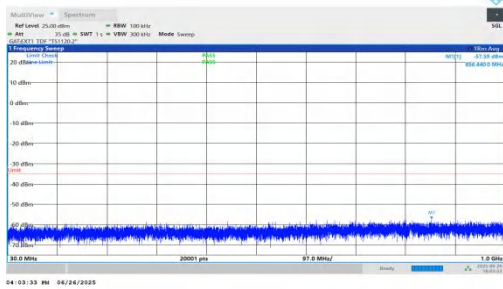
NTNV-n38-PC3-30-15-L-DFT-BPSK-Inner_1RB_Right-30-1000-P ASS
