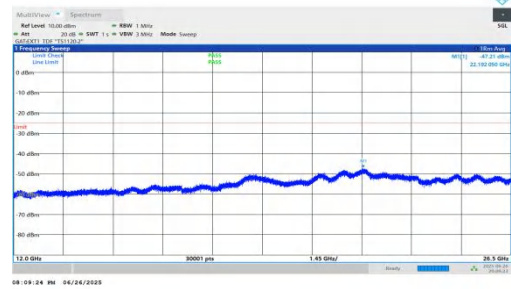
NTNV-n38-PC3-30-25-M-DFT-QPSK-Inner_1RB_Left-12000-2650 0-PASS
