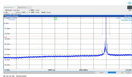
NTNV-n38-PC3-30-25-L-DFT-QPSK-Inner_1RB_Right-1000-3000- PASS
