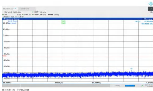
NTNV-n38-PC3-30-10-H-DFT-QPSK-Inner_1RB_Right-30-1000- PASS
