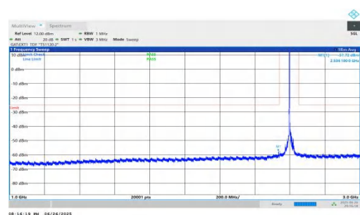
NTNV-n38-PC3-30-25-H-DFT-QPSK-Inner_1RB_Left-1000-3000- PASS
