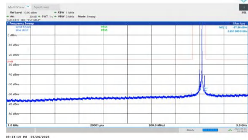
NTNV-n38-PC3-30-25-H-DFT-BPSK-Inner_1RB_Right-1000-3000-P PASS
