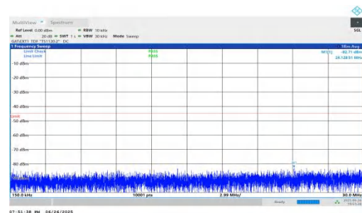
NTNV-n38-PC3-30-20-H-DFT-BPSK-Inner_1RB_Right-0.15-30-PASS
