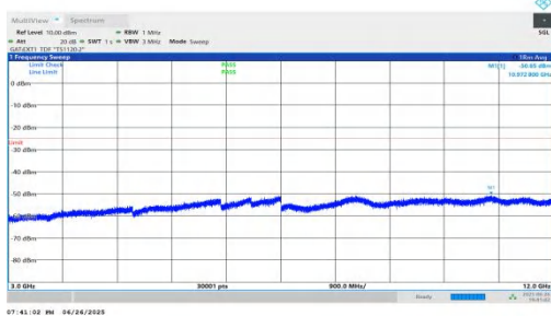
NTNV-n38-PC3-30-20-L-DFT-QPSK-Inner_1RB_Right-3000-120 00-PASS
