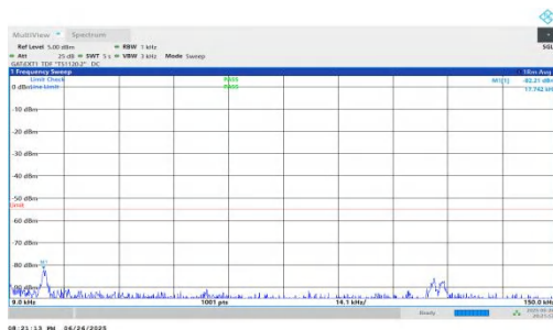
NTNV-n38-PC3-30-30-L-DFT-BPSK-Inner_1RB_Right-0.009-0.15-PASS
