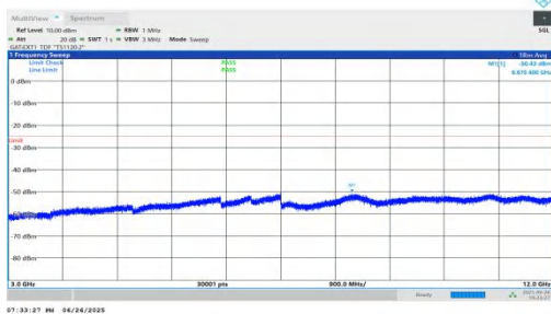
NTNV-n38-PC3-30-15-H-DFT-QPSK-Inner_1RB_Right-3000-120 00-PASS
