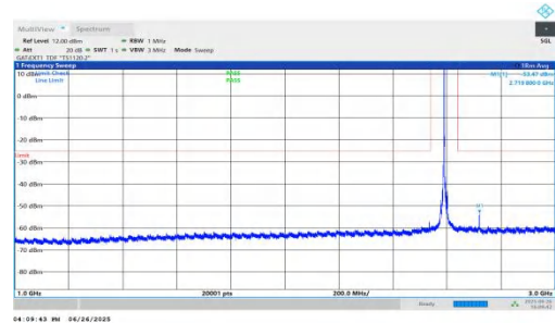
NTNV-n38-PC3-30-15-M-DFT-BPSK-Inner_1RB_Left-1000-3000-PASS
