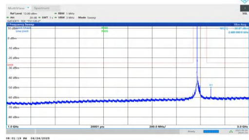
NTNV-n38-PC3-30-25-L-DFT-QPSK-Inner_1RB_Left-1000-3000-P ASS
