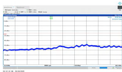
NTNV-n38-PC3-30-15-M-DFT-BPSK-Inner_1RB_Left-12000-26500-PASS
