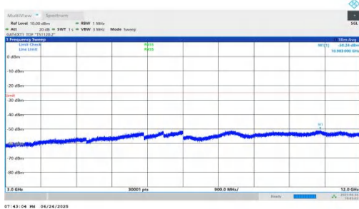
NTNV-n38-PC3-30-20-M-DFT-BPSK-Inner_1RB_Left-3000-12000-PASS
