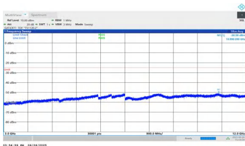
NTNV-n38-PC3-30-10-H-DFT-BPSK-Inner_1RB_Left-3000-12000-PASS
