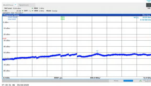
NTNV-n38-PC3-30-20-L-DFT-BPSK-Inner_1RB_Left-3000-12000-PASS
