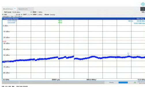
NTNV-n38-PC3-30-25-H-DFT-BPSK-Inner_1RB_Left-3000-12000-PASS
