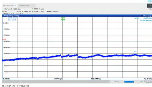
NTNV-n38-PC3-30-25-H-DFT-QPSK-Inner_1RB_Right-3000-12000-PASS
