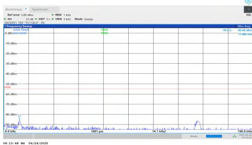
NTNV-n38-PC3-30-15-M-DFT-BPSK-Inner_1RB_Right-0.009-0.15-PASS
