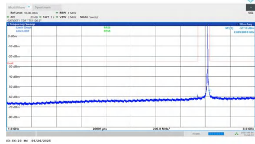
NTNV-n38-PC3-30-10-H-DFT-BPSK-Inner_1RB_Right-1000-3000-PASS
