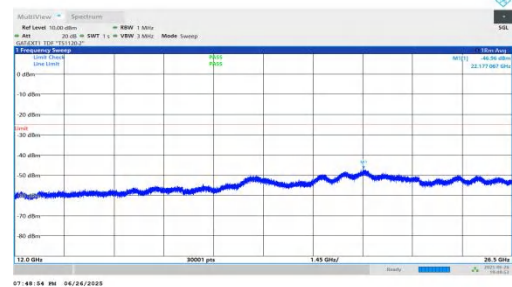
NTNV-n38-PC3-30-20-M-DFT-QPSK-Inner_1RB_Right-12000-26500- 00-PASS
