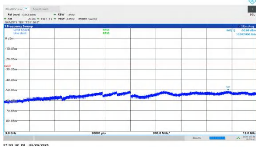
NTNV-n38-PC3-30-25-L-DFT-BPSK-Inner_1RB_Right-3000-1200 0-PASS
