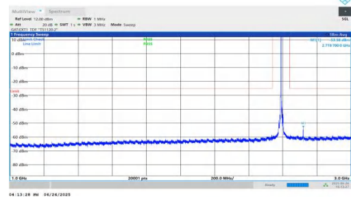
NTNV-n38-PC3-30-15-M-DFT-QPSK-Inner_1RB_Left-1000-3000-PASS
