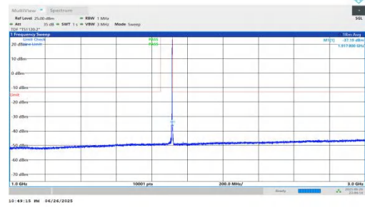
NTNV-n25-PC3-15-20-H-DFT-BPSK-Inner_1RB_Right-1000-3000-PASS
