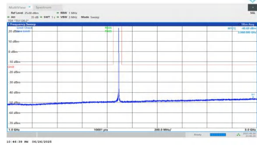
NTNV-n25-PC3-15-20-M-DFT-BPSK-Inner_1RB_Right-1000-3000-PASS
