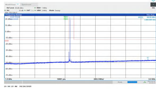
NTNV-n25-PC3-15-15-L-DFT-BPSK-Inner_1RB_Right-1000-3000-PASS
