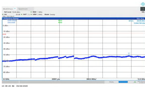
NTNV-n25-PC3-15-15-M-DFT-BPSK-Inner_1RB_Left-3000-12000-PASS
