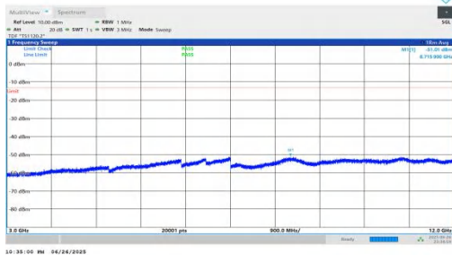
NTNV-n25-PC3-15-10-H-DFT-QPSK-Inner_1RB_Right-3000-12000- 00-PASS
