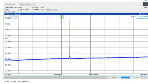
NTNV-n25-PC3-15-10-H-DFT-BPSK-Inner_1RB_Right-1000-3000-PASS
