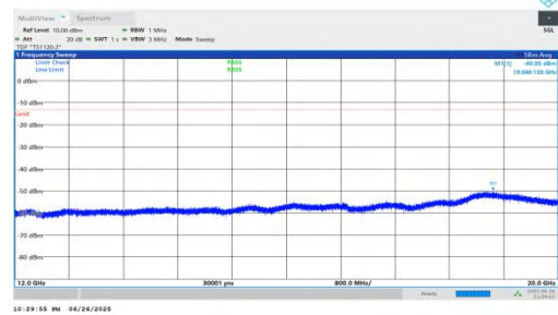
NTVN-n25-PC3-15-10-L-DFT-QPSK-Inner_1RB_Right-12000-2000 00-PASS
