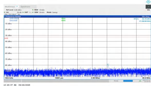
NTVN-n25-PC3-15-5-H-DFT-QPSK-Inner_1RB_Right-0.15-30-PA-SS
