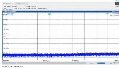
NTNV-n25-PC3-15-10-L-DFT-BPSK-Inner_1RB_Left-30-1000-PASS
