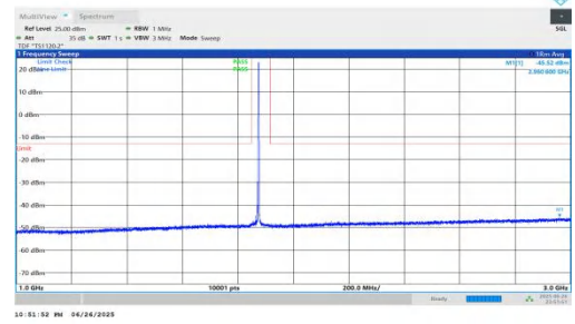
NTNV-n25-PC3-15-25-L-DFT-BPSK-Inner_1RB_Right-1000-3000-P PASS
