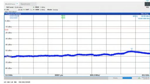
NTNV-n25-PC3-15-20-L-DFT-BPSK-Inner_1RB_Right-12000-200 00-PASS
