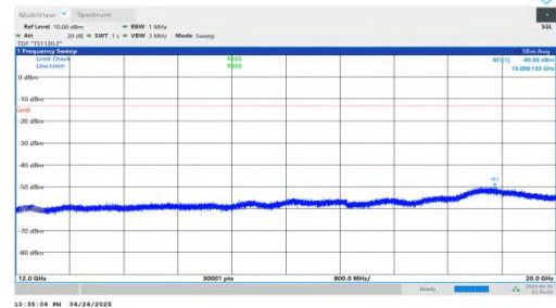
NTNV-n25-PC3-15-10-H-DFT-QPSK-Inner_1RB_Right-12000-20000- 00-PASS
