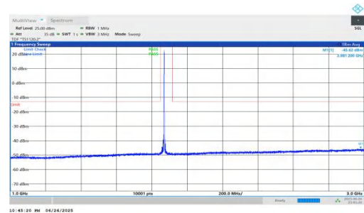
NTNV-n25-PC3-15-20-L-DFT-QPSK-Inner_1RB_Right-1000-3000- PASS
