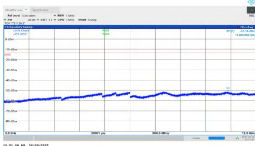
NTNV-n25-PC3-15-25-L-DFT-BPSK-Inner_1RB_Left-3000-12000- -PASS
