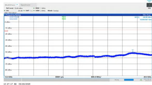
NTVN-n25-PC3-15-5-H-DFT-QPSK-Inner_1RB_Right-12000-20000-PASS
