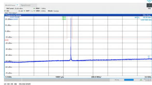
NTNV-n25-PC3-15-15-H-DFT-BPSK-Inner_1RB_Left-1000-3000-PASS
