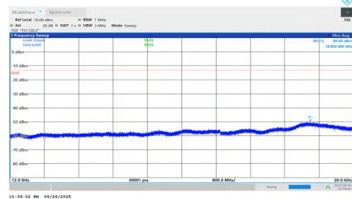
NTNV-n25-PC3-15-15-M-DFT-BPSK-Inner_1RB_Right-12000-20000-PASS
