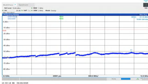
NTNV-n25-PC3-15-25-L-DFT-QPSK-Inner_1RB_Right-3000-12000 00-PASS
