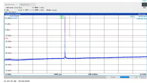
NTNV-n25-PC3-15-20-L-DFT-BPSK-Inner_1RB_Left-1000-3000-PASS
