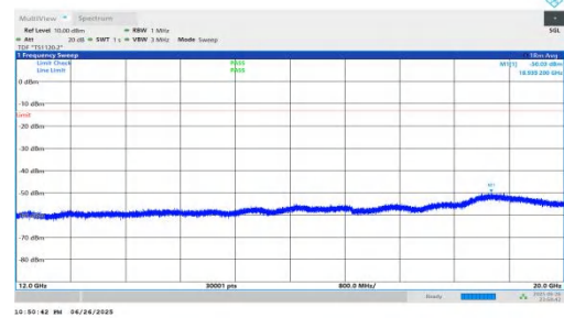
NTNV-n25-PC3-15-20-H-DFT-QPSK-Inner_1RB_Right-12000-20000- 00-PASS
