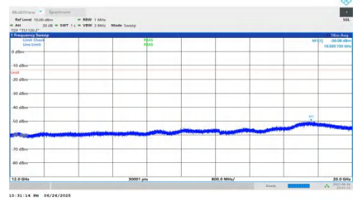
NTNV-n25-PC3-15-10-M-DFT-BPSK-Inner_1RB_Right-12000-20000-PASS
