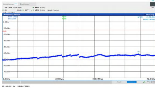
NTNV-n25-PC3-15-15-M-DFT-QPSK-Inner_1RB_Right-3000-120 00-PASS
