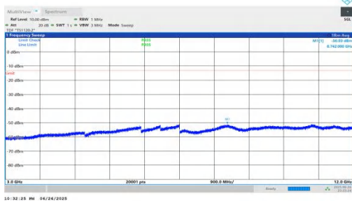
NTNV-n25-PC3-15-10-M-DFT-QPSK-Inner_1RB_Right-3000-12000- 00-PASS
