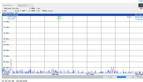
NTNV-n25-PC3-15-10-M-DFT-BPSK-Inner_1RB_Right-0.009-0.15-PASS
