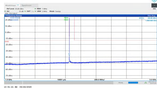
NTNV-n25-PC3-15-25-L-DFT-BPSK-Inner_1RB_Left-1000-3000-PASS ASS
