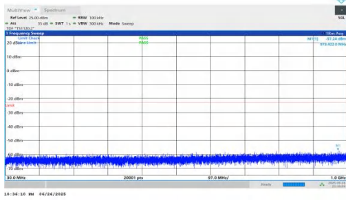
NTNV-n25-PC3-15-15-L-DFT-BPSK-Inner_1RB_Right-30-1000-PASS
