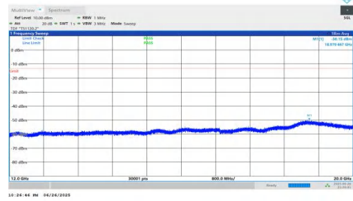
NTVN-n25-PC3-15-5-H-DFT-QPSK-Inner_1RB_Left-12000-20000-PASS
