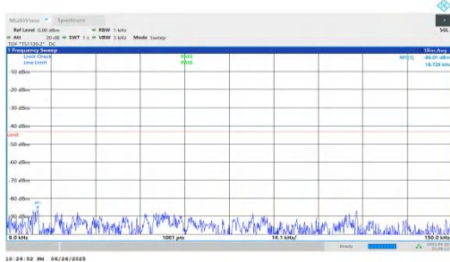
NTVN-n25-PC3-15-5-H-DFT-QPSK-Inner_1RB_Right-0.009-0.15-PASS
