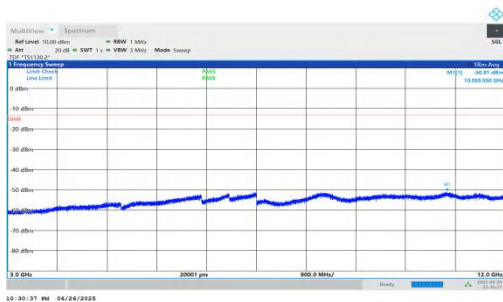
NTNV-n25-PC3-15-10-M-DFT-BPSK-Inner_1RB_Left-3000-12000-PASS
