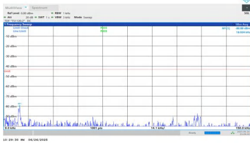
NTVN-n25-PC3-15-10-L-DFT-QPSK-Inner_1RB_Right-0.009-0.1 5-PASS
