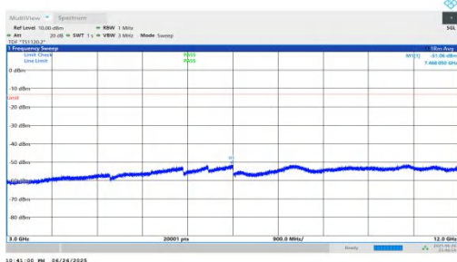
NTNV-n25-PC3-15-15-H-DFT-BPSK-Inner_1RB_Left-3000-12000-PASS
