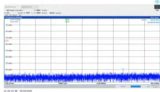
NTNV-n25-PC3-15-10-H-DFT-QPSK-Inner_1RB_Left-0.15-30-PASS
