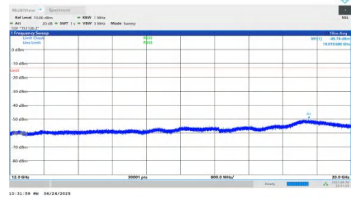
NTNV-n25-PC3-15-10-M-DFT-QPSK-Inner_1RB_Left-12000-2000 0-PASS
