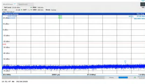
NTNV-n25-PC3-15-25-L-DFT-BPSK-Inner_1RB_Right-30-1000-P ASS
