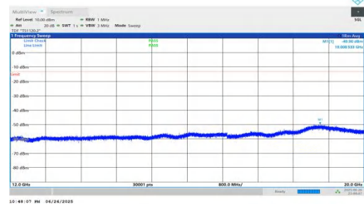
NTNV-n25-PC3-15-20-M-DFT-QPSK-Inner_1RB_Right-12000-20000- 00-PASS
