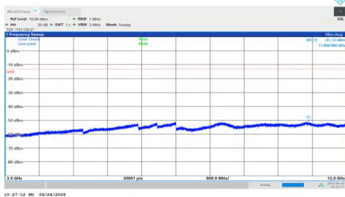
NTVN-n25-PC3-15-5-H-DFT-QPSK-Inner_1RB_Right-3000-12000-PASS
