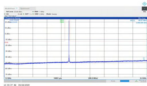
NTNV-n25-PC3-15-10-H-DFT-BPSK-Inner_1RB_Left-1000-3000-PASS
