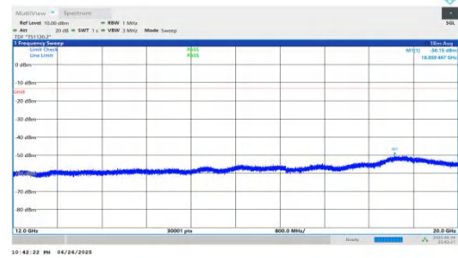
NTNV-n25-PC3-15-15-H-DFT-QPSK-Inner_1RB_Left-12000-2000 0-PASS
