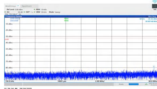
NTNV-n25-PC3-15-15-M-DFT-QPSK-Inner_1RB_Left-0.15-30-PASS
