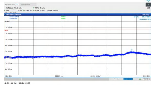
NTNV-n25-PC3-15-10-H-DFT-BPSK-Inner_1RB_Right-12000-20000-PASS
