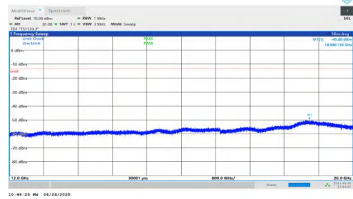
NTNV-n25-PC3-15-20-H-DFT-BPSK-Inner_1RB_Right-12000-20000-PASS
