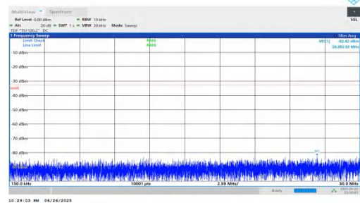
NTNV-n25-PC3-15-10-L-DFT-QPSK-Inner_1RB_Left-0.15-30-PAS S
