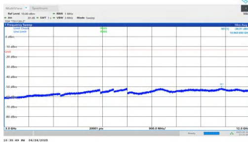
NTNV-n25-PC3-15-15-L-DFT-BPSK-Inner_1RB_Left-3000-12000-PASS
