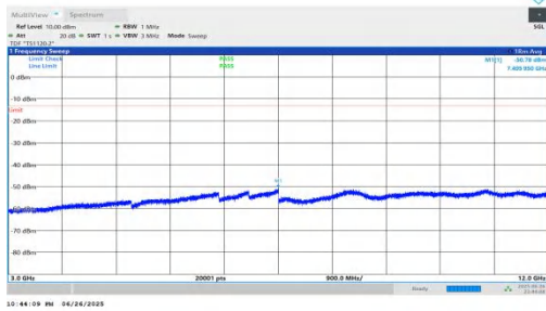
NTNV-n25-PC3-15-20-L-DFT-BPSK-Inner_1RB_Right-3000-1200 0-PASS
