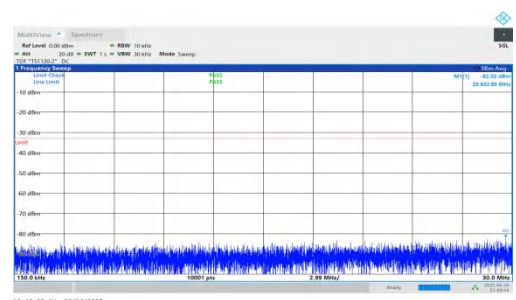
NTNV-n25-PC3-15-20-H-DFT-BPSK-Inner_1RB_Right-0.15-30-PASS
