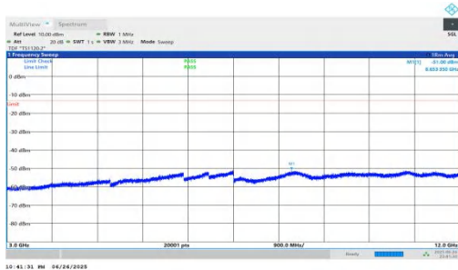
NTNV-n25-PC3-15-15-H-DFT-BPSK-Inner_1RB_Right-3000-120 00-PASS
