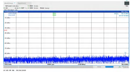
NTNV-n25-PC3-15-20-M-DFT-BPSK-Inner_1RB_Left-0.15-30-PASS
