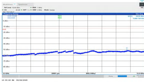
NTNV-n25-PC3-15-10-H-DFT-BPSK-Inner_1RB_Right-3000-12000-PASS
