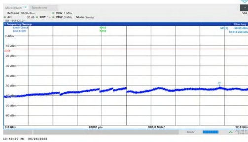
NTNV-n25-PC3-15-20-H-DFT-BPSK-Inner_1RB_Right-3000-12000-PASS
