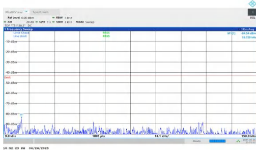
NTNV-n25-PC3-15-25-L-DFT-QPSK-Inner_1RB_Left-0.009-0.15- PASS
