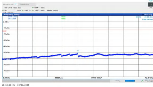
NTNV-n25-PC3-15-25-L-DFT-QPSK-Inner_1RB_Left-3000-12000 -PASS
