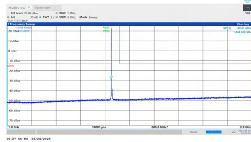
NTNV-n25-PC3-15-10-L-DFT-BPSK-Inner_1RB_Left-1000-3000-PASS
