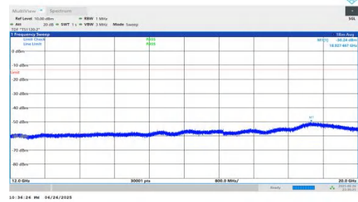
NTNV-n25-PC3-15-15-L-DFT-BPSK-Inner_1RB_Right-12000-20000-PASS
