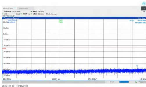
NTNV-n25-PC3-15-15-H-DFT-QPSK-Inner_1RB_Right-30-1000- PASS
