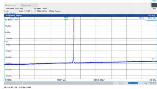
NTNV-n25-PC3-15-10-H-DFT-QPSK-Inner_1RB_Left-1000-3000-PASS
