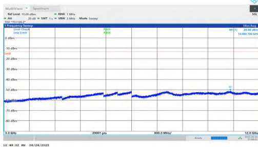
NTNV-n25-PC3-15-20-M-DFT-QPSK-Inner_1RB_Right-3000-12000- 00-PASS
