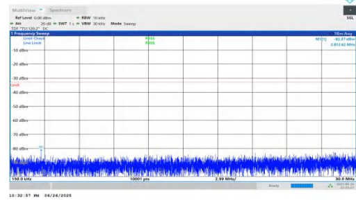
NTNV-n25-PC3-15-10-H-DFT-BPSK-Inner_1RB_Left-0.15-30-PAS
