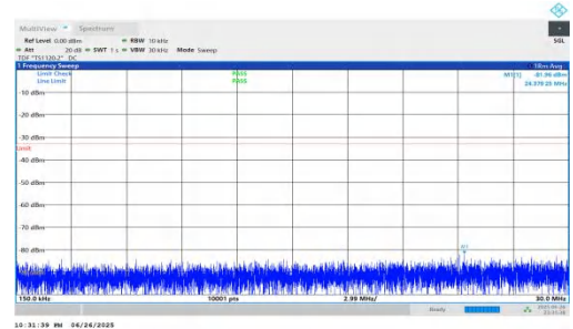
NTNV-n25-PC3-15-10-M-DFT-QPSK-Inner_1RB_Left-0.15-30-PASS
