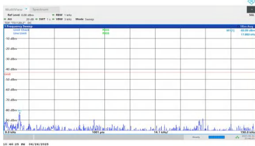
NTNV-n25-PC3-15-20-M-DFT-BPSK-Inner_1RB_Right-0.009-0.15-PASS
