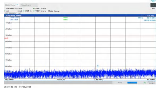
NTNV-n25-PC3-15-15-M-DFT-BPSK-Inner_1RB_Right-0.15-30-PASS
