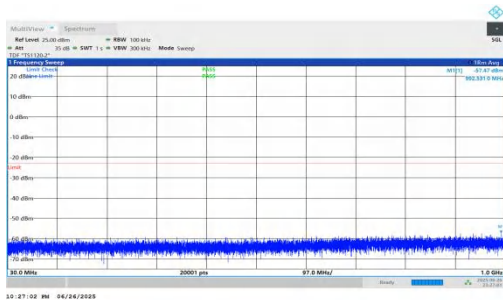
NTVN-n25-PC3-15-5-H-DFT-QPSK-Inner_1RB_Right-30-1000-PASS
