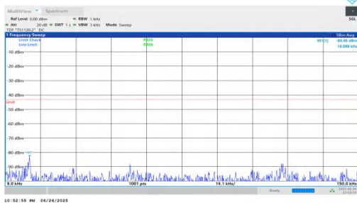
NTNV-n25-PC3-15-25-L-DFT-QPSK-Inner_1RB_Right-0.009-0.1 5-PASS
