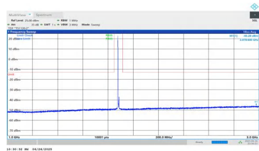
NTNV-n25-PC3-15-10-M-DFT-BPSK-Inner_1RB_Left-1000-3000-PASS
