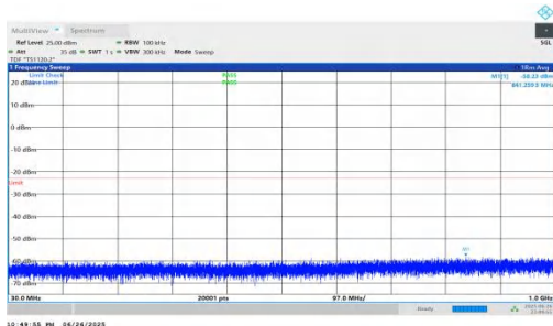
NTNV-n25-PC3-15-20-H-DFT-QPSK-Inner_1RB_Left-30-1000-PASS
