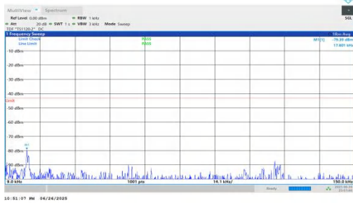
NTNV-n25-PC3-15-25-L-DFT-BPSK-Inner_1RB_Left-0.009-0.15- PASS
