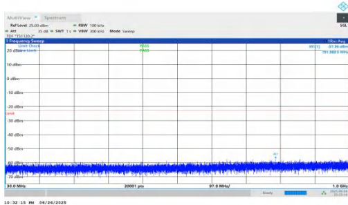
NTNV-n25-PC3-15-10-M-DFT-QPSK-Inner_1RB_Right-30-1000- PASS
