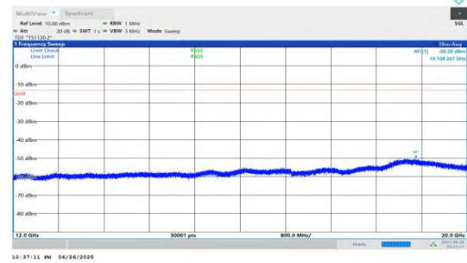
NTNV-n25-PC3-15-15-L-DFT-QPSK-Inner_1RB_Left-12000-2000 0-PASS
