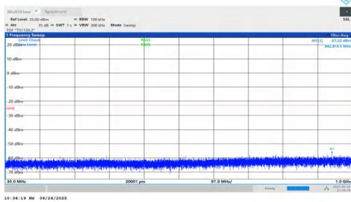
NTNV-n25-PC3-15-10-H-DFT-QPSK-Inner_1RB_Left-30-1000-PASS
