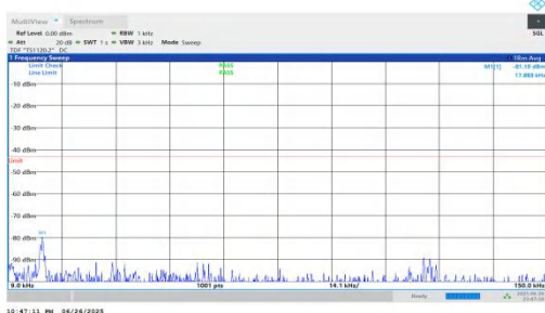
NTNV-n25-PC3-15-20-M-DFT-QPSK-Inner_1RB_Left-0.009-0.15-PASS
