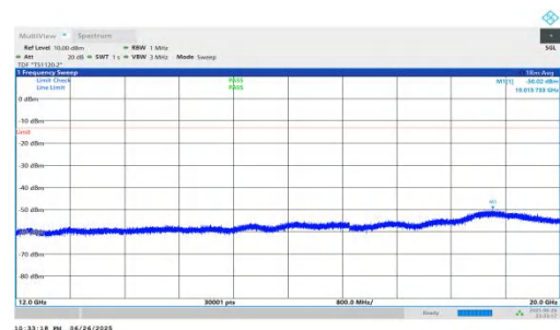
NTNV-n25-PC3-15-10-H-DFT-BPSK-Inner_1RB_Left-12000-20000-PASS
