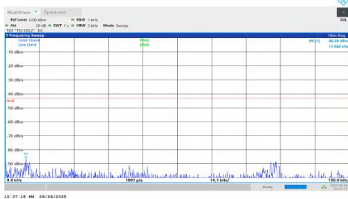
NTNV-n25-PC3-15-15-L-DFT-QPSK-Inner_1RB_Right-0.009-0.1 5-PASS
