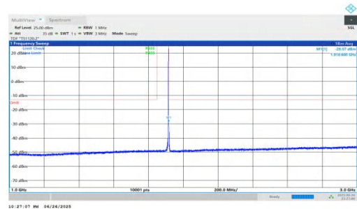
NTVN-n25-PC3-15-5-H-DFT-QPSK-Inner_1RB_Right-1000-3000-PASS
