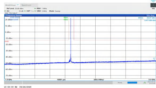
NTNV-n25-PC3-15-25-L-DFT-QPSK-Inner_1RB_Right-1000-3000- PASS
