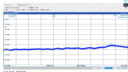
NTNV-n25-PC3-15-25-L-DFT-BPSK-Inner_1RB_Left-12000-20000- -PASS
