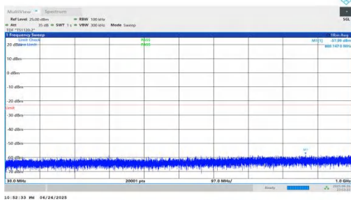
NTNV-n25-PC3-15-25-L-DFT-QPSK-Inner_1RB_Left-30-1000-PA SS
