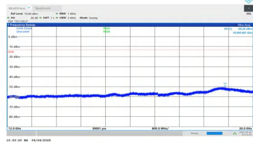
NTNV-n25-PC3-15-25-L-DFT-QPSK-Inner_1RB_Right-12000-20000 00-PASS
