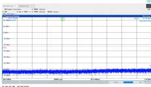
NTNV-n25-PC3-15-10-H-DFT-QPSK-Inner_1RB_Right-30-1000- PASS
