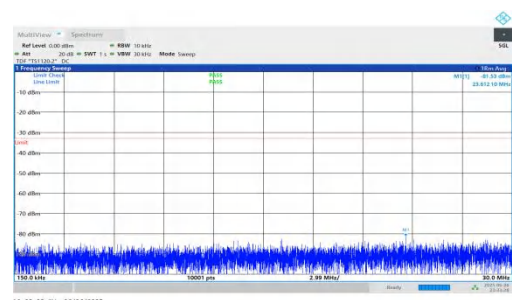
NTNV-n25-PC3-15-10-H-DFT-BPSK-Inner_1RB_Right-0.15-30-PASS
