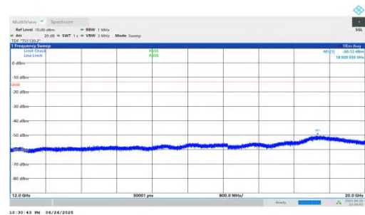
NTNV-n25-PC3-15-10-M-DFT-BPSK-Inner_1RB_Left-12000-20000-PASS
