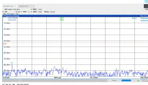
NTNV-n25-PC3-15-15-L-DFT-BPSK-Inner_1RB_Right-0.009-0.15-PASS
