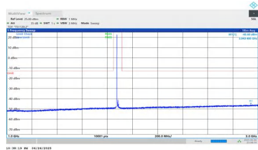
NTNV-n25-PC3-15-15-M-DFT-BPSK-Inner_1RB_Left-1000-3000-PASS
