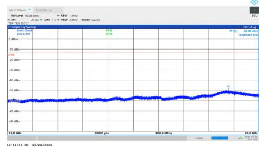
NTNV-n25-PC3-15-15-H-DFT-BPSK-Inner_1RB_Left-12000-20000-PASS
