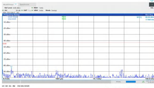
NTNV-n25-PC3-15-15-H-DFT-BPSK-Inner_1RB_Left-0.009-0.15-PASS
