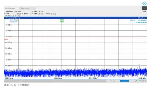
NTNV-n25-PC3-15-15-L-DFT-QPSK-Inner_1RB_Left-0.15-30-PASS
