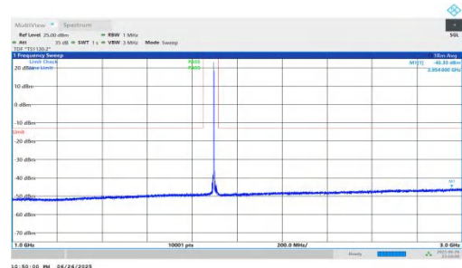
NTNV-n25-PC3-15-20-H-DFT-QPSK-Inner_1RB_Left-1000-3000-PASS
