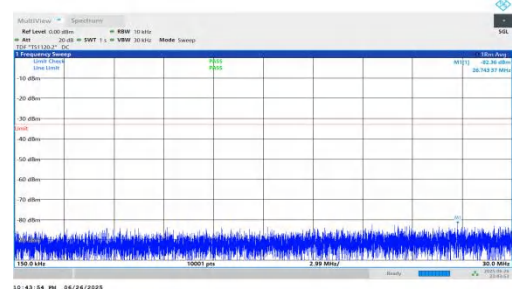
NTNV-n25-PC3-15-20-L-DFT-BPSK-Inner_1RB_Right-0.15-30-PASS
