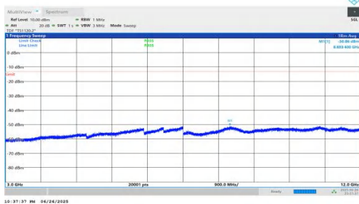
NTNV-n25-PC3-15-15-L-DFT-QPSK-Inner_1RB_Right-3000-12000 00-PASS
