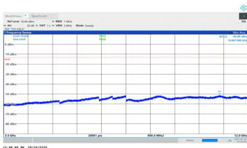
NTNV-n25-PC3-15-20-H-DFT-BPSK-Inner_1RB_Left-3000-12000-PASS
