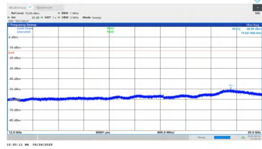
NTNV-n25-PC3-15-20-H-DFT-QPSK-Inner_1RB_Left-12000-2000 0-PASS
