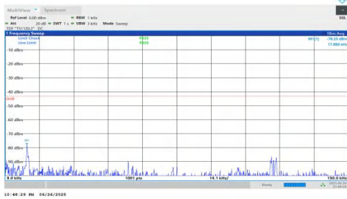
NTNV-n25-PC3-15-20-H-DFT-BPSK-Inner_1RB_Left-0.009-0.15-PASS
