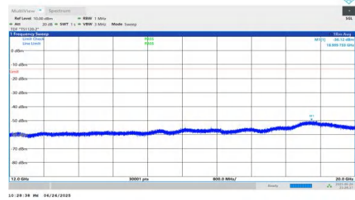
NTNV-n25-PC3-15-10-L-DFT-BPSK-Inner_1RB_Right-12000-200 00-PASS
