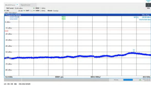
NTNV-n25-PC3-15-15-L-DFT-BPSK-Inner_1RB_Left-12000-20000-PASS
