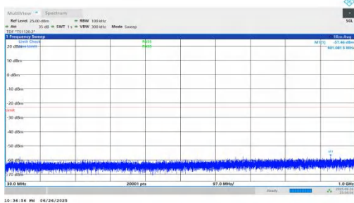
NTNV-n25-PC3-15-15-L-DFT-QPSK-Inner_1RB_Left-30-1000-PASS
