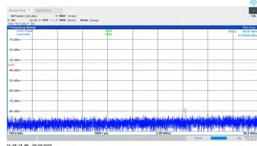
NTNV-n25-PC3-15-10-L-DFT-BPSK-Inner_1RB_Right-0.15-30-PASS
