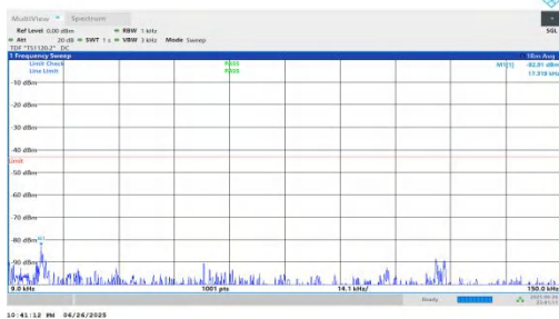
NTNV-n25-PC3-15-15-H-DFT-BPSK-Inner_1RB_Right-0.009-0.15-PASS
