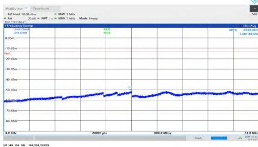
NTNV-n25-PC3-15-20-L-DFT-QPSK-Inner_1RB_Right-3000-120 00-PASS
