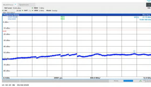
NTNV-n25-PC3-15-15-L-DFT-BPSK-Inner_1RB_Right-3000-12000-PASS
