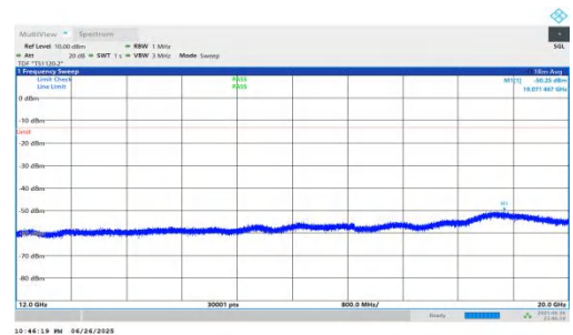
NTNV-n25-PC3-15-20-M-DFT-BPSK-Inner_1RB_Left-12000-20000-PASS
