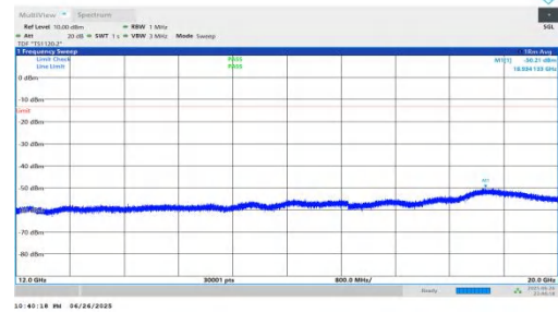
NTNV-n25-PC3-15-15-M-DFT-QPSK-Inner_1RB_Right-12000-200 00-PASS
