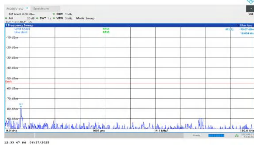
NTNV-n7-PC3-15-30-L-DFT-QPSK-Inner_1RB_Left-0.009-0.15-P ASS
