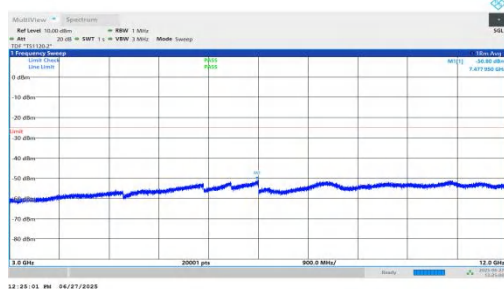
NTNV-n7-PC3-15-25-L-DFT-BPSK-Inner_1RB_Left-3000-12000-PASS
