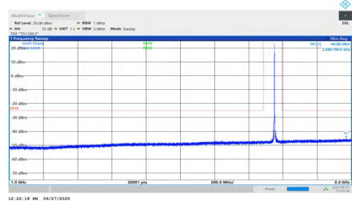
NTNV-n7-PC3-15-20-H-DFT-BPSK-Inner_1RB_Left-1000-3000-P ASS
