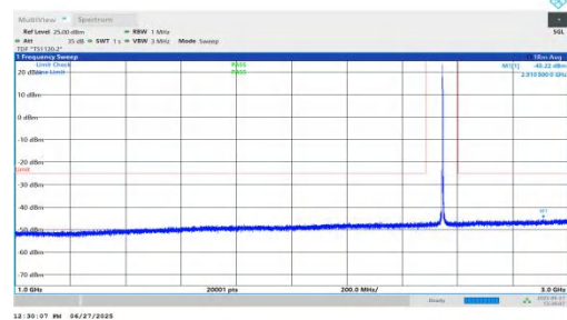
NTNV-n7-PC3-15-25-H-DFT-BPSK-Inner_1RB_Left-1000-3000-P ASS
