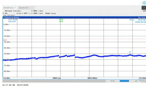
NTNV-n7-PC3-15-20-L-DFT-BPSK-Inner_1RB_Right-3000-12000 -PASS
