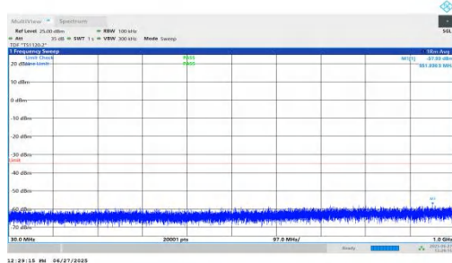
NTNV-n7-PC3-15-25-M-DFT-QPSK-Inner_1RB_Right-30-1000-P ASS
