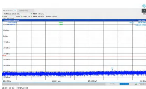
NTNV-n7-PC3-15-15-H-DFT-QPSK-Inner_1RB_Left-30-1000-PA SS
