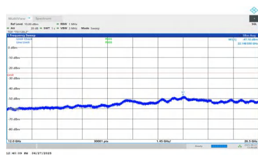
NTNV-n7-PC3-15-30-H-DFT-QPSK-Inner_1RB_Right-12000-26500-PASS
