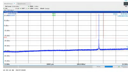
NTNV-n7-PC3-15-30-L-DFT-BPSK-Inner_1RB_Right-1000-3000-P ASS
