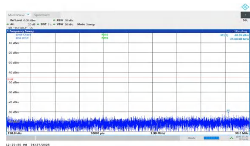
NTNV-n7-PC3-15-20-M-DFT-QPSK-Inner_1RB_Left-0.15-30-PAS S
