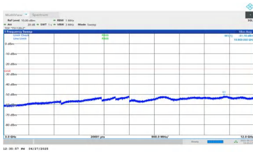
NTNV-n7-PC3-15-30-M-DFT-BPSK-Inner_1RB_Right-3000-1200 0-PASS
