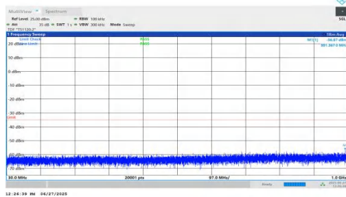
NTNV-n7-PC3-15-25-L-DFT-QPSK-Inner_1RB_Right-30-1000-PASS
