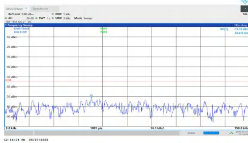
NTVN-n7-PC3-15-15-H-DFT-QPSK-Inner_1RB_Right-0.009-0.15-PASS
