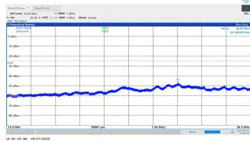
NTNV-n7-PC3-15-35-L-DFT-BPSK-Inner_1RB_Left-12000-26500-PASS
