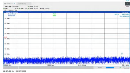
NTNV-n7-PC3-15-25-M-DFT-BPSK-Inner_1RB_Left-0.15-30-PASS
