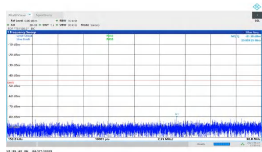
NTNV-n7-PC3-15-30-M-DFT-BPSK-Inner_1RB_Right-0.15-30-PASS SS
