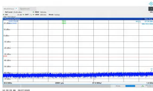
NTNV-n7-PC3-15-30-H-DFT-QPSK-Inner_1RB_Right-30-1000-PASS
