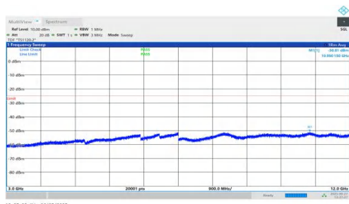
NTNV-n7-PC3-15-30-M-DFT-QPSK-Inner_1RB_Right-3000-12000 0-PASS
