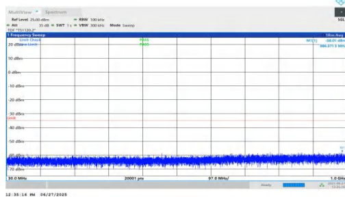
NTNV-n7-PC3-15-30-M-DFT-BPSK-Inner_1RB_Left-30-1000-PASS SS
