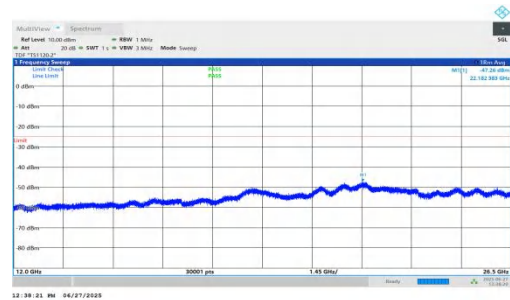
NTNV-n7-PC3-15-30-H-DFT-BPSK-Inner_1RB_Left-12000-26500- PASS
