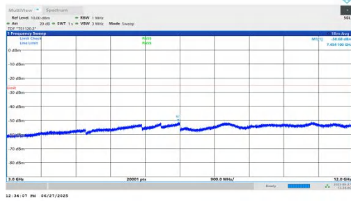
NTNV-n7-PC3-15-30-L-DFT-QPSK-Inner_1RB_Left-3000-12000-PASS
