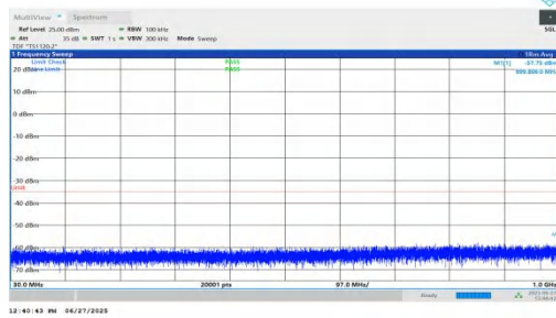
NTNV-n7-PC3-15-35-L-DFT-BPSK-Inner_1RB_Left-30-1000-PASS
