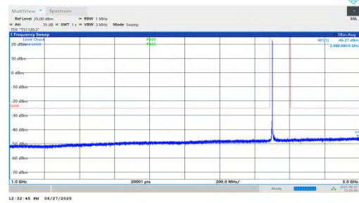
NTNV-n7-PC3-15-30-L-DFT-BPSK-Inner_1RB_Left-1000-3000-PASS
