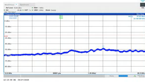
NTVN-n7-PC3-15-15-H-DFT-QPSK-Inner_1RB_Left-12000-26500-PASS
