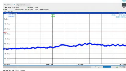
NTNV-n7-PC3-15-25-L-DFT-BPSK-Inner_1RB_Left-12000-26500-PASS
