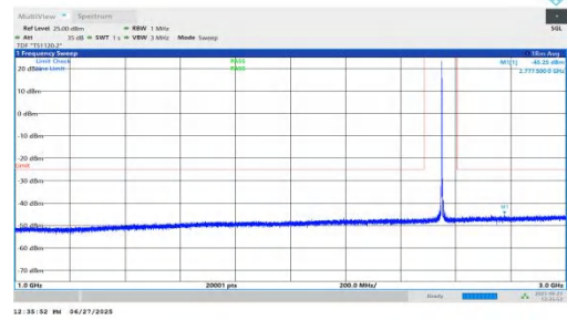
NTNV-n7-PC3-15-30-M-DFT-BPSK-Inner_1RB_Right-1000-3000-P PASS
