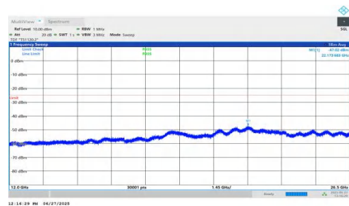
NTVN-n7-PC3-15-15-H-DFT-QPSK-Inner_1RB_Right-12000-26500-PASS
