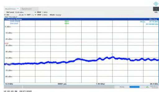
NTNV-n7-PC3-15-20-H-DFT-BPSK-Inner_1RB_Left-12000-26500- PASS
