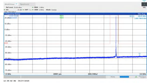
NTNV-n7-PC3-15-30-H-DFT-BPSK-Inner_1RB_Right-1000-3000-P PASS
