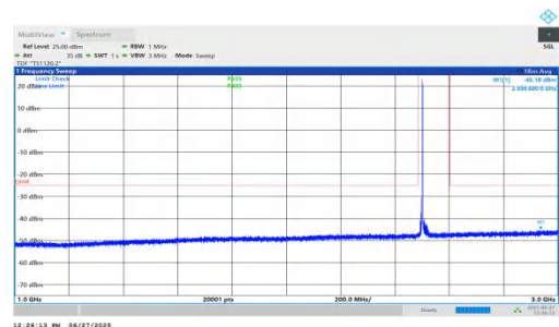
NTNV-n7-PC3-15-25-L-DFT-QPSK-Inner_1RB_Left-1000-3000-PA SS
