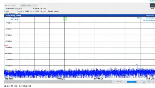
NTNV-n7-PC3-15-20-H-DFT-QPSK-Inner_1RB_Right-0.15-30-PA-SS
