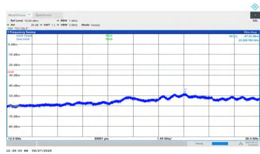
NTNV-n7-PC3-15-30-M-DFT-BPSK-Inner_1RB_Right-12000-2650 0-PASS
