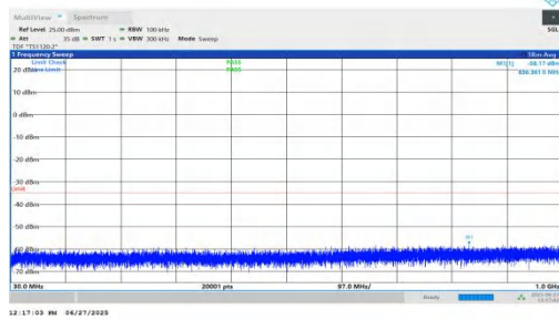
NTNV-n7-PC3-15-20-L-DFT-BPSK-Inner_1RB_Left-30-1000-PASS
