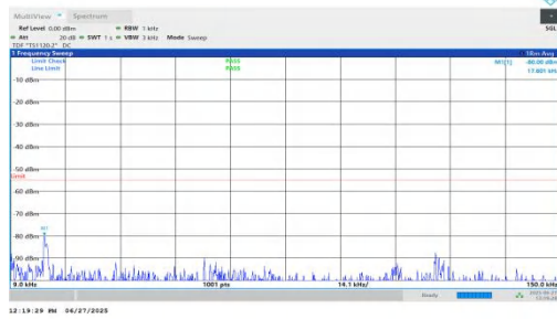
NTVN-n7-PC3-15-20-M-DFT-BPSK-Inner_1RB_Left-0.009-0.15-P ASS
