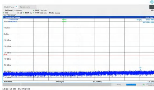
NTNV-n7-PC3-15-20-H-DFT-BPSK-Inner_1RB_Left-30-1000-P ASS
