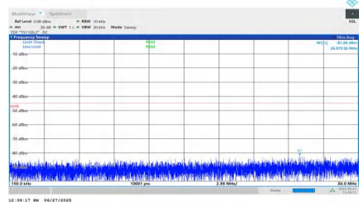
NTNV-n7-PC3-15-30-H-DFT-QPSK-Inner_1RB_Left-0.15-30-P PASS
