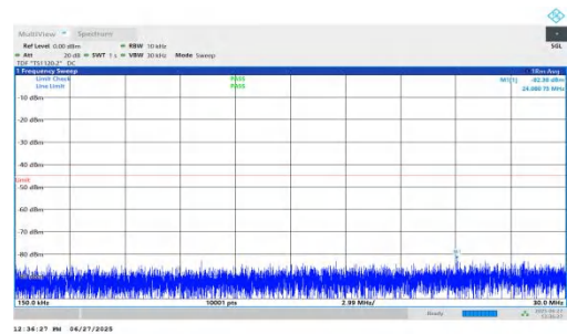
NTNV-n7-PC3-15-30-M-DFT-QPSK-Inner_1RB_Left-0.15-30-PAS S
