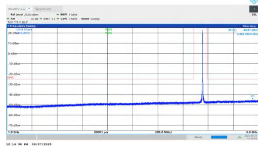
NTNV-n7-PC3-15-15-H-DFT-BPSK-Inner_1RB_Left-1000-3000-PASS
