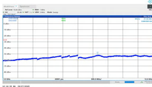
NTNV-n7-PC3-15-15-H-DFT-BPSK-Inner_1RB_Left-3000-12000-PASS
