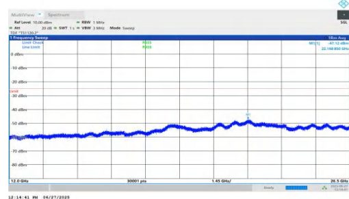
NTNV-n7-PC3-15-15-H-DFT-BPSK-Inner_1RB_Left-12000-26500-PASS
