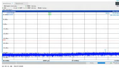
NTNV-n7-PC3-15-30-L-DFT-BPSK-Inner_1RB_Right-30-1000-PA SS
