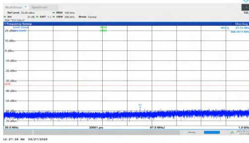
NTNV-n7-PC3-15-25-M-DFT-BPSK-Inner_1RB_Right-30-1000-P ASS
