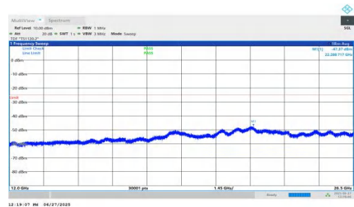
NTNV-n7-PC3-15-20-L-DFT-QPSK-Inner_1RB_Right-12000-26500-PASS
