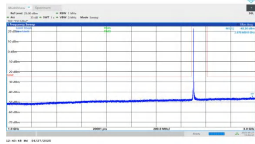
NTNV-n7-PC3-15-35-L-DFT-BPSK-Inner_1RB_Left-1000-3000-PASS
