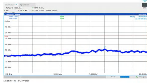
NTNV-n7-PC3-15-25-M-DFT-QPSK-Inner_1RB_Left-12000-26500 -PASS
