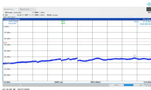
NTVN-n7-PC3-15-20-M-DFT-BPSK-Inner_1RB_Left-3000-12000- PASS
