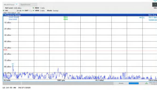
NTNV-n7-PC3-15-20-L-DFT-BPSK-Inner_1RB_Left-0.009-0.15-PASS
