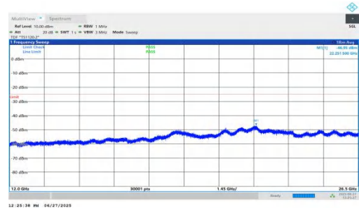
NTNV-n7-PC3-15-25-L-DFT-BPSK-Inner_1RB_Right-12000-2650 0-PASS
