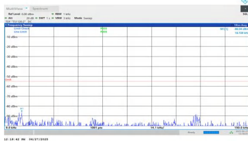
NTNV-n7-PC3-15-20-L-DFT-QPSK-Inner_1RB_Right-0.009-0.15-PASS
