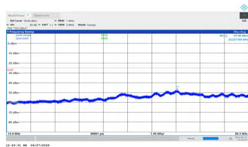
NTNV-n7-PC3-15-25-M-DFT-QPSK-Inner_1RB_Right-12000-2650 0-PASS
