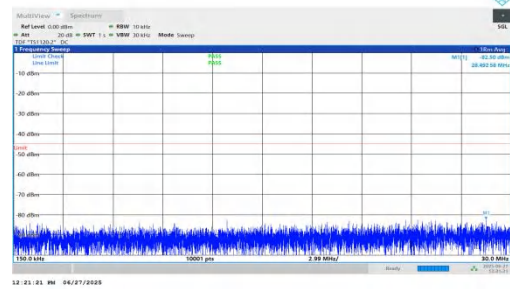
NTNV-n7-PC3-15-20-M-DFT-QPSK-Inner_1RB_Right-0.15-30-PA SS
