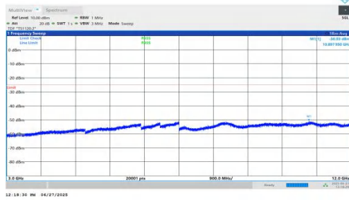
NTNV-n7-PC3-15-20-L-DFT-QPSK-Inner_1RB_Left-3000-12000-PASS
