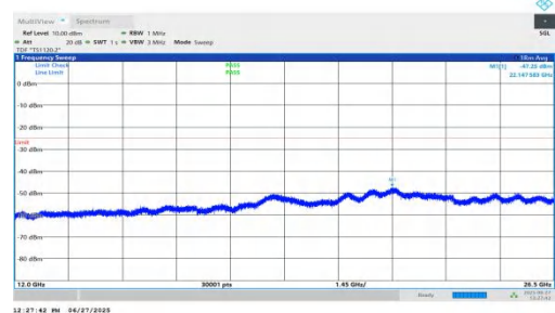
NTNV-n7-PC3-15-25-M-DFT-BPSK-Inner_1RB_Left-12000-26500-PASS
