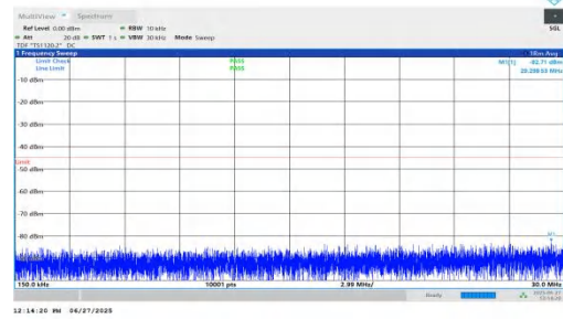
NTNV-n7-PC3-15-15-H-DFT-BPSK-Inner_1RB_Left-0.15-30-PASS
