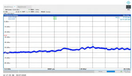
NTNV-n7-PC3-15-20-L-DFT-BPSK-Inner_1RB_Right-12000-2650 0-PASS
