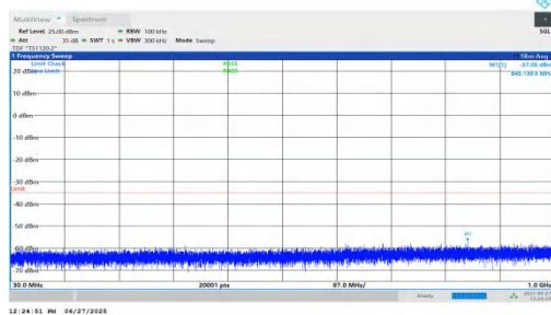
NTNV-n7-PC3-15-25-L-DFT-BPSK-Inner_1RB_Left-30-1000-PASS
