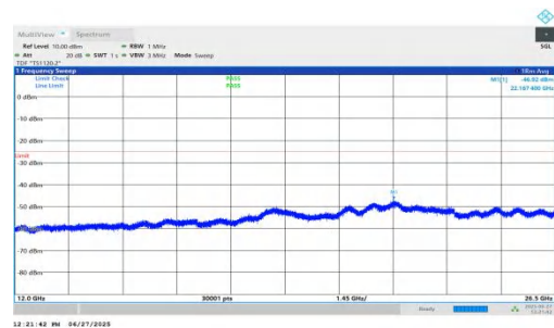
NTNV-n7-PC3-15-20-M-DFT-QPSK-Inner_1RB_Right-12000-2650 0-PASS
