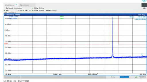
NTNV-n7-PC3-15-30-M-DFT-BPSK-Inner_1RB_Left-1000-3000-PASS ASS
