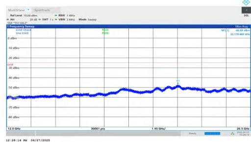
NTNV-n7-PC3-15-25-M-DFT-BPSK-Inner_1RB_Right-12000-26500 0-PASS
