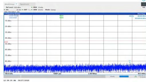
NTNV-n7-PC3-15-30-H-DFT-BPSK-Inner_1RB_Left-0.15-30-PASS
