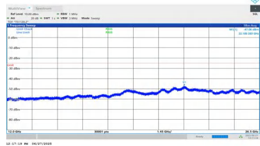
NTNV-n7-PC3-15-20-L-DFT-BPSK-Inner_1RB_Left-12000-26500-PASS
