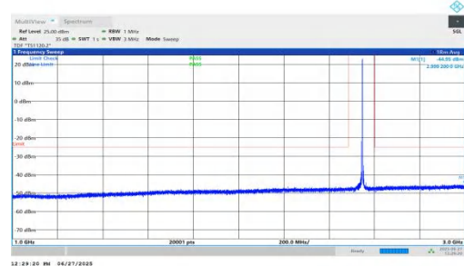
NTNV-n7-PC3-15-25-M-DFT-QPSK-Inner_1RB_Right-1000-3000- PASS
