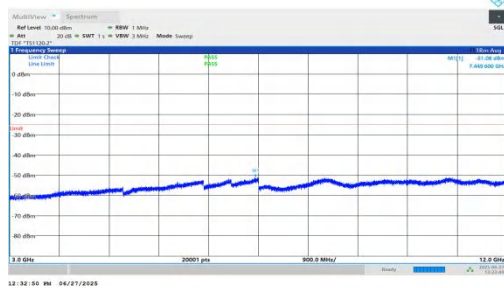
NTNV-n7-PC3-15-30-L-DFT-BPSK-Inner_1RB_Left-3000-12000-PASS
