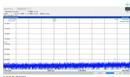
NTNV-n7-PC3-15-20-H-DFT-BPSK-Inner_1RB_Right-0.15-30-PAS S
