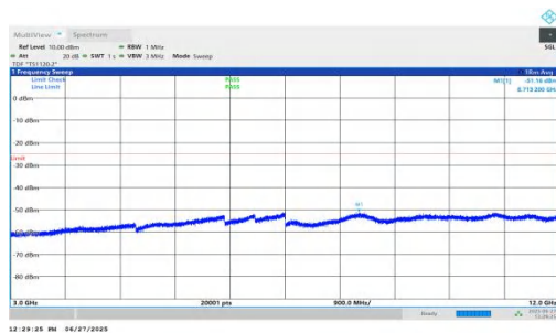
NTNV-n7-PC3-15-25-M-DFT-QPSK-Inner_1RB_Right-3000-1200 0-PASS
