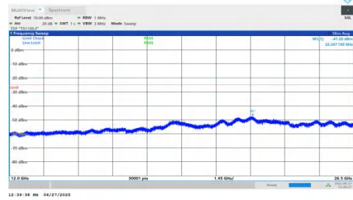
NTNV-n7-PC3-15-30-H-DFT-QPSK-Inner_1RB_Left-12000-26500-PASS
