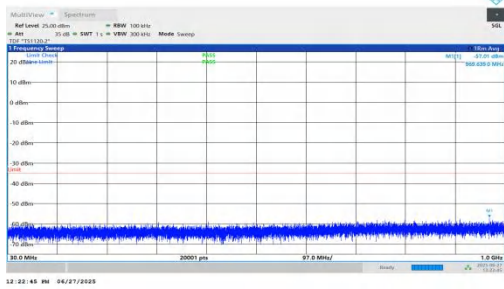
NTNV-n7-PC3-15-20-H-DFT-BPSK-Inner_1RB_Right-30-1000-P ASS
