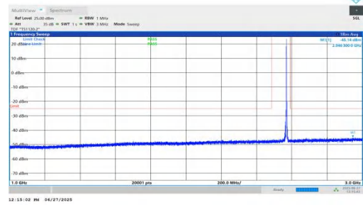
NTNV-n7-PC3-15-15-H-DFT-BPSK-Inner_1RB_Right-1000-3000-P PASS
