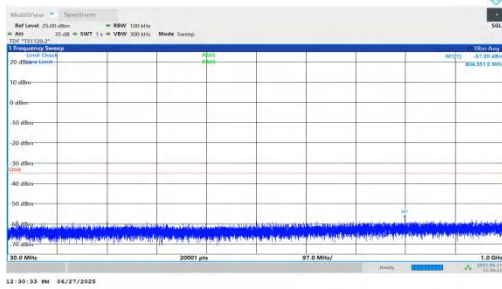
NTNV-n7-PC3-15-25-H-DFT-BPSK-Inner_1RB_Right-30-1000-P ASS
