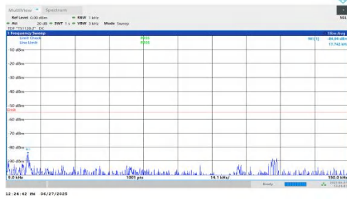
NTNV-n7-PC3-15-25-L-DFT-BPSK-Inner_1RB_Left-0.009-0.15-PASS
