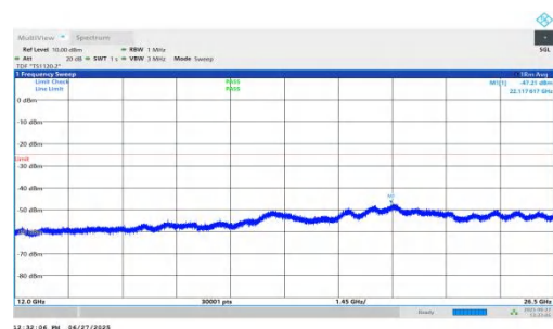
NTV-n7-PC3-15-25-H-DFT-QPSK-Inner_1RB_Right-12000-26500-PASS
