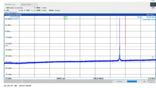
NTNV-n7-PC3-15-25-L-DFT-BPSK-Inner_1RB_Right-1000-3000-P ASS
