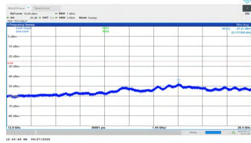
NTNV-n7-PC3-15-20-H-DFT-QPSK-Inner_1RB_Left-12000-26500-PASS
