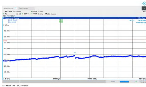
NTNV-n7-PC3-15-30-H-DFT-BPSK-Inner_1RB_Left-3000-12000- PASS
