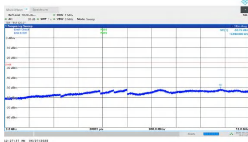
NTNV-n7-PC3-15-25-M-DFT-BPSK-Inner_1RB_Left-3000-12000-PASS
