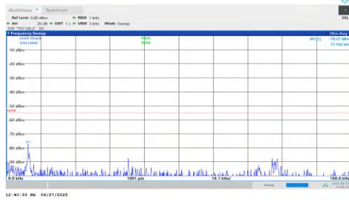
NTNV-n7-PC3-15-35-L-DFT-BPSK-Inner_1RB_Left-0.009-0.15-PASS
