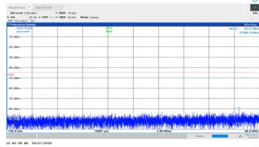
NTNV-n7-PC3-15-35-L-DFT-BPSK-Inner_1RB_Left-0.15-30-PASS
