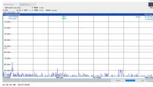
NTNV-n7-PC3-15-30-L-DFT-BPSK-Inner_1RB_Left-0.009-0.15-PASS
