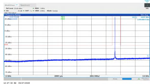
NTNV-n7-PC3-15-25-M-DFT-BPSK-Inner_1RB_Left-1000-3000-PASS
