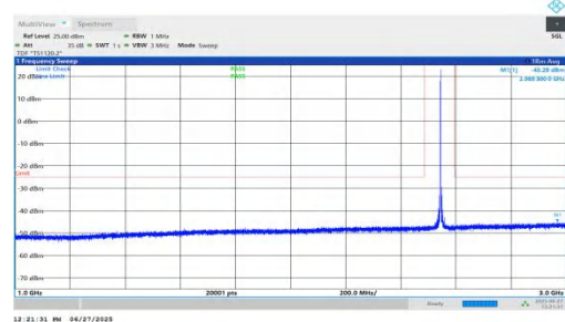
NTNV-n7-PC3-15-20-M-DFT-QPSK-Inner_1RB_Right-1000-3000- PASS
