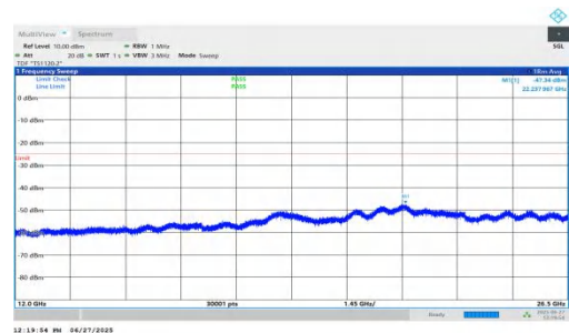
NTVN-n7-PC3-15-20-M-DFT-BPSK-Inner_1RB_Left-12000-26500- PASS
