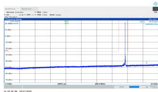
NTNV-n7-PC3-15-30-H-DFT-QPSK-Inner_1RB_Right-1000-3000-PASS
