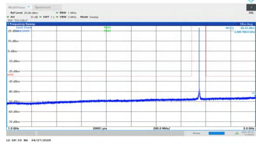
NTNV-n7-PC3-15-25-M-DFT-BPSK-Inner_1RB_Right-1000-3000-P PASS
