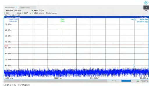
NTNV-n7-PC3-15-20-L-DFT-BPSK-Inner_1RB_Right-0.15-30-PASS
