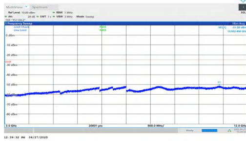
NTNV-n7-PC3-15-30-H-DFT-QPSK-Inner_1RB_Left-3000-12000-PASS
