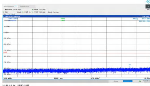
NTNV-n7-PC3-15-20-M-DFT-QPSK-Inner_1RB_Right-30-1000-P ASS
