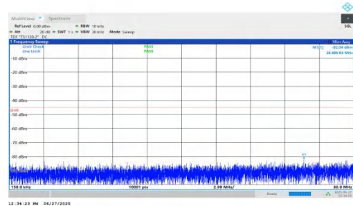
NTNV-n7-PC3-15-30-L-DFT-QPSK-Inner_1RB_Right-0.15-30-PASS
