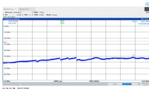
NTNV-n7-PC3-15-10-M-DFT-BPSK-Inner_1RB_Left-3000-12000-PASS
