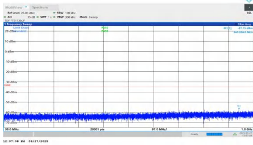
NTNV-n7-PC3-15-10-H-DFT-BPSK-Inner_1RB_Right-30-1000-P ASS
