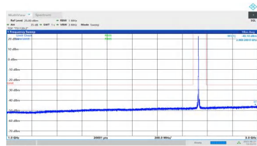
NTNV-n7-PC3-15-15-M-DFT-QPSK-Inner_1RB_Left-1000-3000-PASS
