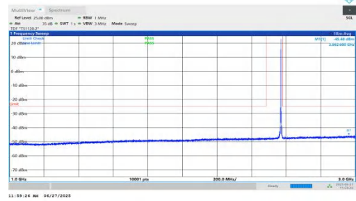
NTNV-n7-PC3-15-5-H-DFT-BPSK-Inner_1RB_Right-1000-3000-P ASS
