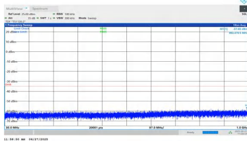
NTVN-n7-PC3-15-5-H-DFT-BPSK-Inner_1RB_Left-30-1000-PAS S
