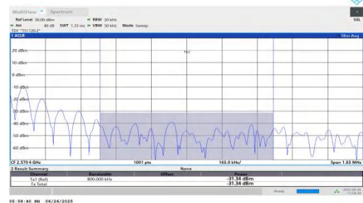
NTNV-n7-PC3-15-40-H-DFT-BPSK-Edge_1RB_Right-PASS
