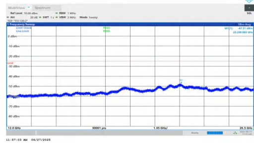
NTNV-n7-PC3-15-5-M-DFT-BPSK-Inner_1RB_Right-12000-26500 -PASS
