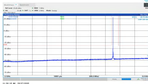
NTNV-n7-PC3-15-5-L-DFT-BPSK-Inner_1RB_Right-1000-3000-PA SS
