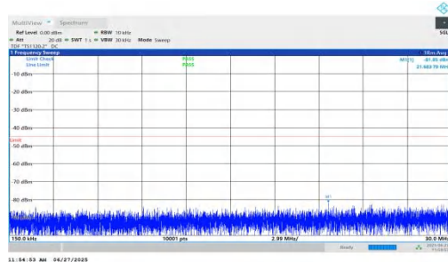
NTNV-n7-PC3-15-5-L-DFT-QPSK-Inner_1RB_Left-0.15-30-PASS
