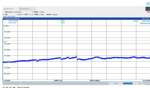
NTNV-n7-PC3-15-5-H-DFT-QPSK-Inner_1RB_Right-3000-12000 -PASS
