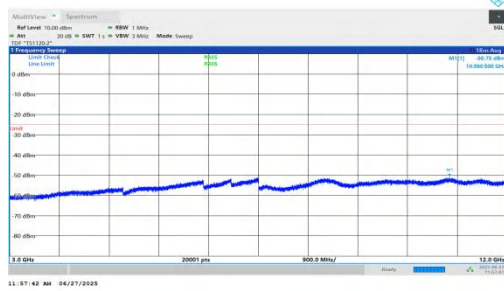
NTNV-n7-PC3-15-5-M-DFT-QPSK-Inner_1RB_Left-3000-12000-PASS
