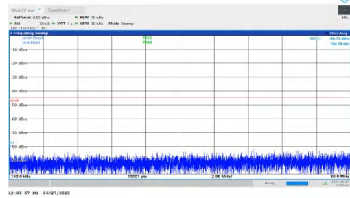
NTNV-n7-PC3-15-10-M-DFT-BPSK-Inner_1RB_Left-0.15-30-PASS
