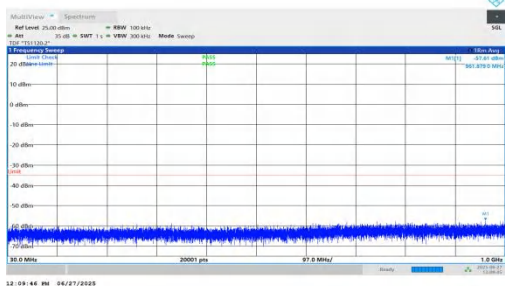
NTNV-n7-PC3-15-15-L-DFT-BPSK-Inner_1RB_Right-30-1000-PA SS
