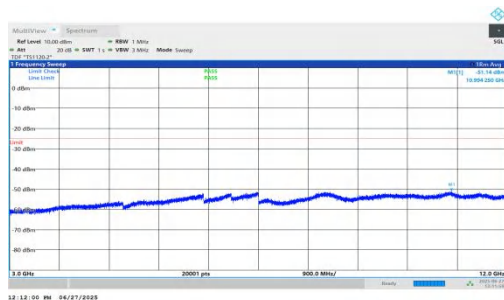
NTNV-n7-PC3-15-15-M-DFT-BPSK-Inner_1RB_Left-3000-12000-PASS
