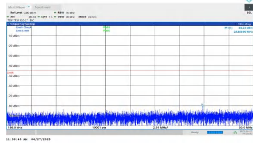
NTVN-n7-PC3-15-5-H-DFT-BPSK-Inner_1RB_Left-0.15-30-PASS
