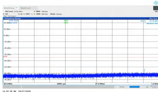
NTNV-n7-PC3-15-5-H-DFT-QPSK-Inner_1RB_Right-30-1000-PA SS
