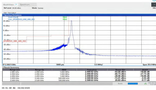
NTNV-n7-PC3-15-35-L-DFT-BPSK-Edge_1RB_Left-PASS
