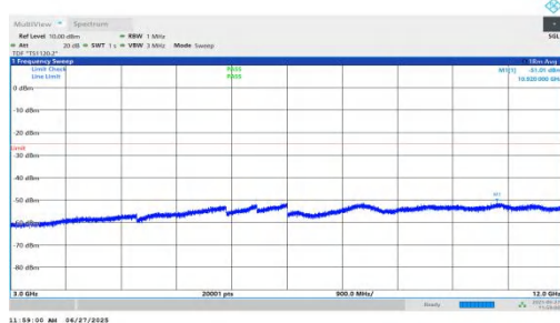
NTVN-n7-PC3-15-5-H-DFT-BPSK-Inner_1RB_Left-3000-12000-P ASS
