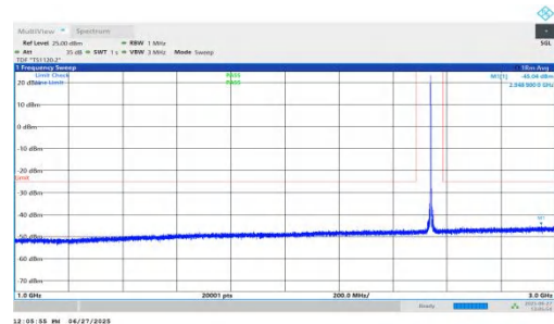
NTNV-n7-PC3-15-10-M-DFT-QPSK-Inner_1RB_Right-1000-3000- PASS
