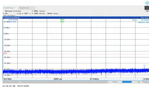
NTNV-n7-PC3-15-10-M-DFT-BPSK-Inner_1RB_Left-30-1000-PASS
