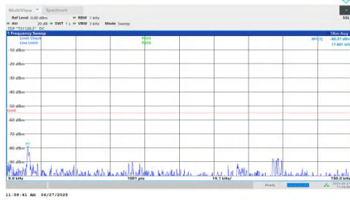
NTVN-n7-PC3-15-5-H-DFT-BPSK-Inner_1RB_Left-0.009-0.15-PA SS
