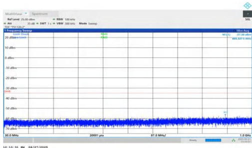
NTNV-n7-PC3-15-15-L-DFT-QPSK-Inner_1RB_Left-30-1000-PA SS
