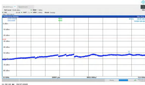
NTNV-n7-PC3-15-5-M-DFT-BPSK-Inner_1RB_Left-3000-12000-PASS
