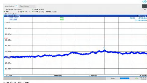
NTNV-n7-PC3-15-10-H-DFT-BPSK-Inner_1RB_Left-12000-26500-PASS
