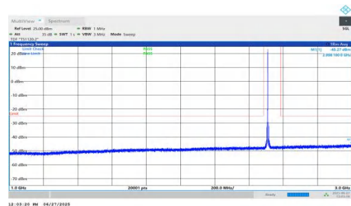
NTNV-n7-PC3-15-10-L-DFT-QPSK-Inner_1RB_Right-1000-3000-PASS
