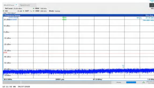
NTNV-n7-PC3-15-15-L-DFT-QPSK-Inner_1RB_Right-30-1000-PASS
