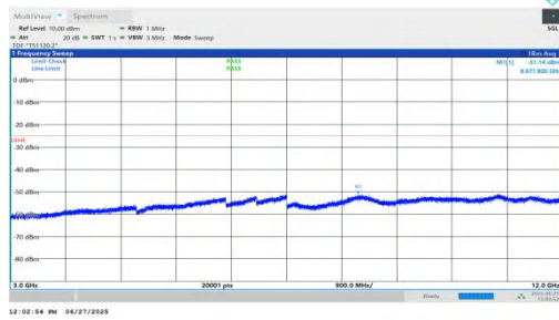
NTNV-n7-PC3-15-10-L-DFT-QPSK-Inner_1RB_Left-3000-12000-PASS
