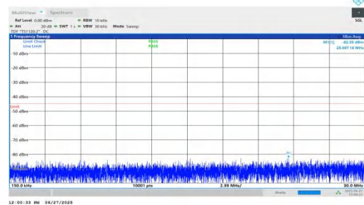
NTNV-n7-PC3-15-5-H-DFT-QPSK-Inner_1RB_Right-0.15-30-PAS S
