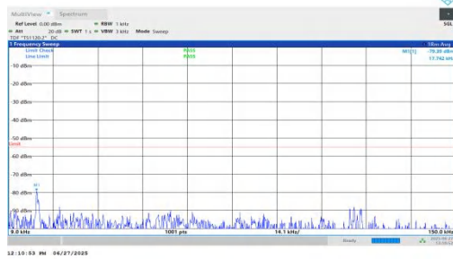
NTNV-n7-PC3-15-15-L-DFT-QPSK-Inner_1RB_Right-0.009-0.15-PASS
