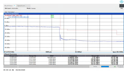
NTNV-n7-PC3-15-40-H-DFT-QPSK-Outer_Full-PASS
