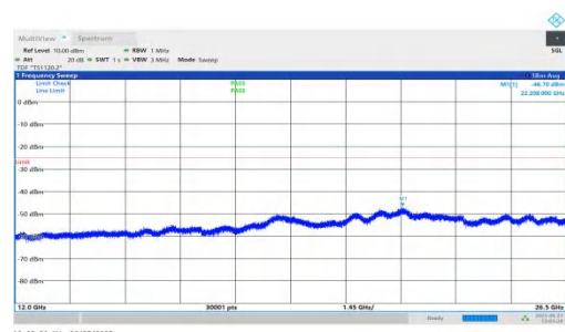
NTNV-n7-PC3-15-10-L-DFT-QPSK-Inner_1RB_Right-12000-26500-PASS
