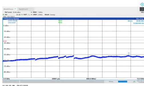
NTNV-n7-PC3-15-10-M-DFT-QPSK-Inner_1RB_Right-3000-1200 0-PASS
