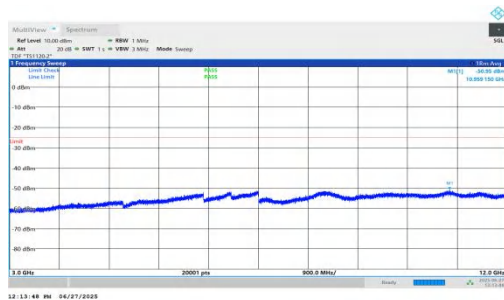
NTNV-n7-PC3-15-15-M-DFT-QPSK-Inner_1RB_Right-3000-1200 0-PASS
