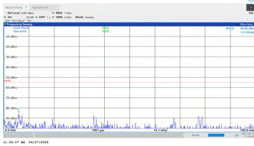
NTNV-n7-PC3-15-5-M-DFT-BPSK-Inner_1RB_Left-0.009-0.15-PASS
