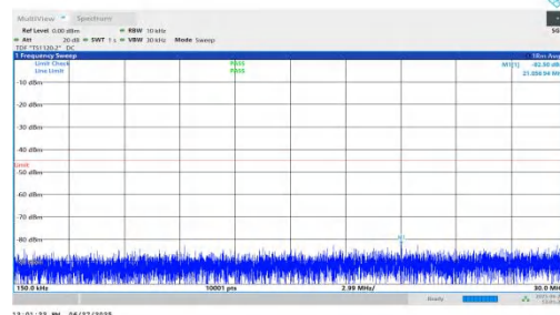
NTNV-n7-PC3-15-10-L-DFT-BPSK-Inner_1RB_Left-0.15-30-PASS
