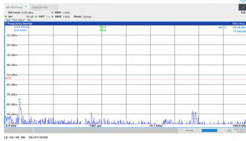
NTNV-n7-PC3-15-10-H-DFT-BPSK-Inner_1RB_Left-0.009-0.15-P ASS
