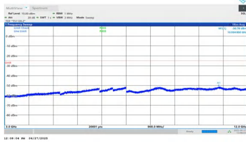
NTNV-n7-PC3-15-10-H-DFT-QPSK-Inner_1RB_Left-3000-12000-PASS
