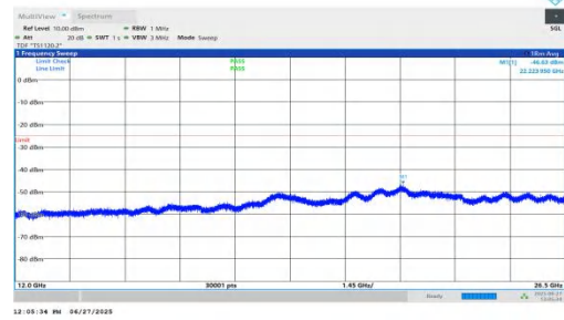
NTNV-n7-PC3-15-10-M-DFT-QPSK-Inner_1RB_Left-12000-26500 -PASS
