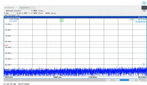
NTNV-n7-PC3-15-5-L-DFT-QPSK-Inner_1RB_Right-0.15-30-PAS S
