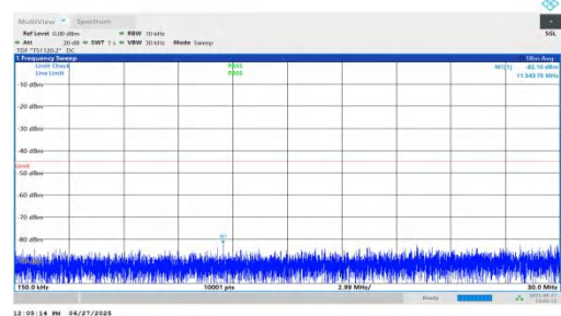
NTNV-n7-PC3-15-10-M-DFT-QPSK-Inner_1RB_Left-0.15-30-PASS
