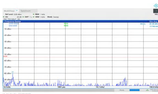
NTNV-n7-PC3-15-10-M-DFT-BPSK-Inner_1RB_Right-0.009-0.15-PASS
