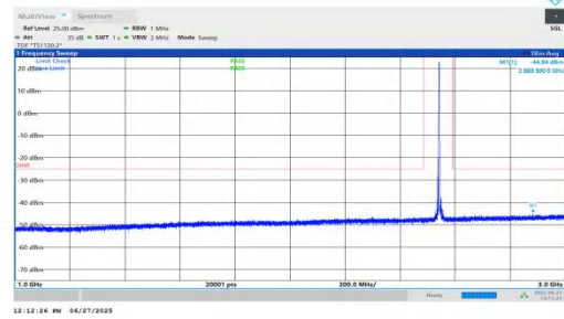
NTNV-n7-PC3-15-15-M-DFT-BPSK-Inner_1RB_Right-1000-3000-PASS
