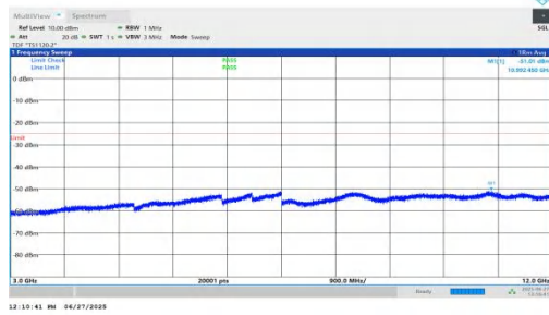
NTNV-n7-PC3-15-15-L-DFT-QPSK-Inner_1RB_Left-3000-12000-PASS
