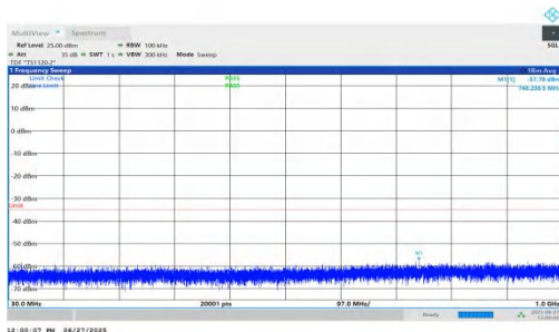
NTNV-n7-PC3-15-5-H-DFT-QPSK-Inner_1RB_Left-30-1000-PAS S
