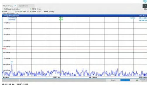
NTNV-n7-PC3-15-10-M-DFT-QPSK-Inner_1RB_Left-0.009-0.15-PASS
