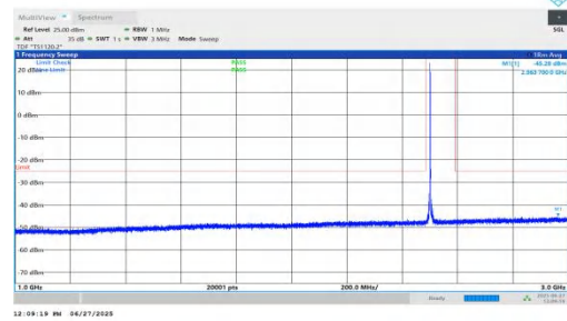
NTNV-n7-PC3-15-15-L-DFT-BPSK-Inner_1RB_Left-1000-3000-PASS
