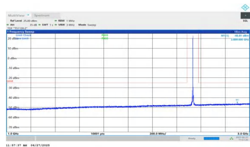
NTNV-n7-PC3-15-5-M-DFT-QPSK-Inner_1RB_Left-1000-3000-PA SS
