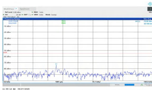
NTVN-n7-PC3-15-5-H-DFT-BPSK-Inner_1RB_Right-0.009-0.15-P ASS
