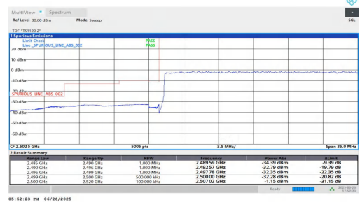
NTNV-n7-PC3-15-35-L-DFT-QPSK-Outer_Full-PASS
