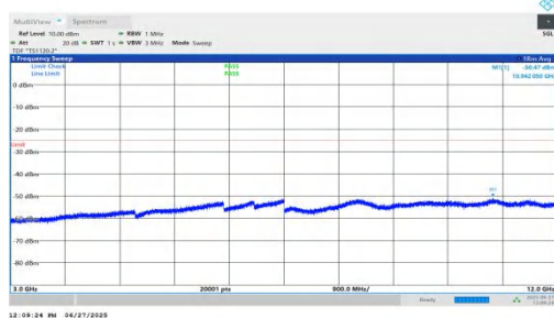
NTNV-n7-PC3-15-15-L-DFT-BPSK-Inner_1RB_Left-3000-12000-PASS
