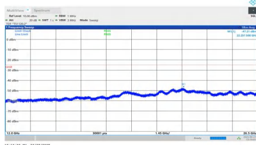
NTNV-n7-PC3-15-15-L-DFT-BPSK-Inner_1RB_Right-12000-2650 0-PASS
