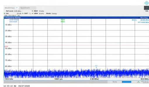
NTNV-n7-PC3-15-10-L-DFT-QPSK-Inner_1RB_Right-0.15-30-PASS
