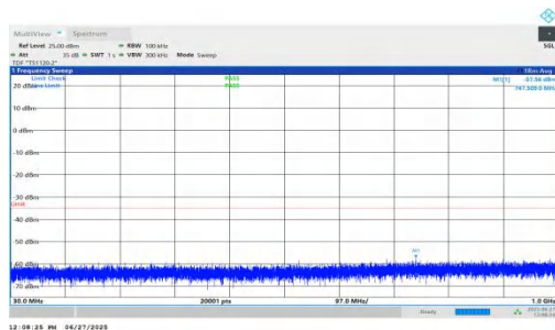
NTNV-n7-PC3-15-10-H-DFT-QPSK-Inner_1RB_Right-30-1000-PASS
