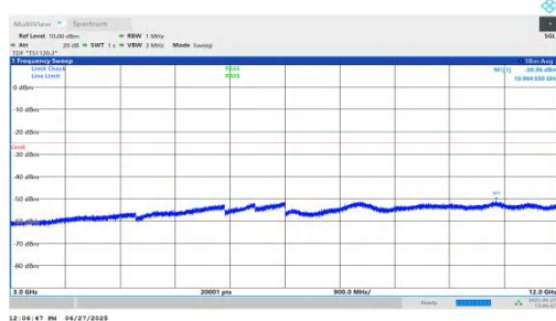
NTNV-n7-PC3-15-10-H-DFT-BPSK-Inner_1RB_Left-3000-12000-PASS
