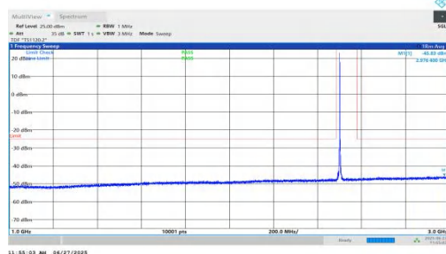
NTNV-n7-PC3-15-5-L-DFT-QPSK-Inner_1RB_Left-1000-3000-PA SS
