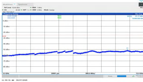
NTNV-n7-PC3-15-5-H-DFT-BPSK-Inner_1RB_Right-3000-12000- PASS
