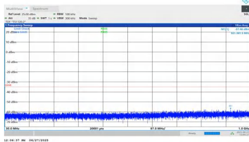
NTNV-n7-PC3-15-10-H-DFT-BPSK-Inner_1RB_Left-30-1000-PASS
