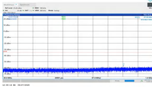
NTNV-n7-PC3-15-15-L-DFT-BPSK-Inner_1RB_Left-30-1000-PASS
