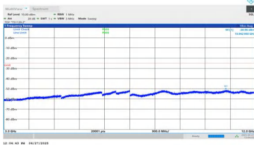
NTNV-n7-PC3-15-10-M-DFT-BPSK-Inner_1RB_Right-3000-12000-0-PASS
