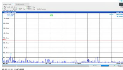
NTNV-n7-PC3-15-5-H-DFT-QPSK-Inner_1RB_Right-0.009-0.15- PASS
