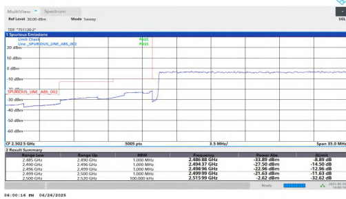
NTNV-n7-PC3-15-50-L-DFT-BPSK-Outer_Full-PASS
