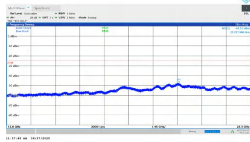
NTNV-n7-PC3-15-5-M-DFT-QPSK-Inner_1RB_Left-12000-26500-PASS
