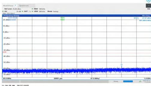
NTNV-n7-PC3-15-5-L-DFT-QPSK-Inner_1RB_Left-30-1000-PAS S
