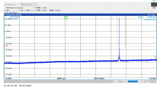
NTVN-n7-PC3-15-10-L-DFT-BPSK-Inner_1RB_Right-1000-3000-P ASS
