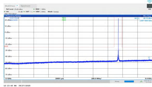
NTNV-n7-PC3-15-15-M-DFT-QPSK-Inner_1RB_Right-1000-3000- PASS
