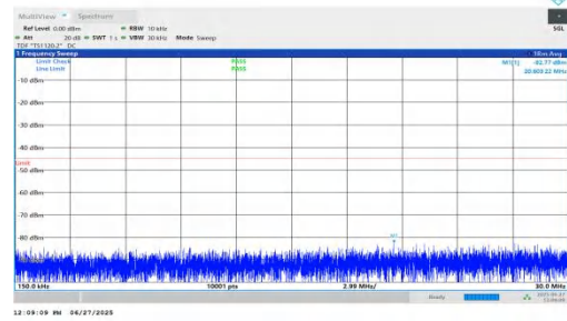
NTNV-n7-PC3-15-15-L-DFT-BPSK-Inner_1RB_Left-0.15-30-PASS
