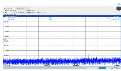
NTNV-n7-PC3-15-15-M-DFT-BPSK-Inner_1RB_Right-0.15-30-PASS
