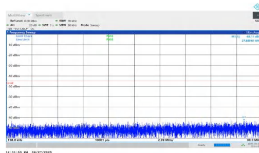
NTNV-n7-PC3-15-10-L-DFT-BPSK-Inner_1RB_Right-0.15-30-PASS
