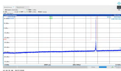
NTNV-n7-PC3-15-10-H-DFT-QPSK-Inner_1RB_Right-1000-3000-PASS
