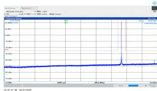
NTNV-n7-PC3-15-10-M-DFT-BPSK-Inner_1RB_Left-1000-3000-PASS
