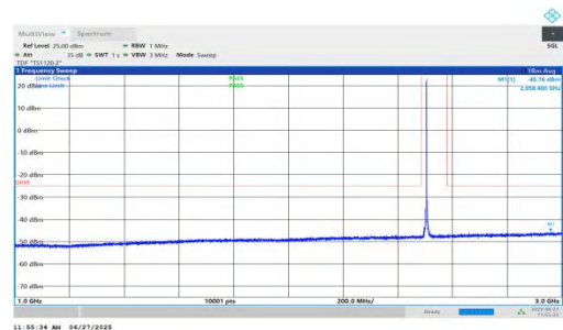
NTNV-n7-PC3-15-5-L-DFT-QPSK-Inner_1RB_Right-1000-3000-P ASS
