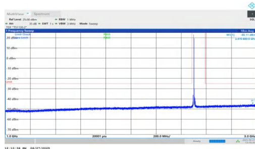
NTNV-n7-PC3-15-15-L-DFT-QPSK-Inner_1RB_Left-1000-3000-PA SS
