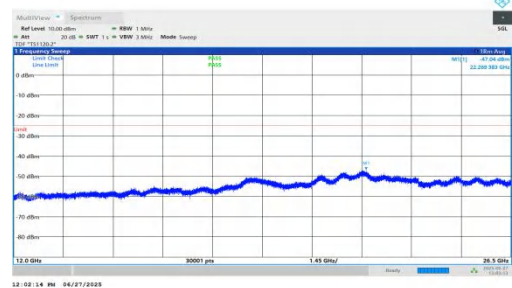
NTVN-n7-PC3-15-10-L-DFT-BPSK-Inner_1RB_Right-12000-2650 0-PASS
