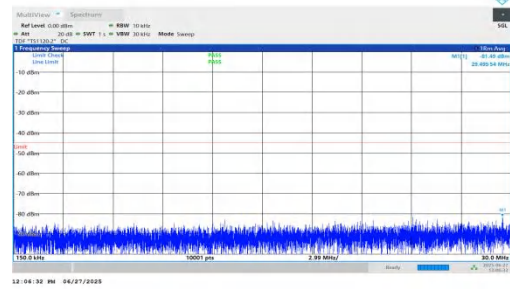
NTNV-n7-PC3-15-10-H-DFT-BPSK-Inner_1RB_Left-0.15-30-PASS
