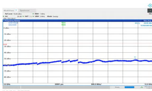
NTNV-n7-PC3-15-10-H-DFT-QPSK-Inner_1RB_Right-3000-12000-PASS
