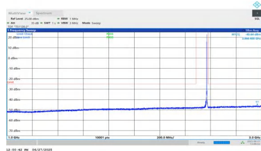
NTNV-n7-PC3-15-5-H-DFT-QPSK-Inner_1RB_Right-1000-3000-P ASS
