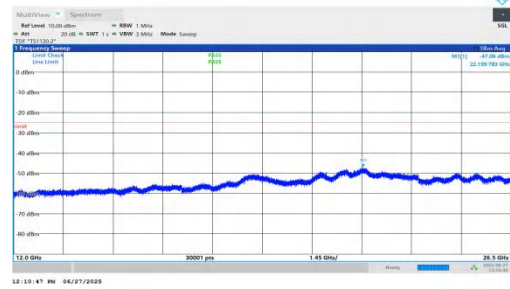
NTNV-n7-PC3-15-15-L-DFT-QPSK-Inner_1RB_Left-12000-26500-PASS
