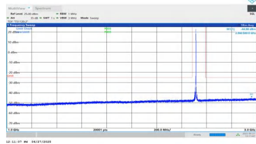
NTNV-n7-PC3-15-15-L-DFT-QPSK-Inner_1RB_Right-1000-3000-PASS
