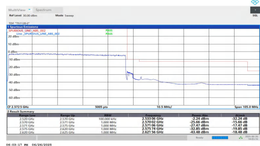
NTNV-n7-PC3-15-50-H-DFT-QPSK-Outer_Full-PASS
