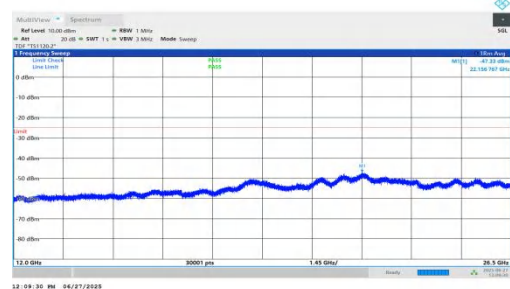
NTNV-n7-PC3-15-15-L-DFT-BPSK-Inner_1RB_Left-12000-26500-PASS
