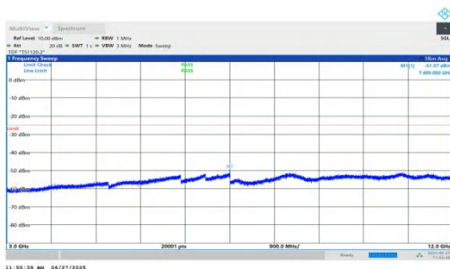
NTNV-n7-PC3-15-5-L-DFT-QPSK-Inner_1RB_Right-3000-12000- PASS
