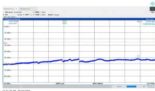
NTNV-n7-PC3-15-10-L-DFT-BPSK-Inner_1RB_Left-3000-12000-PASS
