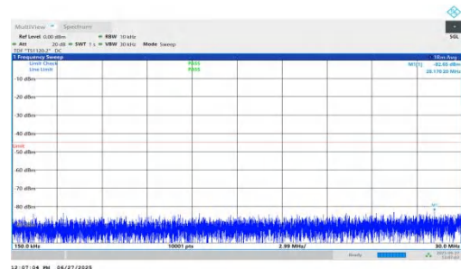
NTNV-n7-PC3-15-10-H-DFT-BPSK-Inner_1RB_Right-0.15-30-PASS
