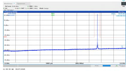
NTNV-n7-PC3-15-5-M-DFT-BPSK-Inner_1RB_Right-1000-3000-P ASS
