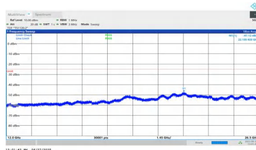
NTNV-n7-PC3-15-10-L-DFT-BPSK-Inner_1RB_Left-12000-26500-PASS
