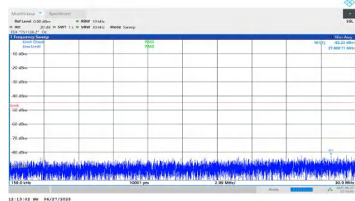
NTNV-n7-PC3-15-15-M-DFT-QPSK-Inner_1RB_Left-0.15-30-PASS
