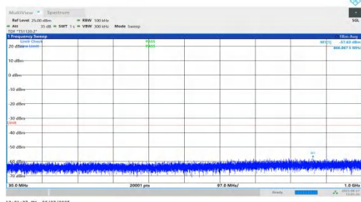
NTNV-n7-PC3-15-10-L-DFT-BPSK-Inner_1RB_Left-30-1000-PASS
