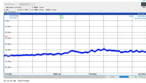
NTNV-n7-PC3-15-15-M-DFT-QPSK-Inner_1RB_Left-12000-26500 -PASS
