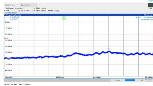
NTNV-n7-PC3-15-5-H-DFT-QPSK-Inner_1RB_Left-12000-26500-P PASS
