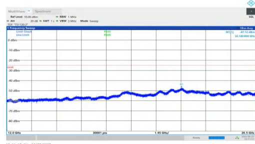
NTNV-n7-PC3-15-15-L-DFT-QPSK-Inner_1RB_Right-12000-26500-PASS
