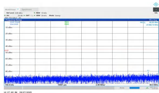
NTNV-n7-PC3-15-10-H-DFT-QPSK-Inner_1RB_Left-0.15-30-PAS S
