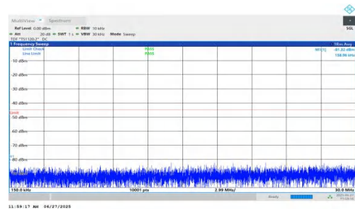
NTVN-n7-PC3-15-5-H-DFT-BPSK-Inner_1RB_Right-0.15-30-PAS S
