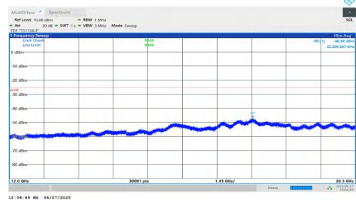
NTNV-n7-PC3-15-10-M-DFT-BPSK-Inner_1RB_Right-12000-26500-0-PASS
