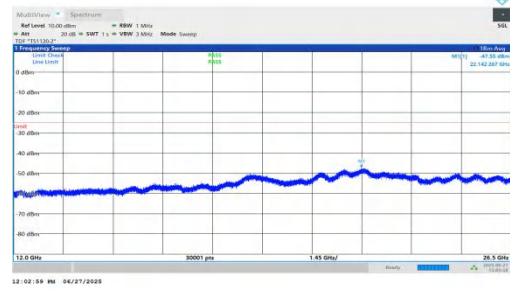
NTNV-n7-PC3-15-10-L-DFT-QPSK-Inner_1RB_Left-12000-26500-PASS
