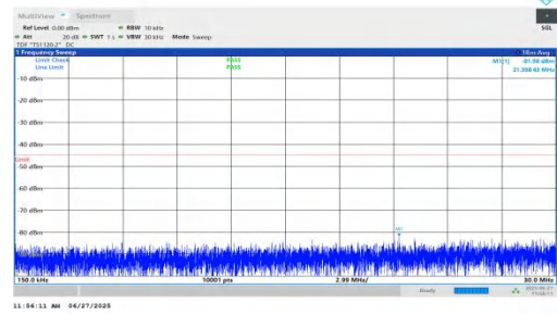
NTNV-n7-PC3-15-5-M-DFT-BPSK-Inner_1RB_Left-0.15-30-PASS
