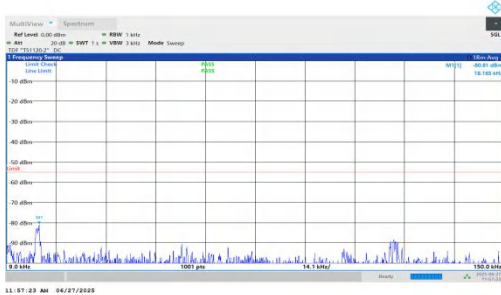
NTNV-n7-PC3-15-5-M-DFT-QPSK-Inner_1RB_Left-0.009-0.15-P ASS
