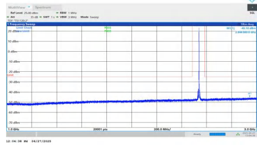
NTNV-n7-PC3-15-10-M-DFT-BPSK-Inner_1RB_Right-1000-3000-P PASS
