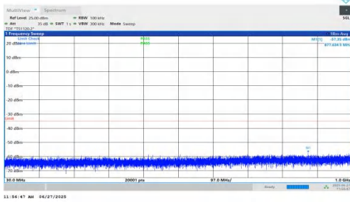
NTNV-n7-PC3-15-5-M-DFT-BPSK-Inner_1RB_Right-30-1000-PA SS
