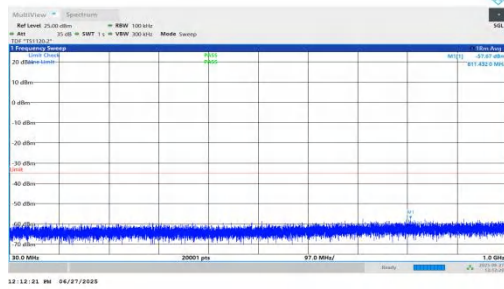
NTNV-n7-PC3-15-15-M-DFT-BPSK-Inner_1RB_Right-30-1000-PASS
