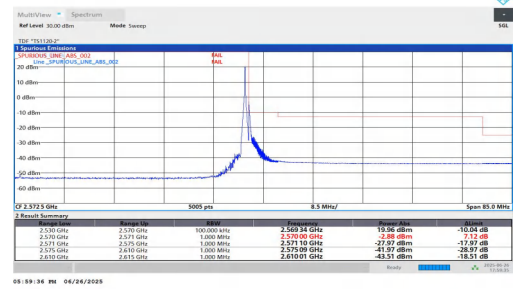
NTNV-n7-PC3-15-40-H-DFT-QPSK-Edge_1RB_Right
