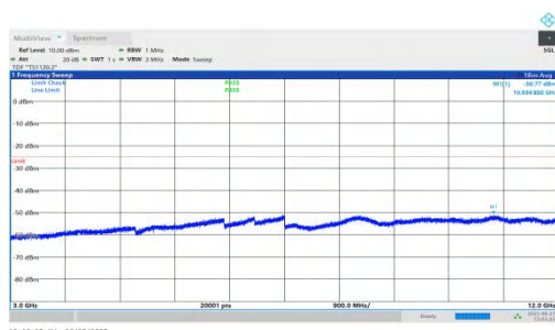
NTNV-n7-PC3-15-10-L-DFT-QPSK-Inner_1RB_Right-3000-12000-PASS
