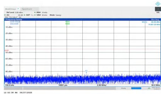
NTVN-n7-PC3-15-10-L-DFT-QPSK-Inner_1RB_Left-0.15-30-PASS
