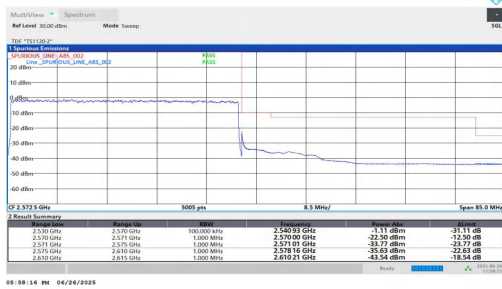
NTNV-n7-PC3-15-40-H-DFT-BPSK-Outer_Full-PASS
