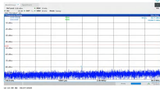
NTNV-n7-PC3-15-15-L-DFT-QPSK-Inner_1RB_Right-0.15-30-PASS
