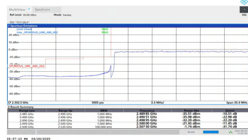
NTNV-n7-PC3-15-40-L-DFT-QPSK-Outer_Full-PASS
