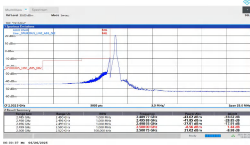
NTNV-n7-PC3-15-50-L-DFT-BPSK-Edge_1RB_Left
