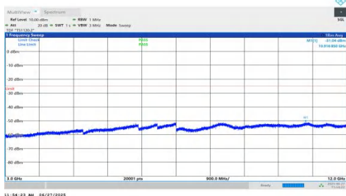
NTNV-n7-PC3-15-5-L-DFT-BPSK-Inner_1RB_Right-3000-12000- PASS
