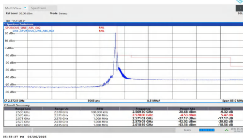
NTNV-n7-PC3-15-40-H-DFT-BPSK-Edge_1RB_Right
