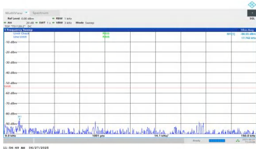
NTNV-n7-PC3-15-5-L-DFT-QPSK-Inner_1RB_Left-0.009-0.15-PA SS
