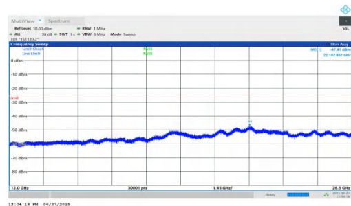
NTNV-n7-PC3-15-10-M-DFT-BPSK-Inner_1RB_Left-12000-26500-PASS
