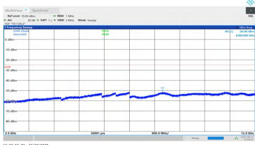
NTNV-n7-PC3-15-15-L-DFT-BPSK-Inner_1RB_Right-3000-12000 -PASS
