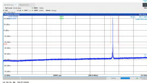
NTNV-n7-PC3-15-15-L-DFT-BPSK-Inner_1RB_Right-1000-3000-P ASS
