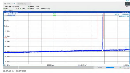
NTNV-n7-PC3-15-10-H-DFT-BPSK-Inner_1RB_Right-1000-3000-P PASS
