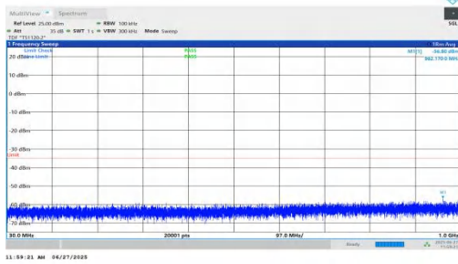
NTNV-n7-PC3-15-5-H-DFT-BPSK-Inner_1RB_Right-30-1000-PA SS
