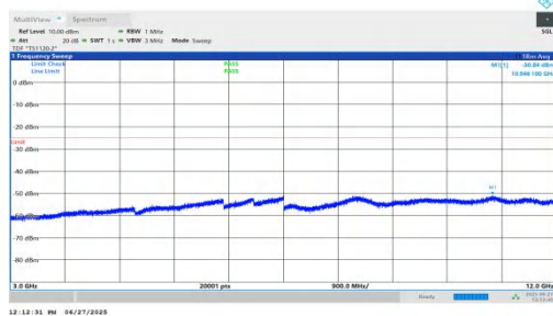
NTNV-n7-PC3-15-15-M-DFT-BPSK-Inner_1RB_Right-3000-12000-PASS
