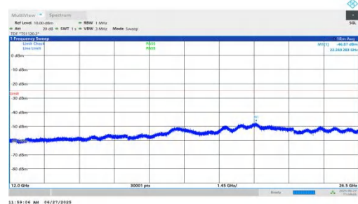
NTVN-n7-PC3-15-5-H-DFT-BPSK-Inner_1RB_Left-12000-26500-P ASS
