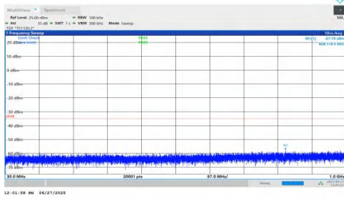
NTVN-n7-PC3-15-10-L-DFT-BPSK-Inner_1RB_Right-30-1000-PA SS
