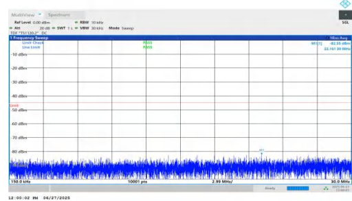
NTNV-n7-PC3-15-5-H-DFT-QPSK-Inner_1RB_Left-0.15-30-PASS
