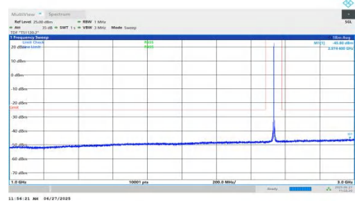
NTNV-n7-PC3-15-5-M-DFT-BPSK-Inner_1RB_Left-1000-3000-PASS
