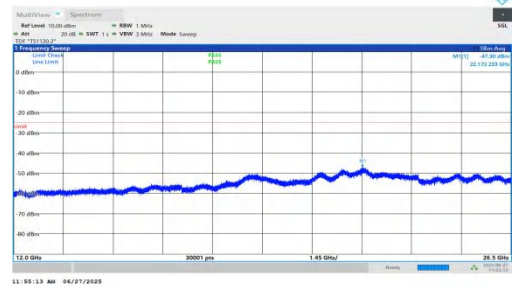
NTNV-n7-PC3-15-5-L-DFT-QPSK-Inner_1RB_Left-12000-26500-P ASS
