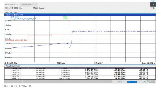
NTNV-n7-PC3-15-50-L-DFT-QPSK-Outer_Full-PASS
