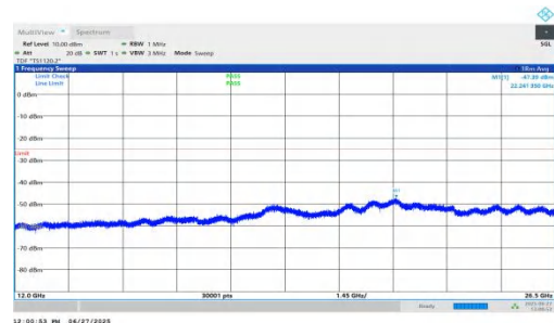
NTNV-n7-PC3-15-5-H-DFT-QPSK-Inner_1RB_Right-12000-26500 -PASS
