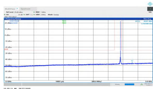
NTNV-n7-PC3-15-5-H-DFT-QPSK-Inner_1RB_Left-1000-3000-PA SS
