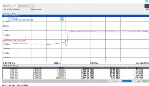
NTNV-n7-PC3-15-40-L-DFT-BPSK-Outer_Full-PASS
