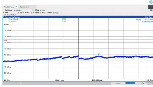
NTNV-n7-PC3-15-15-L-DFT-QPSK-Inner_1RB_Right-3000-12000-PASS
