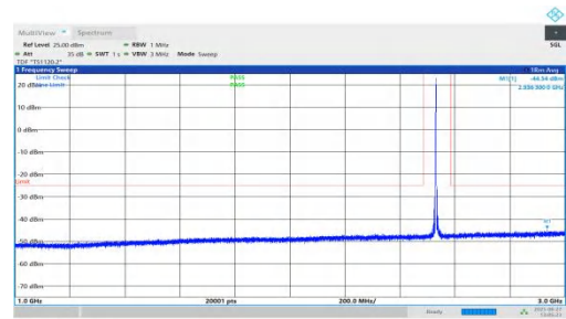
NTNV-n7-PC3-15-10-M-DFT-QPSK-Inner_1RB_Left-1000-3000-PASS
