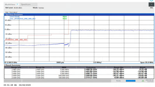
NTNV-n7-PC3-15-35-L-DFT-BPSK-Outer_Full-PASS
