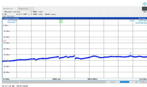
NTNV-n7-PC3-15-10-H-DFT-BPSK-Inner_1RB_Right-3000-1200 0-PASS
