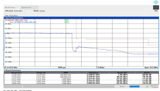
NTNV-n7-PC3-15-35-H-DFT-QPSK-Outer_Full-PASS
