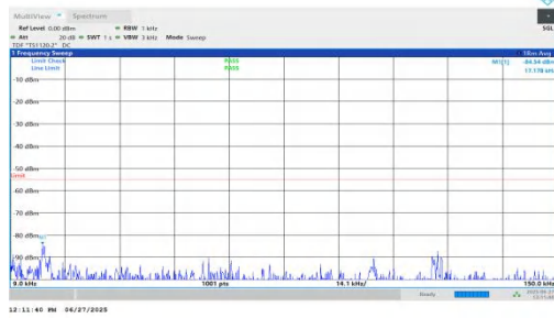
NTNV-n7-PC3-15-15-M-DFT-BPSK-Inner_1RB_Left-0.009-0.15-PASS
