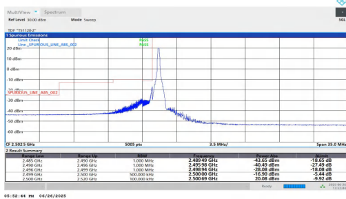
NTNV-n7-PC3-15-35-L-DFT-QPSK-Edge_1RB_Left-PASS
