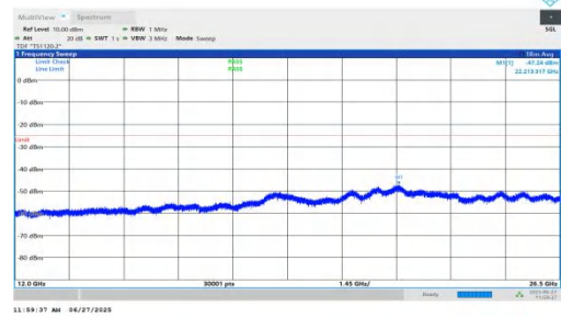
NTNV-n7-PC3-15-5-H-DFT-BPSK-Inner_1RB_Right-12000-26500- PASS
