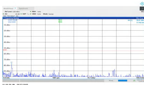
NTNV-n7-PC3-15-10-H-DFT-BPSK-Inner_1RB_Right-0.009-0.15-PASS
