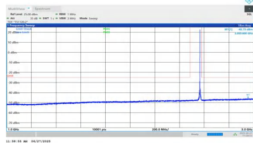
NTVN-n7-PC3-15-5-H-DFT-BPSK-Inner_1RB_Left-1000-3000-PA SS
