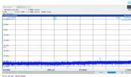
NTNV-n7-PC3-15-15-M-DFT-BPSK-Inner_1RB_Left-30-1000-PASS
