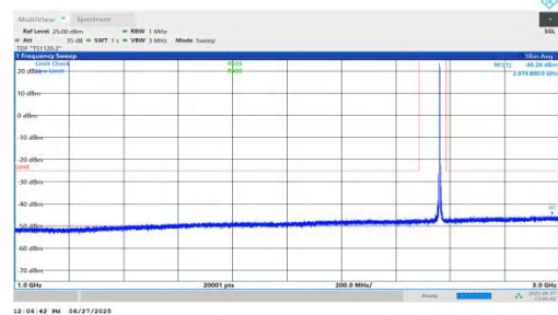
NTNV-n7-PC3-15-10-H-DFT-BPSK-Inner_1RB_Left-1000-3000-PASS
