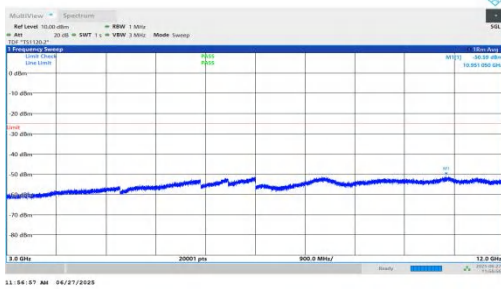
NTNV-n7-PC3-15-5-M-DFT-BPSK-Inner_1RB_Right-3000-12000 -PASS
