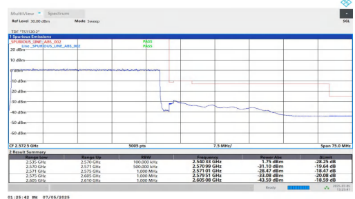
NTNV-n7-PC3-15-35-H-DFT-BPSK-Outer_Full-PASS
