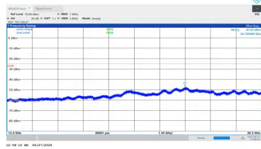
NTNV-n7-PC3-15-10-H-DFT-QPSK-Inner_1RB_Left-12000-26500-PASS
