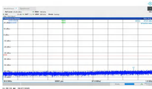
NTNV-n7-PC3-15-5-M-DFT-QPSK-Inner_1RB_Right-30-1000-PASS
