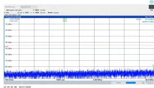
NTNV-n7-PC3-15-10-M-DFT-QPSK-Inner_1RB_Right-0.15-30-PA SS
