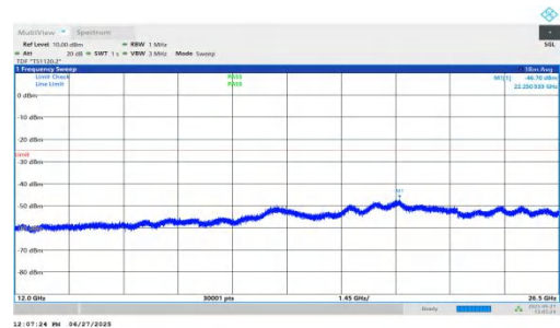
NTNV-n7-PC3-15-10-H-DFT-BPSK-Inner_1RB_Right-12000-2650 0-PASS
