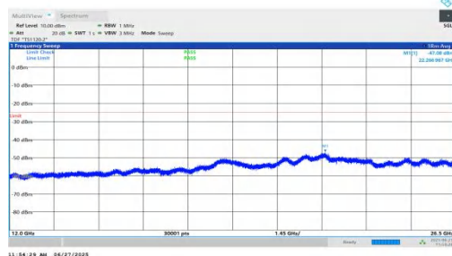
NTNV-n7-PC3-15-5-L-DFT-BPSK-Inner_1RB_Right-12000-26500- PASS
