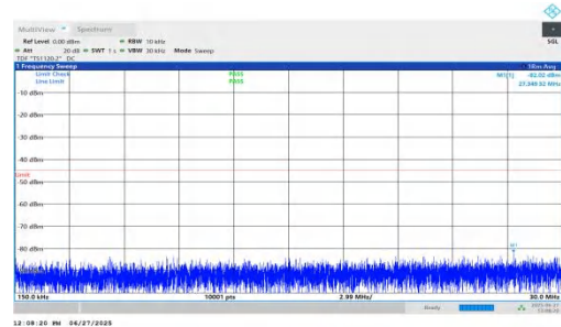
NTNV-n7-PC3-15-10-H-DFT-QPSK-Inner_1RB_Right-0.15-30-PA-SS
