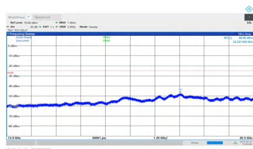
NTNV-n7-PC3-15-10-H-DFT-QPSK-Inner_1RB_Right-12000-26500-PASS
