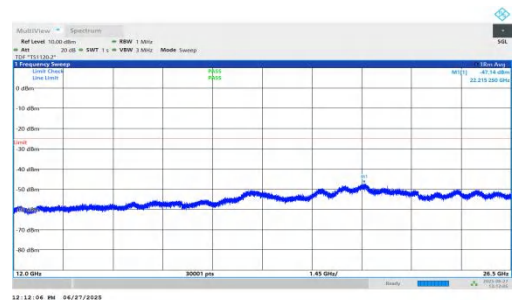
NTNV-n7-PC3-15-15-M-DFT-BPSK-Inner_1RB_Left-12000-26500-PASS
