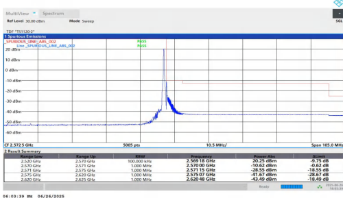
NTNV-n7-PC3-15-50-H-DFT-QPSK-Edge_1RB_Right-PASS
