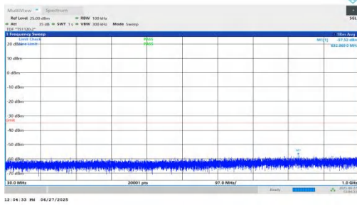
NTNV-n7-PC3-15-10-M-DFT-BPSK-Inner_1RB_Right-30-1000-P ASS
