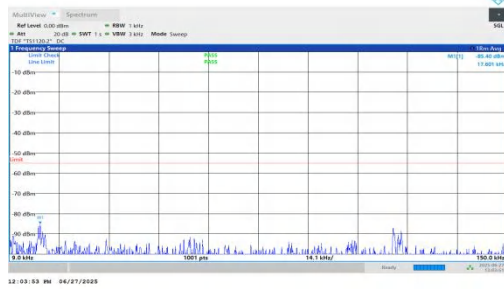
NTNV-n7-PC3-15-10-M-DFT-BPSK-Inner_1RB_Left-0.009-0.15-PASS
