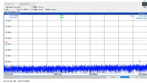
NTNV-n7-PC3-15-15-M-DFT-QPSK-Inner_1RB_Right-0.15-30-PA SS
