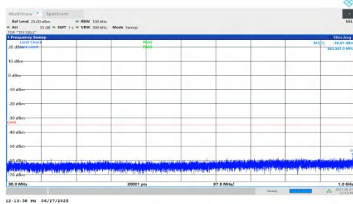
NTNV-n7-PC3-15-15-M-DFT-QPSK-Inner_1RB_Right-30-1000-P ASS
