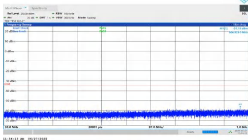
NTNV-n7-PC3-15-5-L-DFT-BPSK-Inner_1RB_Right-30-1000-PA SS
