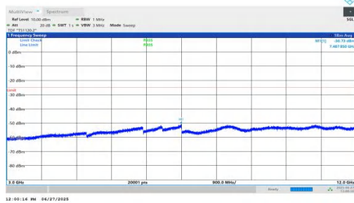
NTNV-n7-PC3-15-5-H-DFT-QPSK-Inner_1RB_Left-3000-12000-P ASS
