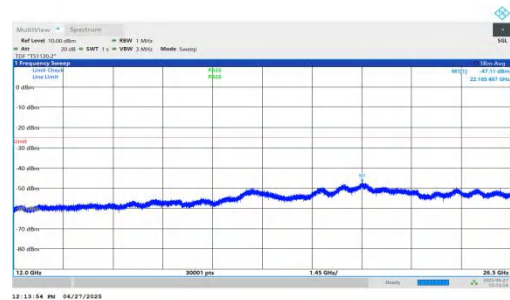
NTNV-n7-PC3-15-15-M-DFT-QPSK-Inner_1RB_Right-12000-2650 0-PASS
