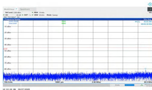
NTNV-n7-PC3-15-15-L-DFT-QPSK-Inner_1RB_Left-0.15-30-PASS
