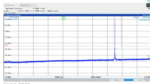
NTNV-n7-PC3-15-10-L-DFT-BPSK-Inner_1RB_Left-1000-3000-PASS
