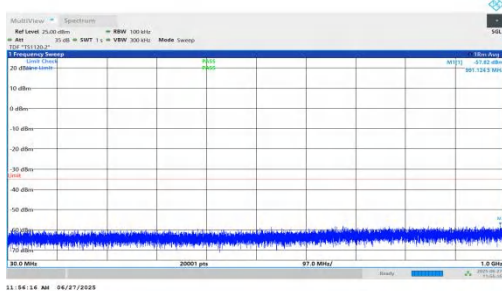
NTNV-n7-PC3-15-5-M-DFT-BPSK-Inner_1RB_Left-30-1000-PASS
