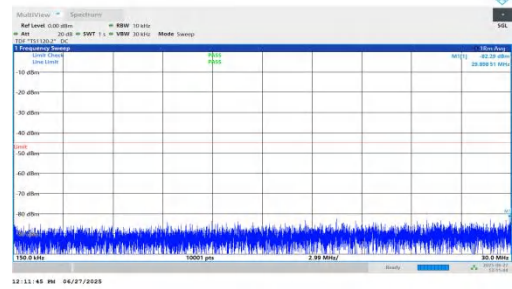
NTNV-n7-PC3-15-15-M-DFT-BPSK-Inner_1RB_Left-0.15-30-PASS
