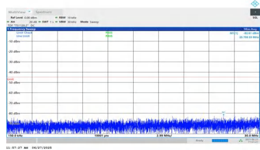
NTNV-n7-PC3-15-5-M-DFT-QPSK-Inner_1RB_Left-0.15-30-PASS
