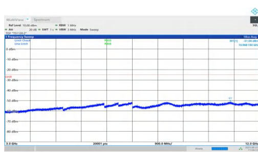
NTNV-n7-PC3-15-5-M-DFT-QPSK-Inner_1RB_Right-3000-12000-PASS
