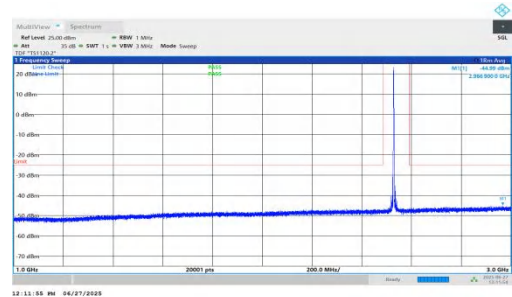
NTNV-n7-PC3-15-15-M-DFT-BPSK-Inner_1RB_Left-1000-3000-PASS
