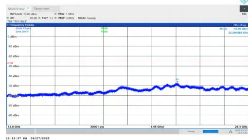
NTNV-n7-PC3-15-15-M-DFT-BPSK-Inner_1RB_Right-12000-26500-PASS
