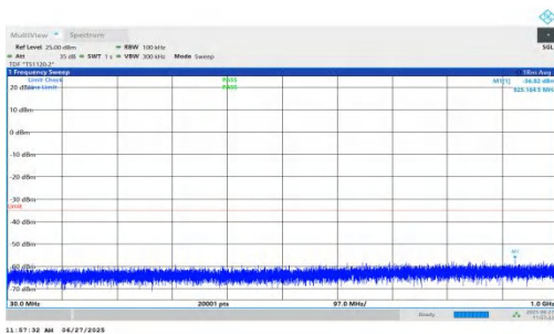
NTNV-n7-PC3-15-5-M-DFT-QPSK-Inner_1RB_Left-30-1000-PAS S
