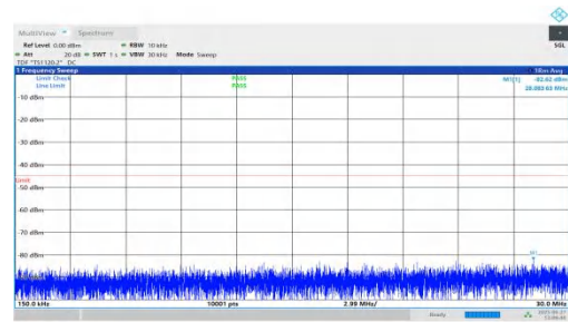
NTNV-n7-PC3-15-15-L-DFT-BPSK-Inner_1RB_Right-0.15-30-PASS
