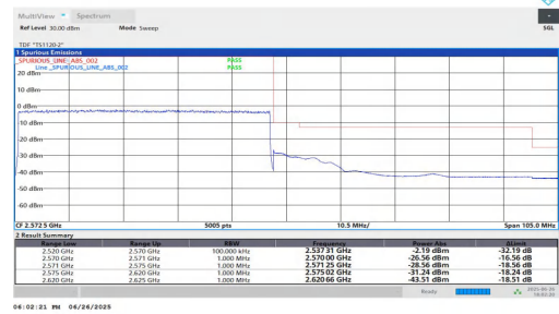
NTNV-n7-PC3-15-50-H-DFT-BPSK-Outer_Full-PASS
