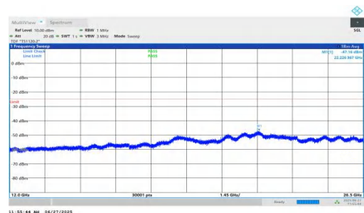
NTNV-n7-PC3-15-5-L-DFT-QPSK-Inner_1RB_Right-12000-26500- PASS
