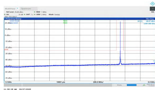
NTNV-n7-PC3-15-5-M-DFT-QPSK-Inner_1RB_Right-1000-3000-PASS
