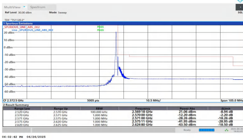
NTNV-n7-PC3-15-50-H-DFT-BPSK-Edge_1RB_Right-PASS
