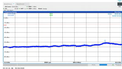
NTNV-n2-PC3-15-30-M-DFT-BPSK-Inner_1RB_Left-12000-20000-PASS PASS
