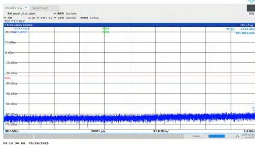
NTNV-n2-PC3-15-35-M-DFT-BPSK-Inner_1RB_Left-30-1000-PASS SS
