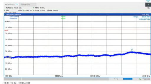
NTNV-n2-PC3-15-25-L-DFT-BPSK-Inner_1RB_Right-12000-2000 0-PASS
