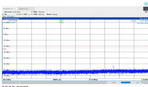
NTNV-n2-PC3-15-30-H-DFT-QPSK-Inner_1RB_Left-30-1000-P ASS
