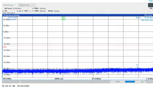
NTNV-n2-PC3-15-25-L-DFT-QPSK-Inner_1RB_Right-30-1000-PASS
