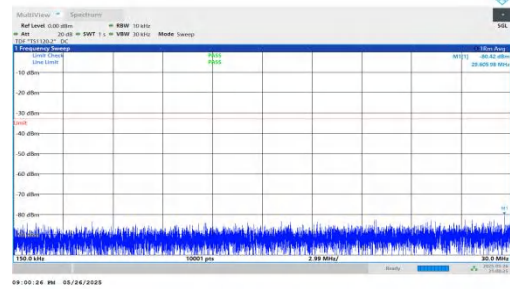
NTNV-n2-PC3-15-30-L-DFT-BPSK-Inner_1RB_Left-0.15-30-PASS
