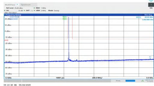
NTNV-n2-PC3-15-35-M-DFT-BPSK-Inner_1RB_Left-1000-3000-P ASS
