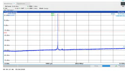
NTNV-n2-PC3-15-25-M-DFT-BPSK-Inner_1RB_Right-1000-3000-P PASS
