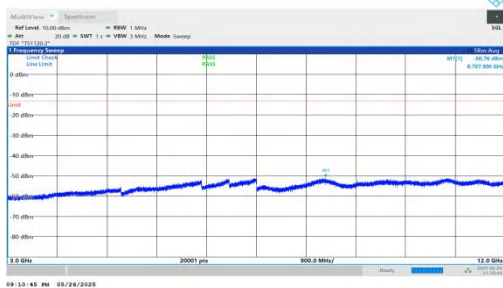
NTNV-n2-PC3-15-35-M-DFT-BPSK-Inner_1RB_Left-3000-12000-PASS
