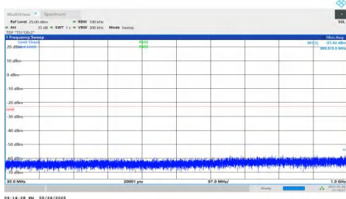
NTNV-n2-PC3-15-35-H-DFT-QPSK-Inner_1RB_Left-30-1000-P ASS
