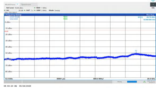
NTNV-n2-PC3-15-25-H-DFT-QPSK-Inner_1RB_Left-12000-20000-PASS
