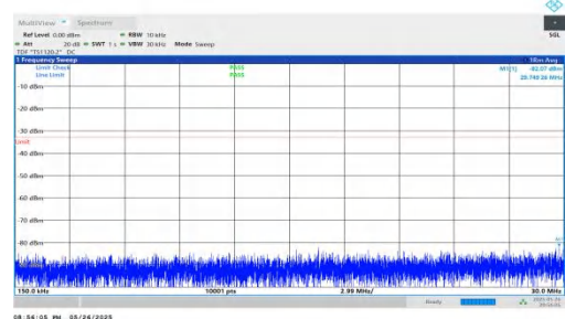
NTNV-n2-PC3-15-25-M-DFT-BPSK-Inner_1RB_Right-0.15-30-PASS SS
