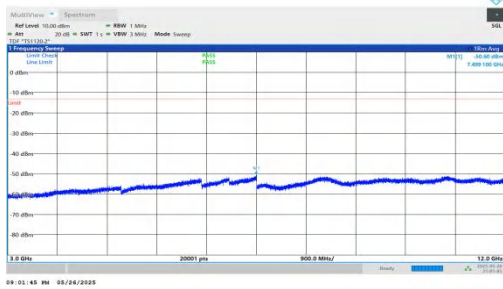
NTNV-n2-PC3-15-30-L-DFT-QPSK-Inner_1RB_Left-3000-12000-PASS
