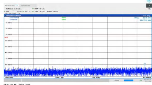
NTNV-n2-PC3-15-35-M-DFT-BPSK-Inner_1RB_Right-0.15-30-PASS SS
