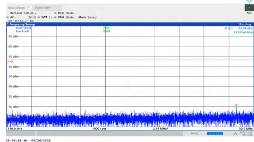
NTNV-n2-PC3-15-25-L-DFT-QPSK-Inner_1RB_Right-0.15-30-PASS
