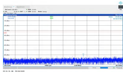
NTNV-n2-PC3-15-30-L-DFT-QPSK-Inner_1RB_Left-0.15-30-PASS
