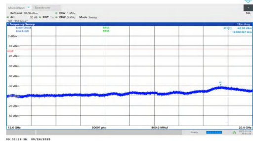
NTNV-n2-PC3-15-30-L-DFT-BPSK-Inner_1RB_Right-12000-2000 0-PASS
