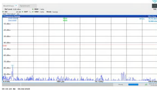
NTNV-n2-PC3-15-30-M-DFT-BPSK-Inner_1RB_Right-0.009-0.15 -PASS
