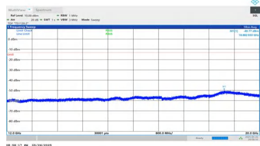
NTNV-n2-PC3-15-25-H-DFT-BPSK-Inner_1RB_Left-12000-20000-PASS
