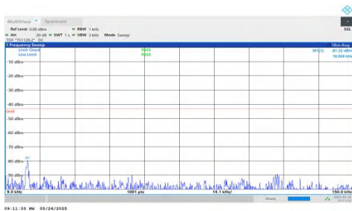
NTNV-n2-PC3-15-35-M-DFT-QPSK-Inner_1RB_Left-0.009-0.15- PASS
