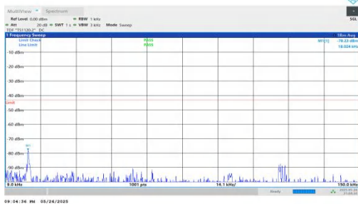
NTNV-n2-PC3-15-30-M-DFT-QPSK-Inner_1RB_Right-0.009-0.15 -PASS
