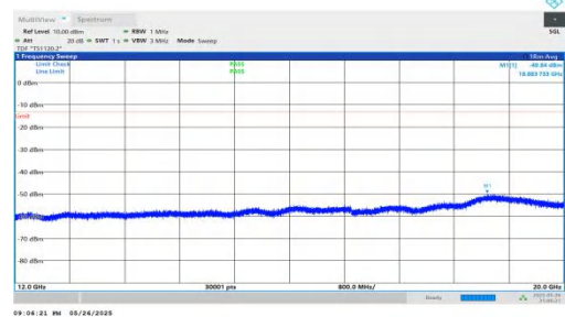
NTNV-n2-PC3-15-30-H-DFT-BPSK-Inner_1RB_Right-12000-20000 PASS
