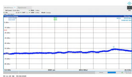
NTNV-n2-PC3-15-35-M-DFT-BPSK-Inner_1RB_Right-12000-2000 0-PASS
