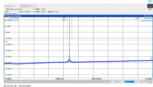
NTNV-n2-PC3-15-30-L-DFT-QPSK-Inner_1RB_Right-1000-3000-PASS
