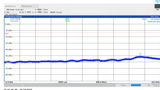
NTNV-n2-PC3-15-30-L-DFT-BPSK-Inner_1RB_Left-12000-20000-PASS
