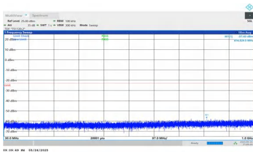
NTNV-n2-PC3-15-35-L-DFT-QPSK-Inner_1RB_Right-30-1000-PASS
