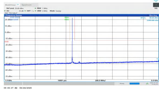
NTNV-n2-PC3-15-30-H-DFT-BPSK-Inner_1RB_Left-1000-3000-P ASS
