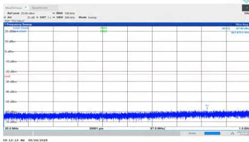
NTNV-n2-PC3-15-35-H-DFT-BPSK-Inner_1RB_Left-30-1000-PASS
