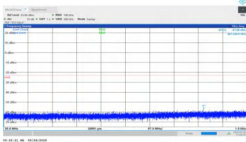
NTNV-n2-PC3-15-30-L-DFT-QPSK-Inner_1RB_Right-30-1000-PASS
