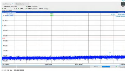
NTNV-n2-PC3-15-30-H-DFT-BPSK-Inner_1RB_Left-30-1000-PASS
