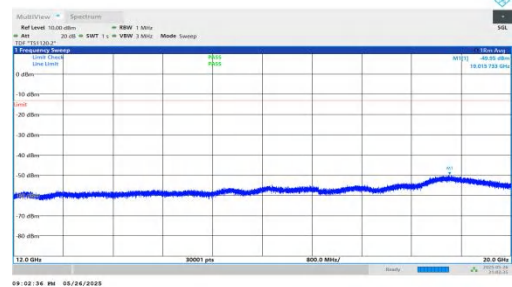
NTNV-n2-PC3-15-30-L-DFT-QPSK-Inner_1RB_Right-12000-20000-PASS
