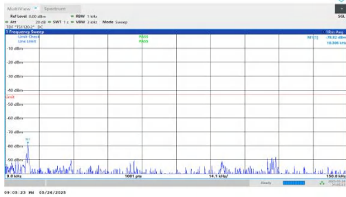
NTNV-n2-PC3-15-30-H-DFT-BPSK-Inner_1RB_Left-0.009-0.15-P ASS
