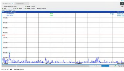
NTNV-n2-PC3-15-35-M-DFT-BPSK-Inner_1RB_Left-0.009-0.15-P ASS
