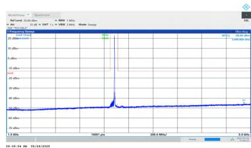
NTNV-n2-PC3-15-35-L-DFT-QPSK-Inner_1RB_Right-1000-3000-PASS
