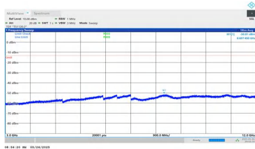
NTNV-n2-PC3-15-25-M-DFT-BPSK-Inner_1RB_Right-3000-1200 0-PASS
