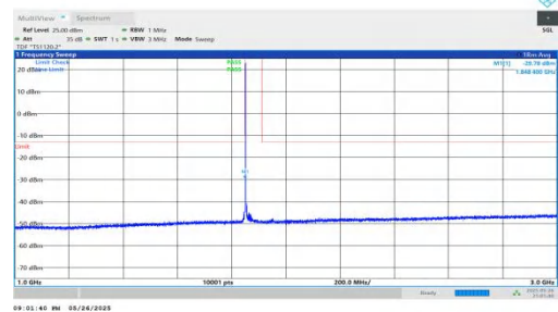
NTNV-n2-PC3-15-30-L-DFT-QPSK-Inner_1RB_Left-1000-3000-PA SS
