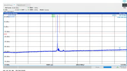
NTNV-n2-PC3-15-35-H-DFT-QPSK-Inner_1RB_Left-1000-3000-P ASS
