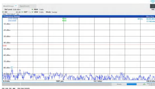
NTNV-n2-PC3-15-30-H-DFT-QPSK-Inner_1RB_Left-0.009-0.15-P ASS
