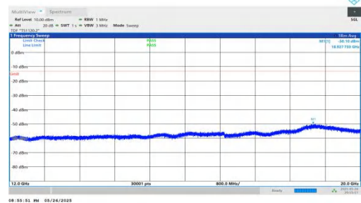
NTNV-n2-PC3-15-25-M-DFT-BPSK-Inner_1RB_Left-12000-20000-PASS PASS
