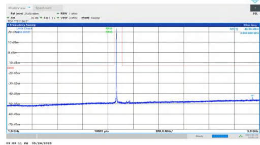
NTNV-n2-PC3-15-30-M-DFT-BPSK-Inner_1RB_Left-1000-3000-P ASS
