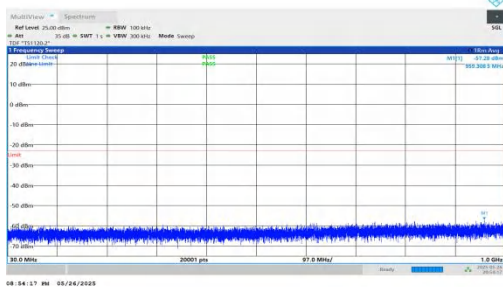
NTNV-n2-PC3-15-25-L-DFT-QPSK-Inner_1RB_Left-30-1000-PA SS
