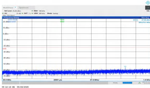
NTNV-n2-PC3-15-35-M-DFT-QPSK-Inner_1RB_Right-30-1000-P ASS
