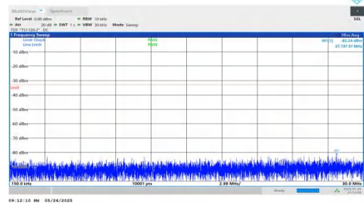
NTNV-n2-PC3-15-35-M-DFT-QPSK-Inner_1RB_Right-0.15-30-PA SS
