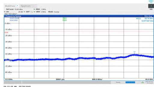
NTNV-n2-PC3-15-35-H-DFT-BPSK-Inner_1RB_Left-12000-20000-PASS
