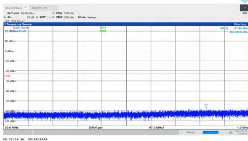
NTNV-n2-PC3-15-30-M-DFT-BPSK-Inner_1RB_Left-30-1000-PASS SS
