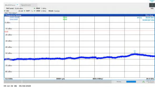
NTNV-n2-PC3-15-35-M-DFT-QPSK-Inner_1RB_Right-12000-2000 0-PASS
