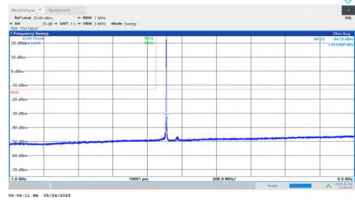
NTNV-n2-PC3-15-30-H-DFT-BPSK-Inner_1RB_Right-1000-3000-P PASS
