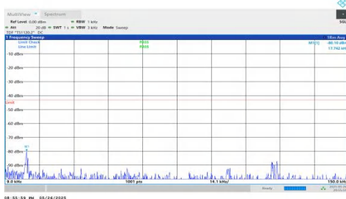
NTNV-n2-PC3-15-25-M-DFT-BPSK-Inner_1RB_Right-0.009-0.15 -PASS
