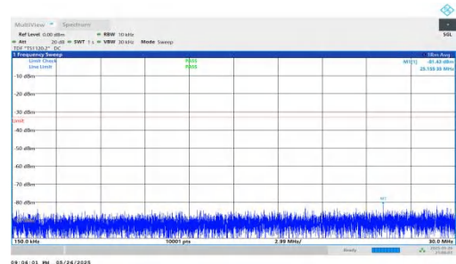
NTNV-n2-PC3-15-30-H-DFT-BPSK-Inner_1RB_Right-0.15-30-PASS
