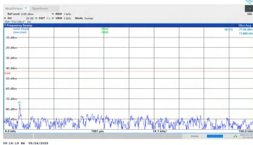
NTNV-n2-PC3-15-35-H-DFT-QPSK-Inner_1RB_Left-0.009-0.15-P ASS
