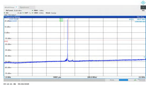
NTNV-n2-PC3-15-35-M-DFT-QPSK-Inner_1RB_Right-1000-3000- PASS
