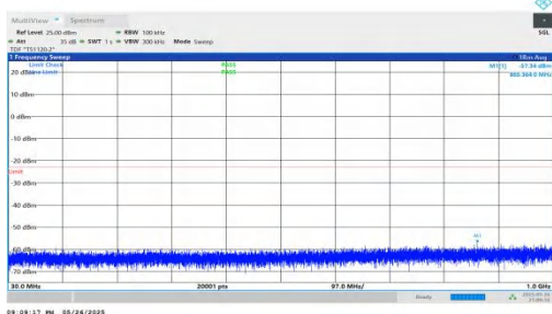
NTNV-n2-PC3-15-35-L-DFT-QPSK-Inner_1RB_Left-30-1000-PA SS
