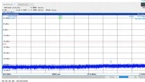
NTNV-n2-PC3-15-25-M-DFT-BPSK-Inner_1RB_Left-30-1000-PASS SS
