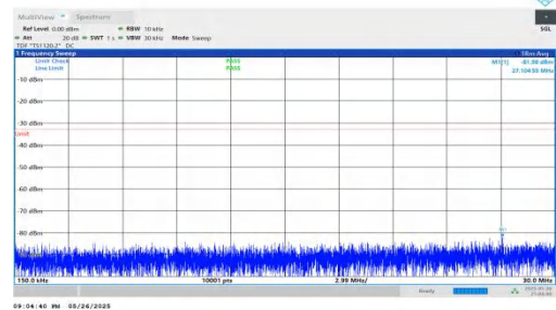
NTNV-n2-PC3-15-30-M-DFT-QPSK-Inner_1RB_Right-0.15-30-PA SS
