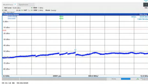
NTNV-n2-PC3-15-30-L-DFT-BPSK-Inner_1RB_Right-3000-12000 -PASS
