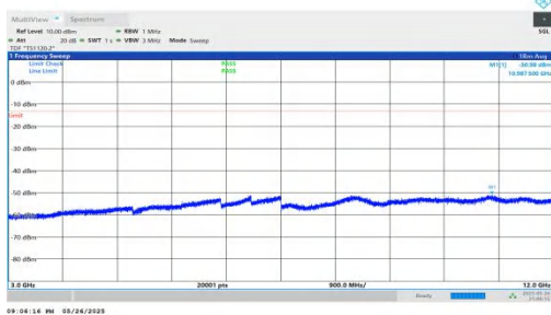
NTNV-n2-PC3-15-30-H-DFT-BPSK-Inner_1RB_Right-3000-12000 PASS
