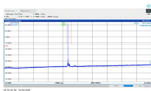
NTNV-n2-PC3-15-25-M-DFT-QPSK-Inner_1RB_Left-1000-3000-P ASS
