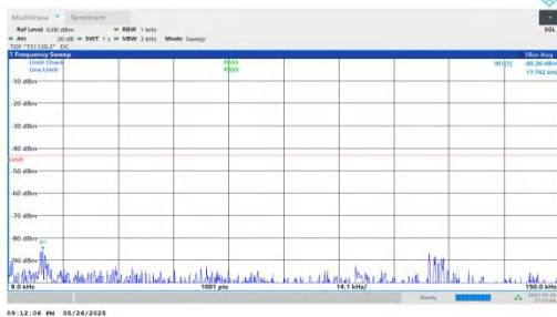
NTNV-n2-PC3-15-35-M-DFT-QPSK-Inner_1RB_Right-0.009-0.15 -PASS
