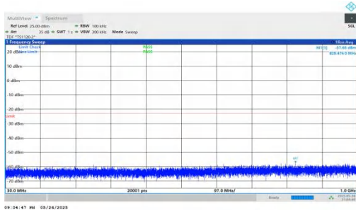
NTNV-n2-PC3-15-30-M-DFT-QPSK-Inner_1RB_Right-30-1000-P ASS
