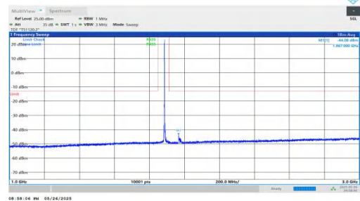
NTNV-n2-PC3-15-25-H-DFT-BPSK-Inner_1RB_Left-1000-3000-PASS
