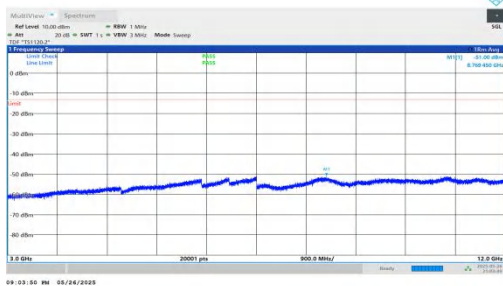
NTNV-n2-PC3-15-30-M-DFT-BPSK-Inner_1RB_Right-3000-12000-PASS
