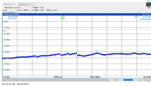
NTNV-n2-PC3-15-30-M-DFT-QPSK-Inner_1RB_Left-3000-12000 -PASS
