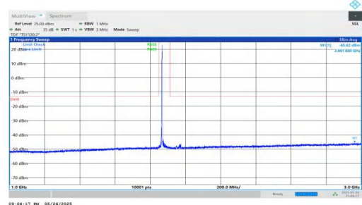
NTNV-n2-PC3-15-30-M-DFT-QPSK-Inner_1RB_Left-1000-3000-PASS
