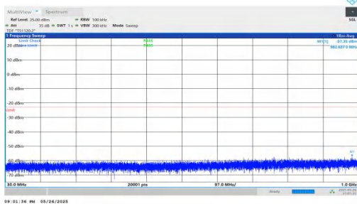
NTNV-n2-PC3-15-30-L-DFT-QPSK-Inner_1RB_Left-30-1000-PA SS
