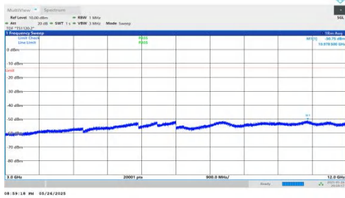
NTNV-n2-PC3-15-25-H-DFT-QPSK-Inner_1RB_Left-3000-12000-PASS
