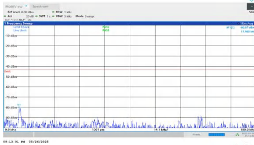
NTNV-n2-PC3-15-35-H-DFT-BPSK-Inner_1RB_Left-0.009-0.15-P ASS
