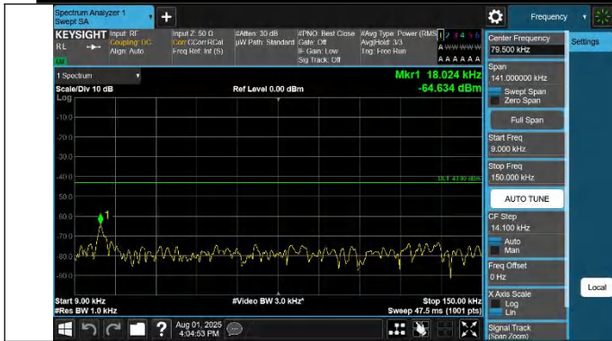
42-42-20MHz-20MHz-QPSK-QPSK-42491-42689-1RB#0-1RB#9 9-0.009~0.15MHz-PASS
