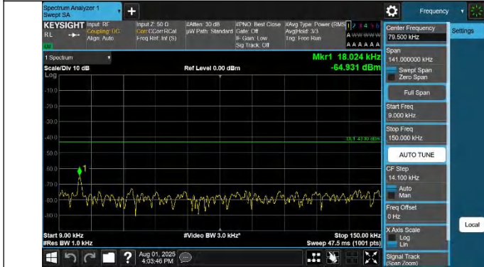
42-42-20MHz-20MHz-QPSK-QPSK-42190-42388-1RB#0-0RB#0- 0.009~0.15MHz-PASS
