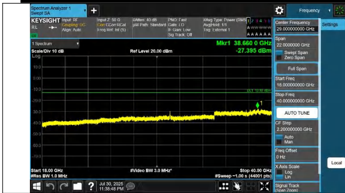
42-42-20MHz-20MHz-QPSK-QPSK-42190-42388-1RB#99-0RB#0-18000~40000MHz-PASS
