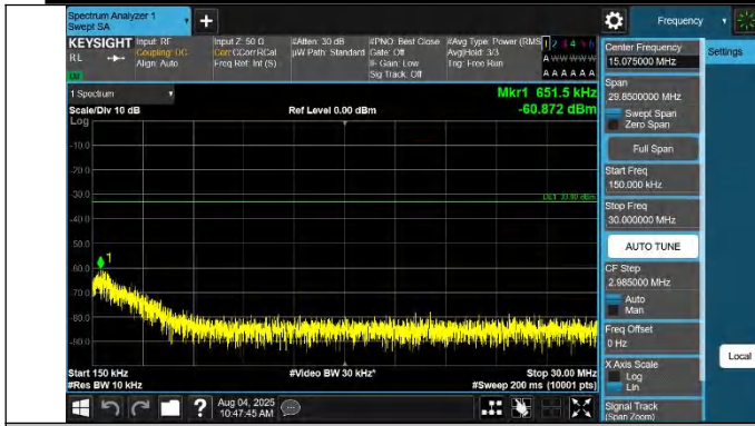
42-42-20MHz-15MHz-QPSK-QPSK-42841-43012-1RB#0-0RB#0-0.15~30MHz-PASS
