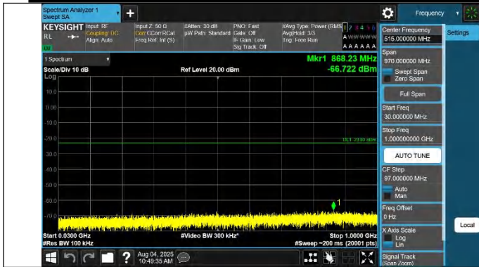
42-42-20MHz-15MHz-QPSK-QPSK-42841-43012-1RB#0-1RB#7 4-30~1000MHz-PASS
