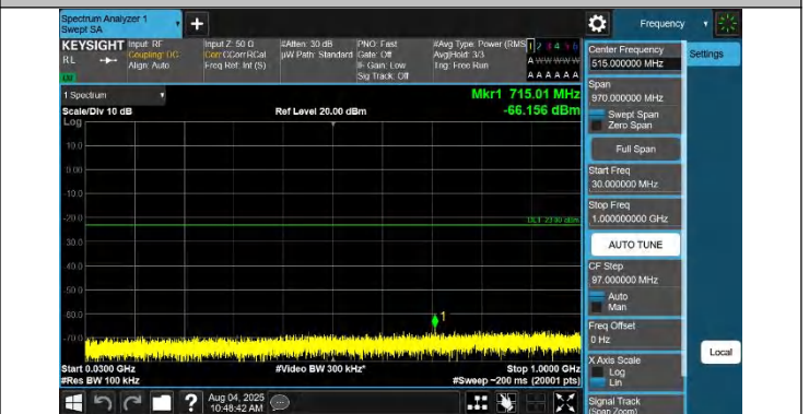
42-42-20MHz-15MHz-QPSK-QPSK-42841-43012-1RB#99-0RB# 0-30~1000MHz-PASS
