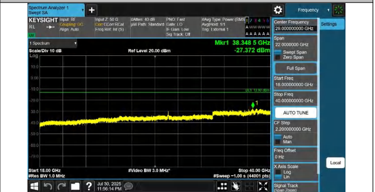
42-42-20MHz-20MHz-QPSK-QPSK-42792-42990-1RB#0-1RB#9 9-18000~40000MHz-PASS
