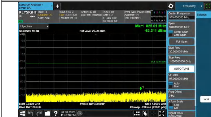
42-42-20MHz-20MHz-QPSK-QPSK-42491-42689-1RB#0-1RB#9 9-30~1000MHz-PASS
