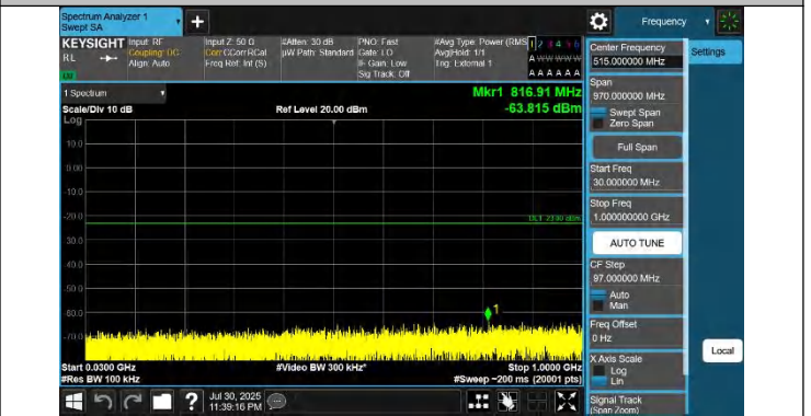
42-42-20MHz-20MHz-QPSK-QPSK-42190-42388-1RB#0-1RB#99-0.30~1000MHz-PASS
