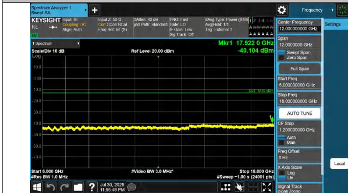
42-42-20MHz-20MHz-QPSK-QPSK-42792-42990-1RB#0-1RB#9 9-6000~18000MHz-PASS
