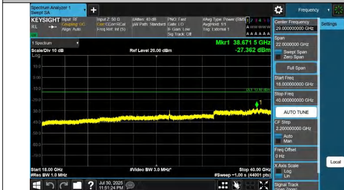
42-42-20MHz-20MHz-QPSK-QPSK-42792-42990-1RB#0-0RB#0-18000~40000MHz-PASS
