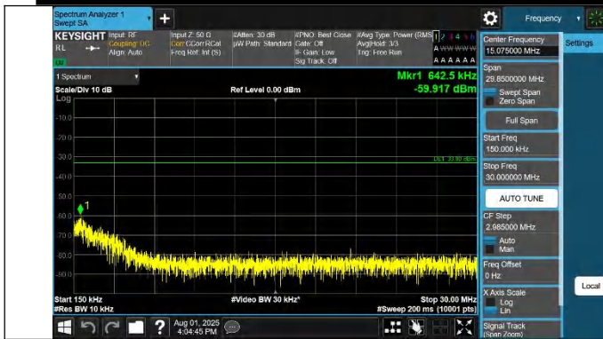
42-42-20MHz-20MHz-QPSK-QPSK-42491-42689-1RB#99-0RB# 0-0.15~30MHz-PASS
