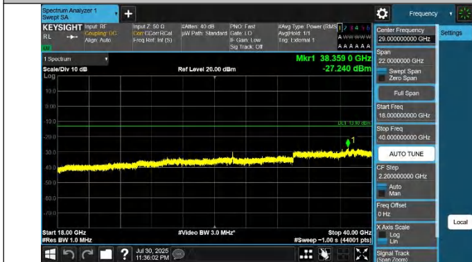
42-42-20MHz-20MHz-QPSK-QPSK-42190-42388-1RB#0-0RB#0-18000~40000MHz-PASS
