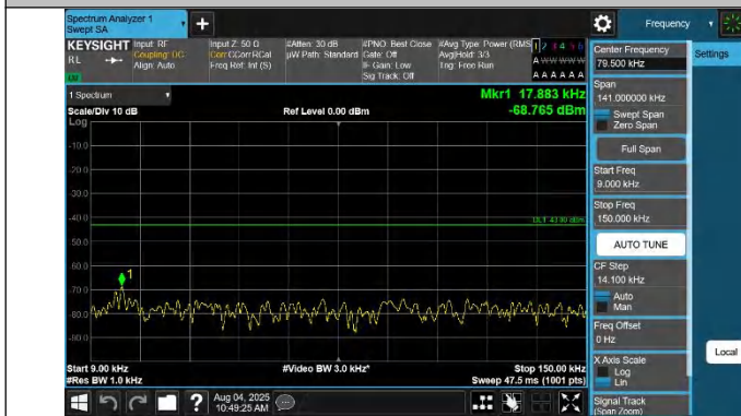
42-42-20MHz-15MHz-QPSK-QPSK-42841-43012-1RB#0-1RB#74-0.009~0.15MHz-PASS
