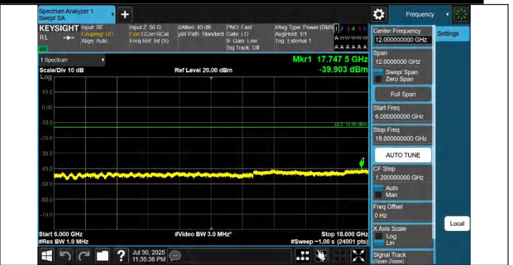
42-42-20MHz-20MHz-QPSK-QPSK-42190-42388-1RB#0-0RB#0-6000~18000MHz-PASS
