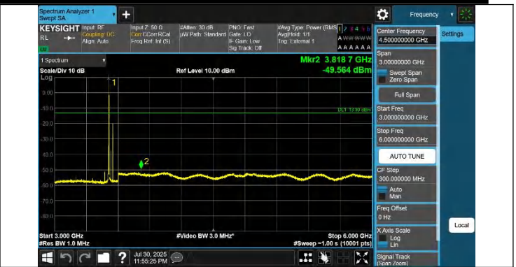
42-42-20MHz-20MHz-QPSK-QPSK-42792-42990-1RB#0-1RB#9 9-3000~6000MHz-PASS
