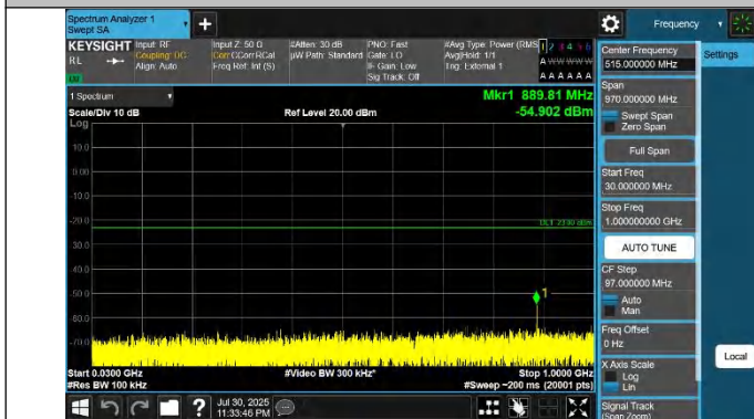
42-42-20MHz-20MHz-QPSK-QPSK-42190-42388-1RB#0-0RB#0- 30~1000MHz-PASS
