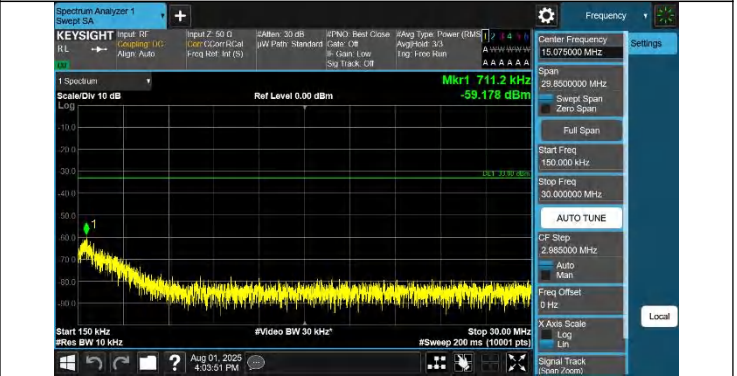
42-42-20MHz-20MHz-QPSK-QPSK-42190-42388-1RB#0-0RB#0- 0.15~30MHz-PASS
