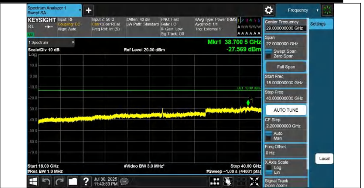
42-42-20MHz-20MHz-QPSK-QPSK-42190-42388-1RB#0-1RB#9 9-18000~40000MHz-PASS
