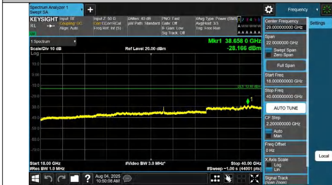
42-42-20MHz-15MHz-QPSK-QPSK-42841-43012-1RB#0-1RB#7 4-18000~40000MHz-PASS
