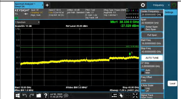
42-42-20MHz-20MHz-QPSK-QPSK-42491-42689-1RB#99-0RB# 0-18000~40000MHz-PASS
