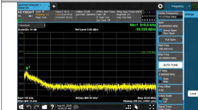
42-42-20MHz-15MHz-QPSK-QPSK-42841-43012-1RB#99-0RB# 0-0.15~30MHz-PASS
