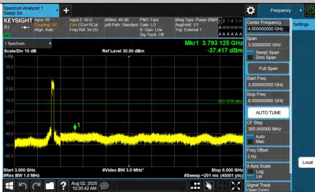
Band42(3450-3550)-20MHz-QPSK-42990-1RB#0-3000~6000-PA
