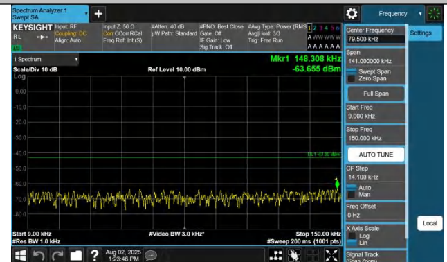
Band42(3450-3550)-10MHz-QPSK-42590-1RB#49-0.009~0.15-PA
