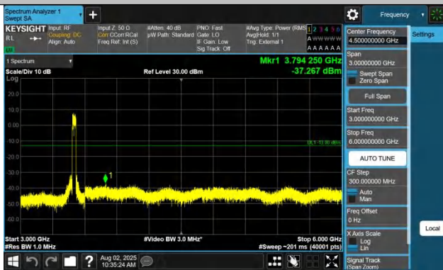
Band42(3450-3550)-20MHz-QPSK-42590-1RB#0-3000~6000-PA
