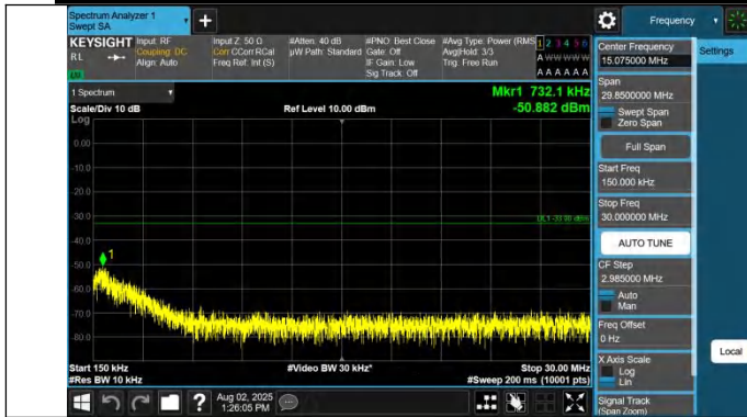
Band42(3450-3550)-20MHz-QPSK-42590-1RB#99-0.15~30-PAS
