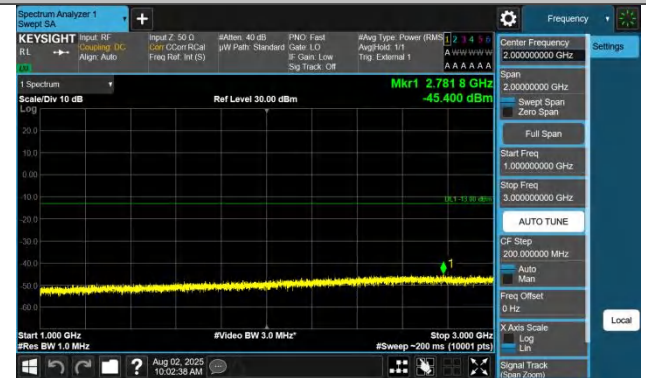
Band42(3450-3550)-20MHz-QPSK-42990-1RB#0-1000~3000-PAS
