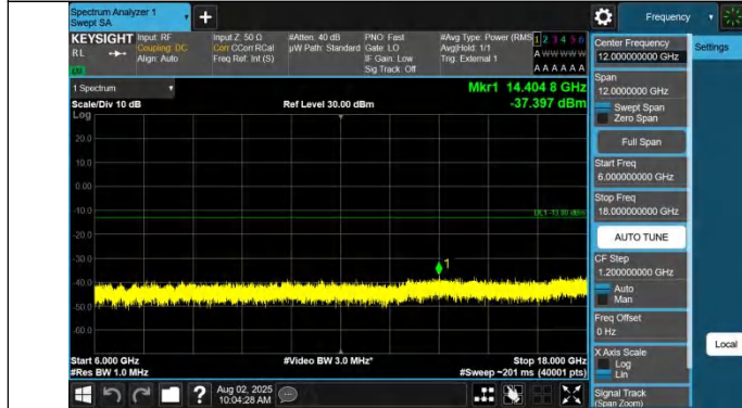
Band42(3450-3550)-20MHz-QPSK-42990-1RB#99-6000~18000-P ASS
