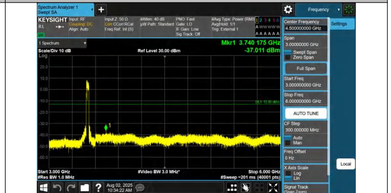
Band42(3450-3550)-15MHz-QPSK-42165-1RB#74-3000~6000-PA
