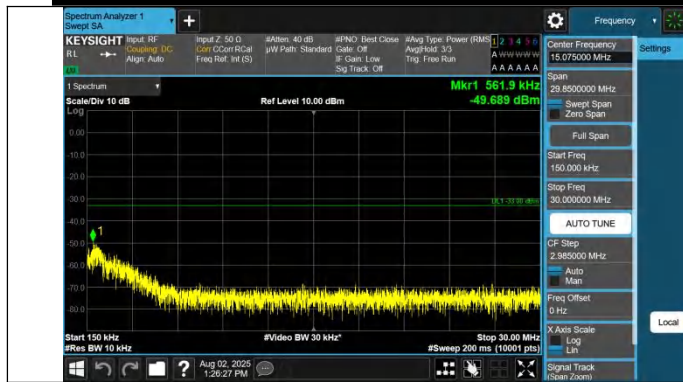
Band42(3450-3550)-20MHz-QPSK-42990-1RB#99-0.15~30-PAS S
