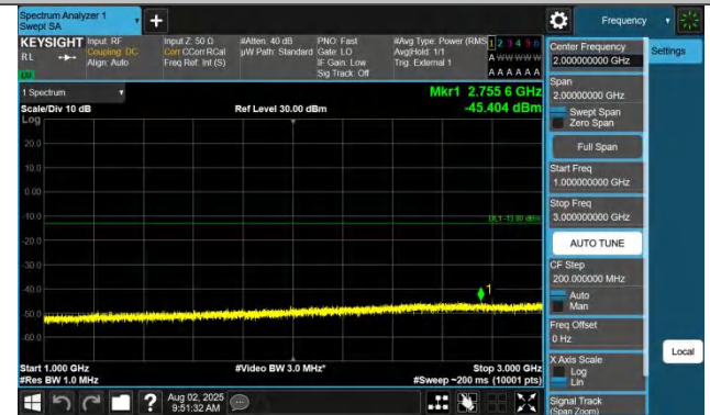
Band42(3450-3550)-15MHz-QPSK-42590-1RB#0-1000~3000-PAS
