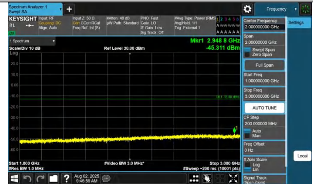
Band42(3450-3550)-10MHz-QPSK-43040-1RB#0-1000~3000-PAS
