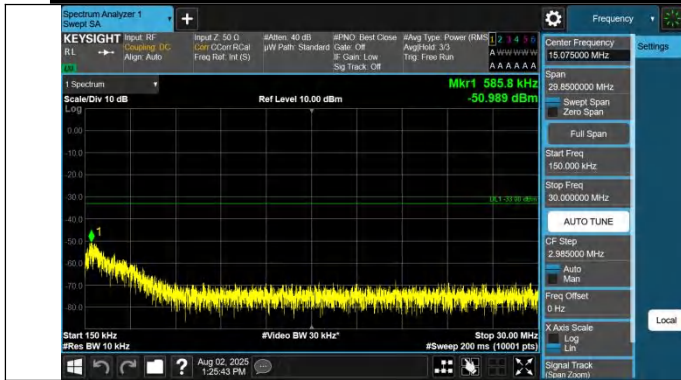
Band42(3450-3550)-20MHz-QPSK-42190-1RB#99-0.15~30-PAS S
