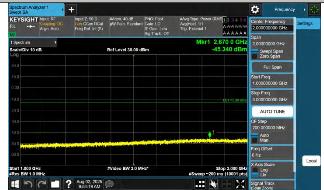
Band42(3450-3550)-15MHz-QPSK-43015-1RB#0-1000~3000-PAS
