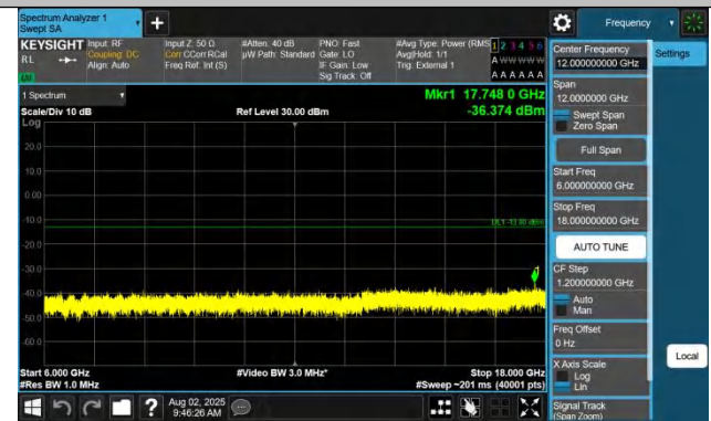
Band42(3450-3550)-10MHz-QPSK-43040-1RB#0-6000~18000-PA
