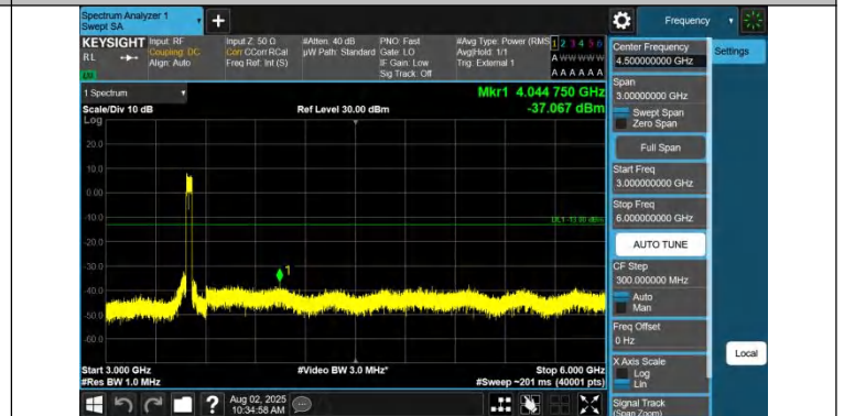
Band42(3450-3550)-15MHz-QPSK-43015-1RB#74-3000~6000-PA SS
