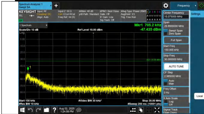
Band42(3450-3550)-15MHz-QPSK-42590-1RB#74-0.15~30-PAS
