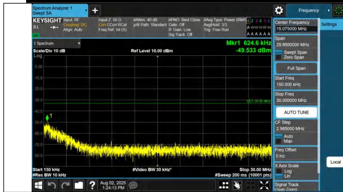
Band42(3450-3550)-10MHz-QPSK-43040-1RB#49-0.15~30-PAS S
