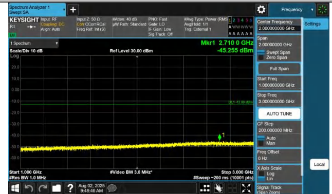
Band42(3450-3550)-15MHz-QPSK-42165-1RB#0-1000~3000-PAS
