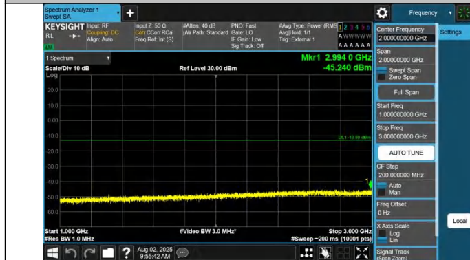
Band42(3450-3550)-15MHz-QPSK-43015-1RB#74-1000~3000-P ASS
