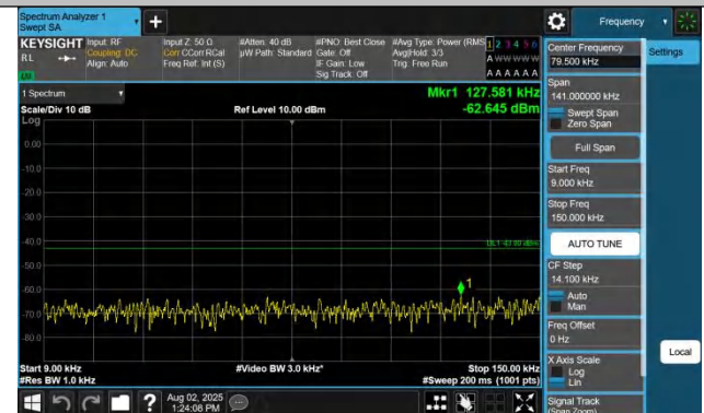
Band42(3450-3550)-10MHz-QPSK-43040-1RB#49-0.009~0.15-PA
