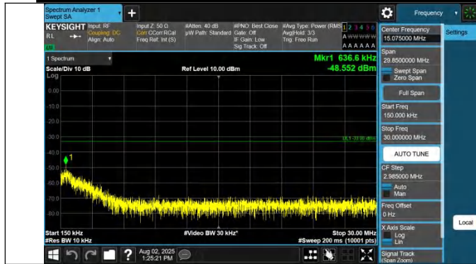
Band42(3450-3550)-15MHz-QPSK-43015-1RB#74-0.15~30-PAS S
