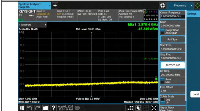
Band42(3450-3550)-20MHz-QPSK-42590-1RB#99-1000~3000-P
