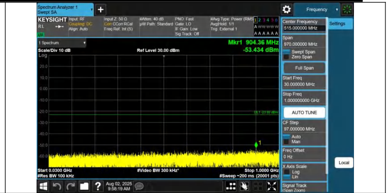
Band42(3450-3550)-20MHz-QPSK-42190-1RB#99-30~1000-PASS
