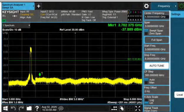
Band42(3450-3550)-10MHz-QPSK-43040-1RB#0-3000~6000-PA
