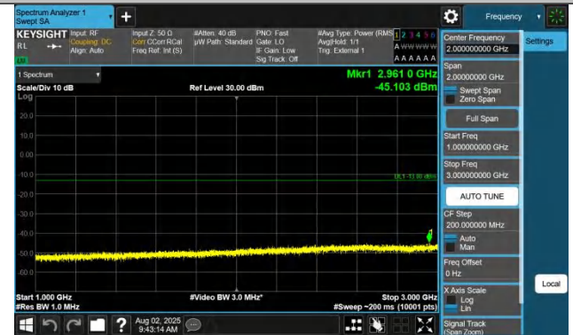
Band42(3450-3550)-10MHz-QPSK-42590-1RB#0-1000~3000-PAS
