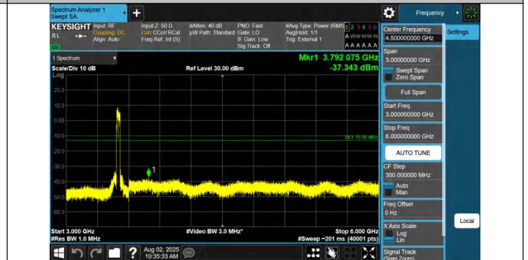
Band42(3450-3550)-20MHz-QPSK-42590-1RB#99-3000~6000-PA
