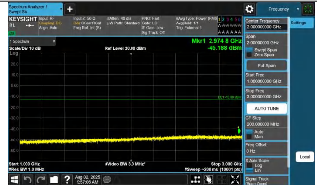
Band42(3450-3550)-20MHz-QPSK-42190-1RB#0-1000~3000-PAS
