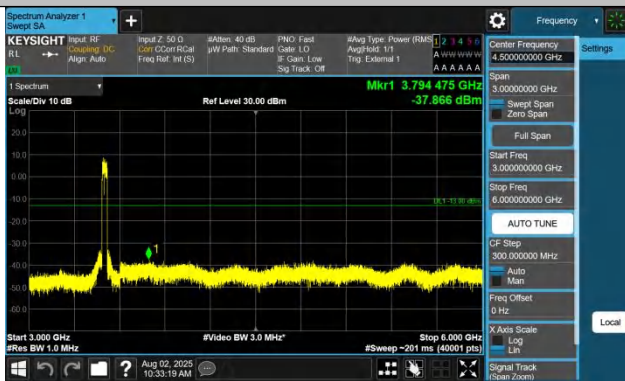
Band42(3450-3550)-10MHz-QPSK-42140-1RB#0-3000~6000-PA
