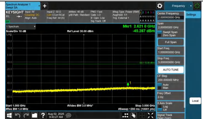
Band42(3450-3550)-10MHz-QPSK-42140-1RB#0-1000~3000-PAS
