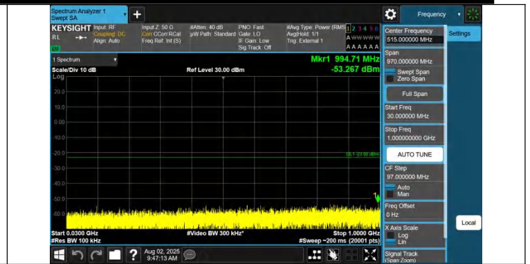
Band42(3450-3550)-10MHz-QPSK-43040-1RB#49-30~1000-PASS
