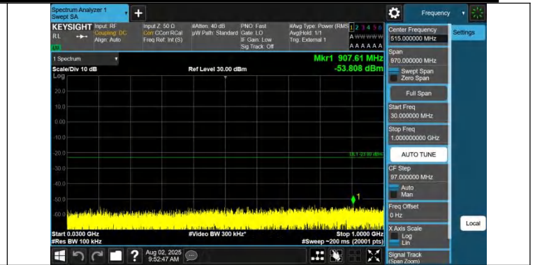
Band42(3450-3550)-15MHz-QPSK-42590-1RB#74-30~1000-PASS
