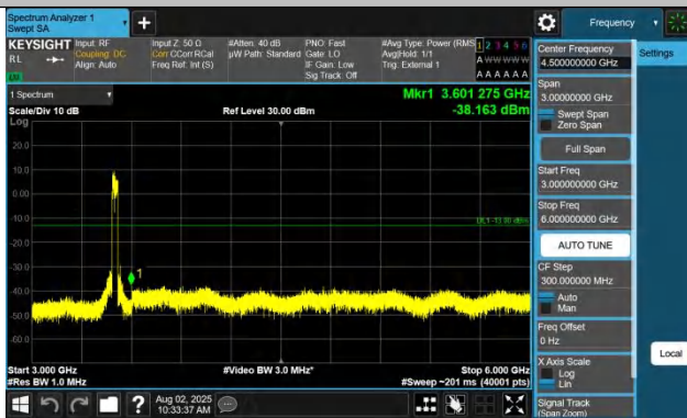
Band42(3450-3550)-10MHz-QPSK-42590-1RB#0-3000~6000-PA
