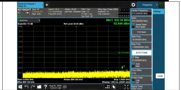
Band42(3450-3550)-20MHz-QPSK-42990-1RB#99-30~1000-PASS
