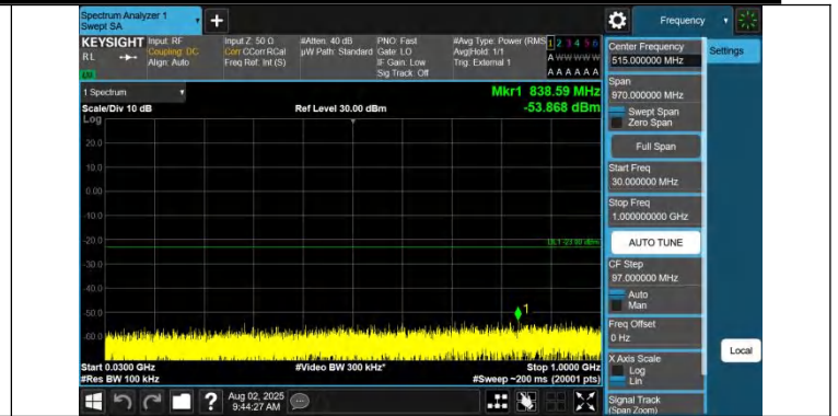
Band42(3450-3550)-10MHz-QPSK-42590-1RB#49-30~1000-PASS
