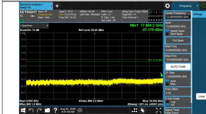
Band42(3450-3550)-10MHz-QPSK-43040-1RB#49-6000~18000-P ASS
