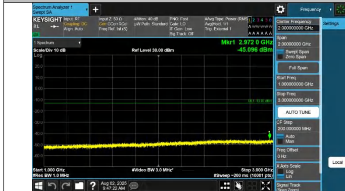
Band42(3450-3550)-10MHz-QPSK-43040-1RB#49-1000~3000-P ASS
