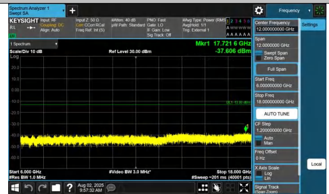
Band42(3450-3550)-20MHz-QPSK-42190-1RB#0-6000~18000-PA
