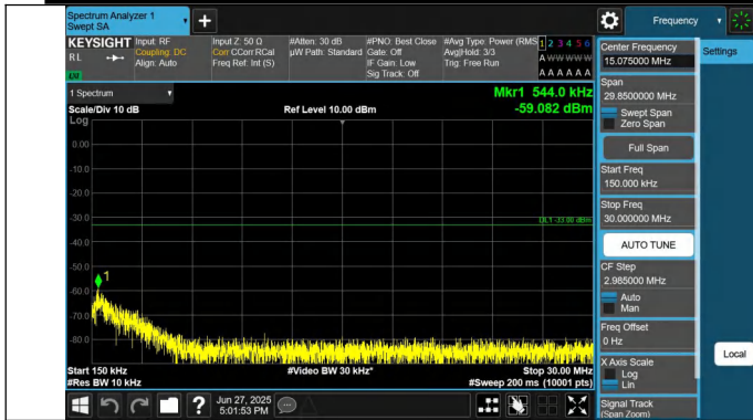
66-66-20MHz-15MHz-QPSK-QPSK-132072-132243-1RB#0-1RB #74-0.15~30MHz-PASS
