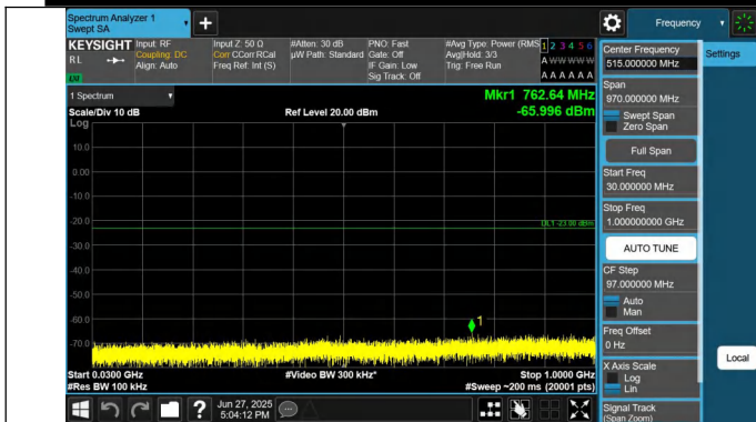
66-66-20MHz-15MHz-QPSK-QPSK-132348-132519-1RB#0-1RB #74-30~1000MHz-PASS
