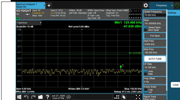
66-66-20MHz-15MHz-QPSK-QPSK-132423-132594-1RB#0-0RB #0-0.009~0.15MHz-PASS
