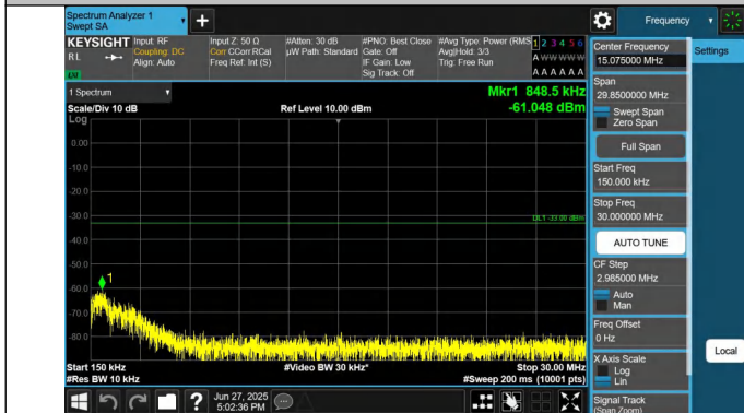
66-66-20MHz-15MHz-QPSK-QPSK-132348-132519-1RB#0-0RB #0-0.15~30MHz-PASS
