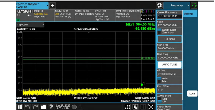
66-66-20MHz-15MHz-QPSK-QPSK-132348-132519-1RB#0-0RB #0-30~1000MHz-PASS
