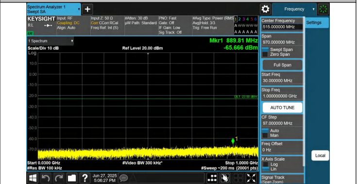
66-66-20MHz-15MHz-QPSK-QPSK-132423-132594-1RB#0-1RB #74-30~1000MHz-PASS
