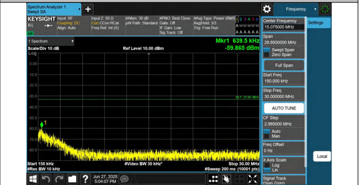
66-66-20MHz-15MHz-QPSK-QPSK-132348-132519-1RB#0-1RB #74-0.15~30MHz-PASS
