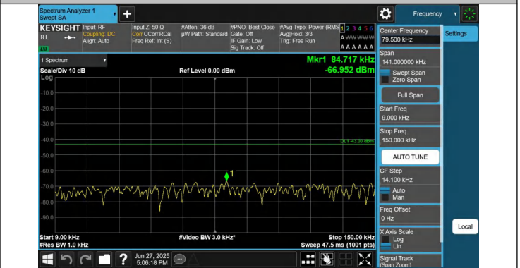
66-66-20MHz-15MHz-QPSK-QPSK-132423-132594-1RB#0-1RB #74-0.009~0.15MHz-PASS
