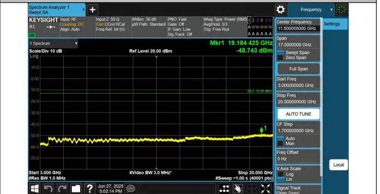
66-66-20MHz-15MHz-QPSK-QPSK-132072-132243-1RB#0-1RB #74-3000~20000MHz-PASS
