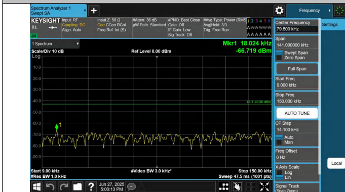
66-66-20MHz-15MHz-QPSK-QPSK-132072-132243-1RB#0-0RB #0-0.009~0.15MHz-PASS
