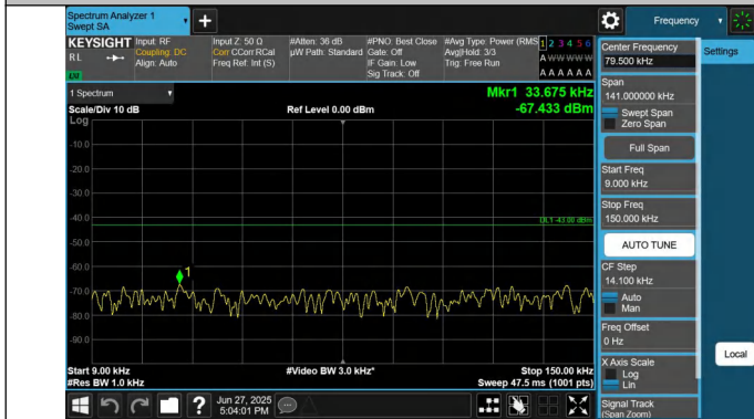
66-66-20MHz-15MHz-QPSK-QPSK-132348-132519-1RB#0-1RB #74-0.009~0.15MHz-PASS
