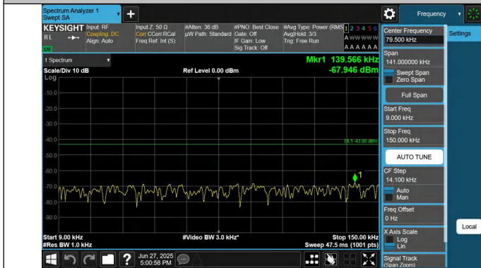
66-66-20MHz-15MHz-QPSK-QPSK-132072-132243-1RB#99-0R B#0-0.009~0.15MHz-PASS
