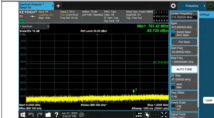
66-66-20MHz-15MHz-QPSK-QPSK-132423-132594-1RB#0-0RB #0-30~1000MHz-PASS
