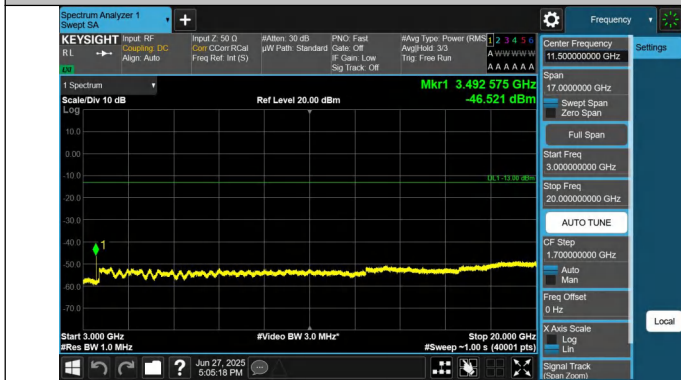
66-66-20MHz-15MHz-QPSK-QPSK-132423-132594-1RB#0-0RB #0-3000~20000MHz-PASS
