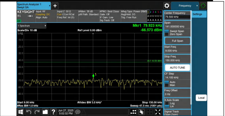
66-66-20MHz-15MHz-QPSK-QPSK-132348-132519-1RB#0-0RB #0-0.009~0.15MHz-PASS
