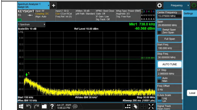
66-66-20MHz-15MHz-QPSK-QPSK-132423-132594-1RB#0-1RB #74-0.15~30MHz-PASS
