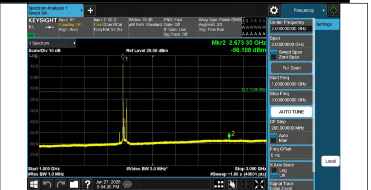
66-66-20MHz-15MHz-QPSK-QPSK-132348-132519-1RB#0-1RB #74-1000~3000MHz-PASS
