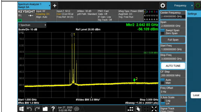
66-66-20MHz-15MHz-QPSK-QPSK-132072-132243-1RB#0-1RB #74-1000~3000MHz-PASS
