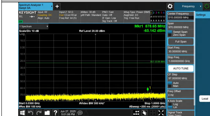
66-66-20MHz-15MHz-QPSK-QPSK-132072-132243-1RB#99-0R B#0-30~1000MHz-PASS
