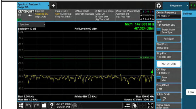
66-66-10MHz-15MHz-QPSK-QPSK-132025-132145-1RB#0-1RB #74-0.009~0.15MHz-PASS
