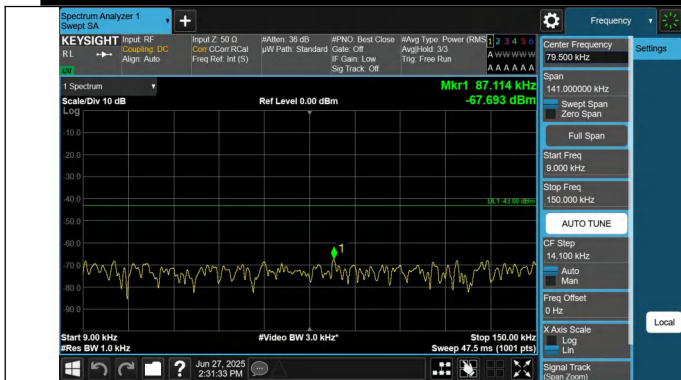
66-66-10MHz-15MHz-QPSK-QPSK-132351-132471-1RB#49-0R B#0-0.009~0.15MHz-PASS
