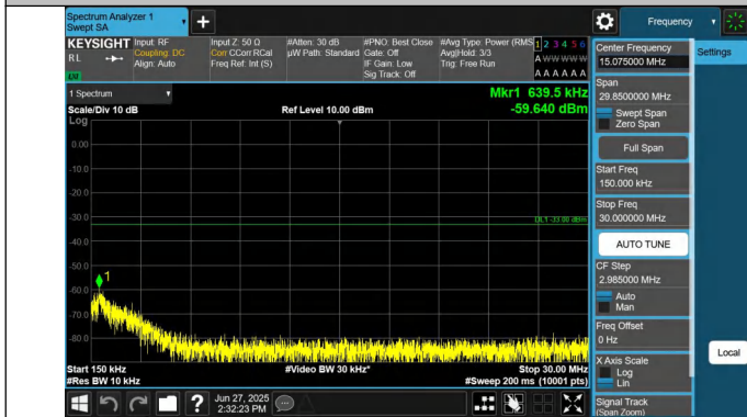
66-66-10MHz-15MHz-QPSK-QPSK-132351-132471-1RB#0-0RB #74-0.15~30MHz-PASS
