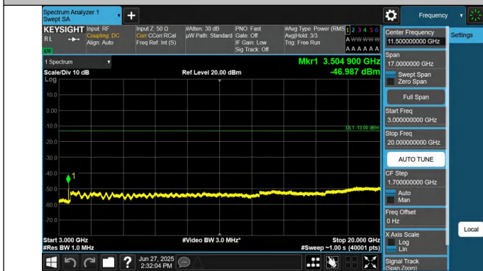
66-66-10MHz-15MHz-QPSK-QPSK-132351-132471-1RB#49-0R B#0-3000~20000MHz-PASS
