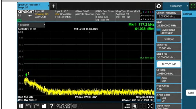
66-66-5MHz-20MHz-QPSK-QPSK-132428-132572-1RB#0-1RB# 99-0.15~30MHz-PASS
