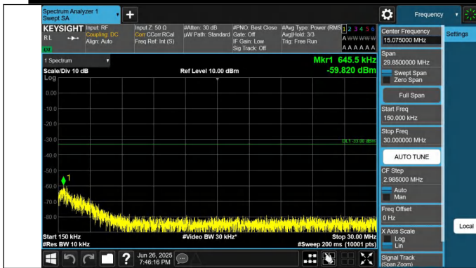
66-66-5MHz-20MHz-QPSK-QPSK-132027-132171-1RB#0-1RB# 99-0.15~30MHz-PASS
