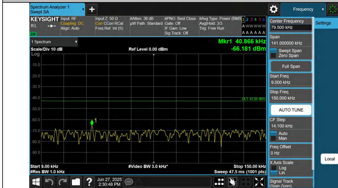
66-66-10MHz-15MHz-QPSK-QPSK-132351-132471-1RB#0-0RB #0-0.009~0.15MHz-PASS
