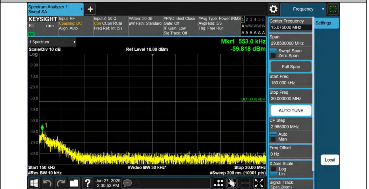
66-66-10MHz-15MHz-QPSK-QPSK-132351-132471-1RB#0-0RB #0-0.15~30MHz-PASS
