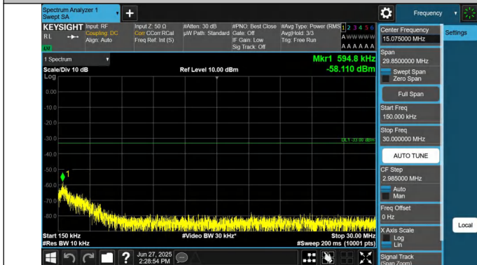
66-66-10MHz-15MHz-QPSK-QPSK-132025-132145-1RB#49-0R B#0-0.15~30MHz-PASS
