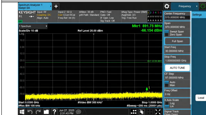
66-66-10MHz-15MHz-QPSK-QPSK-132351-132471-1RB#49-0R B#0-30~1000MHz-PASS
