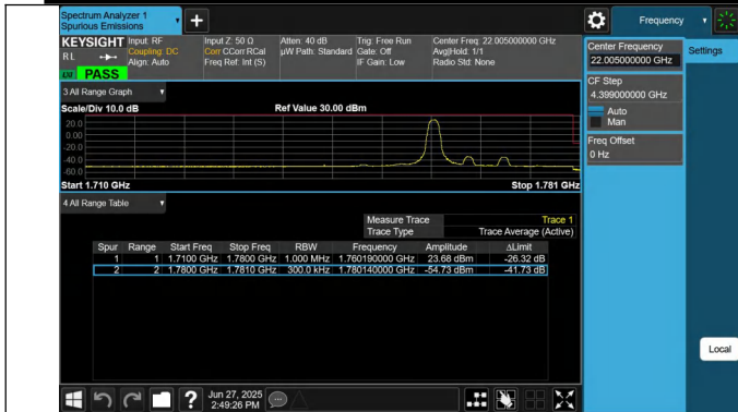
66-66-10MHz-20MHz-QPSK@QPSK-QPSK@QPSK-132428-13 2572-1RB#49@50RB#0-0RB#0@100RB#0-PASS
