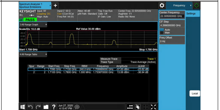
66-66-20MHz-5MHz-QPSK@QPSK-QPSK@QPSK-132072-132189-1RB#0@100RB#0-0RB#0@25RB#0-PASS
