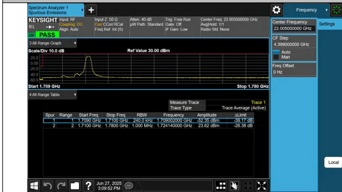
66-66-15MHz-10MHz-QPSK@QPSK-QPSK@QPSK-132047-13 2167-1RB#74@75RB#0-0RB#0@50RB#0-PASS
