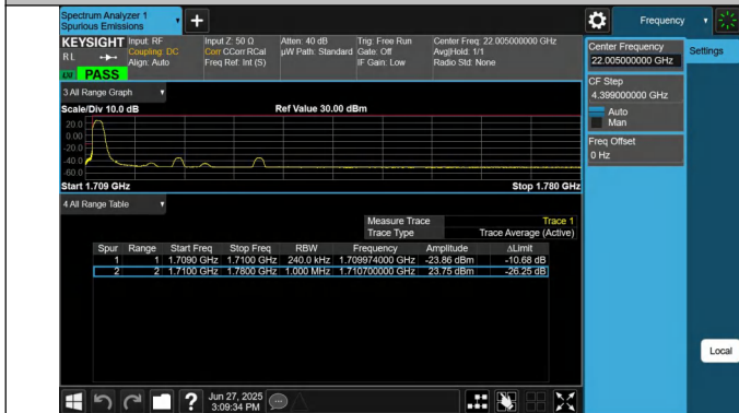
66-66-15MHz-10MHz-QPSK@QPSK-QPSK@QPSK-132047-13 2167-1RB#0@75RB#0-0RB#0@50RB#0-PASS
