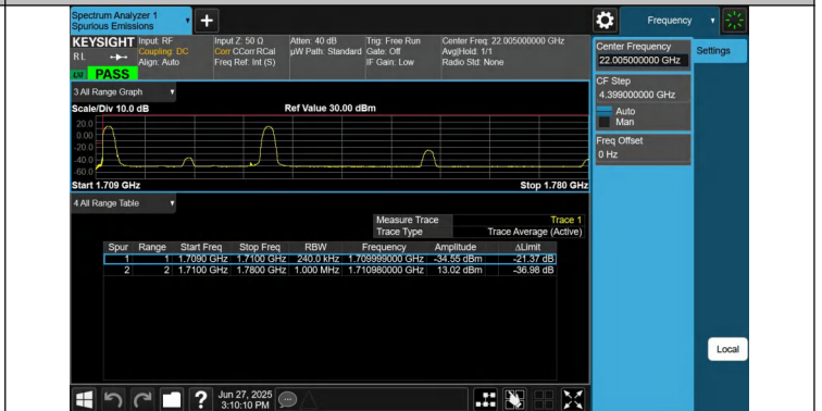
66-66-15MHz-10MHz-QPSK@QPSK-QPSK@QPSK-132047-1321 67-1RB#0@75RB#0-1RB#49@50RB#0-PASS
