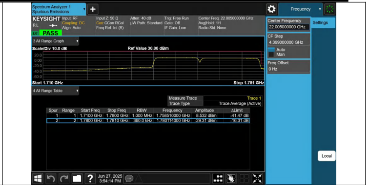
66-66-15MHz-20MHz-QPSK@QPSK-QPSK@QPSK-132401-132572-1RB#74@75RB#0-0RB#0@100RB#0-PASS
