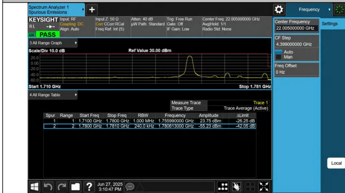
66-66-15MHz-10MHz-QPSK@QPSK-QPSK@QPSK-132499-13 2619-1RB#0@75RB#0-0RB#0@50RB#0-PASS
