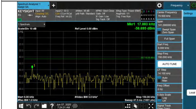
66-66-15MHz-5MHz-QPSK-QPSK-132549-132642-1RB#74-0RB #0-0.009~0.15MHz-PASS
