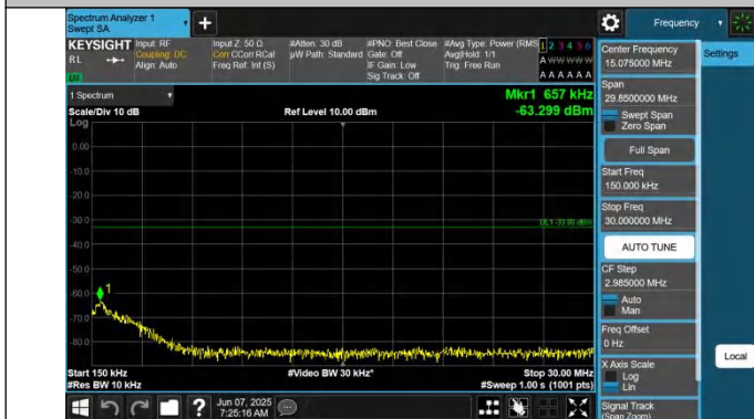
66-66-15MHz-5MHz-QPSK-QPSK-132549-132642-1RB#0-1RB# 24-0.15~30MHz-PASS
