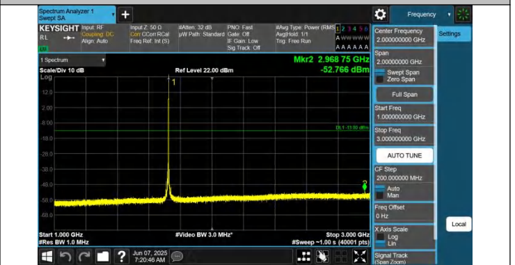
66-66-15MHz-5MHz-QPSK-QPSK-132047-132140-1RB#74-0RB #0-1000~3000MHz-PASS
