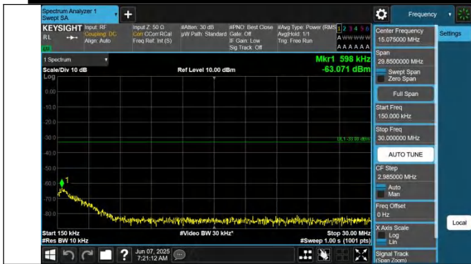
66-66-15MHz-5MHz-QPSK-QPSK-132047-132140-1RB#0-1RB# 24-0.15~30MHz-PASS
