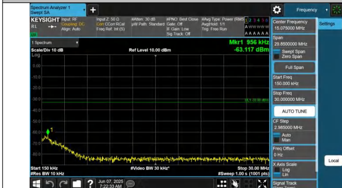
66-66-15MHz-5MHz-QPSK-QPSK-132398-132491-1RB#74-0RB #0-0.15~30MHz-PASS
