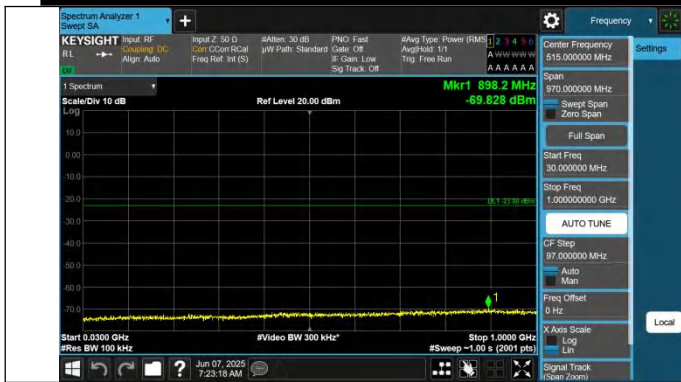
66-66-15MHz-5MHz-QPSK-QPSK-132398-132491-1RB#0-1RB# 24-30~1000MHz-PASS
