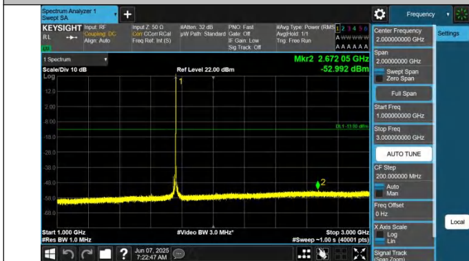
66-66-15MHz-5MHz-QPSK-QPSK-132398-132491-1RB#74-0RB #0-1000~3000MHz-PASS
