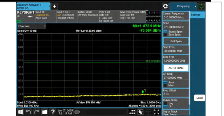
66-66-15MHz-5MHz-QPSK-QPSK-132047-132140-1RB#0-1RB# 24-30~1000MHz-PASS
