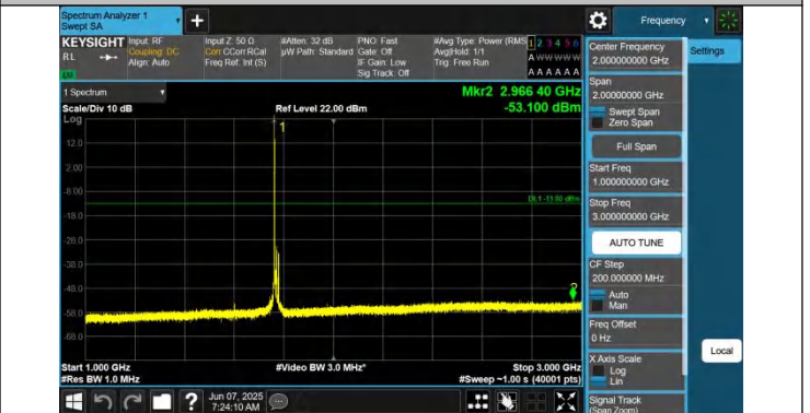
66-66-15MHz-5MHz-QPSK-QPSK-132549-132642-1RB#0-0RB# 0-1000~3000MHz-PASS
