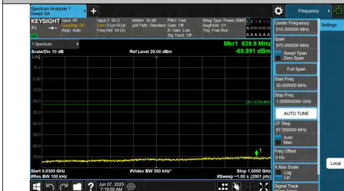
66-66-15MHz-5MHz-QPSK-QPSK-132047-132140-1RB#0-0RB# 0-30~1000MHz-PASS
