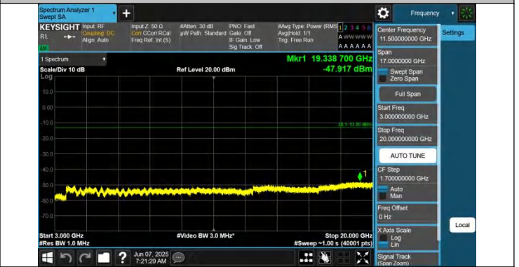
66-66-15MHz-5MHz-QPSK-QPSK-132047-132140-1RB#0-1RB# 24-3000~20000MHz-PASS
