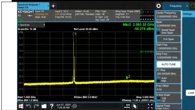
66-66-15MHz-5MHz-QPSK-QPSK-132549-132642-1RB#0-1RB# 24-1000~3000MHz-PASS
