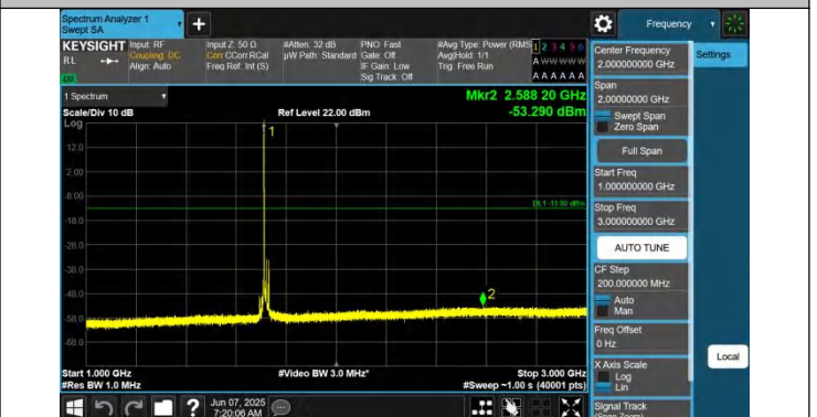
66-66-15MHz-5MHz-QPSK-QPSK-132047-132140-1RB#0-0RB# 0-1000~3000MHz-PASS
