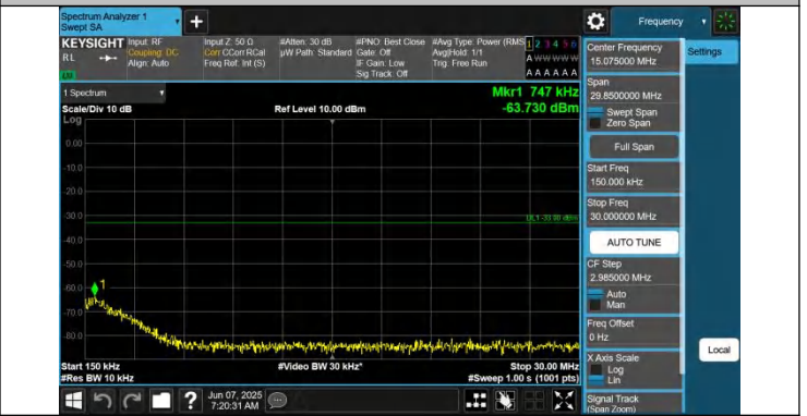
66-66-15MHz-5MHz-QPSK-QPSK-132047-132140-1RB#74-0RB #0-0.15~30MHz-PASS
