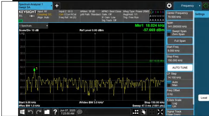
66-66-15MHz-5MHz-QPSK-QPSK-132549-132642-1RB#0-0RB# 0-0.009~0.15MHz-PASS
