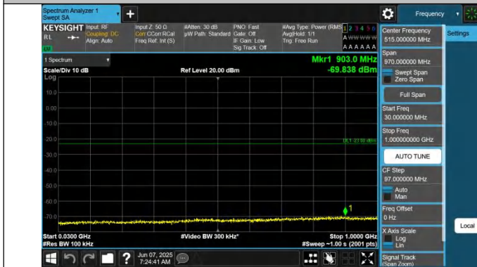
66-66-15MHz-5MHz-QPSK-QPSK-132549-132642-1RB#74-0RB #0-30~1000MHz-PASS
