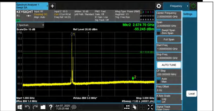
66-66-15MHz-5MHz-QPSK-QPSK-132398-132491-1RB#0-1RB# 24-1000~3000MHz-PASS
