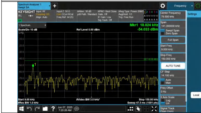
66-66-15MHz-5MHz-QPSK-QPSK-132047-132140-1RB#74-0RB #0-0.009~0.15MHz-PASS
