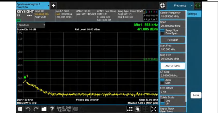
66-66-15MHz-5MHz-QPSK-QPSK-132549-132642-1RB#0-0RB# 0-0.15~30MHz-PASS
