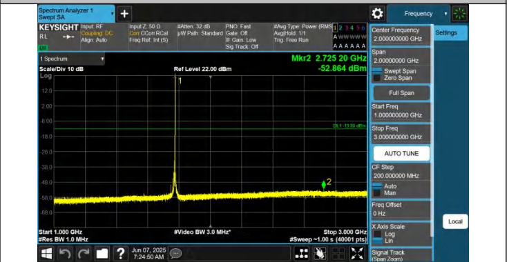
66-66-15MHz-5MHz-QPSK-QPSK-132549-132642-1RB#74-0RB #0-1000~3000MHz-PASS
