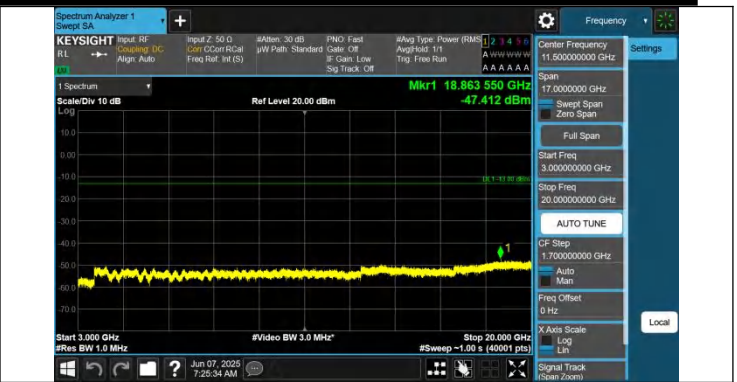
66-66-15MHz-5MHz-QPSK-QPSK-132549-132642-1RB#0-1RB# 24-3000~20000MHz-PASS
