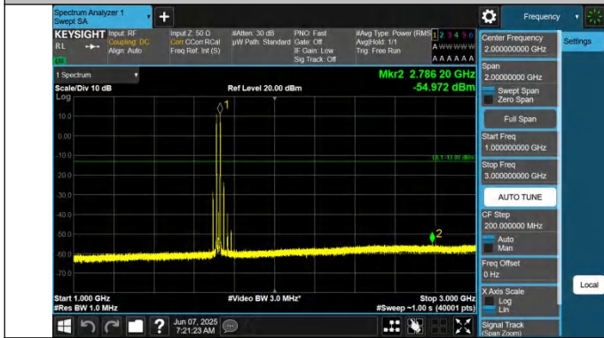
66-66-15MHz-5MHz-QPSK-QPSK-132047-132140-1RB#0-1RB# 24-1000~3000MHz-PASS
