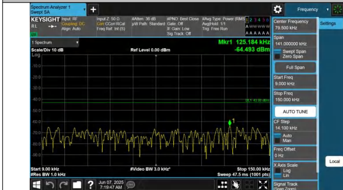
66-66-15MHz-5MHz-QPSK-QPSK-132047-132140-1RB#0-0RB# 0-0.009~0.15MHz-PASS
