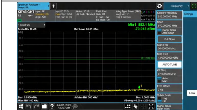
66-66-15MHz-5MHz-QPSK-QPSK-132047-132140-1RB#74-0RB #0-30~1000MHz-PASS
