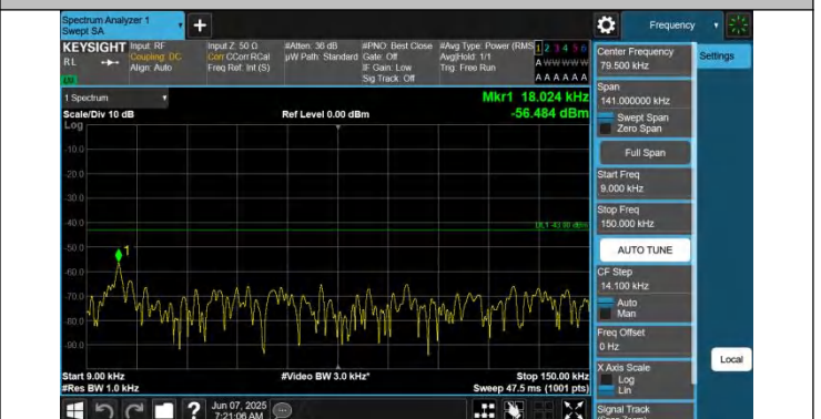
66-66-15MHz-5MHz-QPSK-QPSK-132047-132140-1RB#0-1RB# 24-0.009~0.15MHz-PASS
