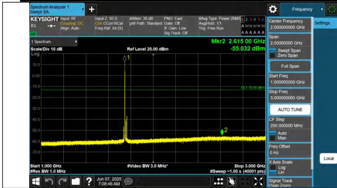
66-66-5MHz-15MHz-QPSK-QPSK-132353-132446-1RB#0-1RB# 74-1000~3000MHz-PASS
