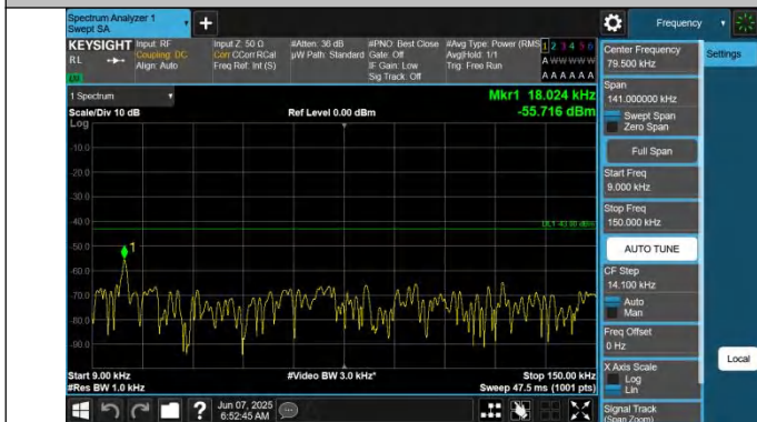
66-66-10MHz-10MHz-QPSK-QPSK-132022-132121-1RB#0-1RB #49-0.009~0.15MHz-PASS
