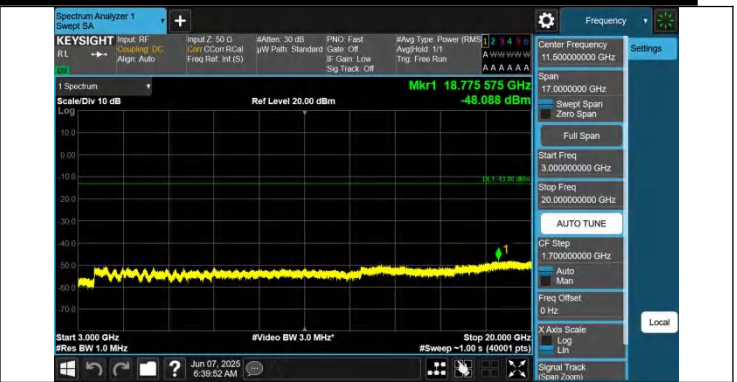
66-66-10MHz-5MHz-QPSK-QPSK-132022-132094-1RB#0-1RB# 24-3000~20000MHz-PASS
