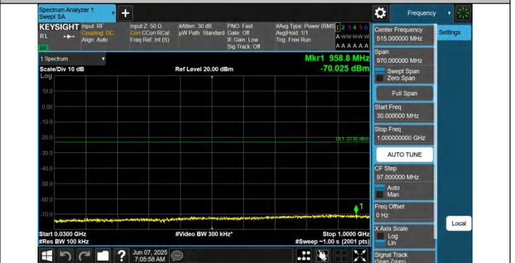
66-66-5MHz-15MHz-QPSK-QPSK-132002-132095-1RB#0-1RB# 74-30~1000MHz-PASS
