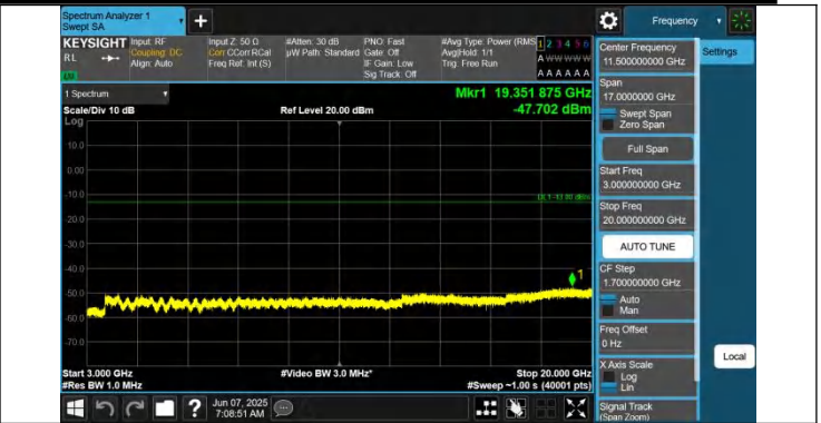
66-66-5MHz-15MHz-QPSK-QPSK-132353-132446-1RB#0-1RB# 74-3000~20000MHz-PASS
