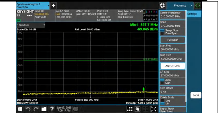
66-66-5MHz-15MHz-QPSK-QPSK-132353-132446-25RB#0-75R B#0-30~1000MHz-PASS
