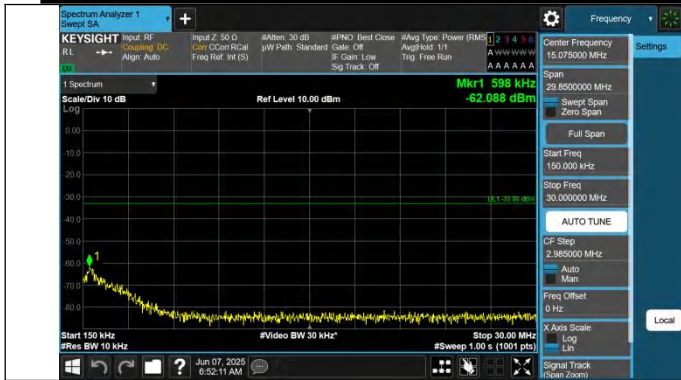
66-66-10MHz-10MHz-QPSK-QPSK-132022-132121-1RB#49-0R B#0-0.15~30MHz-PASS
