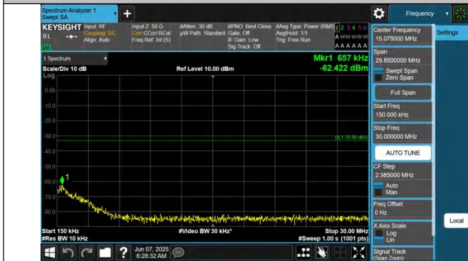
66-66-5MHz-10MHz-QPSK-QPSK-132375-132447-1RB#0-1RB# 49-0.15~30MHz-PASS
