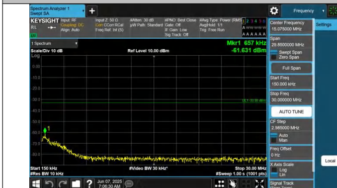
B#0-0.15~30MHz-PASS
