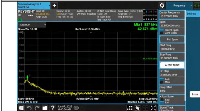
66-66-10MHz-5MHz-QPSK-QPSK-132397-132469-1RB#49-0RB #0-0.15~30MHz-PASS
