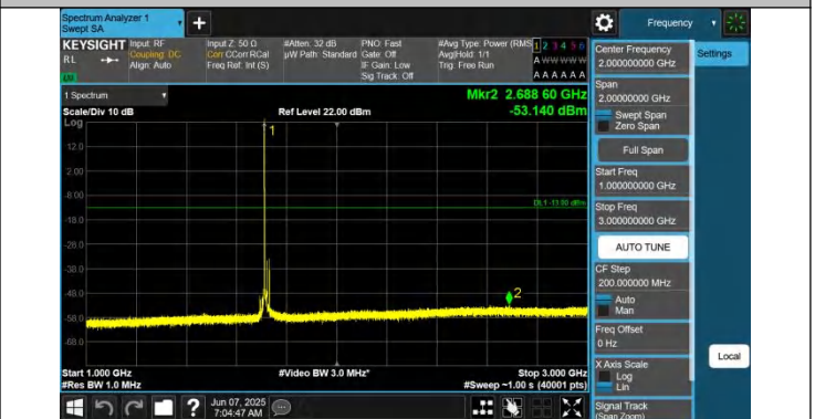
66-66-5MHz-15MHz-QPSK-QPSK-132002-132095-1RB#0-0RB# 0-1000~3000MHz-PASS
