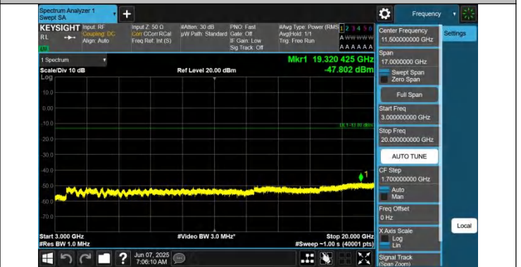
66-66-5MHz-15MHz-QPSK-QPSK-132002-132095-1RB#0-1RB# 74-3000~20000MHz-PASS
