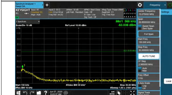
66-66-10MHz-5MHz-QPSK-QPSK-132572-132644-1RB#0-1RB# 24-0.15~30MHz-PASS
