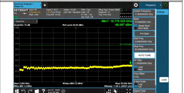
66-66-10MHz-5MHz-QPSK-QPSK-132572-132644-1RB#0-1RB# 24-3000~20000MHz-PASS
