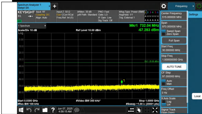
41-41-20MHz-15MHz-QPSK-QPSK-41341-41512-1RB#0-1RB#7 4-30~1000MHz-PASS
