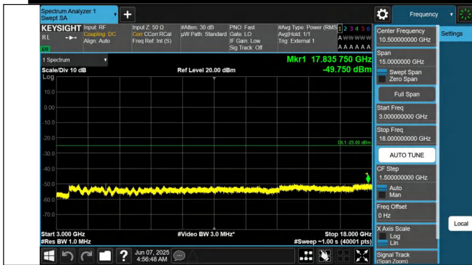
41-41-20MHz-15MHz-QPSK-QPSK-41341-41512-1RB#99-0RB# 0-3000~18000MHz-PASS
