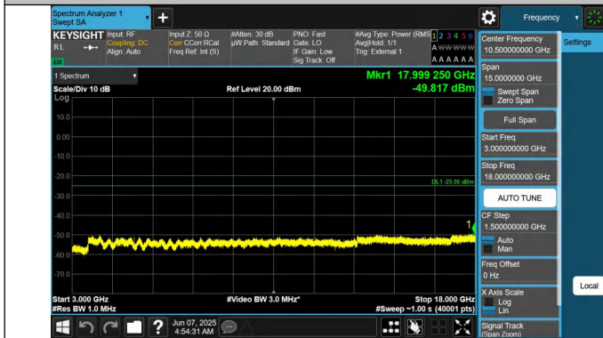
41-41-20MHz-15MHz-QPSK-QPSK-41341-41512-1RB#0-0RB#0- 3000~18000MHz-PASS
