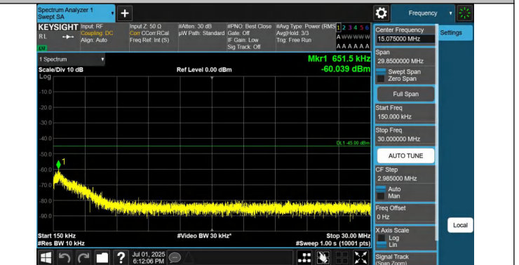
41-41-20MHz-20MHz-QPSK-QPSK-40521-40719-1RB#0-1RB#99-0.15~30MHz-PASS
