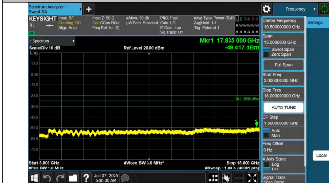
41-41-20MHz-20MHz-QPSK-QPSK-41292-41490-1RB#0-0RB#0-3000~18000MHz-PASS
