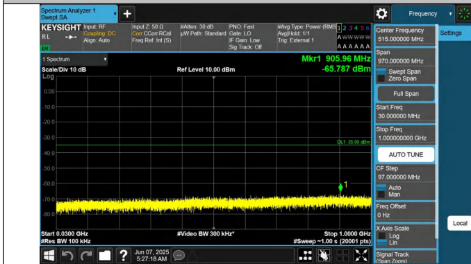
41-41-20MHz-20MHz-QPSK-QPSK-40521-40719-1RB#0-1RB#99-9-30~1000MHz-PASS
