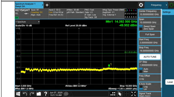
41-41-20MHz-20MHz-QPSK-QPSK-39750-39948-1RB#0-1RB#9 9-3000~18000MHz-PASS
