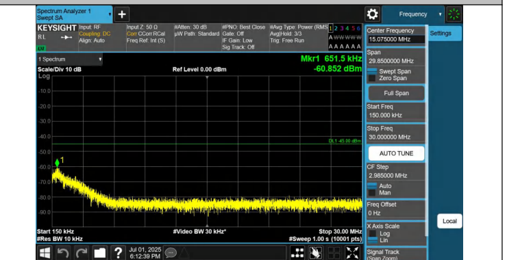
41-41-20MHz-20MHz-QPSK-QPSK-41292-41490-1RB#99-0RB#0 -0.15~30MHz-PASS
