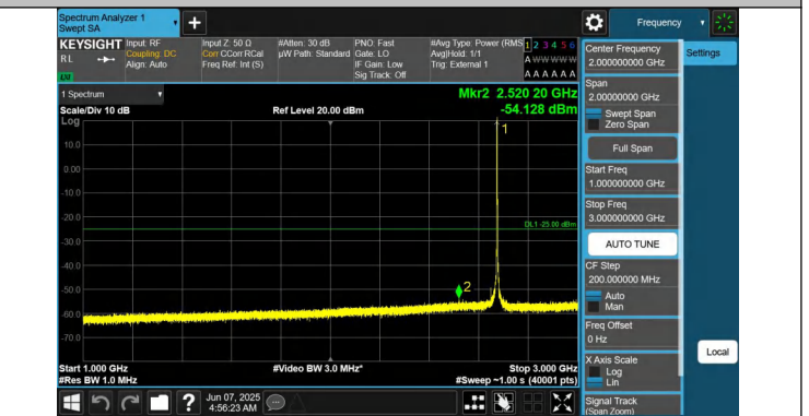
41-41-20MHz-15MHz-QPSK-QPSK-41341-41512-1RB#99-0RB#0 -1000~3000MHz-PASS
