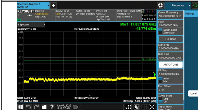
41-41-20MHz-20MHz-QPSK-QPSK-39750-39948-1RB#99-0RB# 0-3000~18000MHz-PASS
