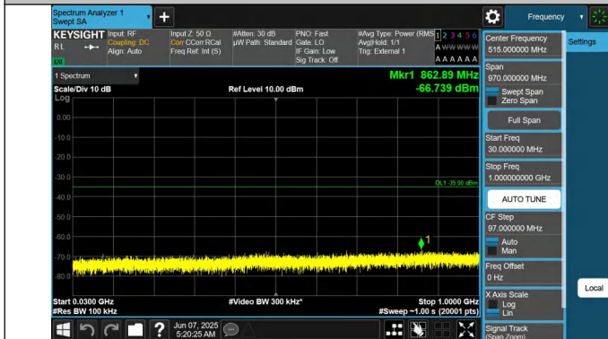
41-41-20MHz-20MHz-QPSK-QPSK-39750-39948-1RB#0-1RB#9 9-30~1000MHz-PASS
