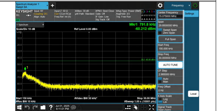
41-41-20MHz-20MHz-QPSK-QPSK-39750-39948-1RB#99-0RB#0 -0.15~30MHz-PASS
