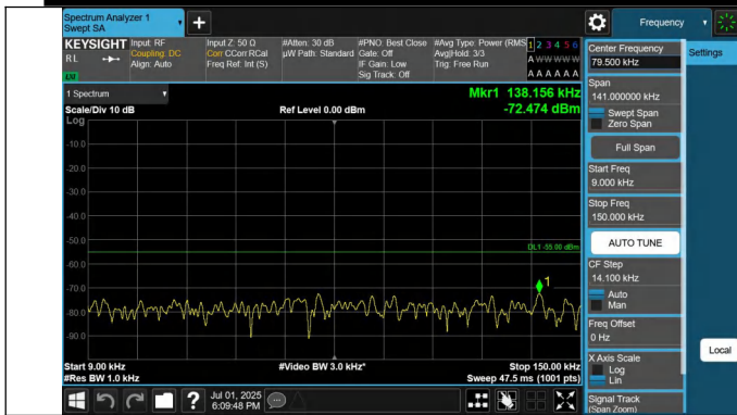
41-41-20MHz-15MHz-QPSK-QPSK-41341-41512-1RB#0-0RB#0- 0.009~0.15MHz-PASS
