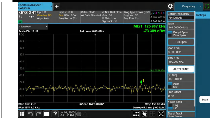
41-41-20MHz-20MHz-QPSK-QPSK-39750-39948-1RB#0-1RB#9 9-0.009~0.15MHz-PASS
