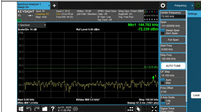
41-41-20MHz-20MHz-QPSK-QPSK-40521-40719-1RB#0-1RB#99-9-0.009~0.15MHz-PASS
