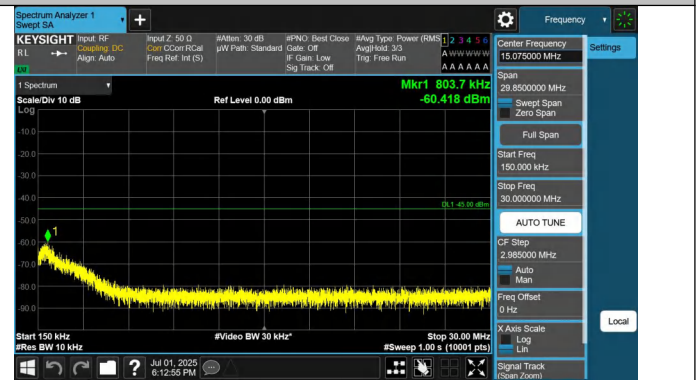
41-41-20MHz-20MHz-QPSK-QPSK-41292-41490-1RB#0-1RB#99-0.15~30MHz-PASS
