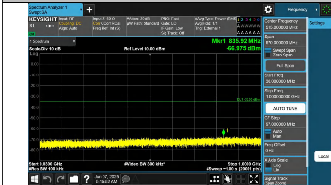
41-41-20MHz-20MHz-QPSK-QPSK-39750-39948-1RB#0-0RB#0- 30~1000MHz-PASS
