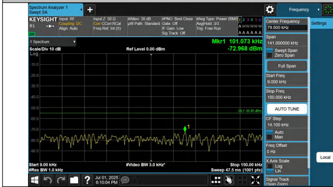
41-41-20MHz-15MHz-QPSK-QPSK-41341-41512-1RB#99-0RB# 0-0.009~0.15MHz-PASS
