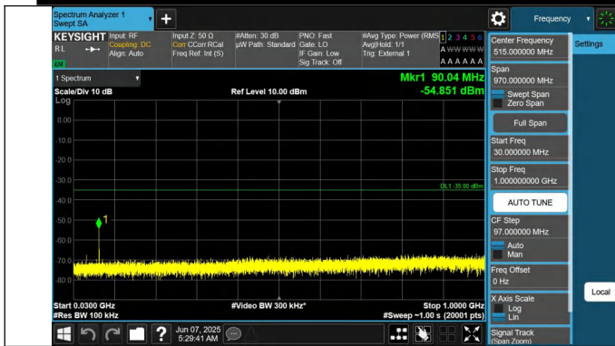
41-41-20MHz-20MHz-QPSK-QPSK-41292-41490-1RB#0-0RB#0-30~1000MHz-PASS
