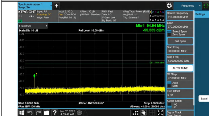
41-41-20MHz-15MHz-QPSK-QPSK-41341-41512-1RB#0-0RB#0- 30~1000MHz-PASS
