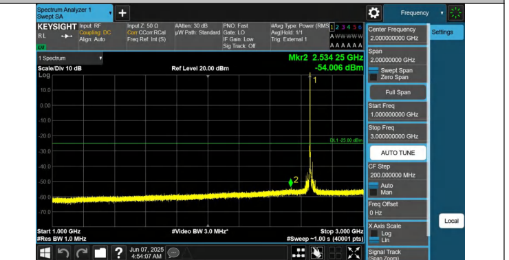
41-41-20MHz-15MHz-QPSK-QPSK-41341-41512-1RB#0-0RB#0- 1000~3000MHz-PASS
