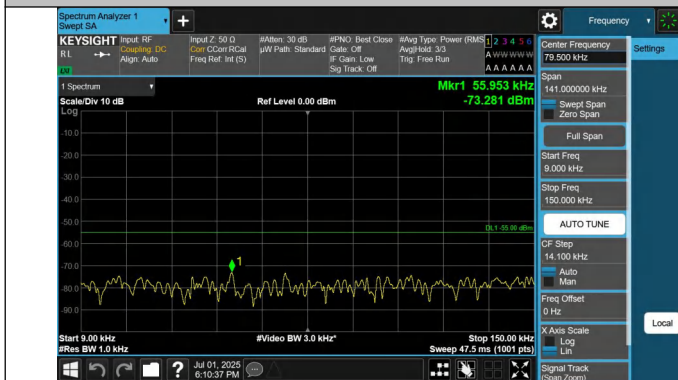
41-41-20MHz-20MHz-QPSK-QPSK-39750-39948-1RB#0-0RB#0- 0.009~0.15MHz-PASS
