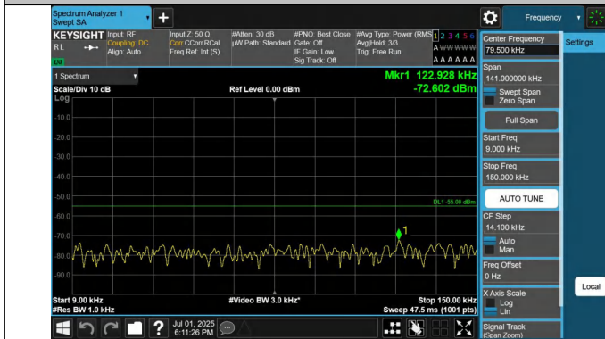
41-41-20MHz-20MHz-QPSK-QPSK-40521-40719-1RB#0-0RB#0- 0.009~0.15MHz-PASS
