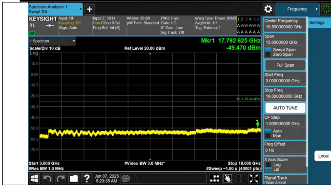
41-41-20MHz-20MHz-QPSK-QPSK-40521-40719-1RB#0-0RB#0-3000~18000MHz-PASS
