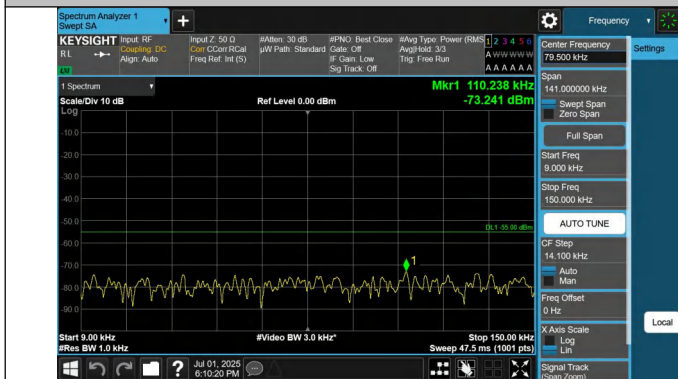
41-41-20MHz-15MHz-QPSK-QPSK-41341-41512-1RB#0-1RB#7 4-0.009~0.15MHz-PASS
