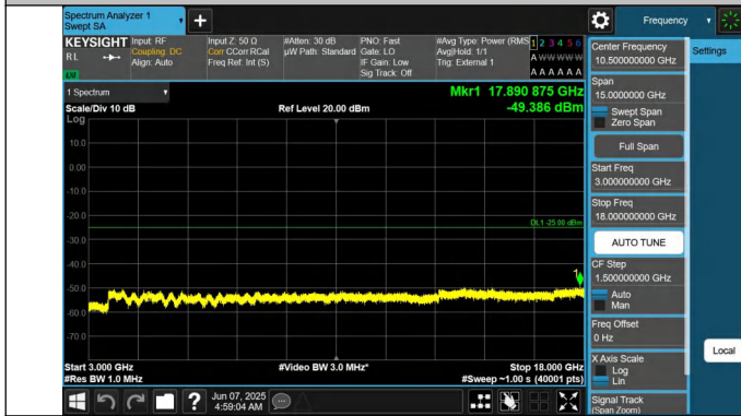
41-41-20MHz-15MHz-QPSK-QPSK-41341-41512-1RB#0-1RB#7 4-3000~18000MHz-PASS
