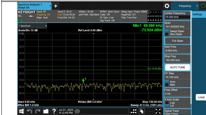
41-41-20MHz-20MHz-QPSK-QPSK-41292-41490-1RB#0-1RB#99-9-0.009~0.15MHz-PASS
