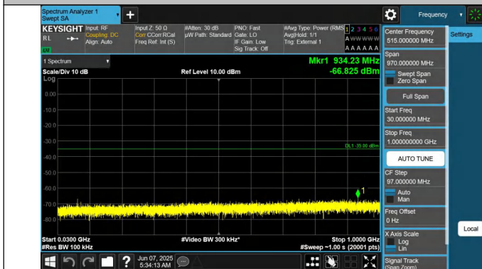
41-41-20MHz-20MHz-QPSK-QPSK-41292-41490-1RB#0-1RB#99-9-30~1000MHz-PASS
