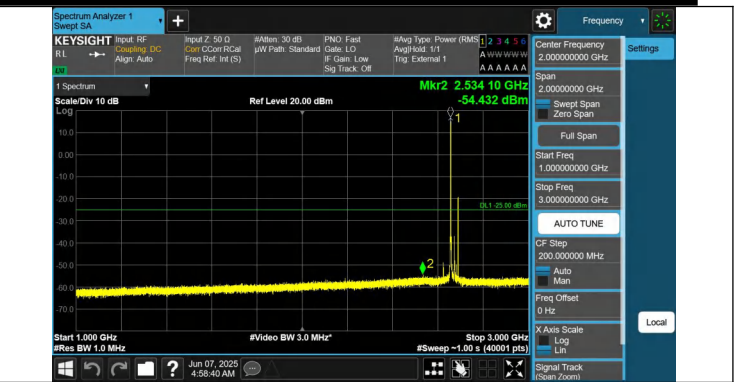
41-41-20MHz-15MHz-QPSK-QPSK-41341-41512-1RB#0-1RB#74 -1000~3000MHz-PASS
