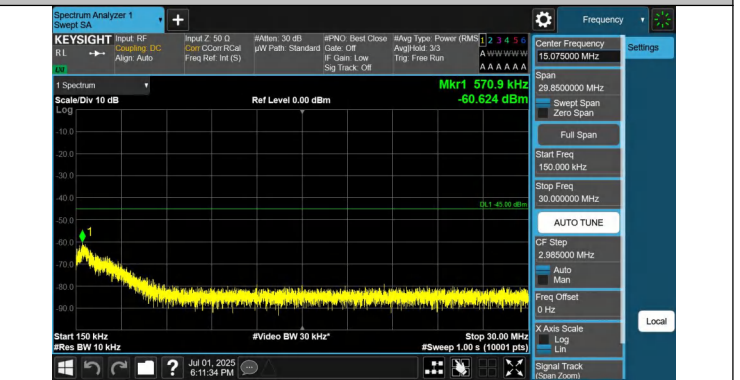
41-41-20MHz-20MHz-QPSK-QPSK-40521-40719-1RB#0-0RB#0- 0.15~30MHz-PASS
