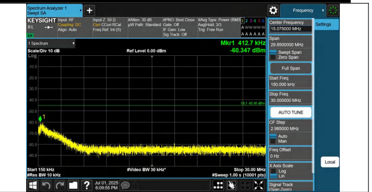
41-41-20MHz-15MHz-QPSK-QPSK-41341-41512-1RB#0-0RB#0- 0.15~30MHz-PASS
