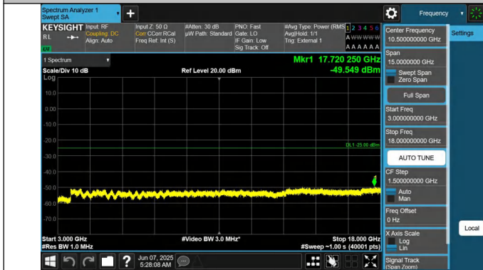
41-41-20MHz-20MHz-QPSK-QPSK-40521-40719-1RB#0-1RB#99-9-3000~18000MHz-PASS
