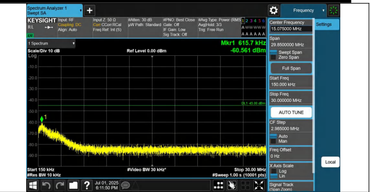
41-41-20MHz-20MHz-QPSK-QPSK-40521-40719-1RB#99-0RB#0 -0.15~30MHz-PASS
