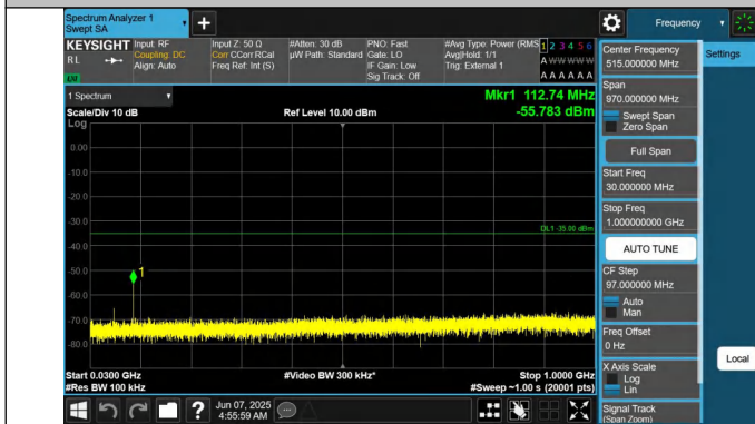
41-41-20MHz-15MHz-QPSK-QPSK-41341-41512-1RB#99-0RB# 0-30~1000MHz-PASS
