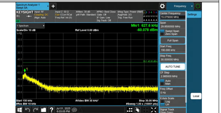
41-41-15MHz-20MHz-QPSK-QPSK-41319-41490-75RB#0-100RB #0-0.15~30MHz-PASS
