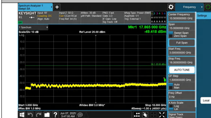
41-41-20MHz-5MHz-QPSK-QPSK-41440-41557-1RB#0-1RB#24- 3000~18000MHz-PASS
