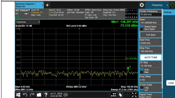
41-41-20MHz-5MHz-QPSK-QPSK-39750-39867-1RB#99-0RB#0-0.009~0.15MHz-PASS
