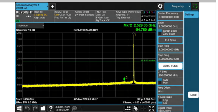
41-41-20MHz-5MHz-QPSK-QPSK-41440-41557-1RB#0-1RB#24- 1000~3000MHz-PASS
