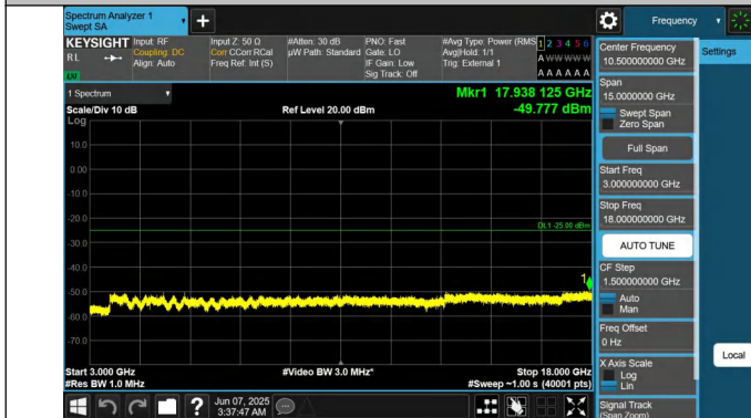
41-41-20MHz-5MHz-QPSK-QPSK-40595-40712-1RB#99-0RB#0-3000~18000MHz-PASS
