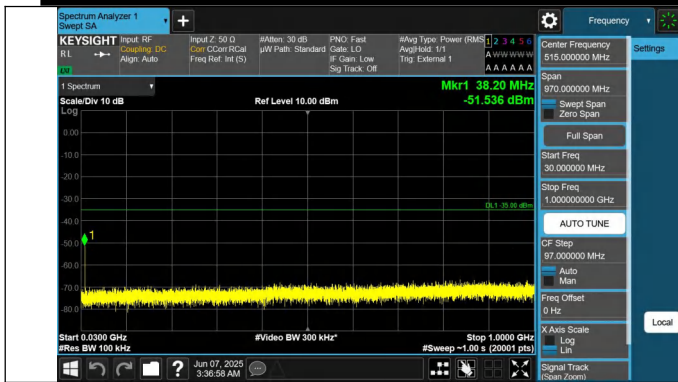
41-41-20MHz-5MHz-QPSK-QPSK-40595-40712-1RB#99-0RB#0-30~1000MHz-PASS
