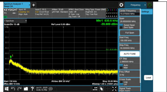
41-41-20MHz-5MHz-QPSK-QPSK-41440-41557-1RB#99-0RB#0- 0.15~30MHz-PASS
