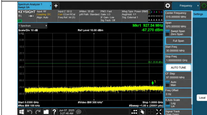
41-41-20MHz-5MHz-QPSK-QPSK-39750-39867-1RB#0-0RB#0-30~1000MHz-PASS
