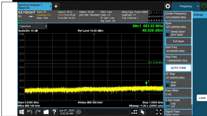
41-41-20MHz-5MHz-QPSK-QPSK-39750-39867-1RB#0-1RB#24-30~1000MHz-PASS
