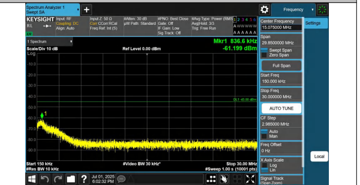
41-41-15MHz-20MHz-QPSK-QPSK-41319-41490-1RB#74-0RB#0 -0.15~30MHz-PASS
