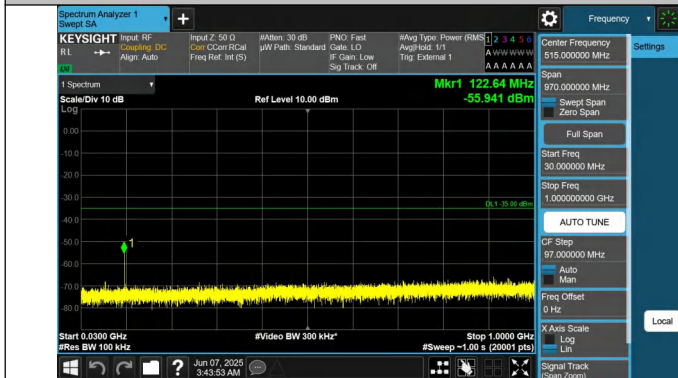
41-41-20MHz-5MHz-QPSK-QPSK-41440-41557-1RB#99-0RB#0- 30~1000MHz-PASS
