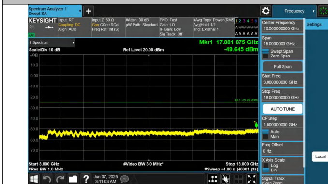
41-41-15MHz-20MHz-QPSK-QPSK-41319-41490-75RB#0-100R B#0-3000~18000MHz-PASS
