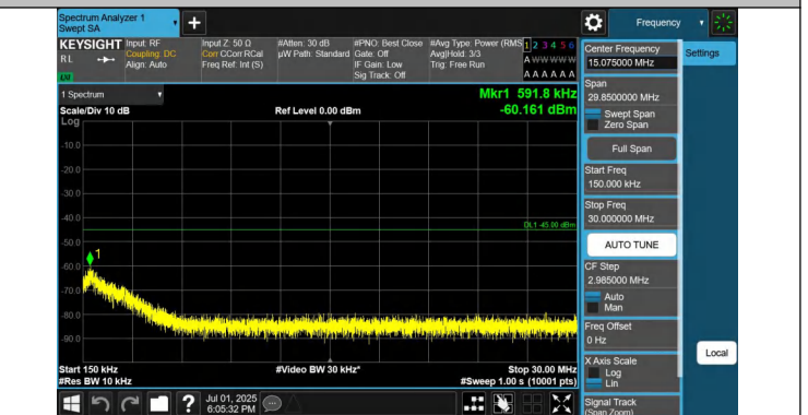
41-41-20MHz-5MHz-QPSK-QPSK-41440-41557-1RB#0-1RB#24- 0.15~30MHz-PASS
