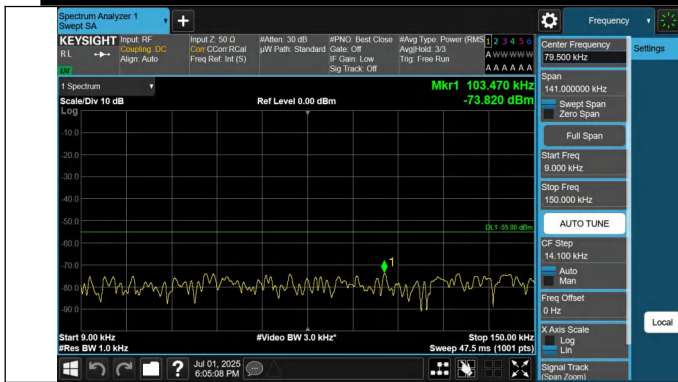
41-41-20MHz-5MHz-QPSK-QPSK-41440-41557-1RB#99-0RB#0- 0.009~0.15MHz-PASS
