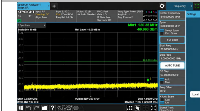
41-41-20MHz-5MHz-QPSK-QPSK-39750-39867-1RB#99-0RB#0-30~1000MHz-PASS
