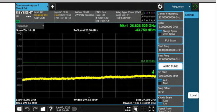
41-41-20MHz-5MHz-QPSK-QPSK-41440-41557-1RB#0-1RB#24- 18000~27000MHz-PASS
