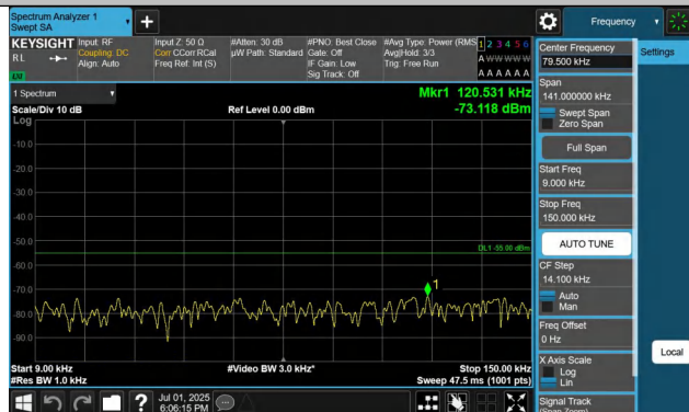
41-41-20MHz-10MHz-QPSK-QPSK-39750-39894-1RB#0-1RB#49-0.009~0.15MHz-PASS
