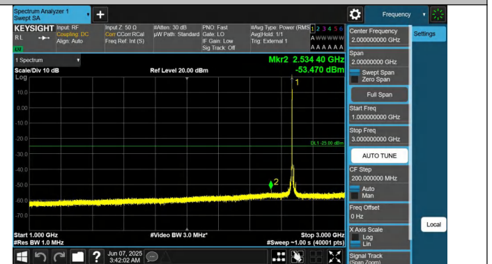
41-41-20MHz-5MHz-QPSK-QPSK-41440-41557-1RB#0-0RB#0-1000~3000MHz-PASS
