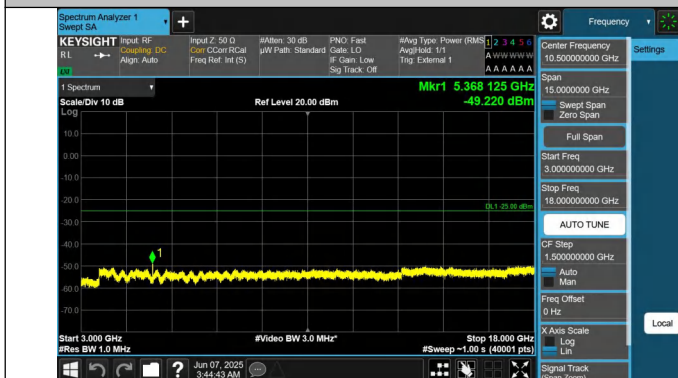
41-41-20MHz-5MHz-QPSK-QPSK-41440-41557-1RB#99-0RB#0- 3000~18000MHz-PASS
