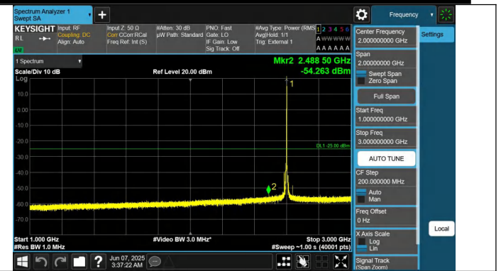
41-41-20MHz-5MHz-QPSK-QPSK-40595-40712-1RB#99-0RB#0-1000~3000MHz-PASS
