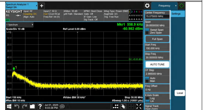
41-41-20MHz-5MHz-QPSK-QPSK-39750-39867-1RB#99-0RB#0-0.15~30MHz-PASS
