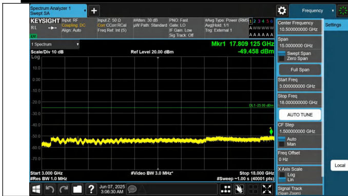
41-41-15MHz-20MHz-QPSK-QPSK-41319-41490-1RB#74-0RB# 0-3000~18000MHz-PASS
