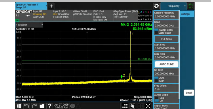
41-41-15MHz-20MHz-QPSK-QPSK-41319-41490-1RB#74-0RB#0 -1000~3000MHz-PASS
