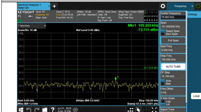
41-41-20MHz-5MHz-QPSK-QPSK-40595-40712-1RB#99-0RB#0- 0.009~0.15MHz-PASS
