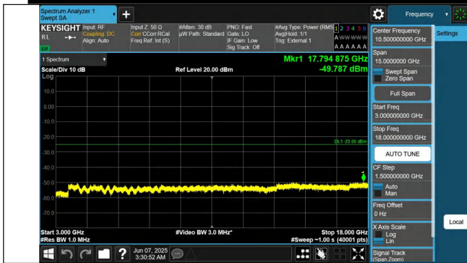
41-41-20MHz-5MHz-QPSK-QPSK-39750-39867-1RB#99-0RB#0-3000~18000MHz-PASS
