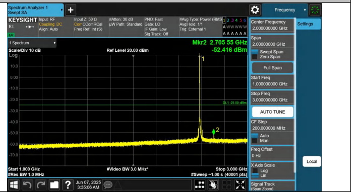
41-41-20MHz-5MHz-QPSK-QPSK-40595-40712-1RB#0-0RB#0-1000~3000MHz-PASS
