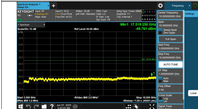
41-41-20MHz-5MHz-QPSK-QPSK-40595-40712-1RB#0-1RB#24- 3000~18000MHz-PASS
