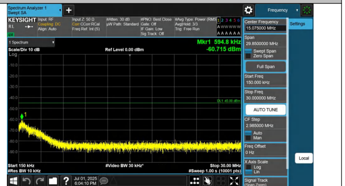
41-41-20MHz-5MHz-QPSK-QPSK-40595-40712-1RB#0-0RB#0-0.15~30MHz-PASS
