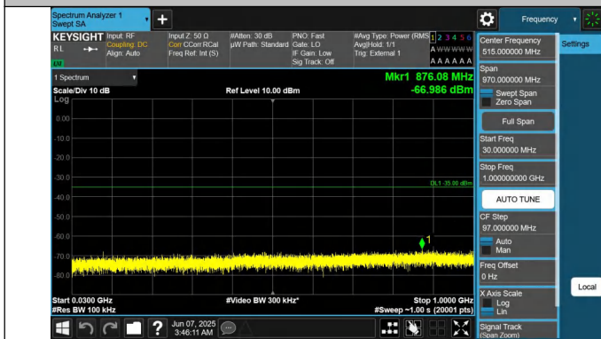
41-41-20MHz-5MHz-QPSK-QPSK-41440-41557-1RB#0-1RB#24- 30~1000MHz-PASS
