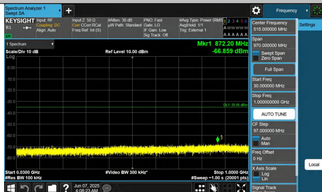
41-41-20MHz-10MHz-QPSK-QPSK-39750-39894-1RB#0-1RB#49-0.30~1000MHz-PASS
