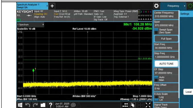
41-41-15MHz-20MHz-QPSK-QPSK-41319-41490-1RB#74-0RB# 0-30~1000MHz-PASS
