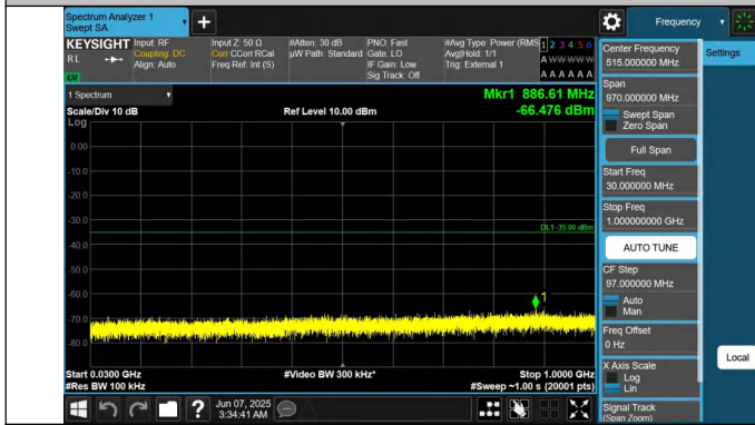
41-41-20MHz-5MHz-QPSK-QPSK-40595-40712-1RB#0-0RB#0-30~1000MHz-PASS
