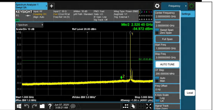
41-41-15MHz-20MHz-QPSK-QPSK-41319-41490-1RB#0-1RB#99 -1000~3000MHz-PASS
