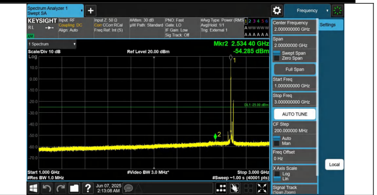
41-41-15MHz-10MHz-QPSK-QPSK-41417-41537-1RB#0-1RB#49 -1000~3000MHz-PASS
