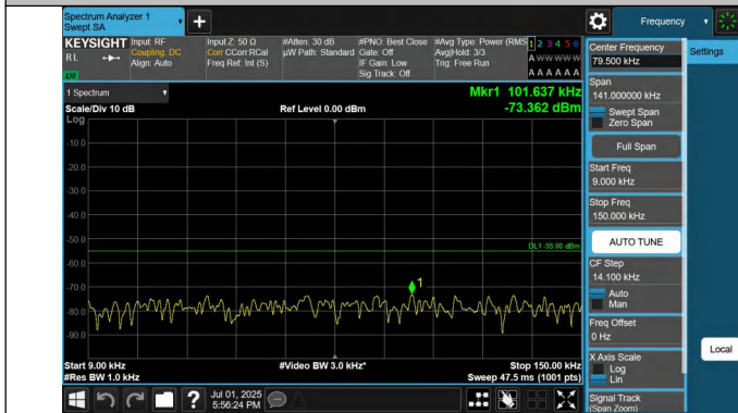
41-41-15MHz-10MHz-QPSK-QPSK-40571-40691-1RB#0-1RB#49-0.009~0.15MHz-PASS
