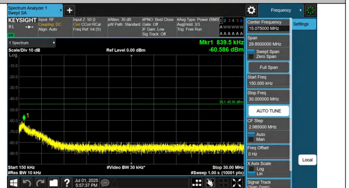
41-41-15MHz-15MHz-QPSK-QPSK-39725-39875-1RB#0-0RB#0- 0.15~30MHz-PASS
