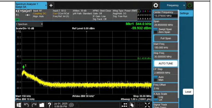
41-41-15MHz-15MHz-QPSK-QPSK-40545-40695-1RB#0-1RB#74-0.15~30MHz-PASS
