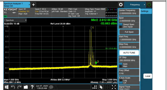
41-41-15MHz-10MHz-QPSK-QPSK-39725-39845-1RB#0-1RB#49-1000~3000MHz-PASS
