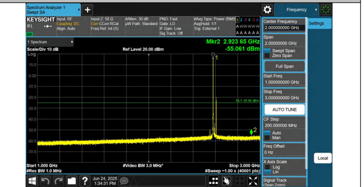
41-41-15MHz-15MHz-QPSK-QPSK-40545-40695-1RB#0-1RB#74-1000~3000MHz-PASS
