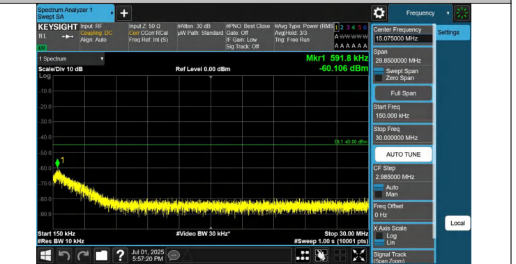
41-41-15MHz-10MHz-QPSK-QPSK-41417-41537-1RB#0-1RB#49 -0.15~30MHz-PASS
