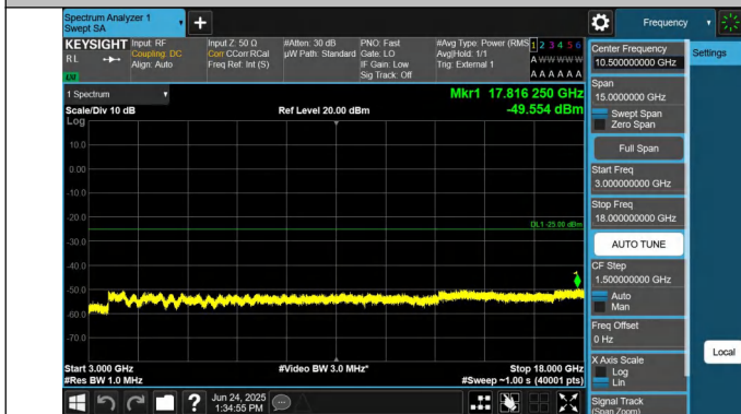
41-41-15MHz-15MHz-QPSK-QPSK-40545-40695-1RB#0-1RB#74-4-3000~18000MHz-PASS
