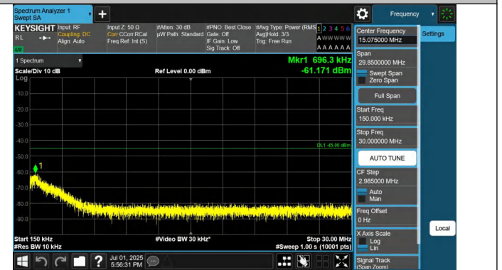
41-41-15MHz-10MHz-QPSK-QPSK-40571-40691-1RB#0-1RB#49-0.15~30MHz-PASS
