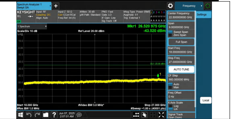
41-41-15MHz-10MHz-QPSK-QPSK-40571-40691-1RB#0-1RB#49 -18000~27000MHz-PASS
