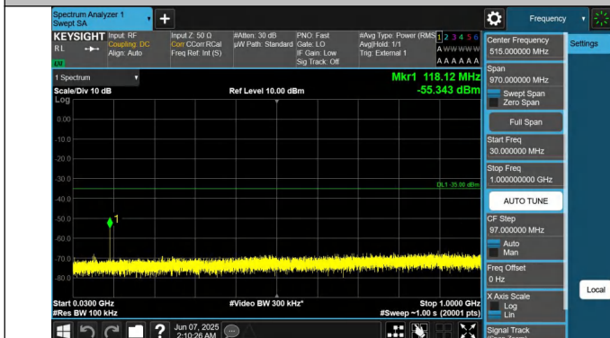
41-41-15MHz-10MHz-QPSK-QPSK-41417-41537-1RB#74-0RB# 0-30~1000MHz-PASS
