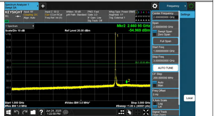
41-41-15MHz-15MHz-QPSK-QPSK-39725-39875-1RB#0-0RB#0- 1000~3000MHz-PASS
