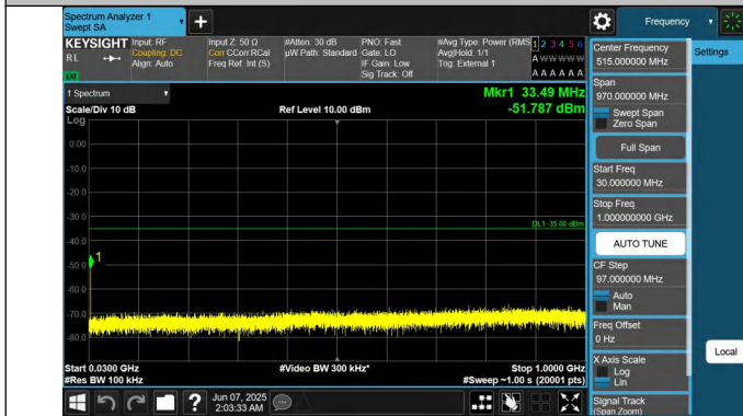
41-41-15MHz-10MHz-QPSK-QPSK-40571-40691-1RB#74-0RB# 0-30~1000MHz-PASS
