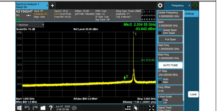
41-41-15MHz-10MHz-QPSK-QPSK-41417-41537-1RB#0-0RB#0- 1000~3000MHz-PASS
