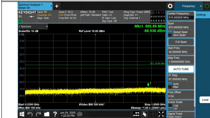
41-41-15MHz-15MHz-QPSK-QPSK-39725-39875-1RB#0-0RB#0- 30~1000MHz-PASS
