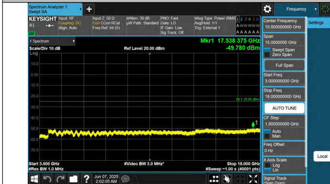
41-41-15MHz-10MHz-QPSK-QPSK-40571-40691-1RB#0-0RB#0-3000~18000MHz-PASS
