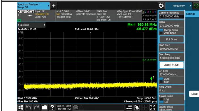
41-41-15MHz-15MHz-QPSK-QPSK-40545-40695-1RB#0-1RB#74-4-30~1000MHz-PASS
