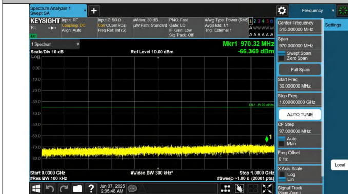
41-41-15MHz-10MHz-QPSK-QPSK-40571-40691-1RB#0-1RB#49-9-30~1000MHz-PASS
