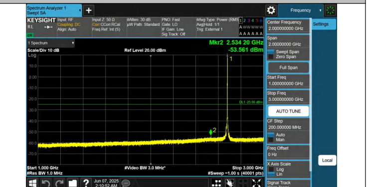
41-41-15MHz-10MHz-QPSK-QPSK-41417-41537-1RB#74-0RB#0 -1000~3000MHz-PASS
