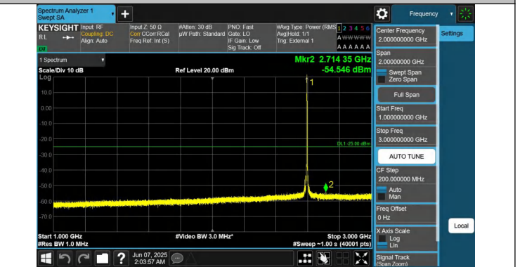
41-41-15MHz-10MHz-QPSK-QPSK-40571-40691-1RB#74-0RB#0 -1000~3000MHz-PASS
