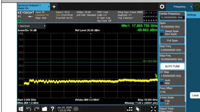
41-41-15MHz-15MHz-QPSK-QPSK-39725-39875-1RB#0-0RB#0- 3000~18000MHz-PASS
