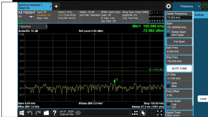
41-41-15MHz-10MHz-QPSK-QPSK-41417-41537-1RB#0-0RB#0- 0.009~0.15MHz-PASS
