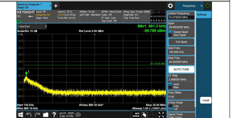
41-41-15MHz-10MHz-QPSK-QPSK-40571-40691-1RB#74-0RB#0 -0.15~30MHz-PASS
