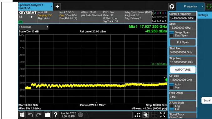
41-41-15MHz-15MHz-QPSK-QPSK-40545-40695-1RB#0-0RB#0-3000~18000MHz-PASS
