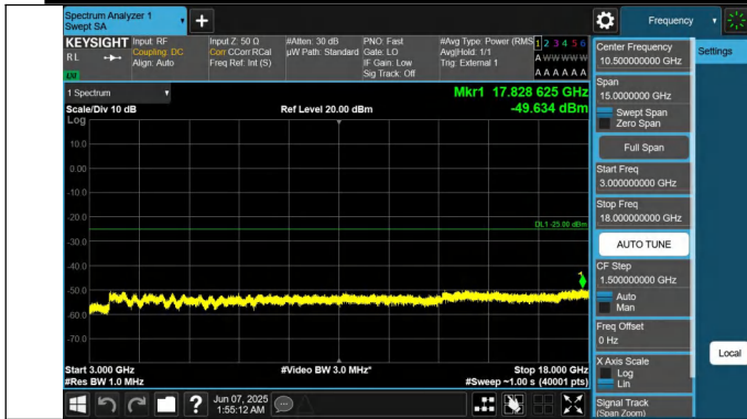
41-41-15MHz-10MHz-QPSK-QPSK-39725-39845-1RB#0-0RB#0-3000~18000MHz-PASS
