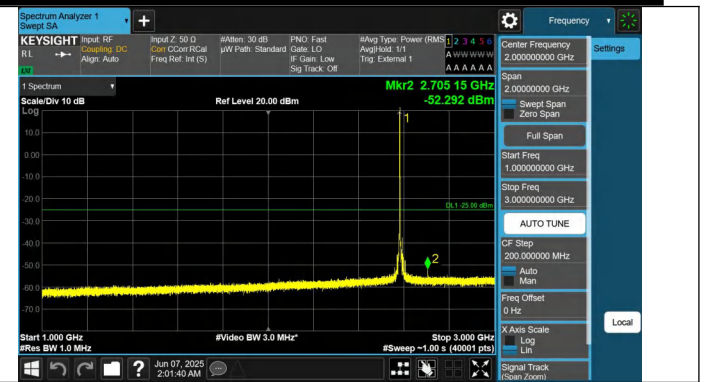
41-41-15MHz-10MHz-QPSK-QPSK-40571-40691-1RB#0-0RB#0-1000~3000MHz-PASS
