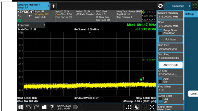
41-41-15MHz-10MHz-QPSK-QPSK-40571-40691-1RB#0-0RB#0-30~1000MHz-PASS
