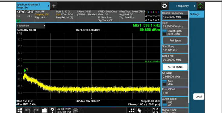
41-41-15MHz-10MHz-QPSK-QPSK-41417-41537-1RB#74-0RB#0 -0.15~30MHz-PASS
