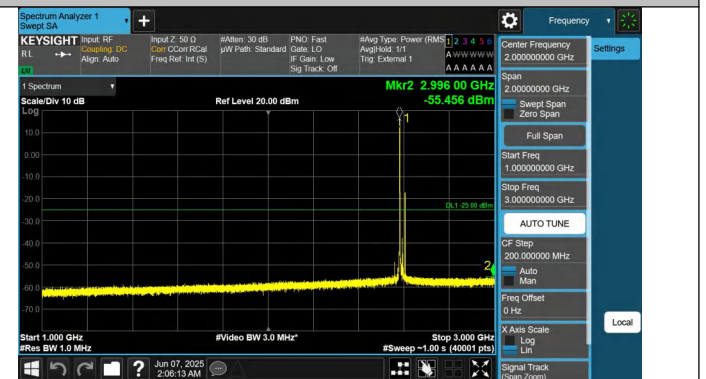
41-41-15MHz-10MHz-QPSK-QPSK-40571-40691-1RB#0-1RB#49-1000~3000MHz-PASS
