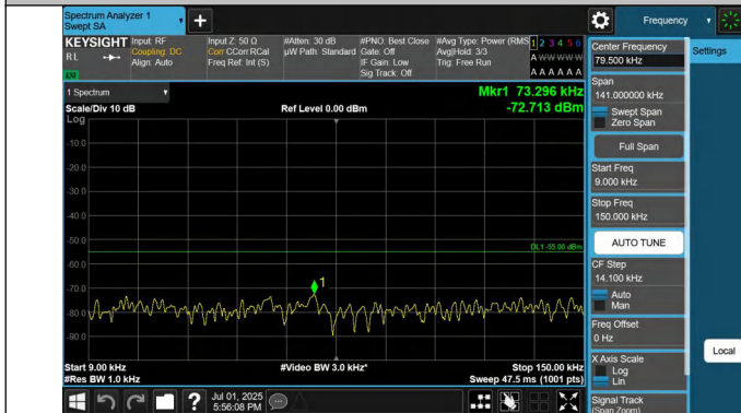
41-41-15MHz-10MHz-QPSK-QPSK-40571-40691-1RB#74-0RB# 0-0.009~0.15MHz-PASS
