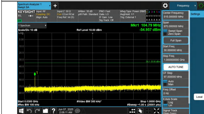
41-41-15MHz-10MHz-QPSK-QPSK-41417-41537-1RB#0-0RB#0- 30~1000MHz-PASS
