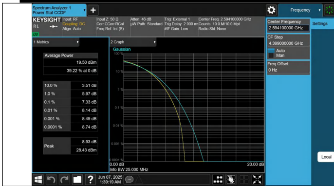
41-41-15MHz-10MHz-256QAM-256QAM-40571-40691-75RB#0-50 RB#0-PASS
