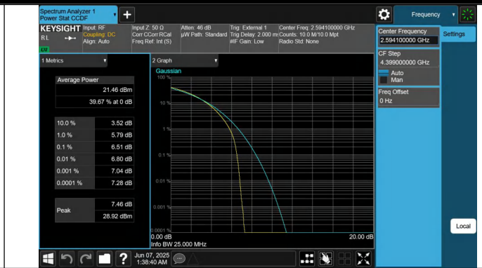
41-41-15MHz-10MHz-16QAM-16QAM-40571-40691-75RB#0-50 RB#0-PASS
