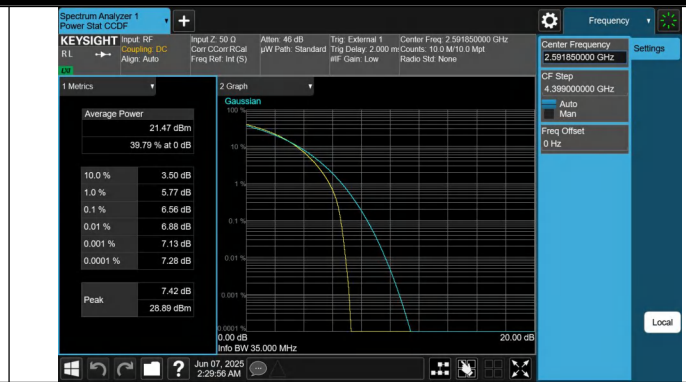
41-41-15MHz-20MHz-16QAM-16QAM-40523-40694-75RB#0-10 ORB#0-PASS
