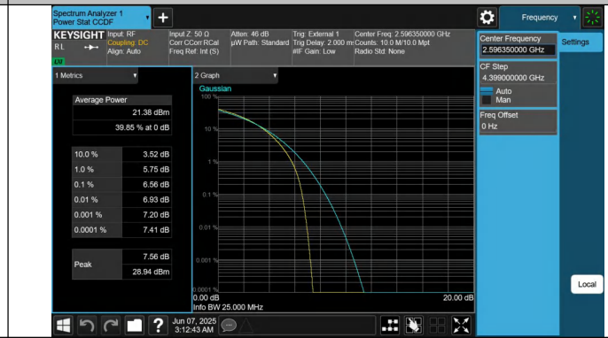
41-41-20MHz-5MHz-16QAM-16QAM-40595-40712-100RB#0-25RB#0-PASS
