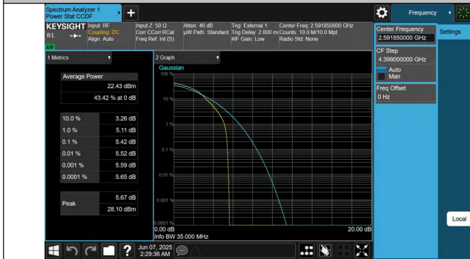
41-41-15MHz-20MHz-QPSK-QPSK-40523-40694-75RB#0-100RB #0-PASS
