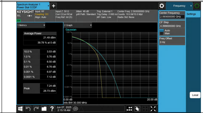
41-41-15MHz-15MHz-16QAM-16QAM-40545-40695-75RB#0-75 RB#0-PASS
