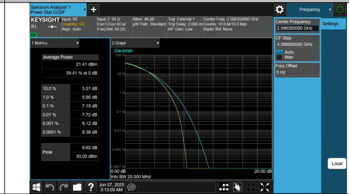
41-41-20MHz-5MHz-64QAM-64QAM-40595-40712-100RB#0-25RB#0-PASS
