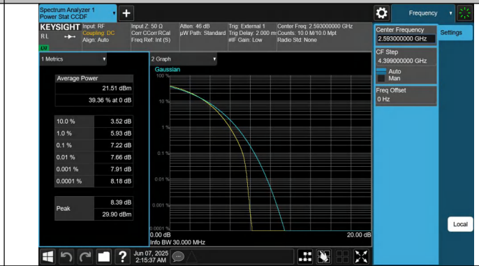
41-41-15MHz-15MHz-64QAM-64QAM-40545-40695-75RB#0-75 RB#0-PASS
