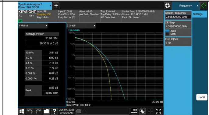
41-41-20MHz-10MHz-64QAM-64QAM-40571-40715-100RB#0-50RB#0-PASS
