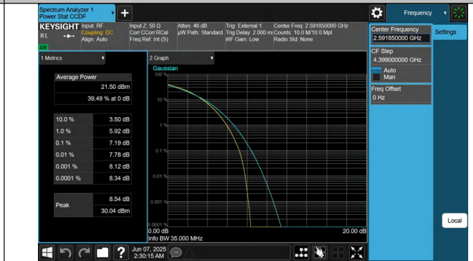
41-41-15MHz-20MHz-64QAM-64QAM-40523-40694-75RB#0-10 ORB#0-PASS
