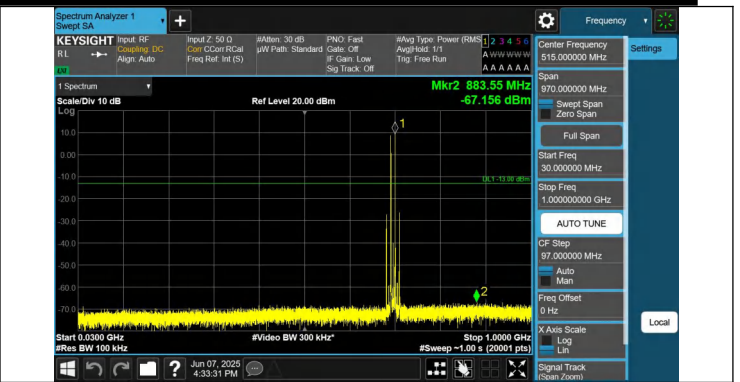
12-12-5MHz-5MHz-QPSK-QPSK-23035-23083-1RB#0-1RB#24-3 0~1000MHz-PASS
