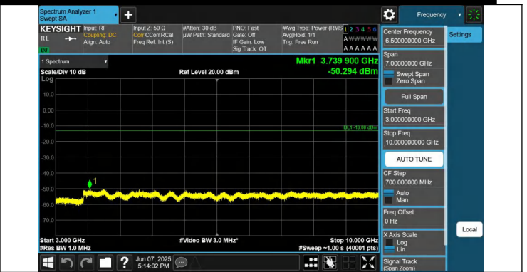
12-12-5MHz-10MHz-QPSK-QPSK-23058-23130-1RB#0-0RB#0-3 000~10000MHz-PASS
