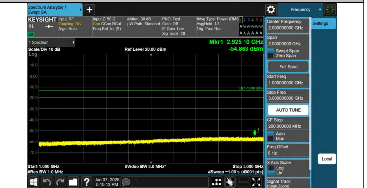
12-12-5MHz-10MHz-QPSK-QPSK-23058-23130-1RB#0-1RB#49- 1000~3000MHz-PASS
