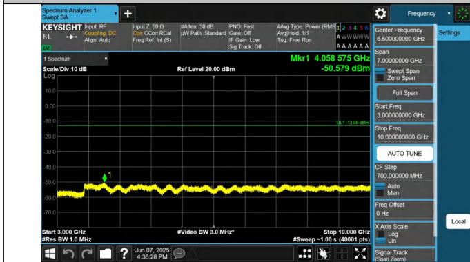
12-12-5MHz-5MHz-QPSK-QPSK-23107-23155-1RB#0-0RB#0-30 00~10000MHz-PASS
