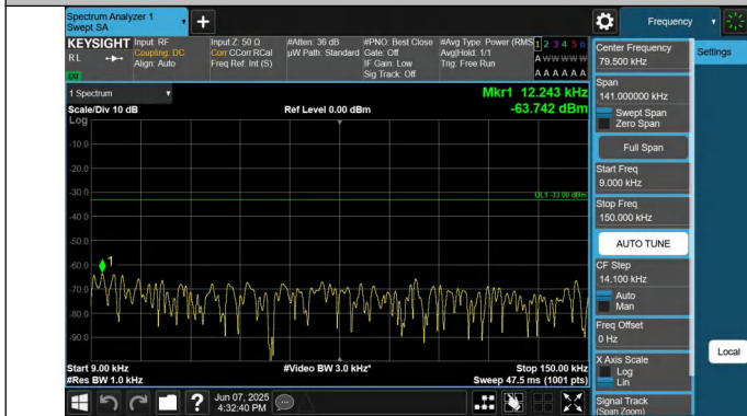
12-12-5MHz-5MHz-QPSK-QPSK-23035-23083-1RB#24-0RB#0-0 .009~0.15MHz-PASS
