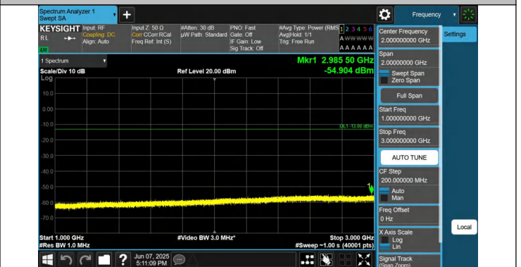
12-12-5MHz-10MHz-QPSK-QPSK-23038-23110-1RB#0-1RB#49- 1000~3000MHz-PASS
