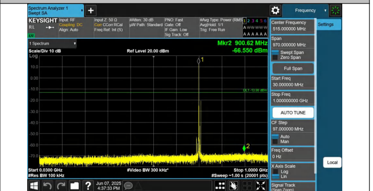
12-12-5MHz-5MHz-QPSK-QPSK-23107-23155-1RB#0-1RB#24-3 0~1000MHz-PASS
