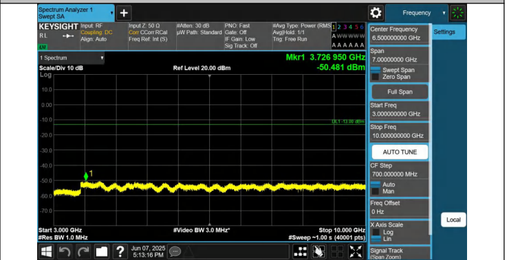
12-12-5MHz-10MHz-QPSK-QPSK-23048-23120-1RB#0-1RB#49- 3000~10000MHz-PASS
