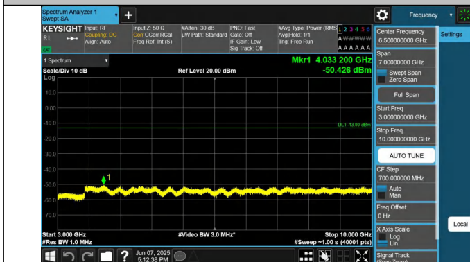
12-12-5MHz-10MHz-QPSK-QPSK-23048-23120-1RB#24-0RB#0- 3000~10000MHz-PASS
