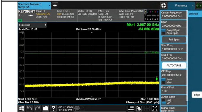
12-12-5MHz-10MHz-QPSK-QPSK-23048-23120-1RB#0-1RB#49- 1000~3000MHz-PASS
