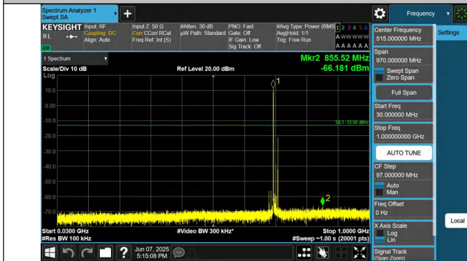
12-12-5MHz-10MHz-QPSK-QPSK-23058-23130-1RB#0-1RB#49- 30~1000MHz-PASS
