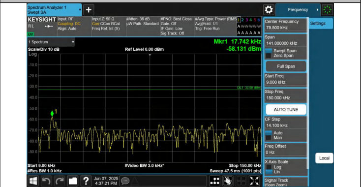
12-12-5MHz-5MHz-QPSK-QPSK-23107-23155-1RB#0-1RB#24-0 .009~0.15MHz-PASS
