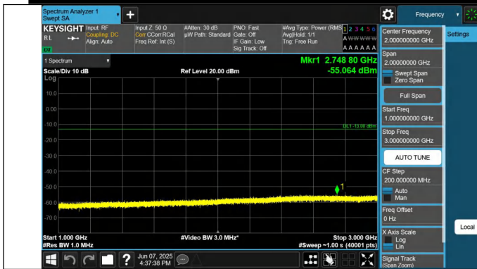
12-12-5MHz-5MHz-QPSK-QPSK-23107-23155-1RB#0-1RB#24-1 000~3000MHz-PASS
