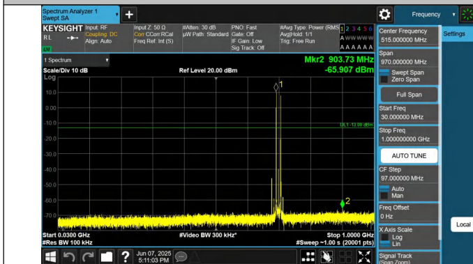
12-12-5MHz-10MHz-QPSK-QPSK-23038-23110-1RB#0-1RB#49- 30~1000MHz-PASS
