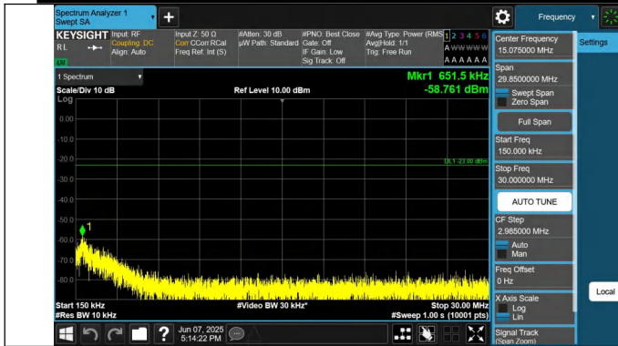
12-12-5MHz-10MHz-QPSK-QPSK-23058-23130-1RB#24-0RB#0- 0.15~30MHz-PASS
