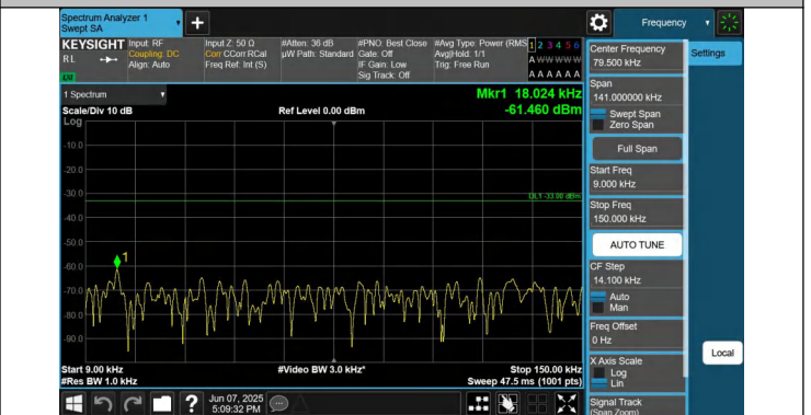
12-12-5MHz-10MHz-QPSK-QPSK-23038-23110-1RB#0-0RB#0-0. 009~0.15MHz-PASS
