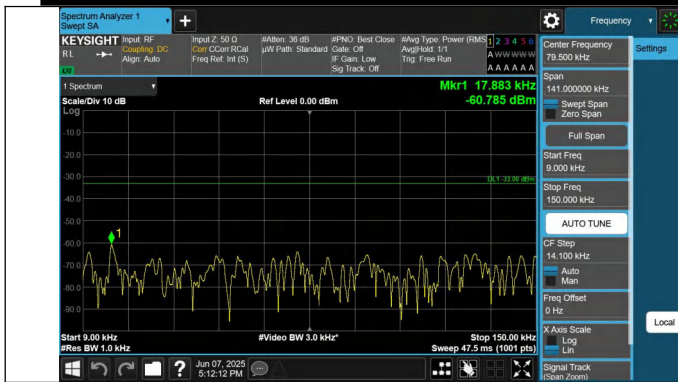
12-12-5MHz-10MHz-QPSK-QPSK-23048-23120-1RB#24-0RB#0- 0.009~0.15MHz-PASS
