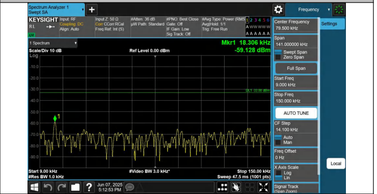
12-12-5MHz-10MHz-QPSK-QPSK-23048-23120-1RB#0-1RB#49- 0.009~0.15MHz-PASS
