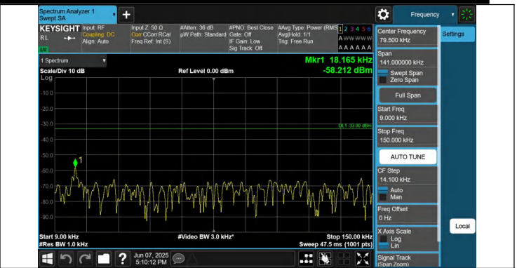
12-12-5MHz-10MHz-QPSK-QPSK-23038-23110-1RB#24-0RB#0- 0.009~0.15MHz-PASS
