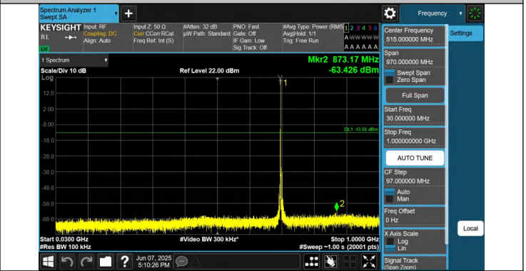
12-12-5MHz-10MHz-QPSK-QPSK-23038-23110-1RB#24-0RB#0- 30~1000MHz-PASS
