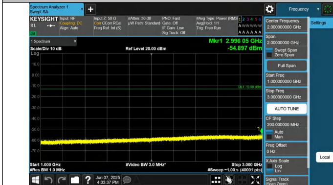
12-12-5MHz-5MHz-QPSK-QPSK-23035-23083-1RB#0-1RB#24-1 000~3000MHz-PASS
