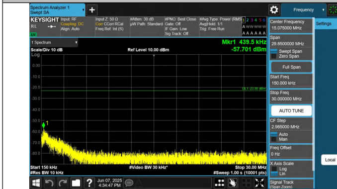
12-12-5MHz-5MHz-QPSK-QPSK-23071-23119-1RB#24-0RB#0-0 .15~30MHz-PASS
