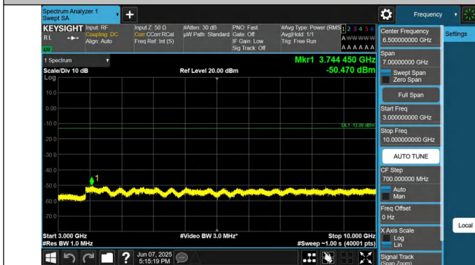
12-12-5MHz-10MHz-QPSK-QPSK-23058-23130-1RB#0-1RB#49- 3000~10000MHz-PASS
