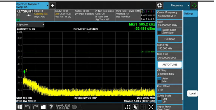
12-12-5MHz-10MHz-QPSK-QPSK-23058-23130-1RB#0-1RB#49- 0.15~30MHz-PASS
