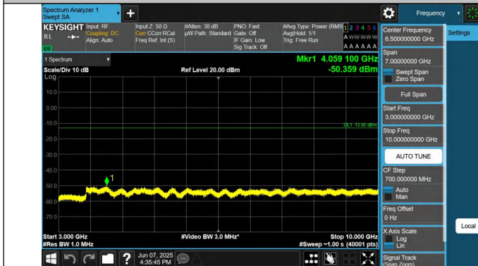
12-12-5MHz-5MHz-QPSK-QPSK-23071-23119-1RB#0-1RB#24-3 000~10000MHz-PASS
