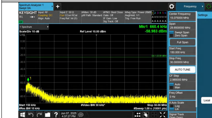
12-12-5MHz-5MHz-QPSK-QPSK-23107-23155-1RB#0-1RB#24-0 .15~30MHz-PASS
