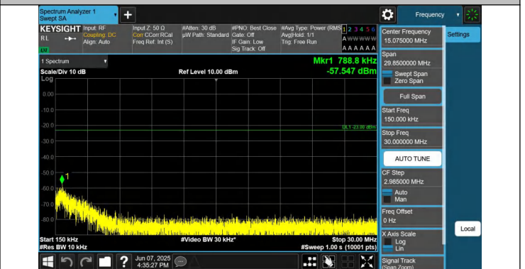
12-12-5MHz-5MHz-QPSK-QPSK-23071-23119-1RB#0-1RB#24-0. 15~30MHz-PASS
