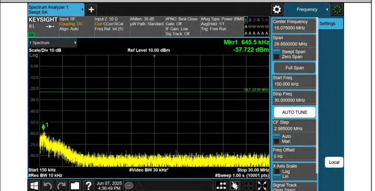
12-12-5MHz-5MHz-QPSK-QPSK-23107-23155-1RB#24-0RB#0-0 .15~30MHz-PASS
