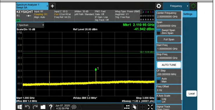
12-12-5MHz-5MHz-QPSK-QPSK-23035-23083-1RB#24-0RB#0-1 000~3000MHz-PASS
