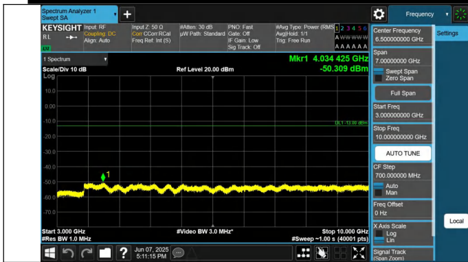
12-12-5MHz-10MHz-QPSK-QPSK-23038-23110-1RB#0-1RB#49- 3000~10000MHz-PASS
