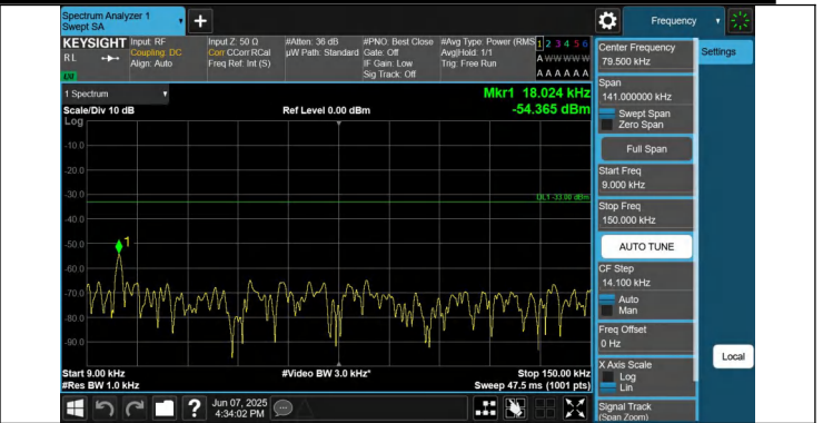
12-12-5MHz-5MHz-QPSK-QPSK-23071-23119-1RB#0-0RB#0-0 09~0.15MHz-PASS
