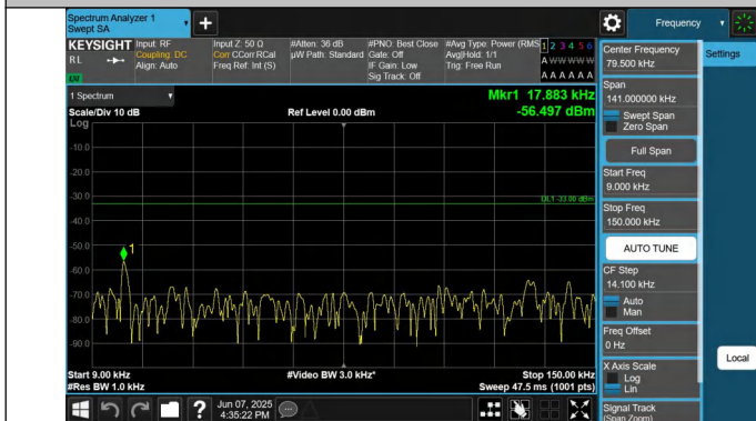
12-12-5MHz-5MHz-QPSK-QPSK-23071-23119-1RB#0-1RB#24-0 .009~0.15MHz-PASS
