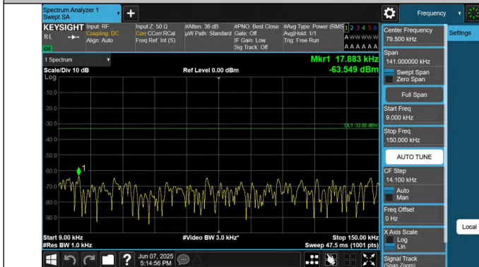
12-12-5MHz-10MHz-QPSK-QPSK-23058-23130-1RB#0-1RB#49- 0.009~0.15MHz-PASS
