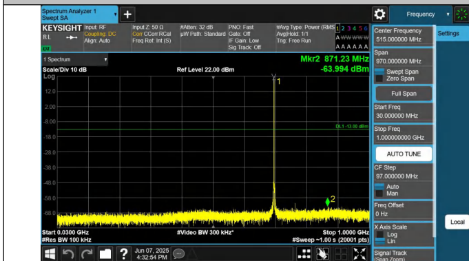
12-12-5MHz-5MHz-QPSK-QPSK-23035-23083-1RB#24-0RB#0-3 0~1000MHz-PASS
