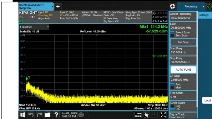
12-12-5MHz-10MHz-QPSK-QPSK-23038-23110-1RB#0-0RB#0-0 .15~30MHz-PASS
