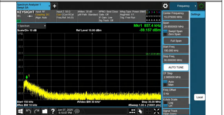
12-12-5MHz-10MHz-QPSK-QPSK-23038-23110-1RB#0-1RB#49- 0.15~30MHz-PASS
