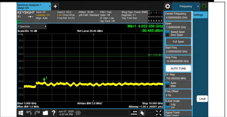
12-12-5MHz-5MHz-QPSK-QPSK-23107-23155-1RB#0-1RB#24-3 000~10000MHz-PASS
