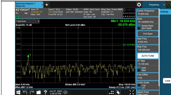
12-12-5MHz-5MHz-QPSK-QPSK-23107-23155-1RB#24-0RB#0-0 .009~0.15MHz-PASS
