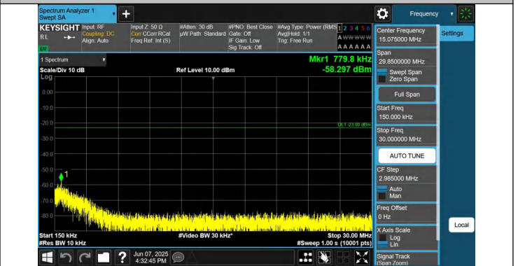
12-12-5MHz-5MHz-QPSK-QPSK-23035-23083-1RB#24-0RB#0-0 .15~30MHz-PASS
