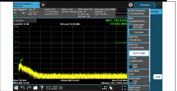
12-12-5MHz-10MHz-QPSK-QPSK-23048-23120-1RB#24-0RB#0- 0.15~30MHz-PASS
