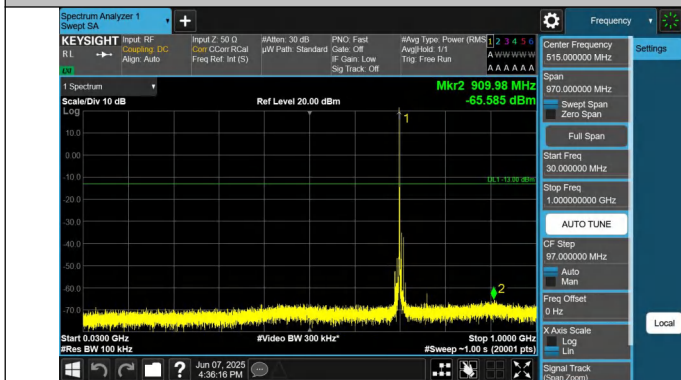
12-12-5MHz-5MHz-QPSK-QPSK-23107-23155-1RB#0-0RB#0-30 ~1000MHz-PASS
