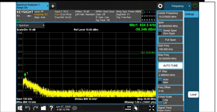
12-12-5MHz-5MHz-QPSK-QPSK-23107-23155-1RB#0-0RB#0-0. 15~30MHz-PASS
