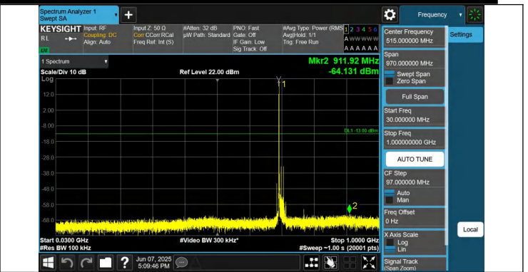
12-12-5MHz-10MHz-QPSK-QPSK-23038-23110-1RB#0-0RB#0-3 0~1000MHz-PASS
