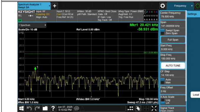
12-12-5MHz-10MHz-QPSK-QPSK-23038-23110-1RB#0-1RB#49- 0.009~0.15MHz-PASS
