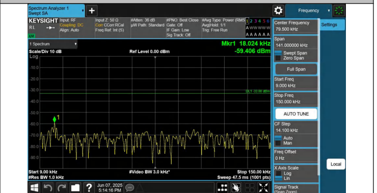
12-12-5MHz-10MHz-QPSK-QPSK-23058-23130-1RB#24-0RB#0- 0.009~0.15MHz-PASS
