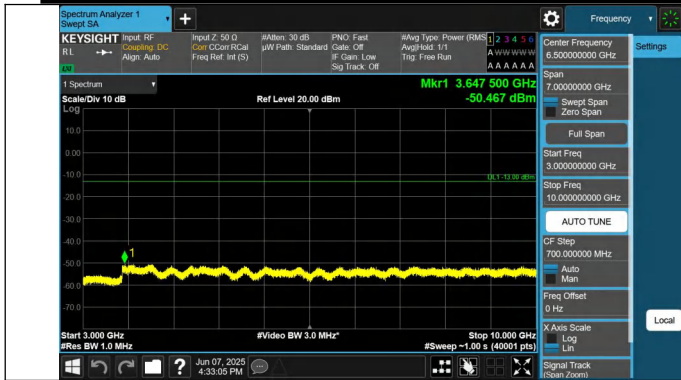
12-12-5MHz-5MHz-QPSK-QPSK-23035-23083-1RB#24-0RB#0-3 000~10000MHz-PASS
