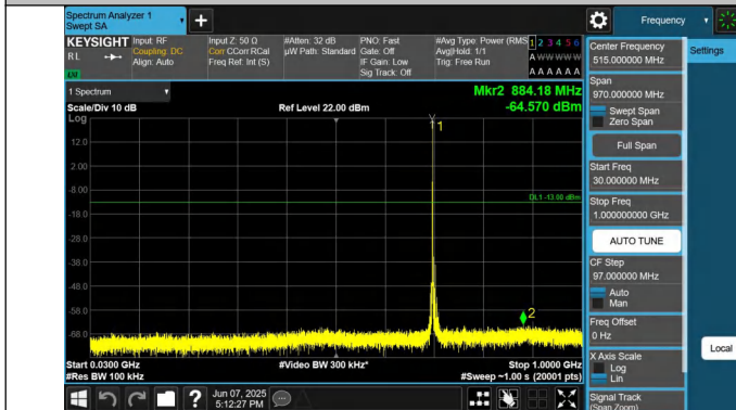
12-12-5MHz-10MHz-QPSK-QPSK-23048-23120-1RB#24-0RB#0- 30~1000MHz-PASS
