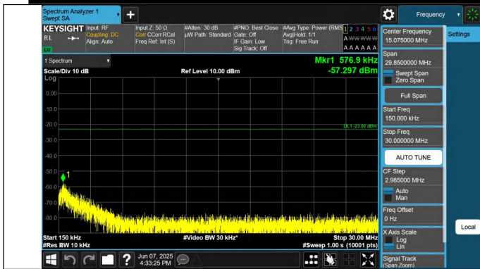
12-12-5MHz-5MHz-QPSK-QPSK-23035-23083-1RB#0-1RB#24-0 .15~30MHz-PASS
