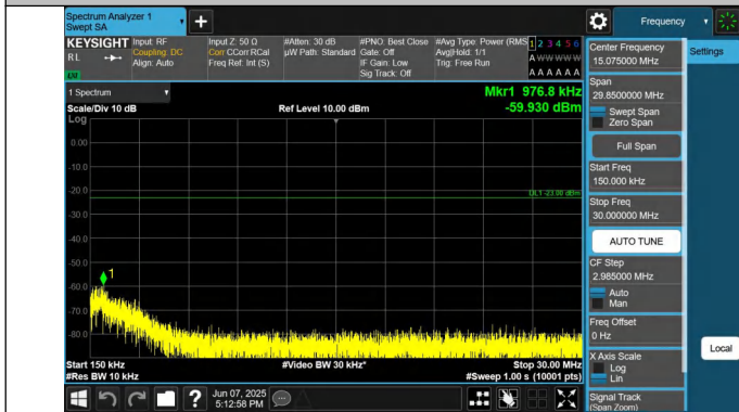
12-12-5MHz-10MHz-QPSK-QPSK-23048-23120-1RB#0-1RB#49- 0.15~30MHz-PASS
