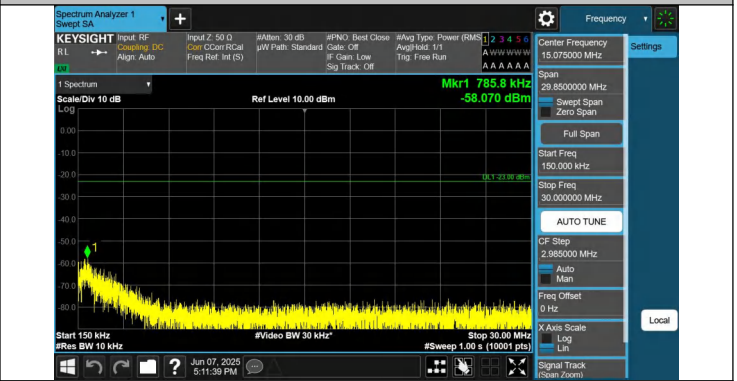
12-12-5MHz-10MHz-QPSK-QPSK-23048-23120-1RB#0-0RB#0-0 .15~30MHz-PASS
