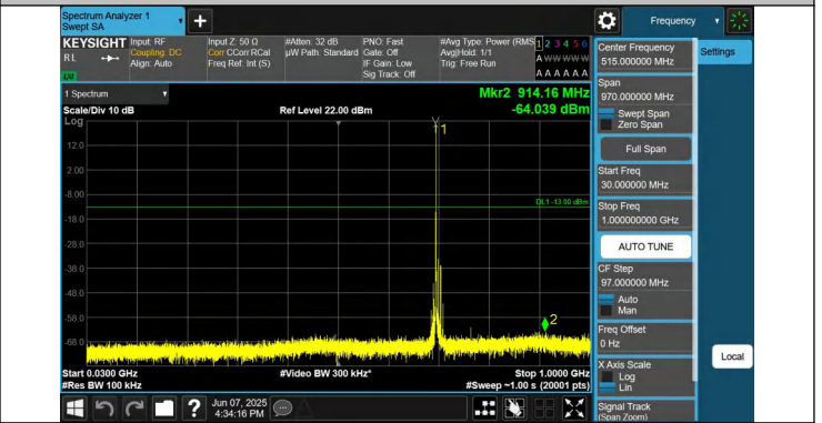
12-12-5MHz-5MHz-QPSK-QPSK-23071-23119-1RB#0-0RB#0-30 ~1000MHz-PASS
