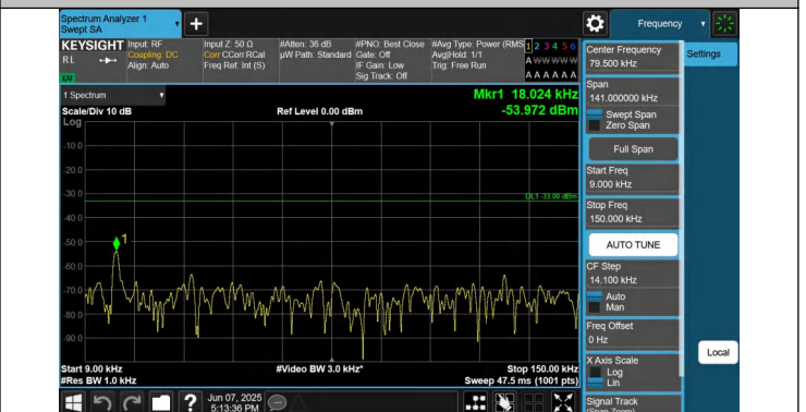
12-12-5MHz-10MHz-QPSK-QPSK-23058-23130-1RB#0-0RB#0-0 .009~0.15MHz-PASS
