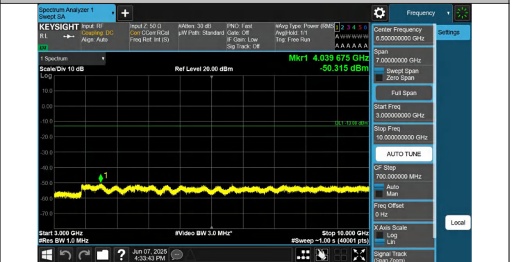
12-12-5MHz-5MHz-QPSK-QPSK-23035-23083-1RB#0-1RB#24-3 000~10000MHz-PASS
