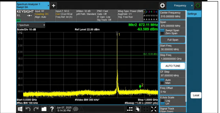
12-12-5MHz-10MHz-QPSK-QPSK-23058-23130-1RB#24-0RB#0- 30~1000MHz-PASS
