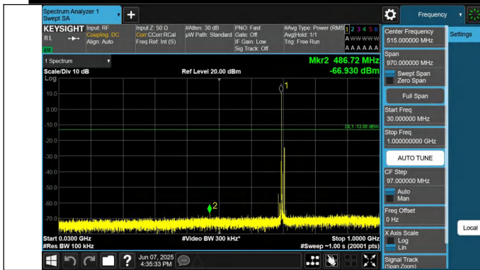
12-12-5MHz-5MHz-QPSK-QPSK-23071-23119-1RB#0-1RB#24-3 0~1000MHz-PASS
