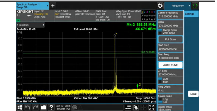
12-12-5MHz-10MHz-QPSK-QPSK-23048-23120-1RB#0-1RB#49- 30~1000MHz-PASS
