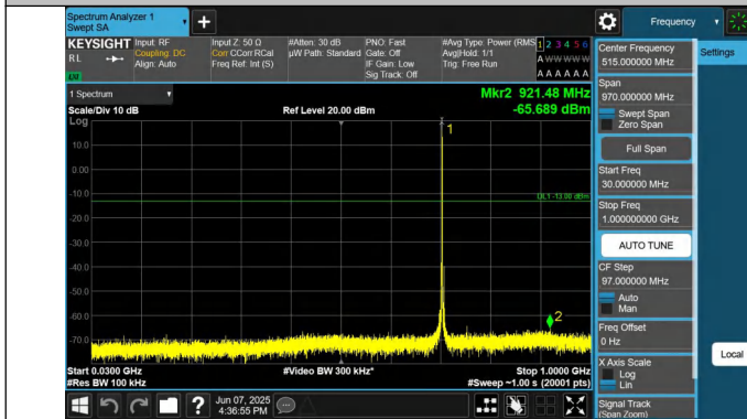
12-12-5MHz-5MHz-QPSK-QPSK-23107-23155-1RB#24-0RB#0-3 0~1000MHz-PASS
