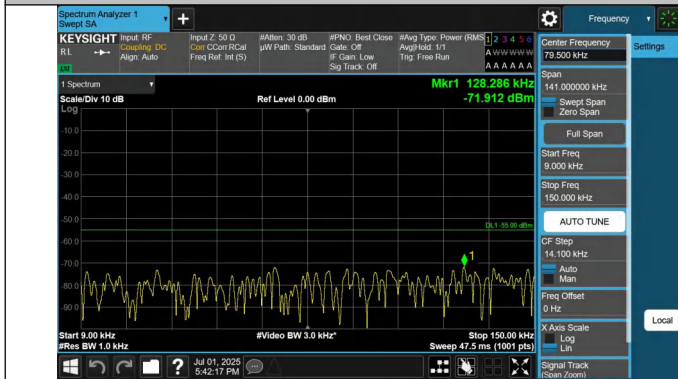
7-7-20MHz-20MHz-QPSK-QPSK-21152-21350-1RB#99-0RB#0-0 .009~0.15MHz-PASS
