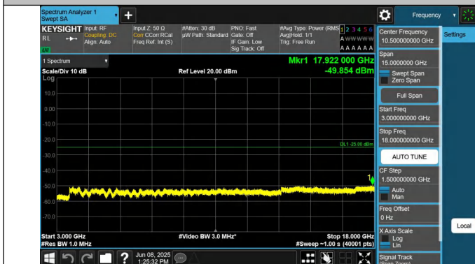
7-7-20MHz-20MHz-QPSK-QPSK-21001-21199-1RB#0-0RB#0-30 00~18000MHz-PASS
