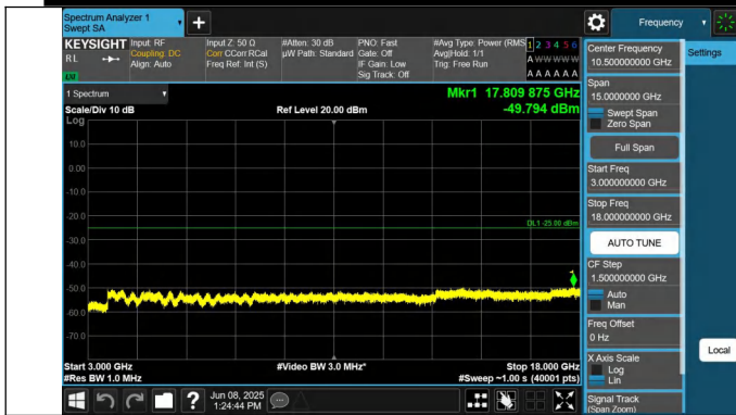
7-7-20MHz-20MHz-QPSK-QPSK-20850-21048-1RB#0-1RB#99-3000~18000MHz-PASS
