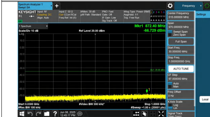
7-7-20MHz-15MHz-QPSK-QPSK-21026-21197-1RB#0-1RB#74-3 0~1000MHz-PASS
