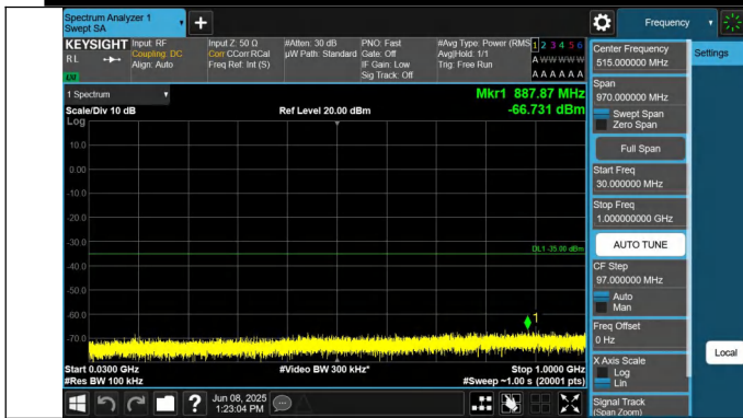
7-7-20MHz-20MHz-QPSK-QPSK-20850-21048-1RB#0-0RB#0-3 0~1000MHz-PASS
