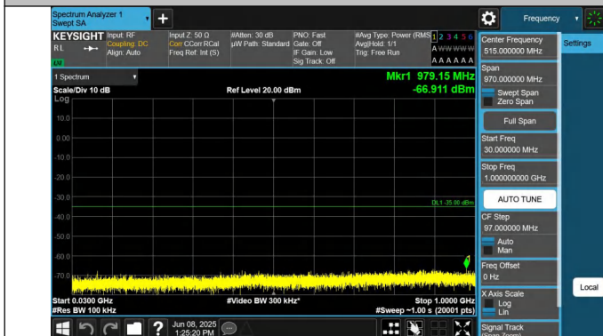
7-7-20MHz-20MHz-QPSK-QPSK-21001-21199-1RB#0-0RB#0-30 ~1000MHz-PASS
