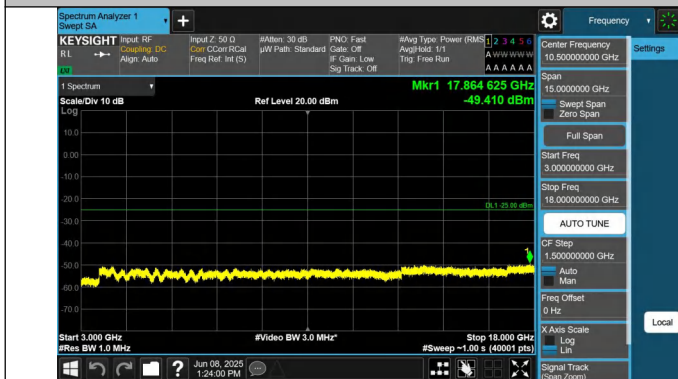
7-7-20MHz-20MHz-QPSK-QPSK-20850-21048-1RB#99-0RB#0-3000~18000MHz-PASS
