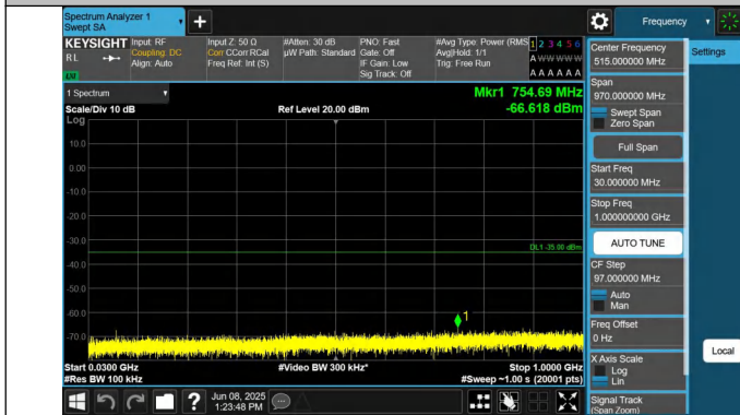
7-7-20MHz-20MHz-QPSK-QPSK-20850-21048-1RB#99-0RB#0-30~1000MHz-PASS
