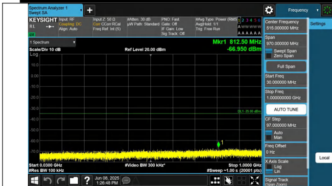
7-7-20MHz-20MHz-QPSK-QPSK-21001-21199-1RB#0-1RB#99-3 0~1000MHz-PASS
