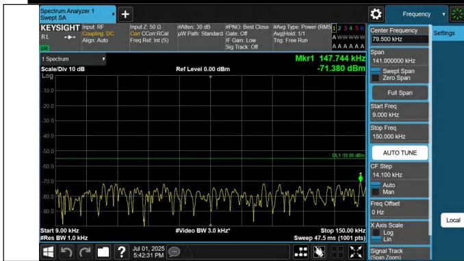
7-7-20MHz-20MHz-QPSK-QPSK-21152-21350-1RB#0-1RB#99-0 .009~0.15MHz-PASS
