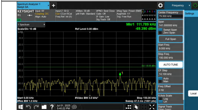
7-7-20MHz-15MHz-QPSK-QPSK-21201-21372-1RB#0-1RB#74- 0.009~0.15MHz-PASS
