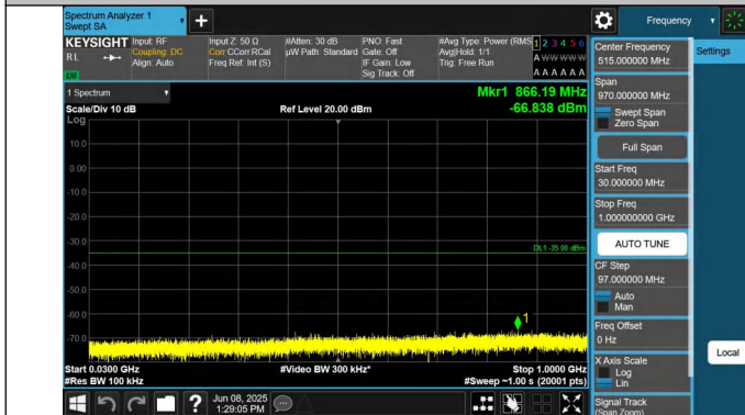
7-7-20MHz-20MHz-QPSK-QPSK-21152-21350-1RB#0-1RB#99-3 0~1000MHz-PASS
