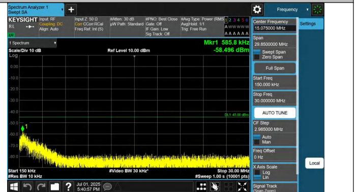
7-7-20MHz-20MHz-QPSK-QPSK-20850-21048-1RB#99-0RB#0-0.15~30MHz-PASS
