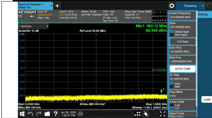
7-7-20MHz-20MHz-QPSK-QPSK-21152-21350-1RB#99-0RB#0-3 0~1000MHz-PASS
