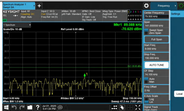
7-7-20MHz-20MHz-QPSK-QPSK-21001-21199-1RB#99-0RB#0-0 .009~0.15MHz-PASS
