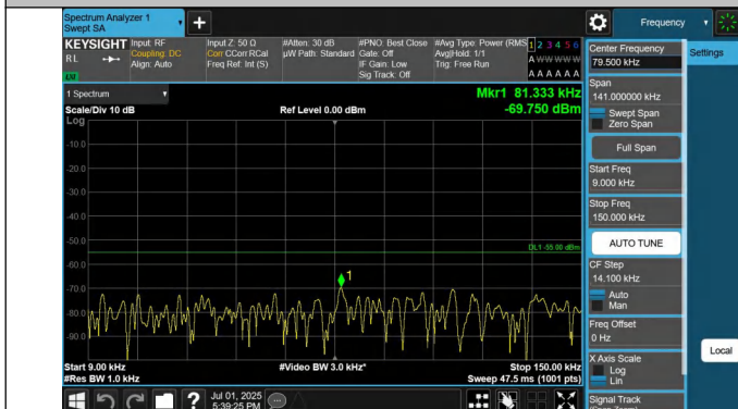
7-7-20MHz-15MHz-QPSK-QPSK-21026-21197-1RB#99-0RB#0-0 .009~0.15MHz-PASS
