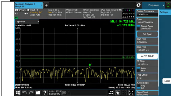
7-7-20MHz-15MHz-QPSK-QPSK-21026-21197-1RB#0-1RB#74-0 .009~0.15MHz-PASS
