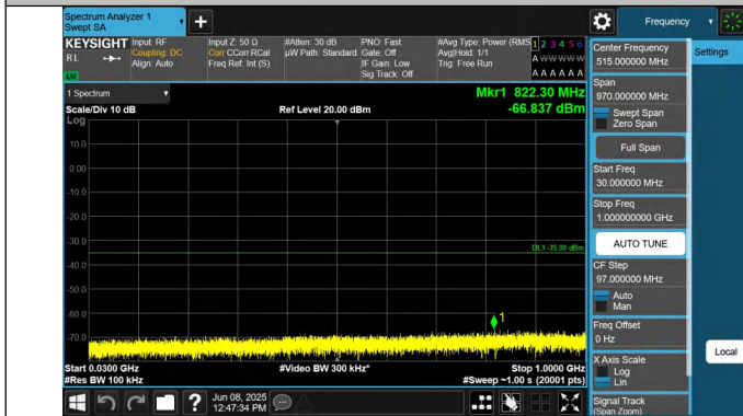
7-7-20MHz-15MHz-QPSK-QPSK-21201-21372-1RB#0-1RB#74- 30~1000MHz-PASS
