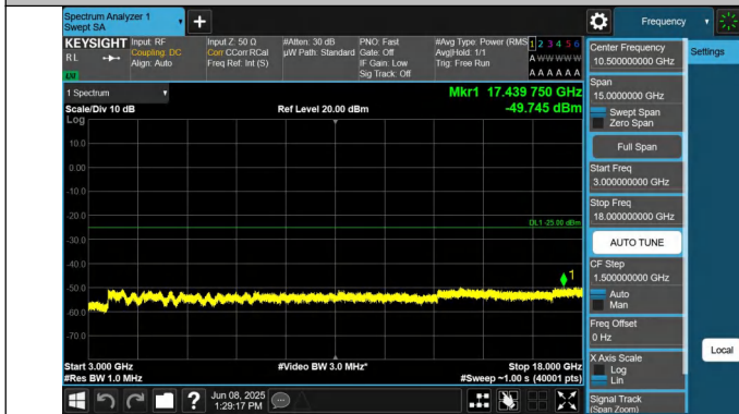
7-7-20MHz-20MHz-QPSK-QPSK-21152-21350-1RB#0-1RB#99-3 000~18000MHz-PASS
