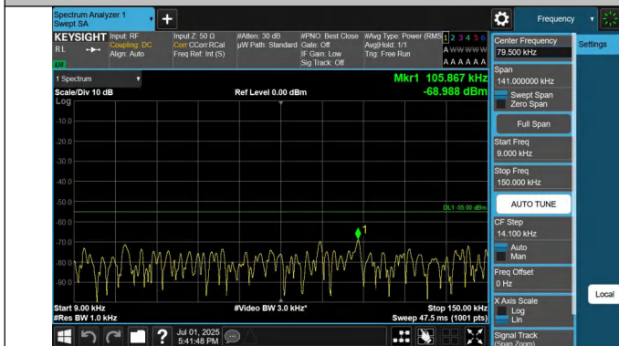
7-7-20MHz-20MHz-QPSK-QPSK-21001-21199-1RB#0-1RB#99-0 .009~0.15MHz-PASS
