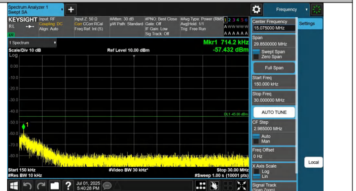
7-7-20MHz-15MHz-QPSK-QPSK-21201-21372-1RB#0-1RB#74-0. 15~30MHz-PASS
