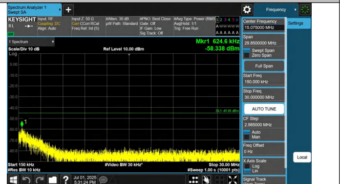
7-7-15MHz-10MHz-QPSK-QPSK-21277-21397-1RB#0-0RB#0-0.1 5~30MHz-PASS
