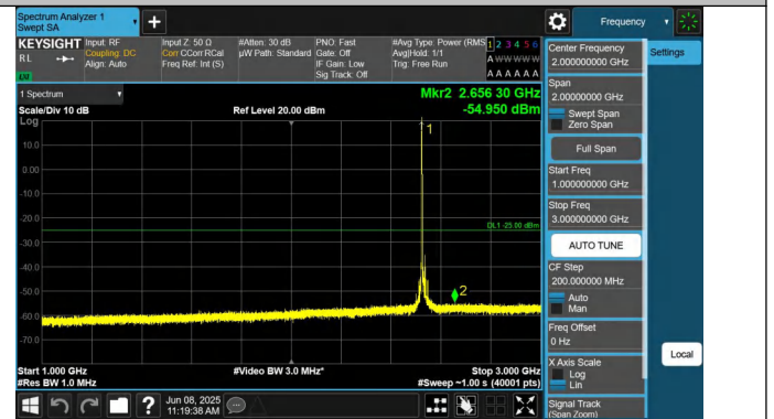
7-7-15MHz-10MHz-QPSK-QPSK-21051-21171-1RB#0-0RB#0-1000~3000MHz-PASS
