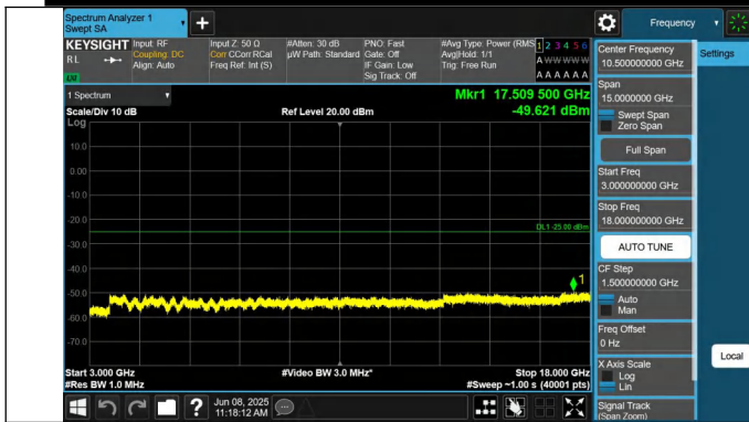
7-7-15MHz-10MHz-QPSK-QPSK-20825-20945-1RB#74-0RB#0-3000~18000MHz-PASS
