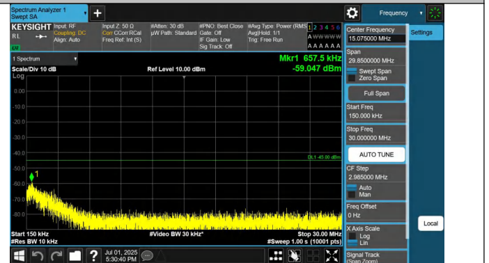
7-7-15MHz-10MHz-QPSK-QPSK-21051-21171-1RB#0-0RB#0-0.15~30MHz-PASS
