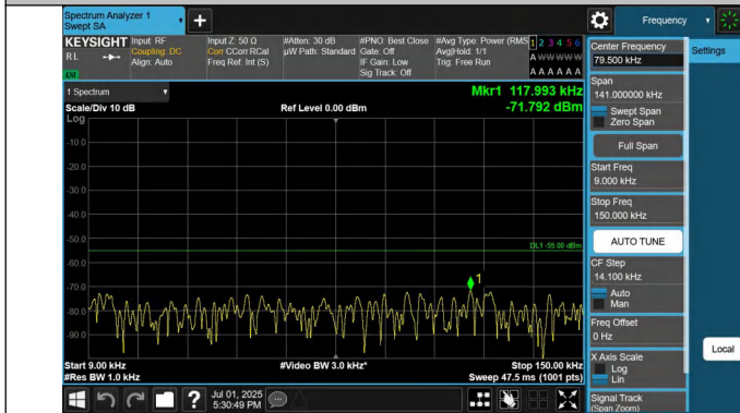
7-7-15MHz-10MHz-QPSK-QPSK-21051-21171-1RB#74-0RB#0-0 .009~0.15MHz-PASS
