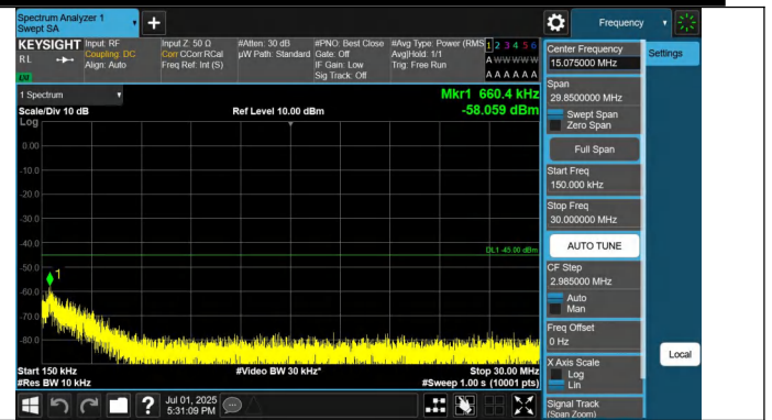
7-7-15MHz-10MHz-QPSK-QPSK-21051-21171-1RB#0-1RB#49-0 15~30MHz-PASS
