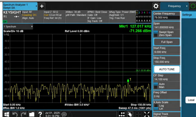
7-7-15MHz-10MHz-QPSK-QPSK-21277-21397-1RB#0-0RB#0-0. 009~0.15MHz-PASS
