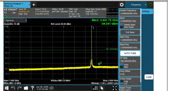
7-7-15MHz-15MHz-QPSK-QPSK-20825-20975-1RB#74-0RB#0-1000~3000MHz-PASS
