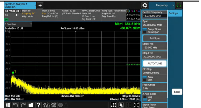
7-7-15MHz-15MHz-QPSK-QPSK-20825-20975-1RB#74-0RB#0-0.15~30MHz-PASS
