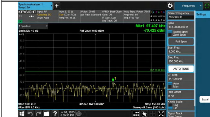
7-7-15MHz-10MHz-QPSK-QPSK-21051-21171-1RB#0-0RB#0-0.009~0.15MHz-PASS
