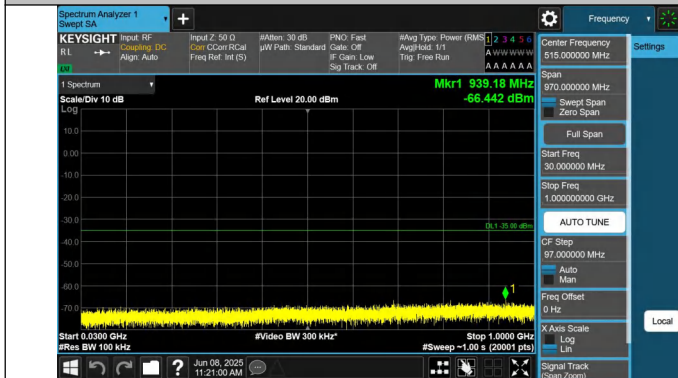
7-7-15MHz-10MHz-QPSK-QPSK-21051-21171-1RB#0-1RB#49-3 0~1000MHz-PASS
