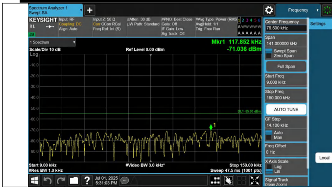
7-7-15MHz-10MHz-QPSK-QPSK-21051-21171-1RB#0-1RB#49-0 .009~0.15MHz-PASS
