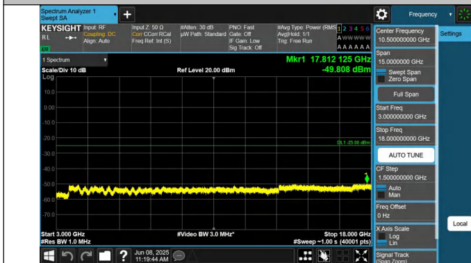
7-7-15MHz-10MHz-QPSK-QPSK-21051-21171-1RB#0-0RB#0-3000~18000MHz-PASS
