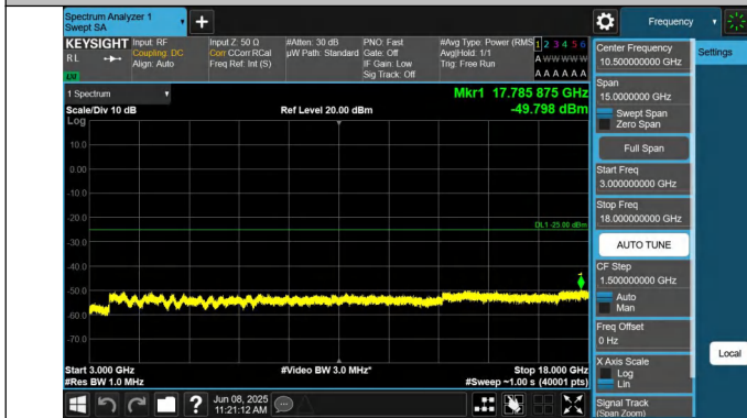
7-7-15MHz-10MHz-QPSK-QPSK-21051-21171-1RB#0-1RB#49-3 000~18000MHz-PASS
