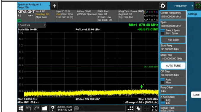
7-7-15MHz-15MHz-QPSK-QPSK-20825-20975-1RB#74-0RB#0-30~1000MHz-PASS
