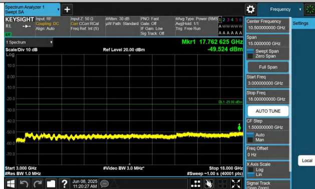
7-7-15MHz-10MHz-QPSK-QPSK-21051-21171-1RB#74-0RB#0-3 000~18000MHz-PASS
