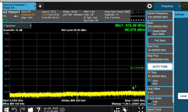
7-7-15MHz-10MHz-QPSK-QPSK-21277-21397-1RB#0-0RB#0-3 0~1000MHz-PASS
