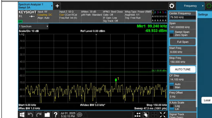
7-7-15MHz-15MHz-QPSK-QPSK-20825-20975-1RB#74-0RB#0-0.009~0.15MHz-PASS
