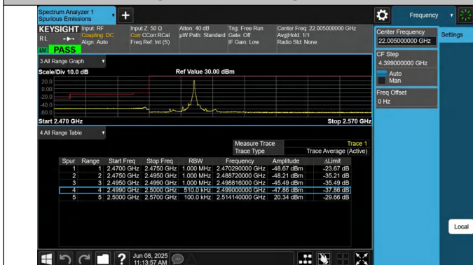
7-7-15MHz-10MHz-QPSK@QPSK-QPSK@QPSK-20825-20945-1RB#74@75RB#0-0RB#0@50RB#0-PASS
