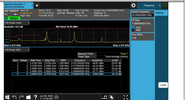
7-7-15MHz-10MHz-QPSK@QPSK-QPSK@QPSK-20825-20945-1RB#0@75RB#0-1RB#49@50RB#0-PASS
