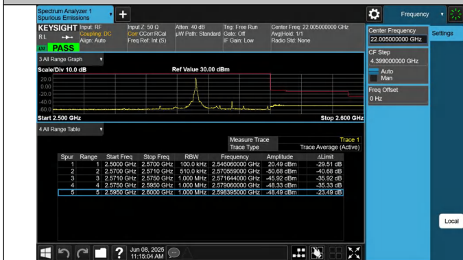
7-7-15MHz-10MHz-QPSK@QPSK-QPSK@QPSK-21277-21397-1RB#0@75RB#0-0RB#0@50RB#0-PASS
