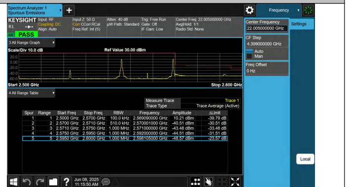
7-7-15MHz-10MHz-QPSK@QPSK-QPSK@QPSK-21277-21397-1RB#0@75RB#0-1RB#49@50RB#0-PASS
