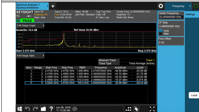
7-7-15MHz-10MHz-QPSK@QPSK-QPSK@QPSK-20825-20945-1RB#0@75RB#0-0RB#0@50RB#0-PASS
