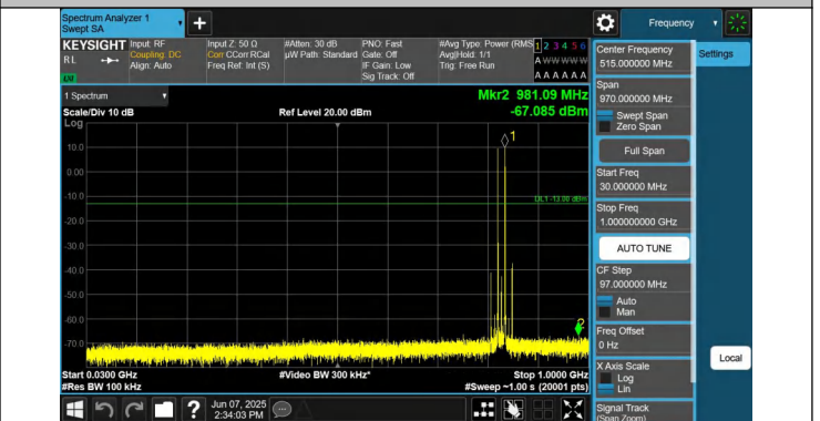
5-5-5MHz-10MHz-QPSK-QPSK-20428-20500-1RB#0-1RB#49-30 ~1000MHz-PASS
