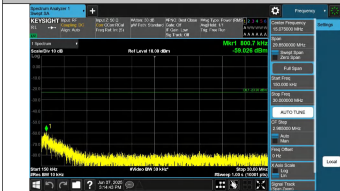
5-5-10MHz-5MHz-QPSK-QPSK-20450-20522-1RB#49-0RB#0-0. 15~30MHz-PASS
