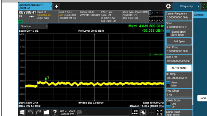
5-5-5MHz-10MHz-QPSK-QPSK-20528-20600-1RB#0-0RB#0-300 0~10000MHz-PASS
