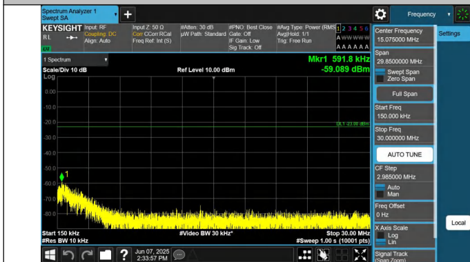
5-5-5MHz-10MHz-QPSK-QPSK-20428-20500-1RB#0-1RB#49-0 15~30MHz-PASS
