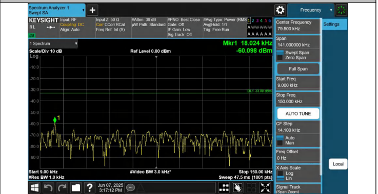
5-5-10MHz-5MHz-QPSK-QPSK-20500-20572-1RB#0-1RB#24-0. 009~0.15MHz-PASS
