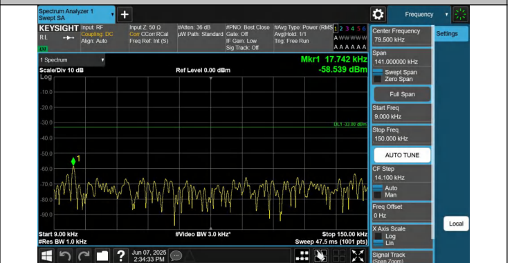
5-5-5MHz-10MHz-QPSK-QPSK-20478-20550-1RB#0-0RB#0-0.0 09~0.15MHz-PASS
