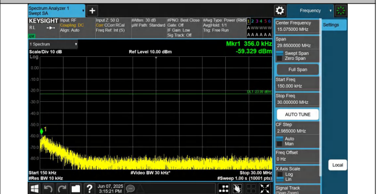
5-5-10MHz-5MHz-QPSK-QPSK-20450-20522-1RB#0-1RB#24-0. 15~30MHz-PASS
