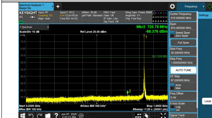
5-5-5MHz-10MHz-QPSK-QPSK-20528-20600-1RB#24-0RB#0-30 ~1000MHz-PASS
