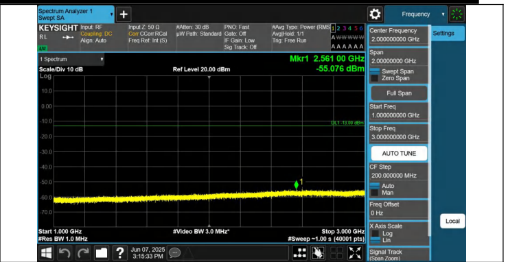
5-5-10MHz-5MHz-QPSK-QPSK-20450-20522-1RB#0-1RB#24-10 00~3000MHz-PASS
