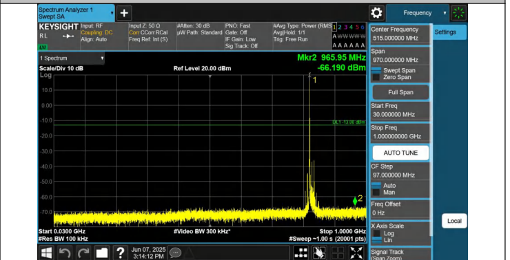
5-5-10MHz-5MHz-QPSK-QPSK-20450-20522-1RB#0-0RB#0-30~ 1000MHz-PASS
