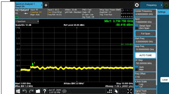
5-5-5MHz-10MHz-QPSK-QPSK-20528-20600-1RB#24-0RB#0-30 00~10000MHz-PASS
