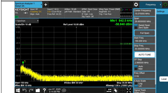
5-5-10MHz-5MHz-QPSK-QPSK-20450-20522-1RB#0-0RB#0-0.1 5~30MHz-PASS
