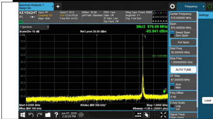
5-5-5MHz-10MHz-QPSK-QPSK-20428-20500-1RB#24-0RB#0-30 ~1000MHz-PASS
