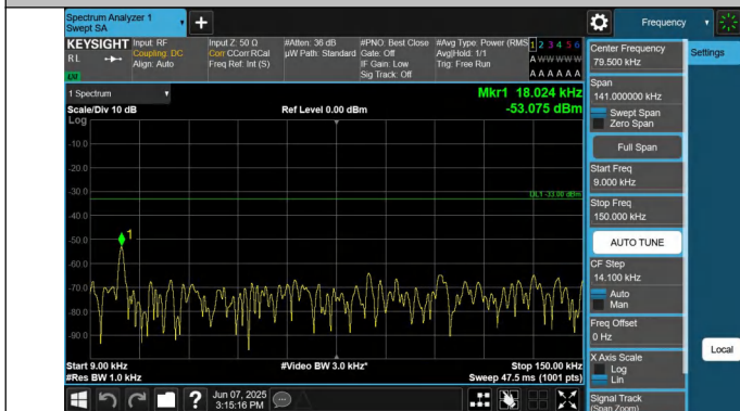
5-5-10MHz-5MHz-QPSK-QPSK-20450-20522-1RB#0-1RB#24-0. 009~0.15MHz-PASS
