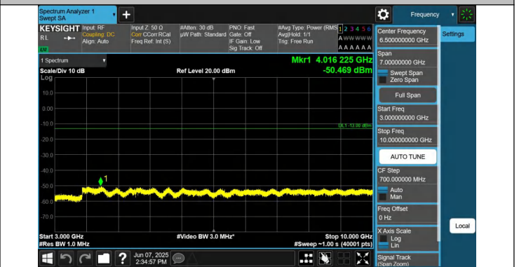
5-5-5MHz-10MHz-QPSK-QPSK-20478-20550-1RB#0-0RB#0-300 0~10000MHz-PASS
