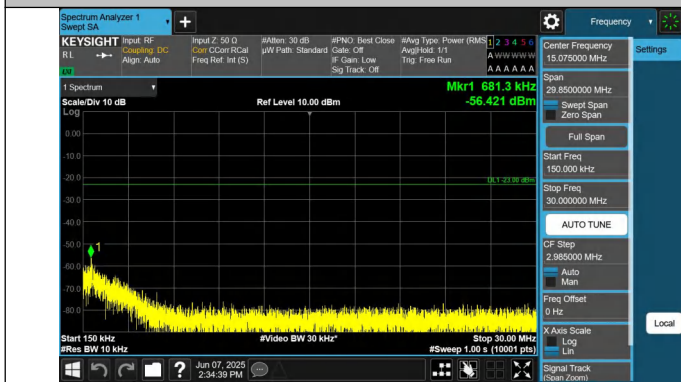
5-5-5MHz-10MHz-QPSK-QPSK-20478-20550-1RB#0-0RB#0-0.1 5~30MHz-PASS
