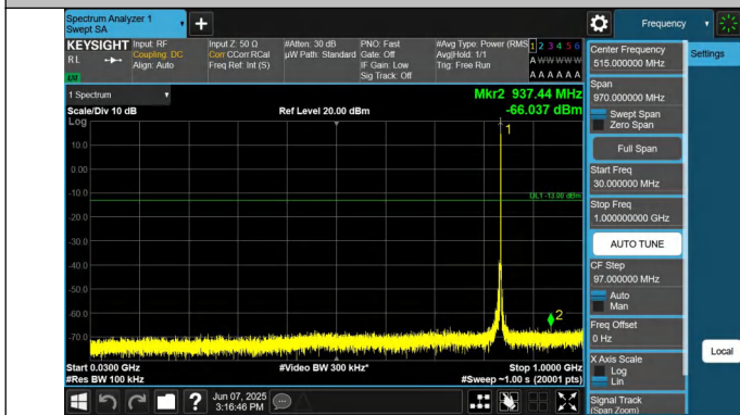
5-5-10MHz-5MHz-QPSK-QPSK-20500-20572-1RB#49-0RB#0-30 ~1000MHz-PASS
