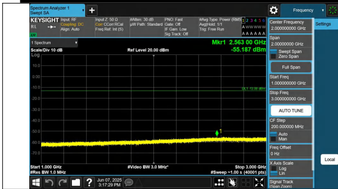
5-5-10MHz-5MHz-QPSK-QPSK-20500-20572-1RB#0-1RB#24-10 00~3000MHz-PASS
