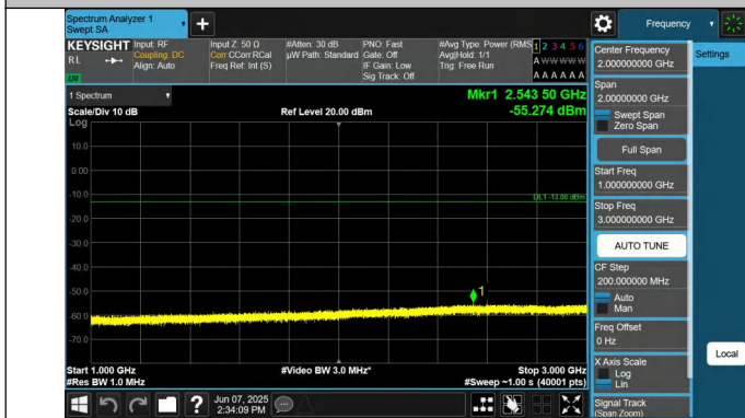
5-5-5MHz-10MHz-QPSK-QPSK-20428-20500-1RB#0-1RB#49-10 00~3000MHz-PASS
