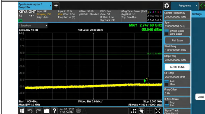
5-5-5MHz-10MHz-QPSK-QPSK-20528-20600-1RB#0-1RB#49-10 00~3000MHz-PASS
