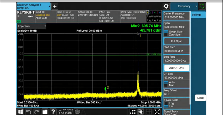
5-5-5MHz-10MHz-QPSK-QPSK-20478-20550-1RB#24-0RB#0-30 ~1000MHz-PASS
