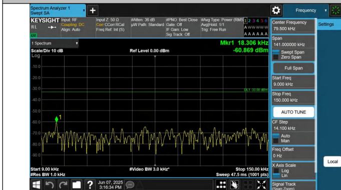
5-5-10MHz-5MHz-QPSK-QPSK-20500-20572-1RB#49-0RB#0-0. 009~0.15MHz-PASS
