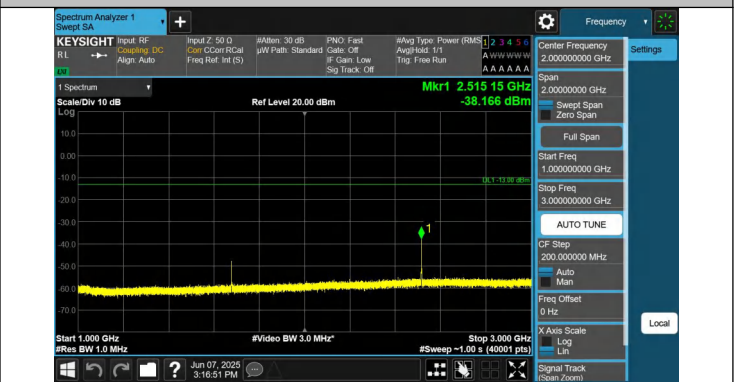
5-5-10MHz-5MHz-QPSK-QPSK-20500-20572-1RB#49-0RB#0-10 00~3000MHz-PASS
