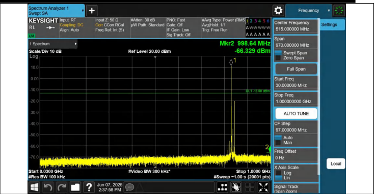
5-5-5MHz-10MHz-QPSK-QPSK-20528-20600-1RB#0-1RB#49-30 ~1000MHz-PASS
