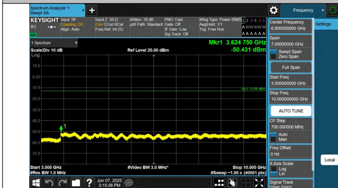
5-5-10MHz-5MHz-QPSK-QPSK-20450-20522-1RB#0-1RB#24-30 00~10000MHz-PASS
