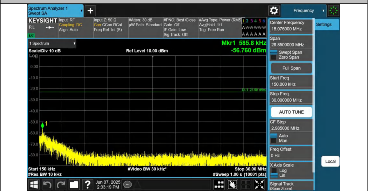
5-5-5MHz-10MHz-QPSK-QPSK-20428-20500-1RB#24-0RB#0-0 15~30MHz-PASS
