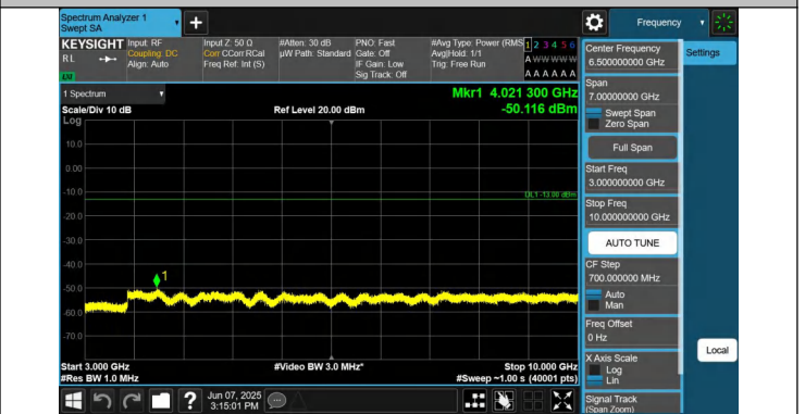
5-5-10MHz-5MHz-QPSK-QPSK-20450-20522-1RB#49-0RB#0-30 00~10000MHz-PASS
