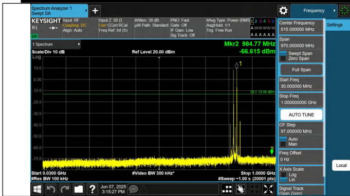
5-5-10MHz-5MHz-QPSK-QPSK-20450-20522-1RB#0-1RB#24-30 ~1000MHz-PASS
