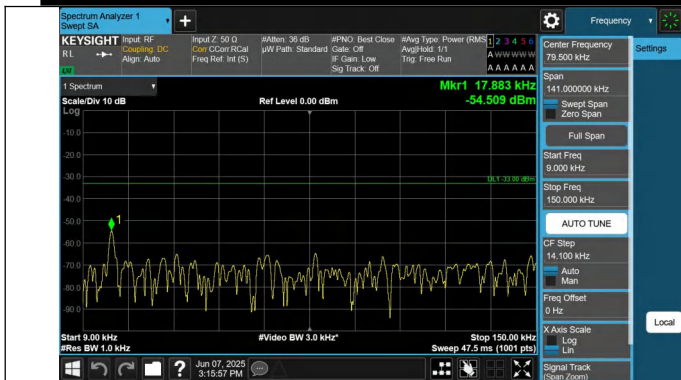
5-5-10MHz-5MHz-QPSK-QPSK-20500-20572-1RB#0-0RB#0-0.0 09~0.15MHz-PASS
