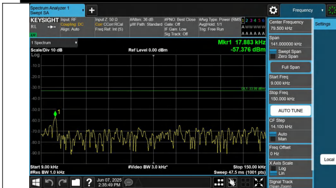
5-5-5MHz-10MHz-QPSK-QPSK-20478-20550-1RB#0-1RB#49-0. 009~0.15MHz-PASS
