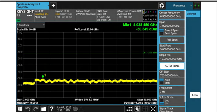
5-5-5MHz-10MHz-QPSK-QPSK-20528-20600-1RB#0-1RB#49-30 00~10000MHz-PASS
