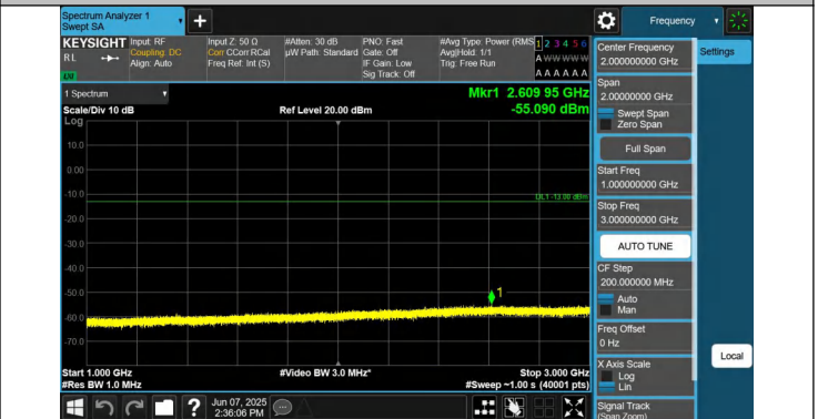
5-5-5MHz-10MHz-QPSK-QPSK-20478-20550-1RB#0-1RB#49-10 00~3000MHz-PASS
