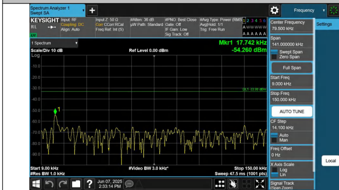
5-5-5MHz-10MHz-QPSK-QPSK-20428-20500-1RB#24-0RB#0-0 009~0.15MHz-PASS
