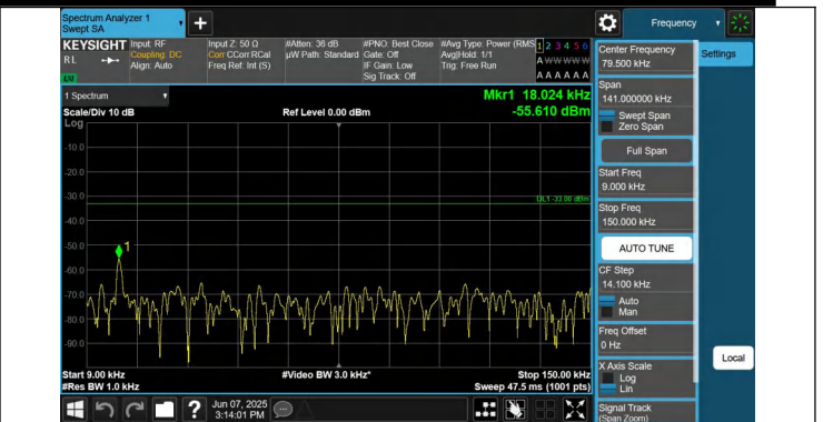
5-5-10MHz-5MHz-QPSK-QPSK-20450-20522-1RB#0-0RB#0-0.0 09~0.15MHz-PASS
