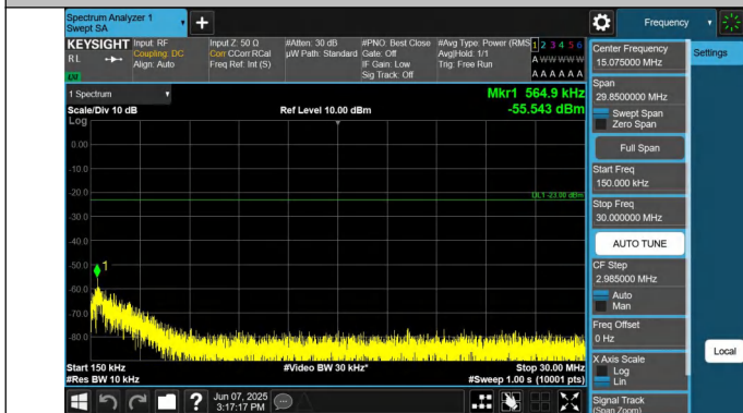
5-5-10MHz-5MHz-QPSK-QPSK-20500-20572-1RB#0-1RB#24-0. 15~30MHz-PASS
