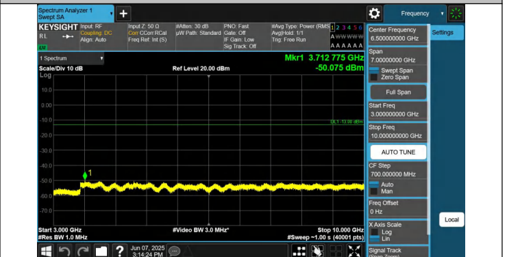
5-5-10MHz-5MHz-QPSK-QPSK-20450-20522-1RB#0-0RB#0-300 0~10000MHz-PASS
