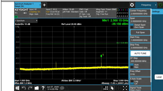
5-5-10MHz-5MHz-QPSK-QPSK-20450-20522-1RB#49-0RB#0-10 00~3000MHz-PASS
