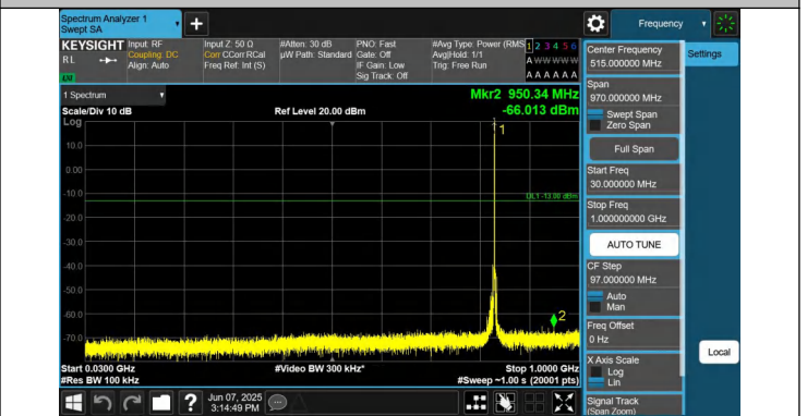
5-5-10MHz-5MHz-QPSK-QPSK-20450-20522-1RB#49-0RB#0-30 ~1000MHz-PASS
