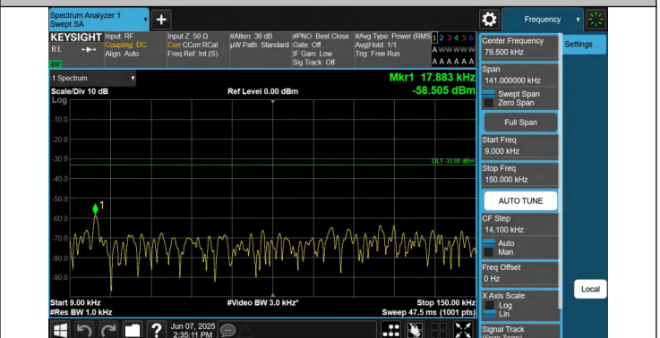
5-5-5MHz-10MHz-QPSK-QPSK-20478-20550-1RB#24-0RB#0-0. 009~0.15MHz-PASS
