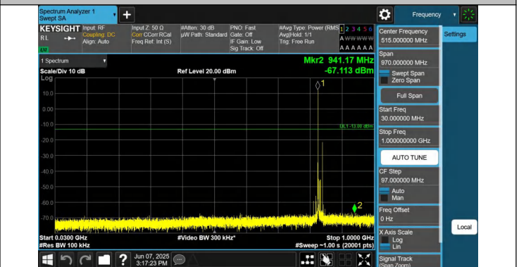
5-5-10MHz-5MHz-QPSK-QPSK-20500-20572-1RB#0-1RB#24-30 ~1000MHz-PASS
