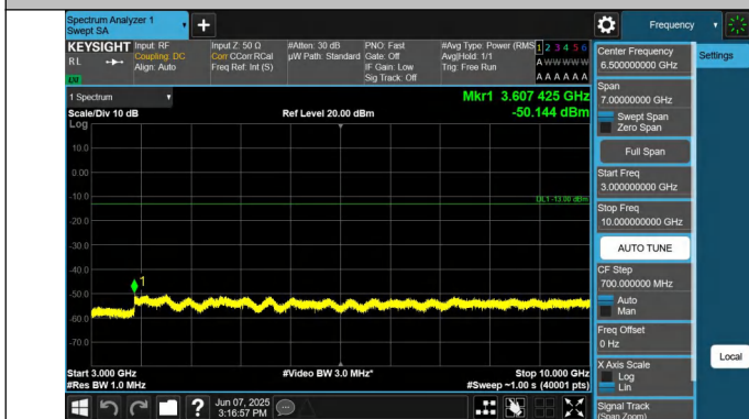
5-5-10MHz-5MHz-QPSK-QPSK-20500-20572-1RB#49-0RB#0-30 00~10000MHz-PASS
