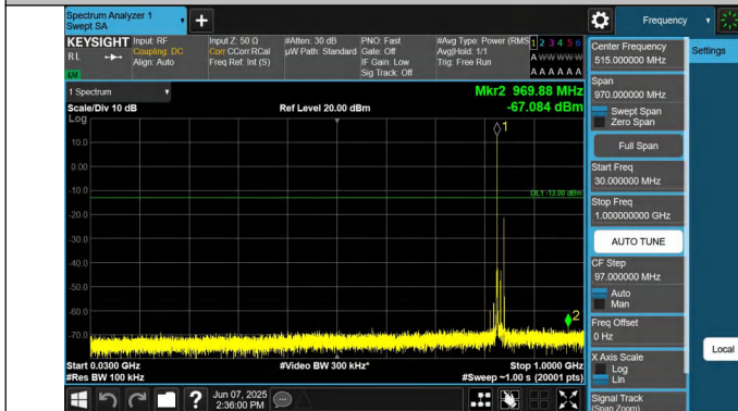
5-5-5MHz-10MHz-QPSK-QPSK-20478-20550-1RB#0-1RB#49-30 ~1000MHz-PASS
