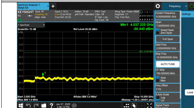
5-5-5MHz-10MHz-QPSK-QPSK-20478-20550-1RB#0-1RB#49-30 00~10000MHz-PASS
