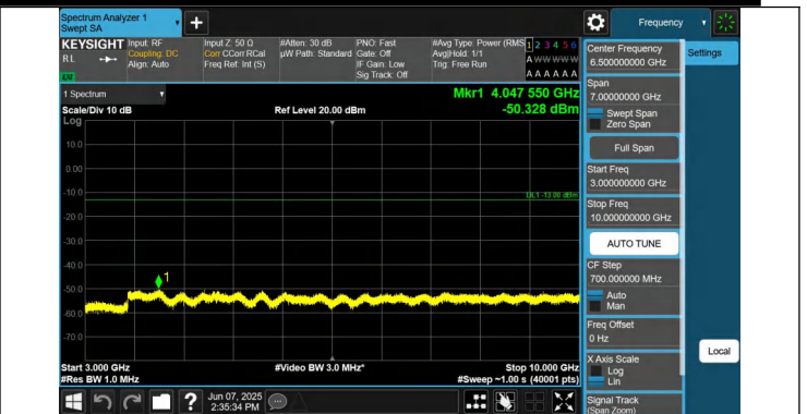
5-5-5MHz-10MHz-QPSK-QPSK-20478-20550-1RB#24-0RB#0-30 00~10000MHz-PASS
