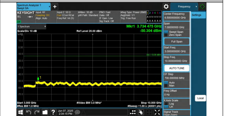
5-5-5MHz-10MHz-QPSK-QPSK-20428-20500-1RB#0-1RB#49-30 00~10000MHz-PASS
