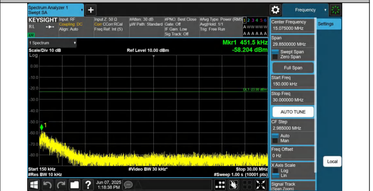
5-5-3MHz-5MHz-QPSK-QPSK-20416-20455-1RB#14-0RB#0-0.1 5~30MHz-PASS
