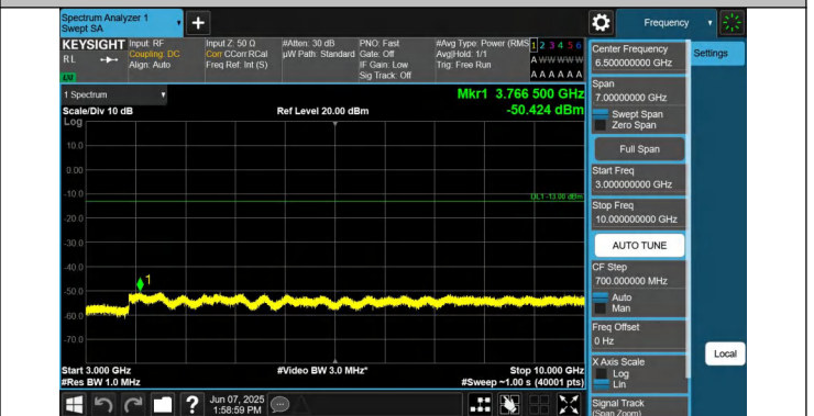
5-5-5MHz-3MHz-QPSK-QPSK-20510-20549-1RB#0-1RB#15-3000~10000MHz-PASS
