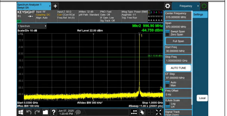
5-5-3MHz-5MHz-QPSK-QPSK-20501-20540-1RB#14-0RB#0-30~1000MHz-PASS
