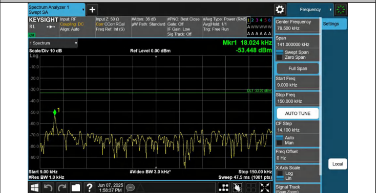
5-5-5MHz-3MHz-QPSK-QPSK-20510-20549-1RB#0-1RB#15-0.009~0.15MHz-PASS
