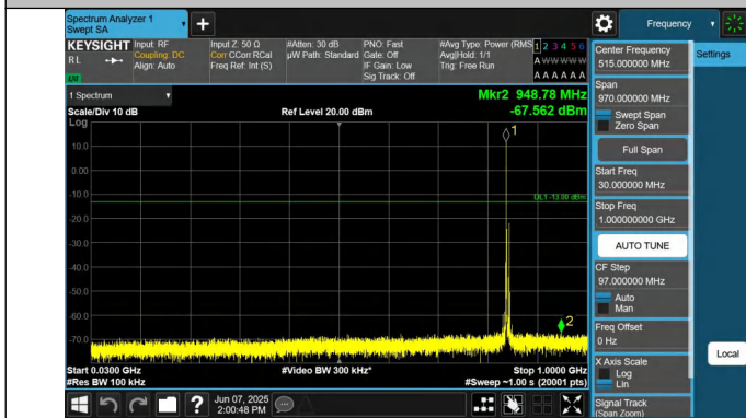
5-5-5MHz-3MHz-QPSK-QPSK-20595-20634-1RB#0-1RB#15-30~ 1000MHz-PASS
