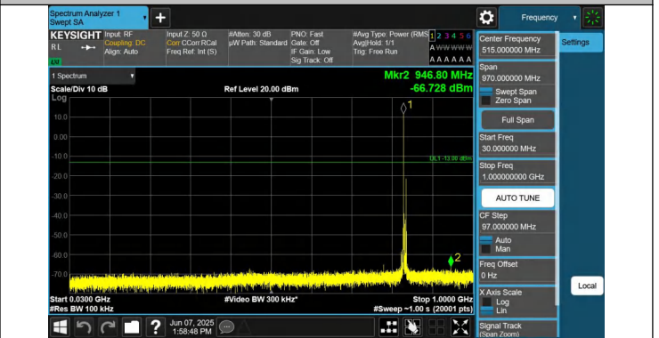
5-5-5MHz-3MHz-QPSK-QPSK-20510-20549-1RB#0-1RB#15-30~1000MHz-PASS
