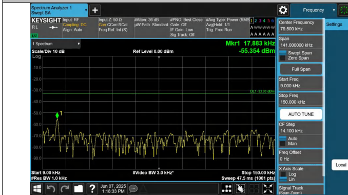
5-5-3MHz-5MHz-QPSK-QPSK-20416-20455-1RB#14-0RB#0-0.0 09~0.15MHz-PASS
