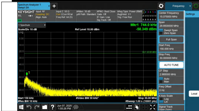
5-5-5MHz-3MHz-QPSK-QPSK-20425-20464-1RB#0-0RB#0-0.15 ~30MHz-PASS
