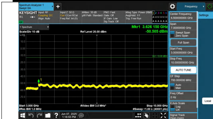
5-5-3MHz-5MHz-QPSK-QPSK-20416-20455-1RB#14-0RB#0-300 0~10000MHz-PASS
