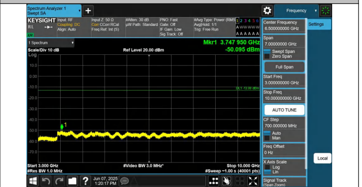
5-5-3MHz-5MHz-QPSK-QPSK-20501-20540-1RB#0-0RB#0-3000 ~10000MHz-PASS
