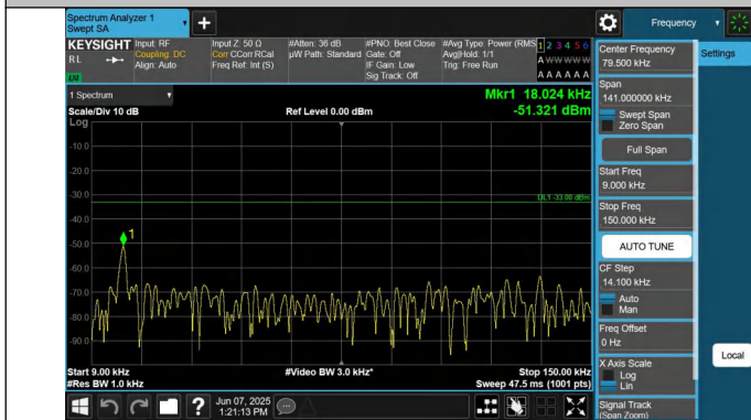
5-5-3MHz-5MHz-QPSK-QPSK-20501-20540-1RB#0-1RB#24-0.0 09~0.15MHz-PASS
