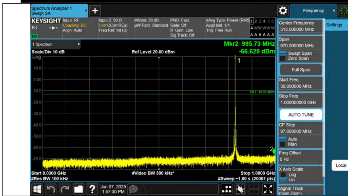
5-5-5MHz-3MHz-QPSK-QPSK-20510-20549-1RB#0-ORB#0-30~1000MHz-PASS
