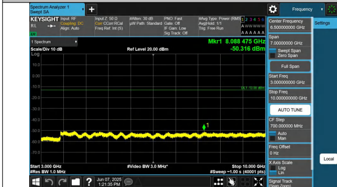
5-5-3MHz-5MHz-QPSK-QPSK-20501-20540-1RB#0-1RB#24-3000~10000MHz-PASS
