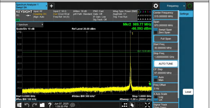
5-5-5MHz-3MHz-QPSK-QPSK-20595-20634-1RB#0-ORB#0-30~1 000MHz-PASS
