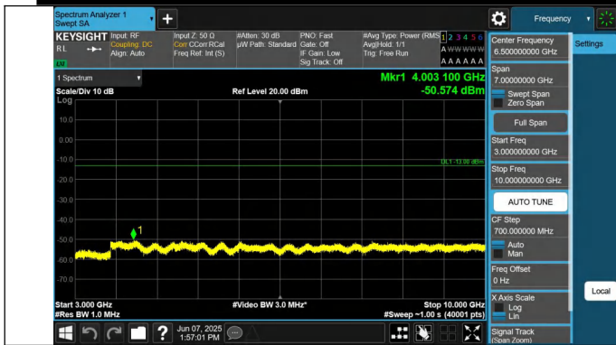
5-5-5MHz-3MHz-QPSK-QPSK-20425-20464-1RB#0-1RB#15-300 0~10000MHz-PASS
