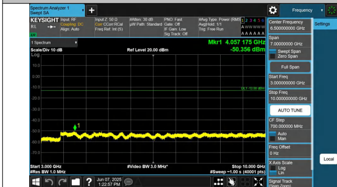
5-5-3MHz-5MHz-QPSK-QPSK-20586-20625-1RB#14-ORB#0-300 0~10000MHz-PASS
