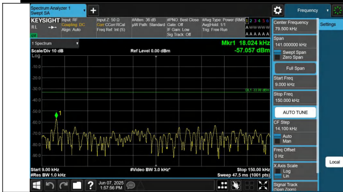
5-5-5MHz-3MHz-QPSK-QPSK-20510-20549-1RB#24-ORB#0-0.0 09~0.15MHz-PASS
