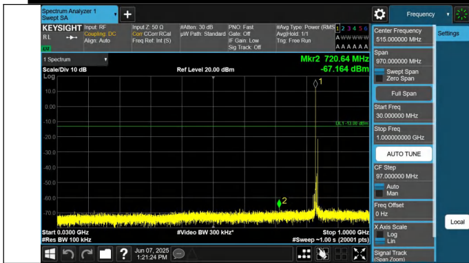
5-5-3MHz-5MHz-QPSK-QPSK-20501-20540-1RB#0-1RB#24-30~1000MHz-PASS
