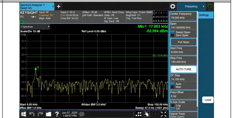
5-5-5MHz-3MHz-QPSK-QPSK-20595-20634-1RB#24-ORB#0-0.0 09~0.15MHz-PASS
