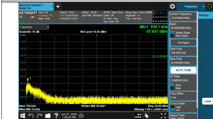
5-5-5MHz-3MHz-QPSK-QPSK-20425-20464-1RB#24-0RB#0-0.1 5~30MHz-PASS
