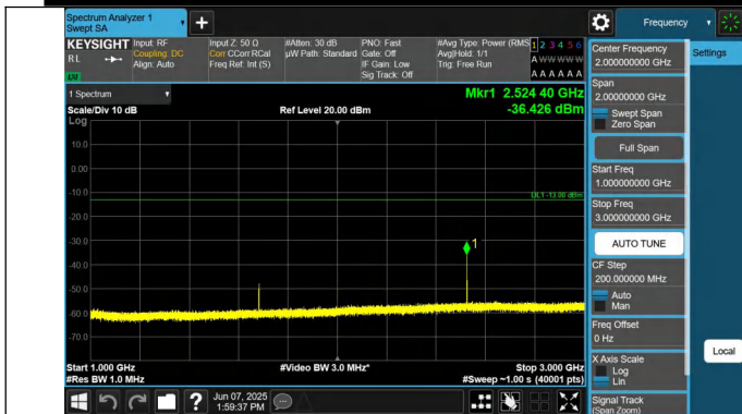
5-5-5MHz-3MHz-QPSK-QPSK-20595-20634-1RB#0-ORB#0-1000 ~3000MHz-PASS
