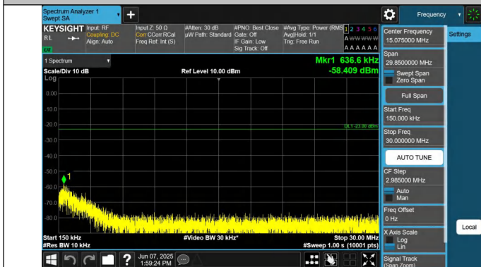
5-5-5MHz-3MHz-QPSK-QPSK-20595-20634-1RB#0-ORB#0-0.15 ~30MHz-PASS
