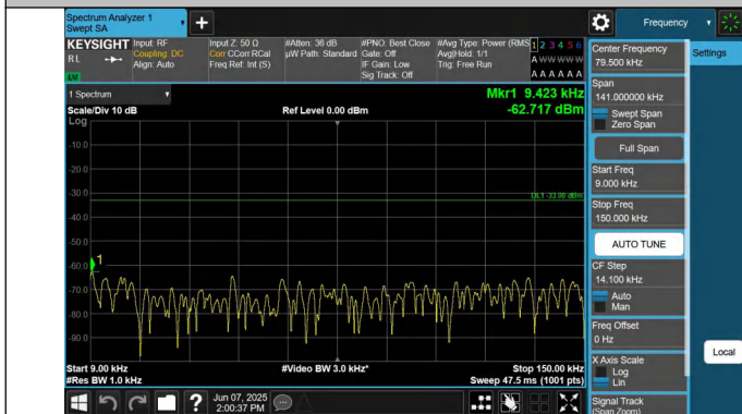
5-5-5MHz-3MHz-QPSK-QPSK-20595-20634-1RB#0-1RB#15-0.0 09~0.15MHz-PASS
