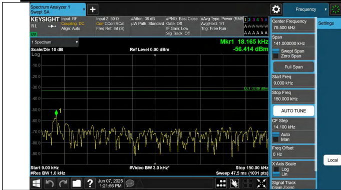
5-5-3MHz-5MHz-QPSK-QPSK-20586-20625-1RB#0-0RB#0-0.00 9~0.15MHz-PASS
