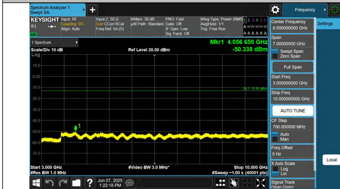
5-5-3MHz-5MHz-QPSK-QPSK-20586-20625-1RB#0-0RB#0-3000 ~10000MHz-PASS
