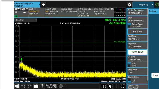
5-5-5MHz-3MHz-QPSK-QPSK-20510-20549-1RB#0-1RB#15-0.15~30MHz-PASS
