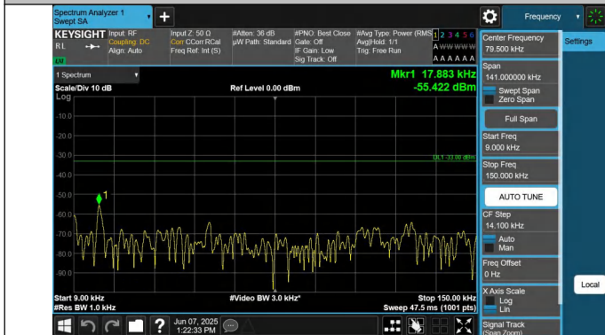
5-5-3MHz-5MHz-QPSK-QPSK-20586-20625-1RB#14-ORB#0-0.0 09~0.15MHz-PASS
