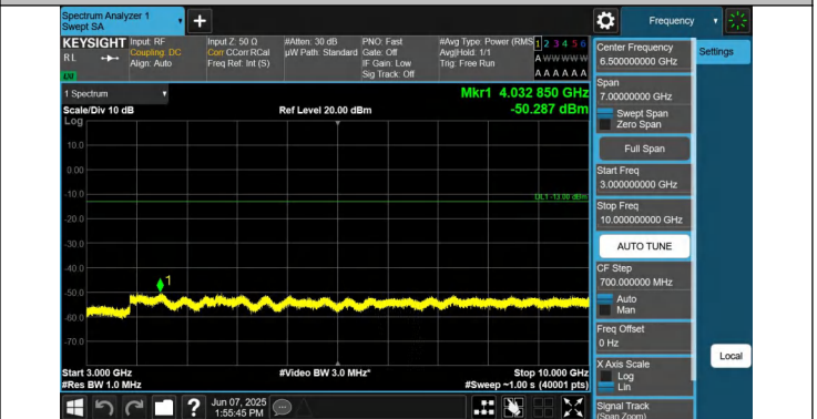
5-5-5MHz-3MHz-QPSK-QPSK-20425-20464-1RB#0-0RB#0-3000 ~10000MHz-PASS
