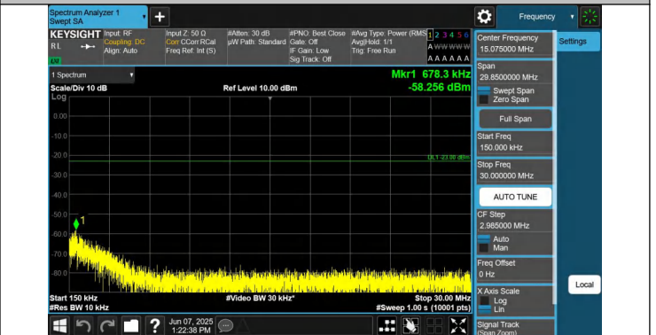
5-5-3MHz-5MHz-QPSK-QPSK-20586-20625-1RB#14-ORB#0-0.1 5~30MHz-PASS
