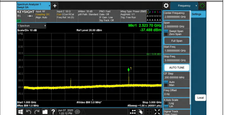
5-5-3MHz-5MHz-QPSK-QPSK-20586-20625-1RB#0-0RB#0-1000 ~3000MHz-PASS
