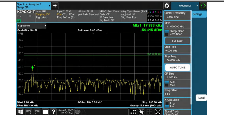
5-5-3MHz-5MHz-QPSK-QPSK-20501-20540-1RB#14-0RB#0-0.009~0.15MHz-PASS
