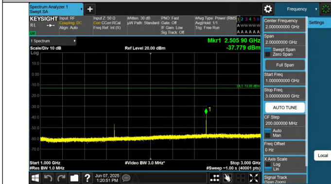
5-5-3MHz-5MHz-QPSK-QPSK-20501-20540-1RB#14-0RB#0-1000~3000MHz-PASS
