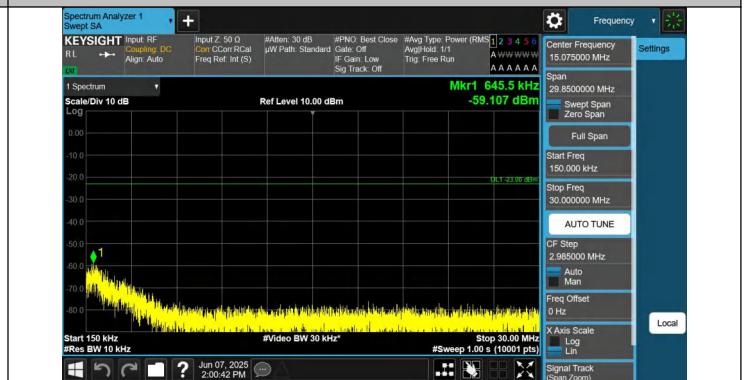
5-5-5MHz-3MHz-QPSK-QPSK-20595-20634-1RB#0-1RB#15-0.1 5~30MHz-PASS
