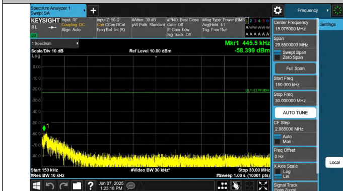
5-5-3MHz-5MHz-QPSK-QPSK-20586-20625-1RB#0-1RB#24-0.1 5~30MHz-PASS
