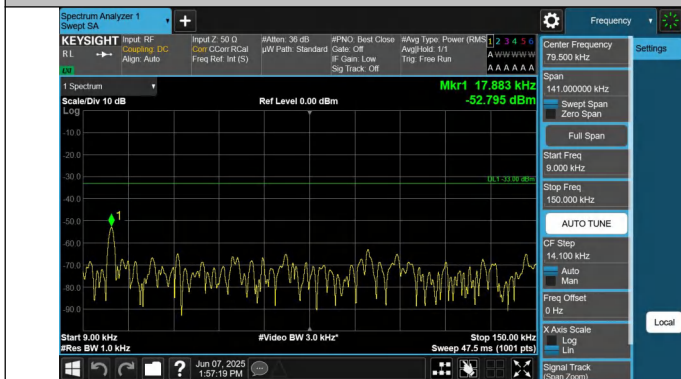
5-5-5MHz-3MHz-QPSK-QPSK-20510-20549-1RB#0-0RB#0-0.00 9~0.15MHz-PASS
