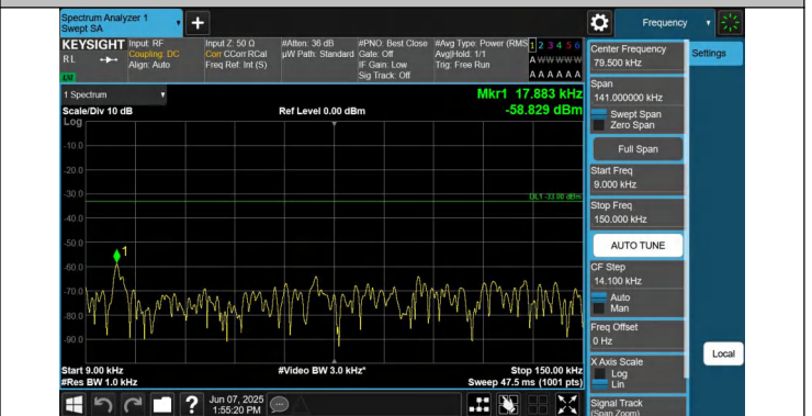
5-5-5MHz-3MHz-QPSK-QPSK-20425-20464-1RB#0-ORB#0-0.00 9~0.15MHz-PASS
