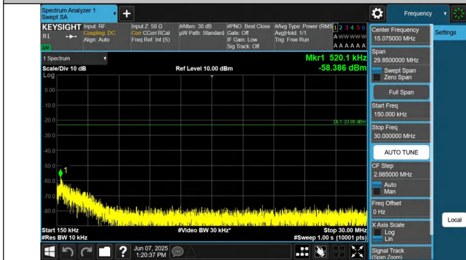
5-5-3MHz-5MHz-QPSK-QPSK-20501-20540-1RB#14-0RB#0-0.15~30MHz-PASS
