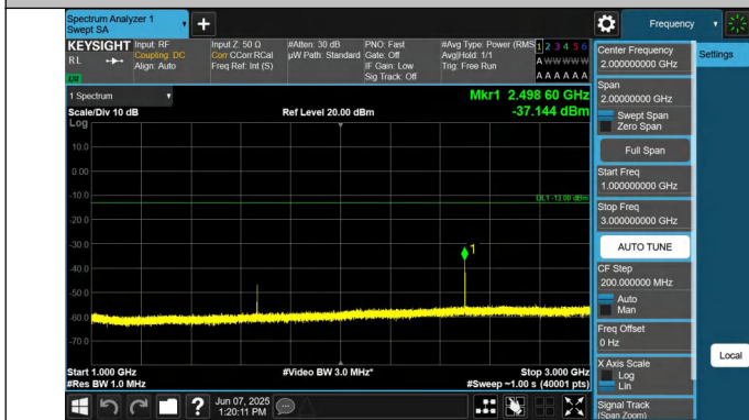
5-5-3MHz-5MHz-QPSK-QPSK-20501-20540-1RB#0-0RB#0-1000 ~3000MHz-PASS
