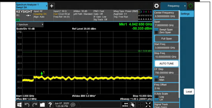
5-5-3MHz-5MHz-QPSK-QPSK-20586-20625-1RB#0-1RB#24-300 0~10000MHz-PASS
