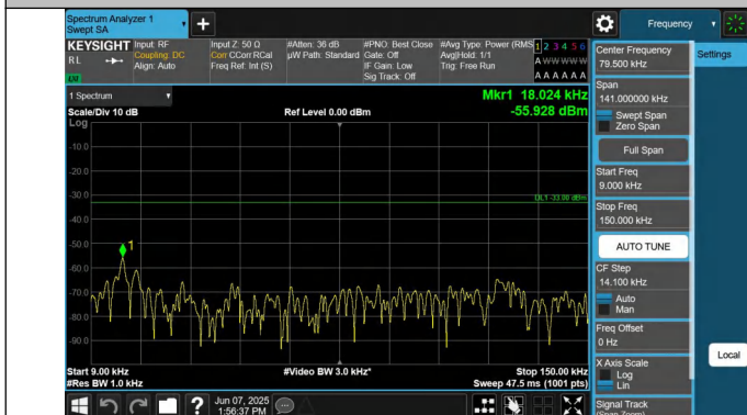
5-5-5MHz-3MHz-QPSK-QPSK-20425-20464-1RB#0-1RB#15-0.0 09~0.15MHz-PASS
