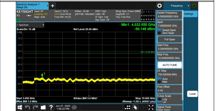
5-5-5MHz-3MHz-QPSK-QPSK-20425-20464-1RB#24-0RB#0-300 0~10000MHz-PASS
