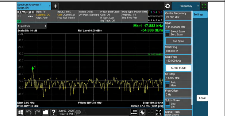
5-5-3MHz-5MHz-QPSK-QPSK-20586-20625-1RB#0-1RB#24-0.0 09~0.15MHz-PASS
