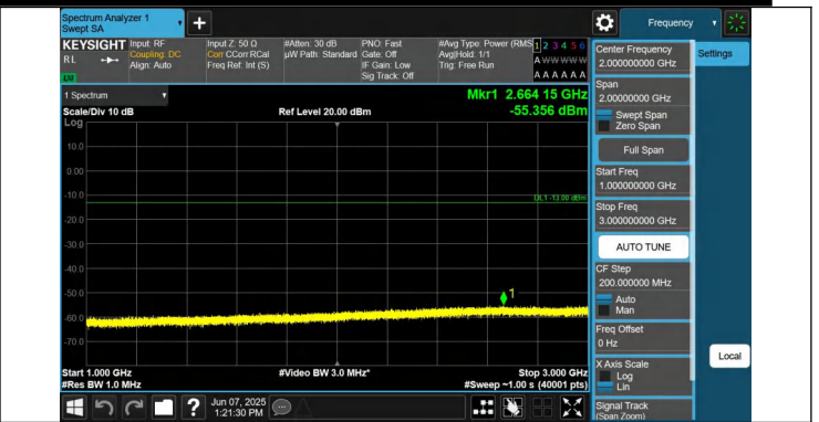
5-5-3MHz-5MHz-QPSK-QPSK-20501-20540-1RB#0-1RB#24-1000~3000MHz-PASS
