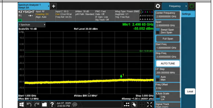
5-5-5MHz-3MHz-QPSK-QPSK-20595-20634-1RB#0-1RB#15-100 0~3000MHz-PASS
