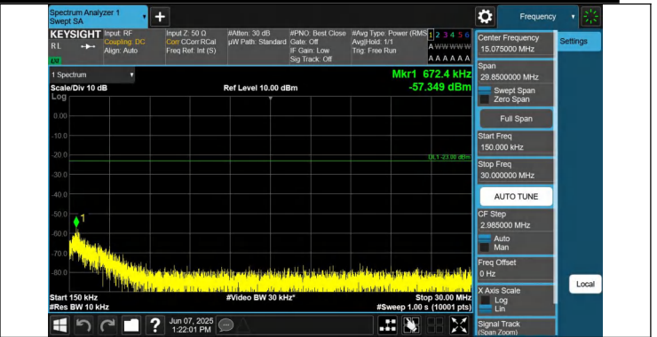
5-5-3MHz-5MHz-QPSK-QPSK-20586-20625-1RB#0-0RB#0-0.15 ~30MHz-PASS
