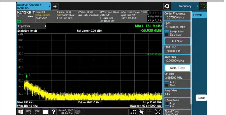
5-5-5MHz-3MHz-QPSK-QPSK-20510-20549-1RB#0-0RB#0-0.15 ~30MHz-PASS
