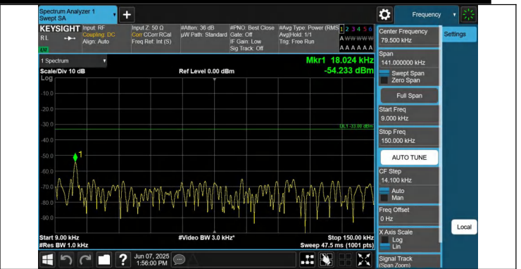
5-5-5MHz-3MHz-QPSK-QPSK-20425-20464-1RB#24-0RB#0-0.0 09~0.15MHz-PASS
