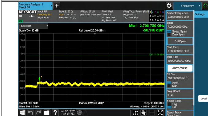
5-5-5MHz-3MHz-QPSK-QPSK-20510-20549-1RB#0-ORB#0-3000~10000MHz-PASS
