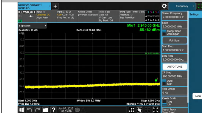
5-5-5MHz-3MHz-QPSK-QPSK-20510-20549-1RB#0-1RB#15-1000~3000MHz-PASS
