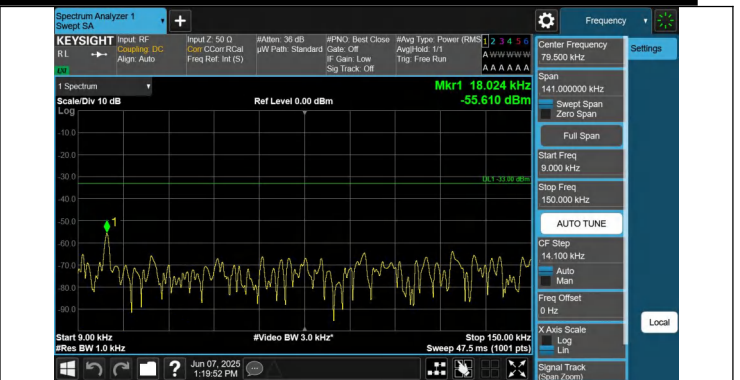
5-5-3MHz-5MHz-QPSK-QPSK-20501-20540-1RB#0-0RB#0-0.00 9~0.15MHz-PASS
