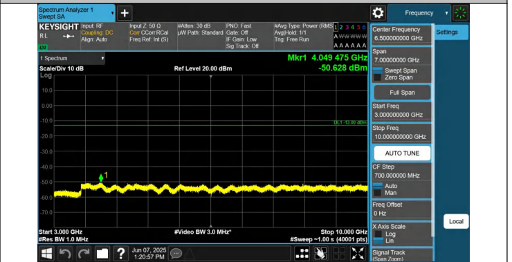
5-5-3MHz-5MHz-QPSK-QPSK-20501-20540-1RB#14-0RB#0-3000~10000MHz-PASS
