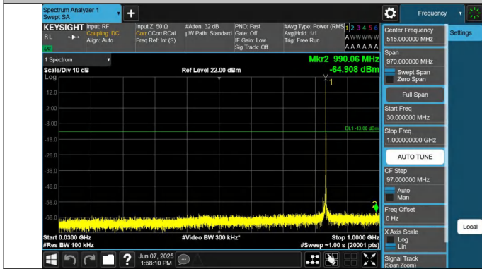
5-5-5MHz-3MHz-QPSK-QPSK-20510-20549-1RB#24-ORB#0-30~ 1000MHz-PASS
