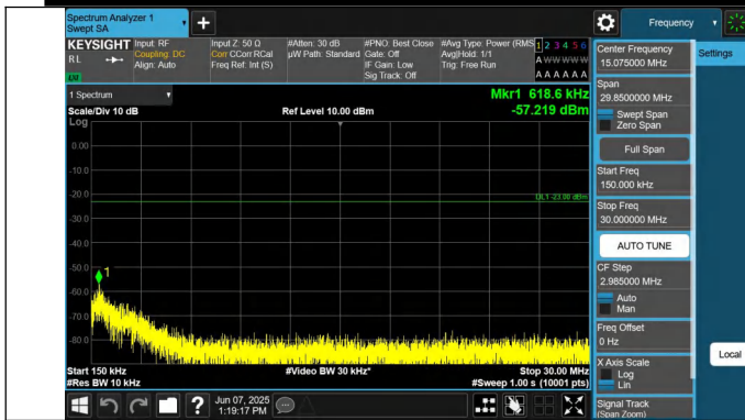
5-5-3MHz-5MHz-QPSK-QPSK-20416-20455-1RB#0-1RB#24-0.1 5~30MHz-PASS
