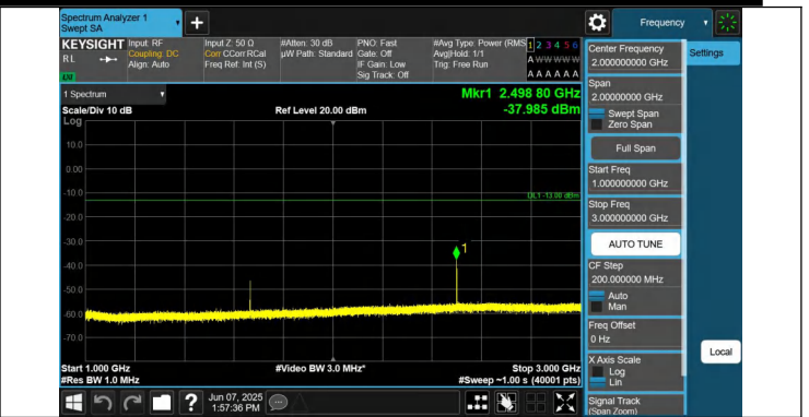
5-5-5MHz-3MHz-QPSK-QPSK-20510-20549-1RB#0-ORB#0-1000~3000MHz-PASS
