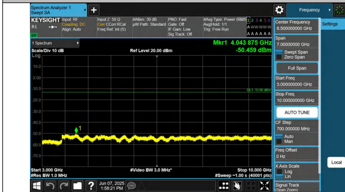
5-5-5MHz-3MHz-QPSK-QPSK-20510-20549-1RB#24-ORB#0-300 0~10000MHz-PASS
