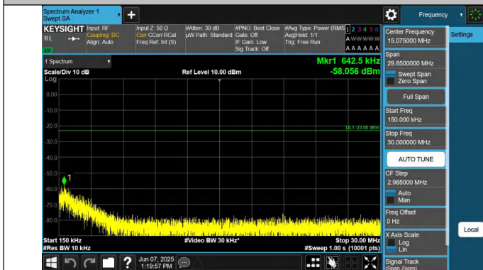
5-5-3MHz-5MHz-QPSK-QPSK-20501-20540-1RB#0-0RB#0-0.15 ~30MHz-PASS
