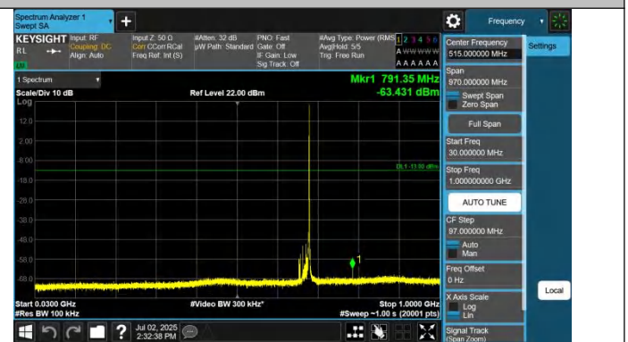
Band71-15MHz-QPSK-133297-1RB#74-30~1000-PASS
