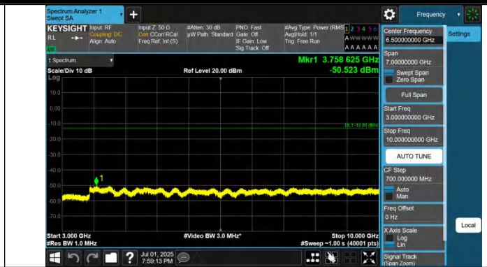
Band71-15MHz-QPSK-133397-1RB#74-3000~10000-PASS
