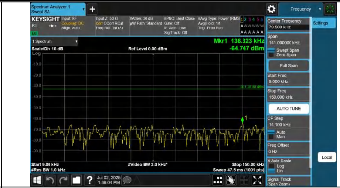
Band71-20MHz-QPSK-133322-1RB#99-0.009~0.15-PASS
