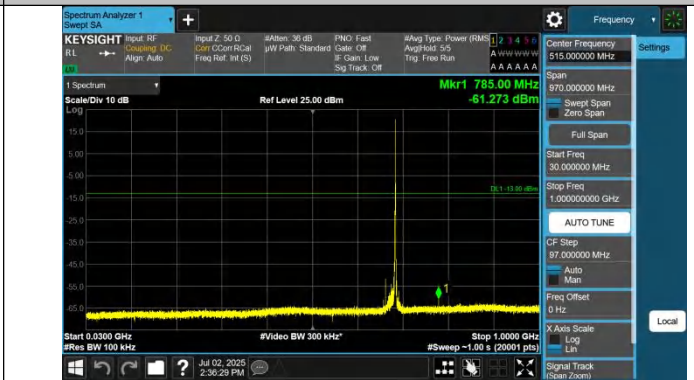
Band71-20MHz-QPSK-133322-1RB#99-30~1000-PASS
