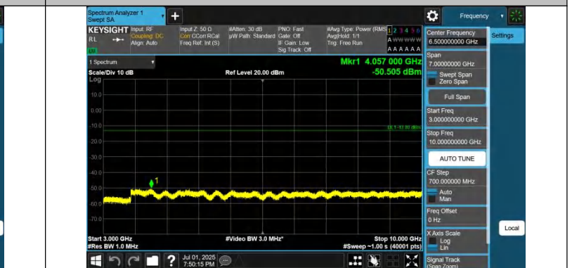
Band71-10MHz-QPSK-133422-1RB#49-3000~10000-PASS
