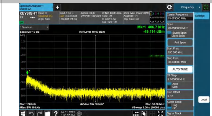
Band71-20MHz-QPSK-133372-1RB#0-0.15~30-PASS
