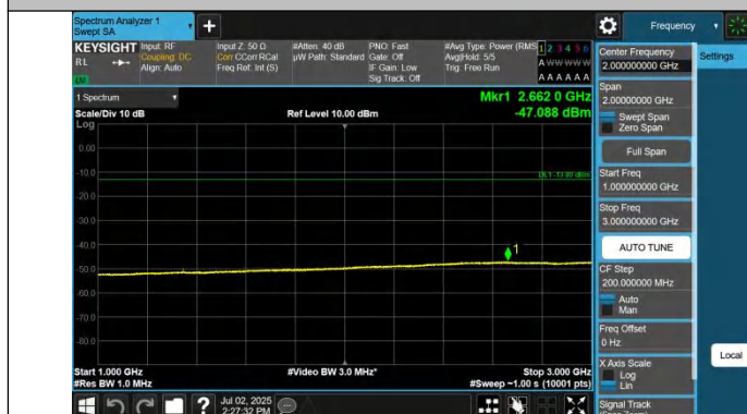
Band71-10MHz-QPSK-133172-1RB#49-1000~3000-PASS
