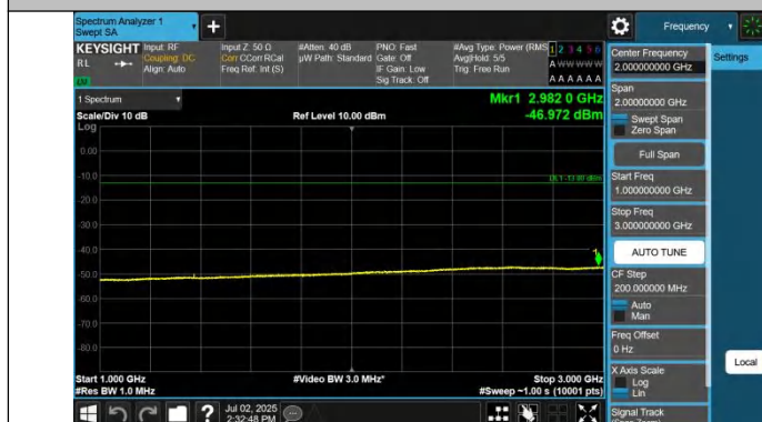
Band71-15MHz-QPSK-133297-1RB#74-1000~3000-PASS
