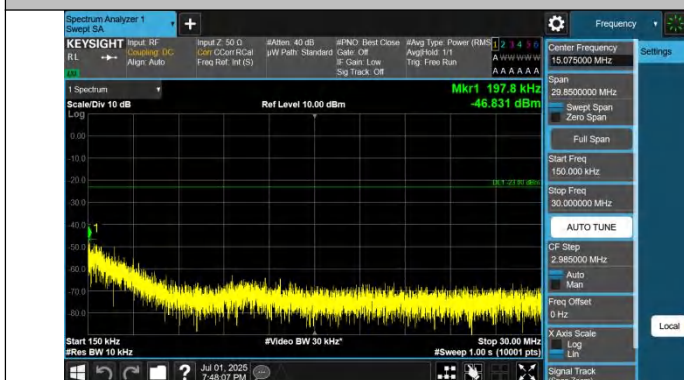
Band71-10MHz-QPSK-133297-1RB#49-0.15~30-PASS
