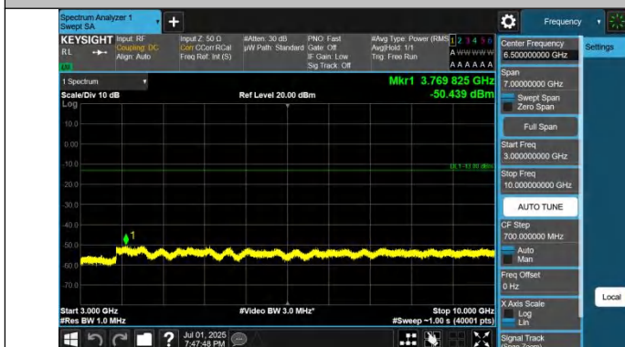
Band71-10MHz-QPSK-133297-1RB#0-3000~10000-PASS
