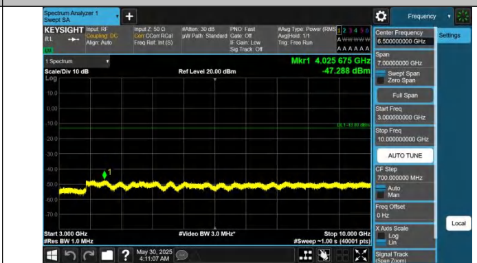
Band71-20MHz-QPSK-133322-1RB#99-3000~10000-PASS
