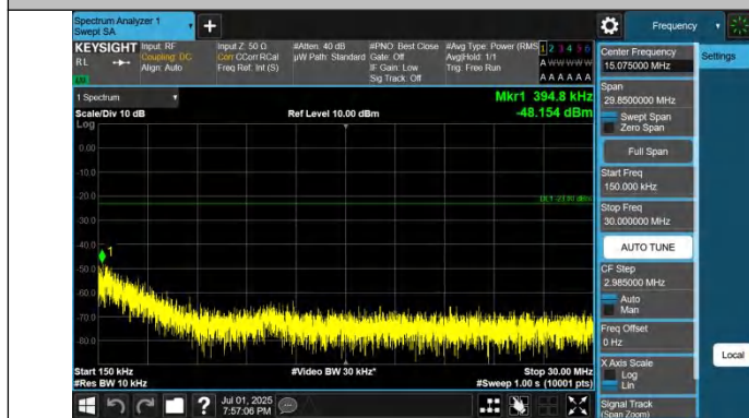
Band71-15MHz-QPSK-133297-1RB#74-0.15~30-PASS
