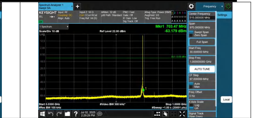
Band71-10MHz-QPSK-133422-1RB#49-30~1000-PASS
