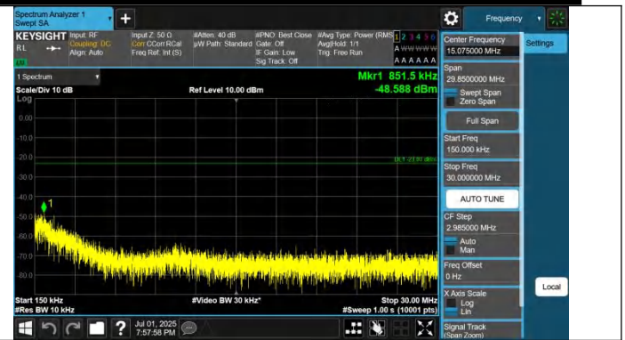
Band71-15MHz-QPSK-133397-1RB#0-0.15~30-PASS
