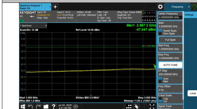
Band71-15MHz-QPSK-133197-1RB#74-1000~3000-PASS
