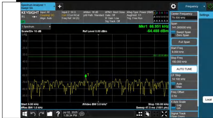
Band71-15MHz-QPSK-133397-1RB#0-0.009~0.15-PASS
