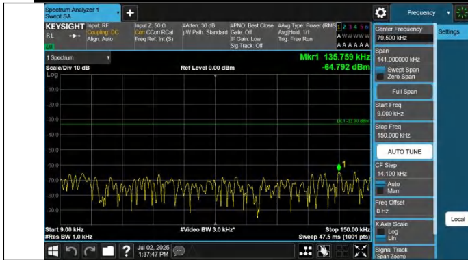
Band71-10MHz-QPSK-133297-1RB#0-0.009~0.15-PASS
