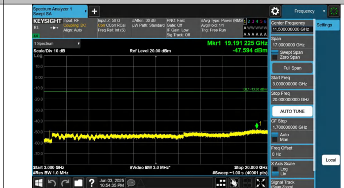
Band66-10MHz-QPSK-132022-1RB#49-3000~20000-PASS
