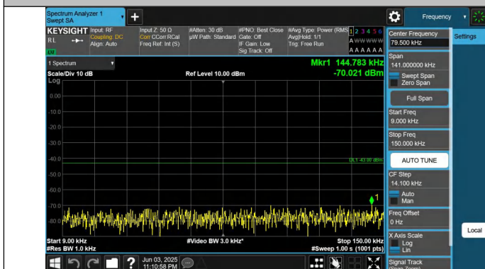
Band66-15MHz-QPSK-132597-1RB#0-0.009~0.15-PASS
