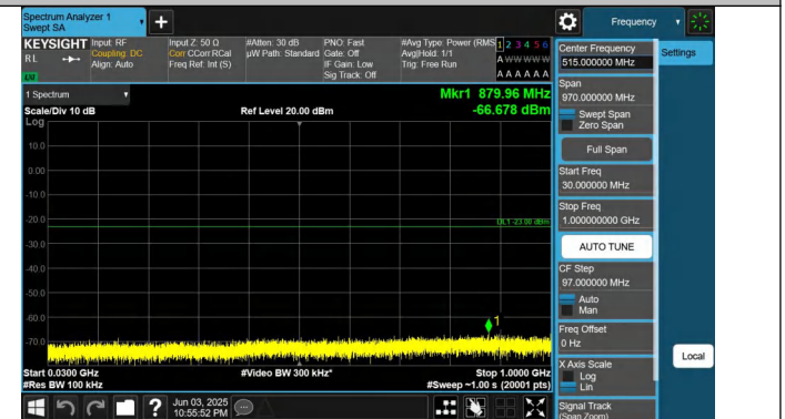
Band66-10MHz-QPSK-132322-1RB#49-30~1000-PASS
