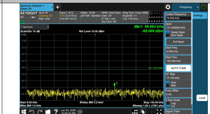
Band66-10MHz-QPSK-132022-1RB#49-0.009~0.15-PASS
