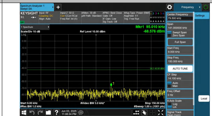
Band66-15MHz-QPSK-132047-1RB#74-0.009~0.15-PASS
