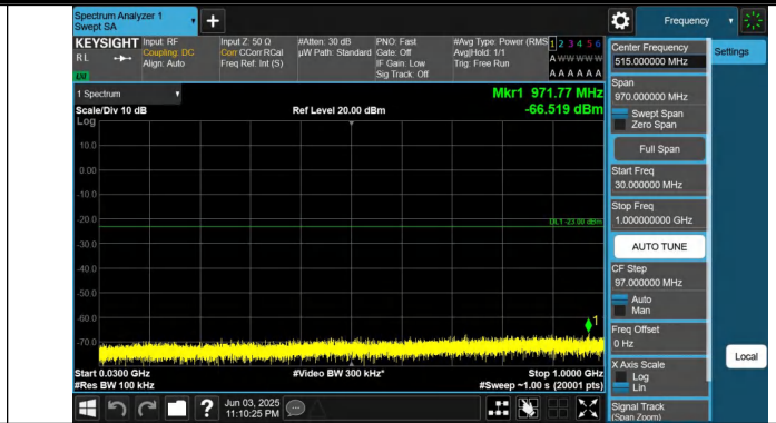
Band66-15MHz-QPSK-132322-1RB#74-30~1000-PASS
