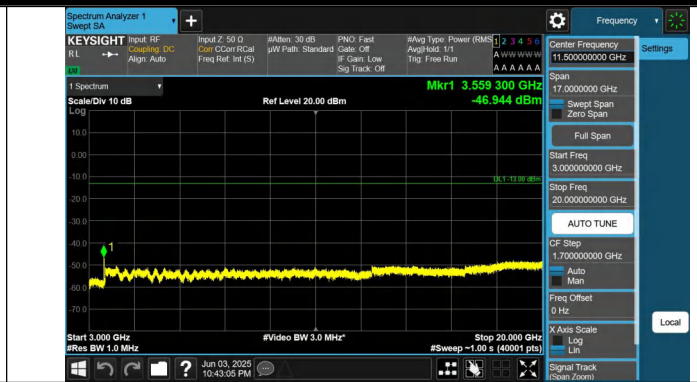
Band66-5MHz-QPSK-132647-1RB#24-3000~20000-PASS
