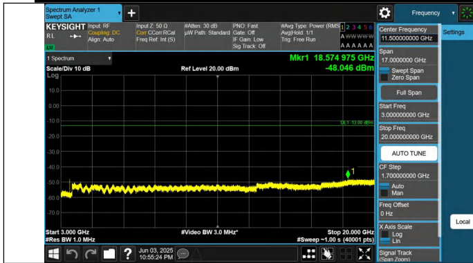
Band66-10MHz-QPSK-132322-1RB#0-3000~20000-PASS
