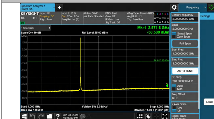
Band66-10MHz-QPSK-132322-1RB#49-1000~3000-PASS
