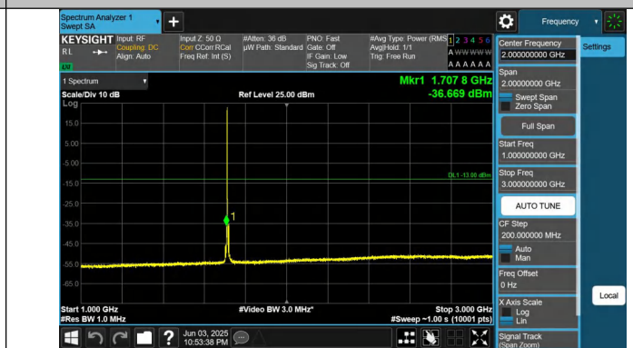
Band66-10MHz-QPSK-132022-1RB#0-1000~3000-PASS
