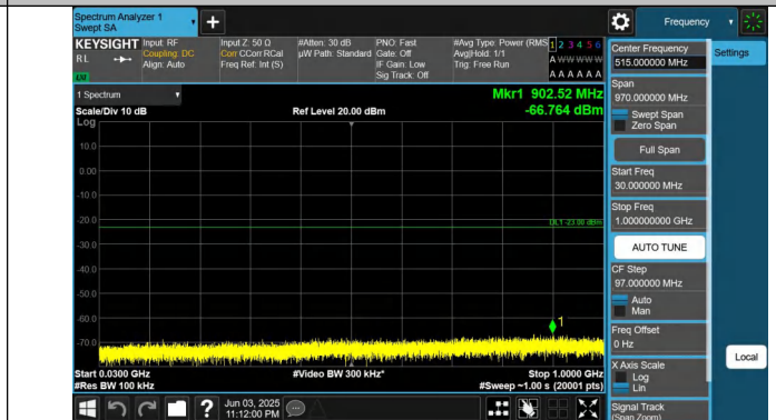
Band66-15MHz-QPSK-132597-1RB#74-30~1000-PASS
