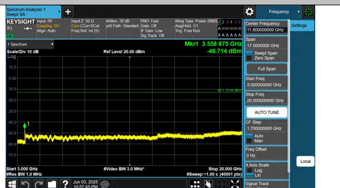
Band66-10MHz-QPSK-132622-1RB#49-3000~20000-PASS
