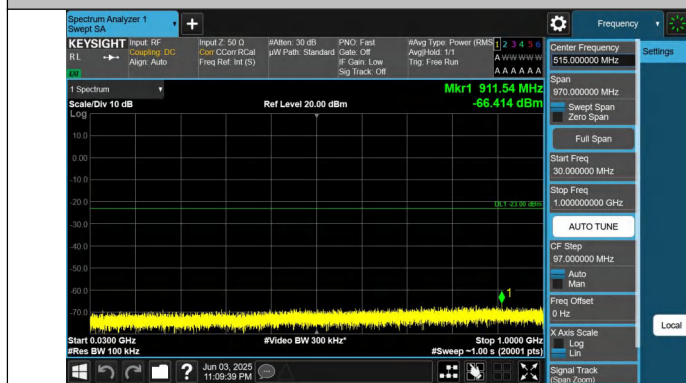
Band66-15MHz-QPSK-132322-1RB#0-30~1000-PASS
