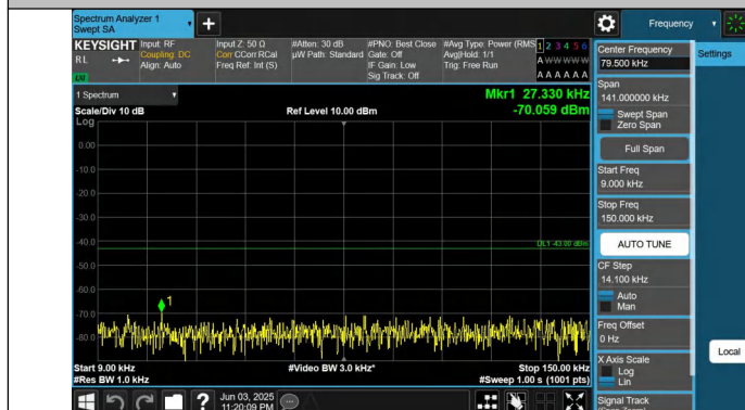
Band66-20MHz-QPSK-132072-1RB#0-0.009~0.15-PASS
