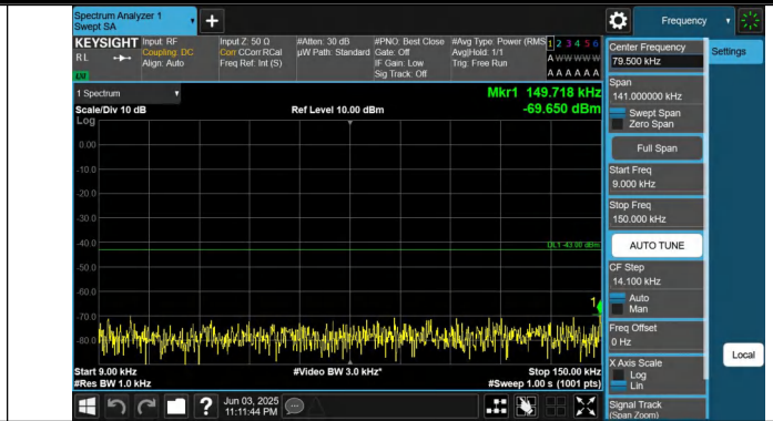
Band66-15MHz-QPSK-132597-1RB#74-0.009~0.15-PASS
