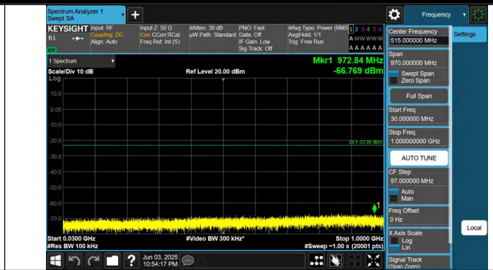
Band66-10MHz-QPSK-132022-1RB#49-30~1000-PASS
