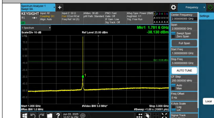
Band66-10MHz-QPSK-132622-1RB#49-1000~3000-PASS
