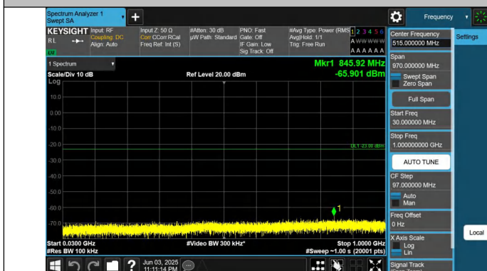
Band66-15MHz-QPSK-132597-1RB#0-30~1000-PASS
