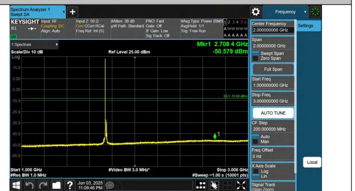
Band66-15MHz-QPSK-132322-1RB#0-1000~3000-PASS
