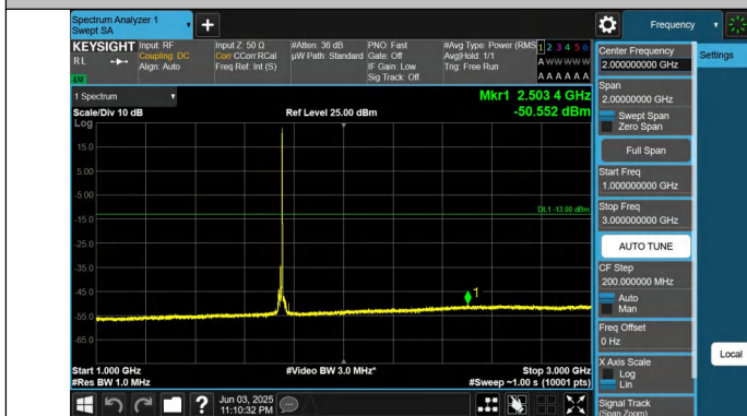
Band66-15MHz-QPSK-132322-1RB#74-1000~3000-PASS
