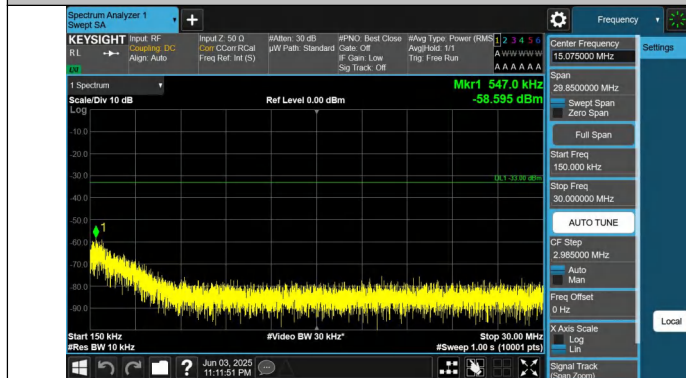
Band66-15MHz-QPSK-132597-1RB#74-0.15~30-PASS
