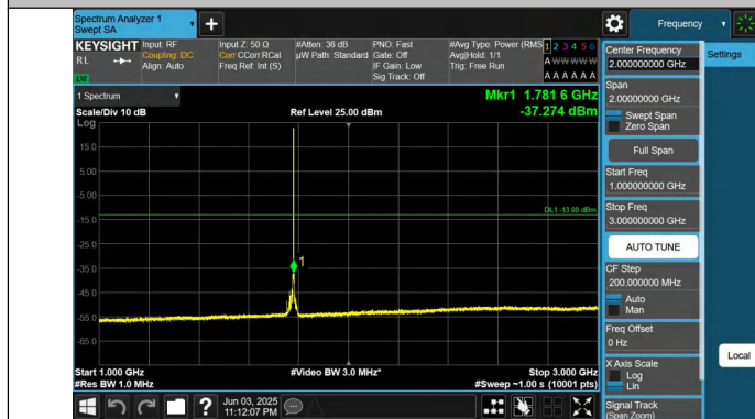
Band66-15MHz-QPSK-132597-1RB#74-1000~3000-PASS
