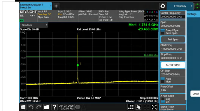
Band66-5MHz-QPSK-132647-1RB#24-1000~3000-PASS
