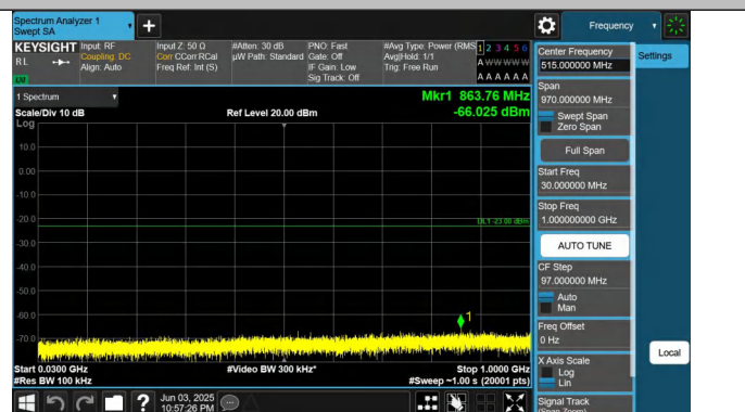
Band66-10MHz-QPSK-132622-1RB#49-30~1000-PASS
