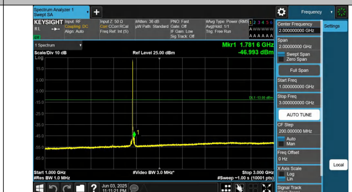
Band66-15MHz-QPSK-132597-1RB#0-1000~3000-PASS
