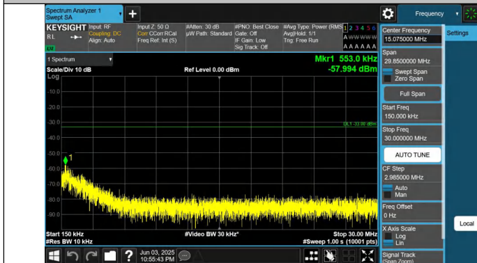
Band66-10MHz-QPSK-132322-1RB#49-0.15~30-PASS
