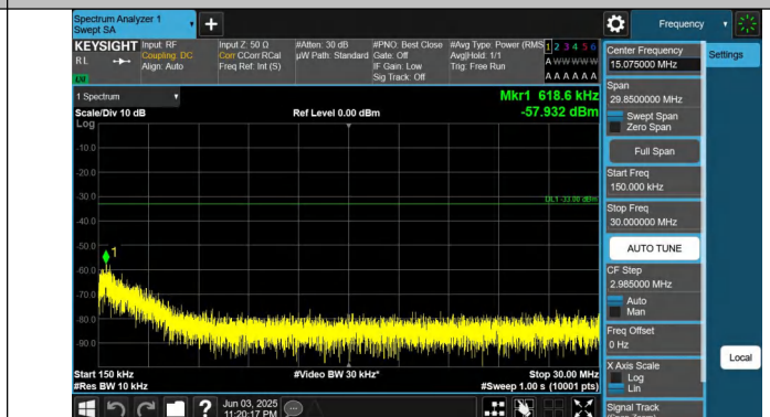
Band66-20MHz-QPSK-132072-1RB#0-0.15~30-PASS
