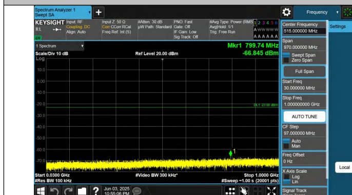
Band66-10MHz-QPSK-132322-1RB#0-30~1000-PASS
