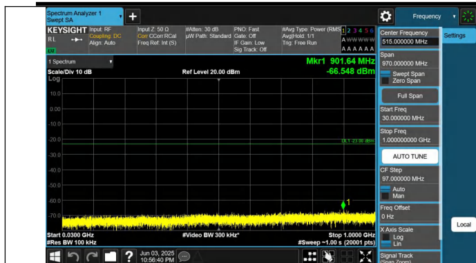
Band66-10MHz-QPSK-132622-1RB#0-30~1000-PASS
