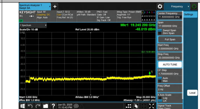
Band66-15MHz-QPSK-132322-1RB#74-3000~20000-PASS
