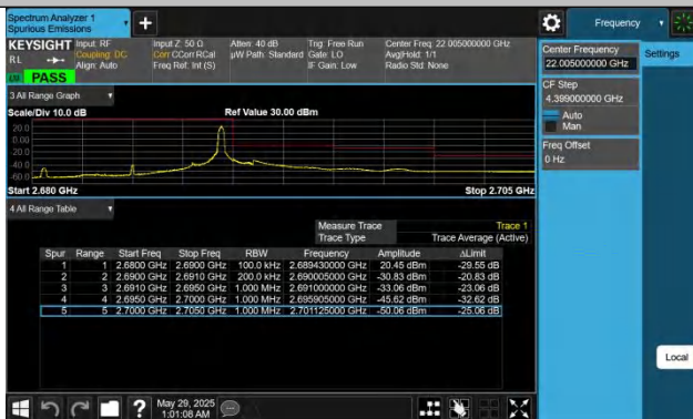
Band41-10MHz-QPSK-41540-1RB#49-PASS
