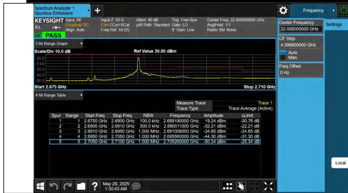
Band41-15MHz-QPSK-41515-1RB#74-PASS
