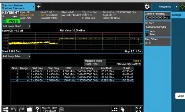
Band41-15MHz-QPSK-39725-75RB#0-PASS
