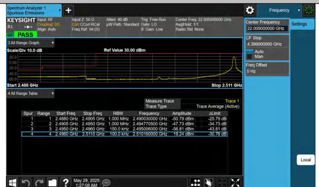
Band41-15MHz-QPSK-39725-1RB#74-PASS
