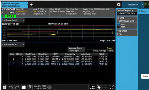
Band41-10MHz-QPSK-39700-50RB#0-PASS
