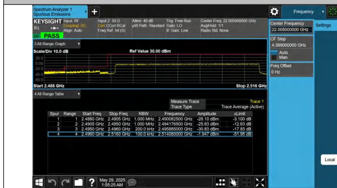
Band41-20MHz-QPSK-39750-100RB#0-PASS
