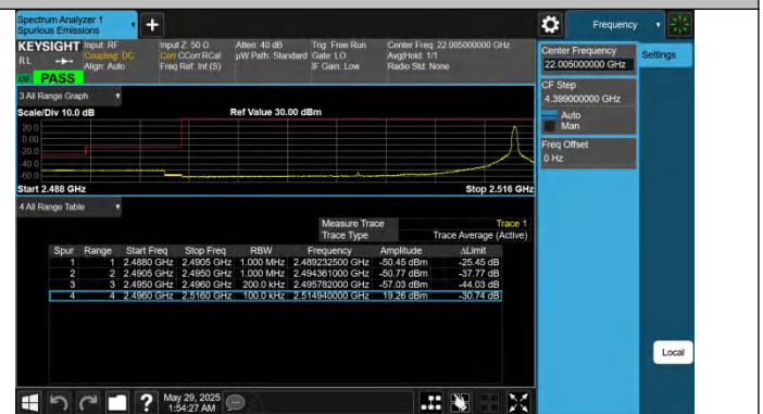
Band41-15MHz-QPSK-39750-1RB#99-PASS
