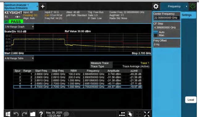
Band41-10MHz-QPSK-41540-50RB#0-PASS
