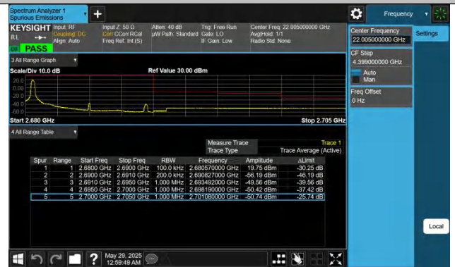
Band41-10MHz-QPSK-41540-1RB#0-PASS
