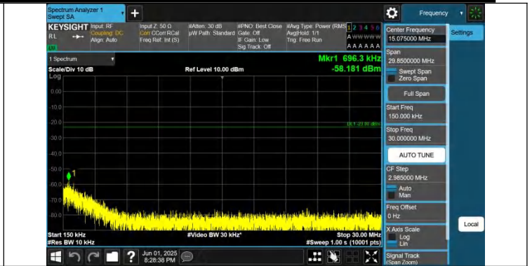
Band26(824-849)-5MHz-QPSK-26915-1RB#0.15~30-PASS
