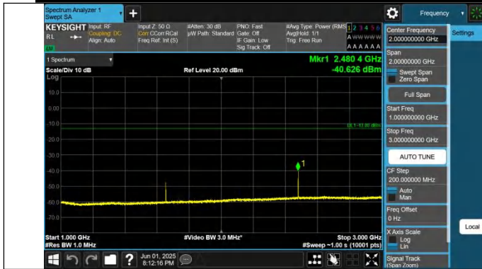
Band26(824-849)-3MHz-QPSK-26805-1RB#14-1000~3000-PASS
