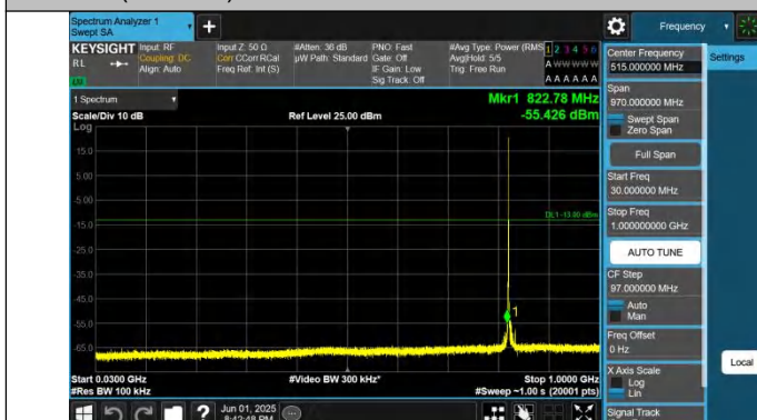
Band26(824-849)-10MHz-QPSK-26840-1RB#0-30~1000-PASS
