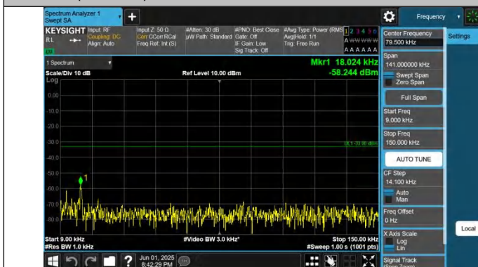
Band26(824-849)-10MHz-QPSK-26840-1RB#0-0.009~0.15-PASS
