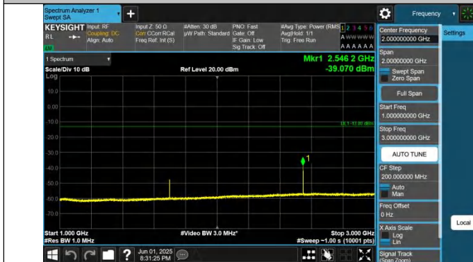
Band26(824-849)-5MHz-QPSK-27015-1RB#24-1000~3000-PASS
