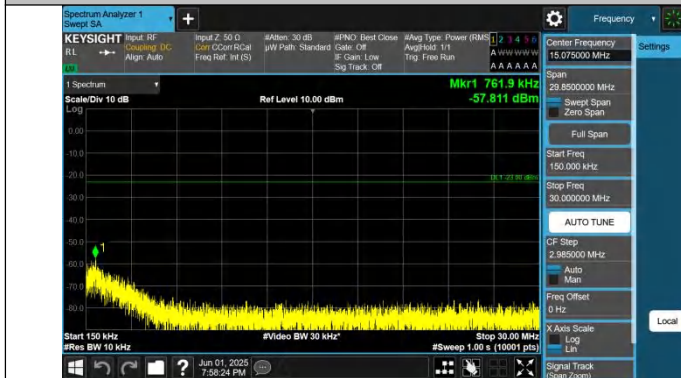
Band26(824-849)-1.4MHz-QPSK-26915-1RB#5-0.15~30-PASS
