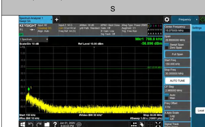
Band26(824-849)-1.4MHz-QPSK-27033-1RB#5-0.15~30-PASS
