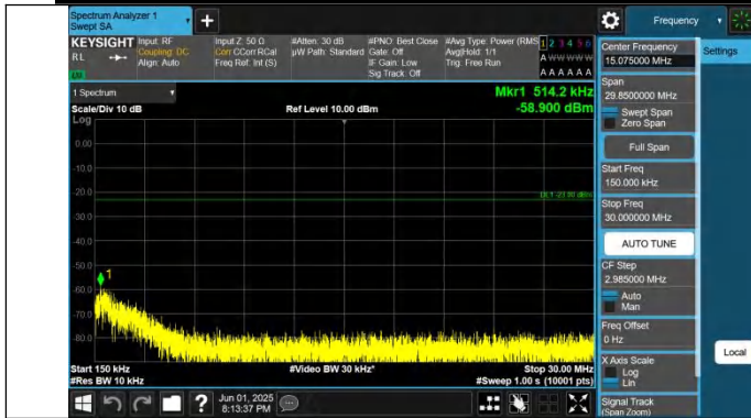
Band26(824-849)-3MHz-QPSK-26915-1RB#14-0.15~30-PASS
