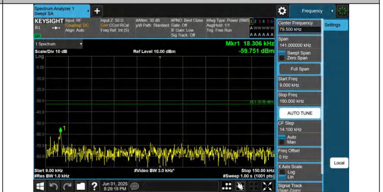
Band26(824-849)-5MHz-QPSK-26915-1RB#24.0.009~0.15-PASS
