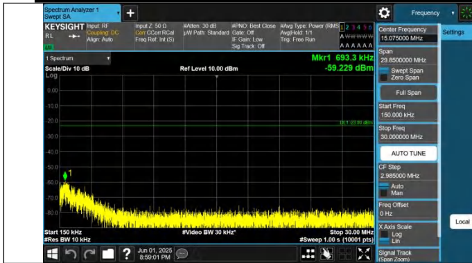
Band26(824-849)-15MHz-QPSK-26865-1RB#74-0.15~30-PASS
