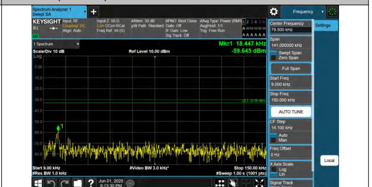
Band26(824-849)-3MHz-QPSK-26915-1RB#14-0.009~0.15-PASS
