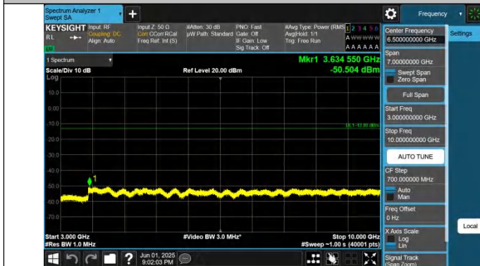
Band26(824-849)-15MHz-QPSK-26965-1RB#0-3000~10000-PASS
