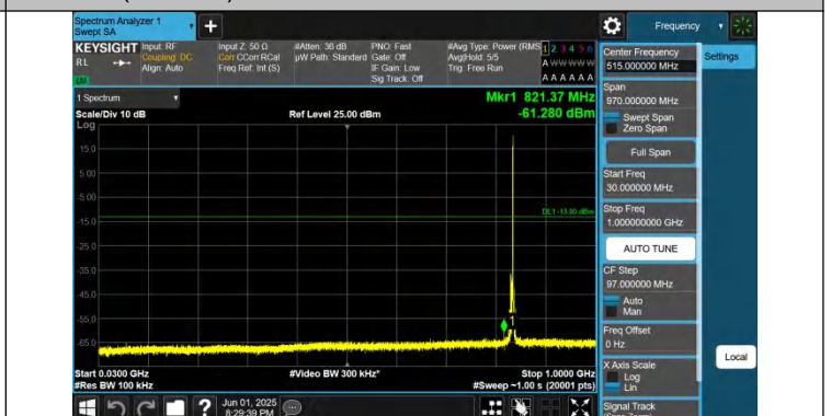
Band26(824-849)-5MHz-QPSK-26915-1RB#24.30~1000-PASS
