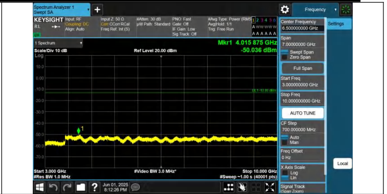
Band26(824-849)-3MHz-QPSK-26805-1RB#14-3000~10000-PASS
