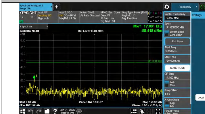
Band26(824-849)-15MHz-QPSK-26915-1RB#0-0.009~0.15-PASS
