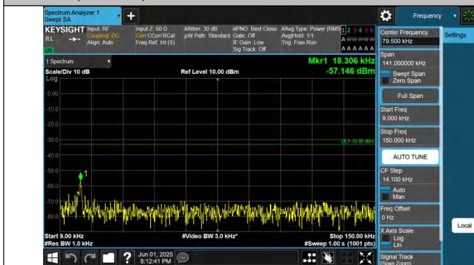
Band26(824-849)-3MHz-QPSK-26915-1RB#0-0.009~0.15-PASS
