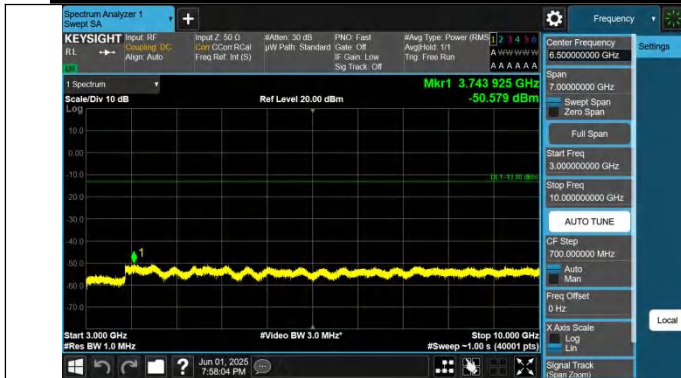
Band26(824-849)-1.4MHz-QPSK-26915-1RB#0-3000~10000-PASS S
