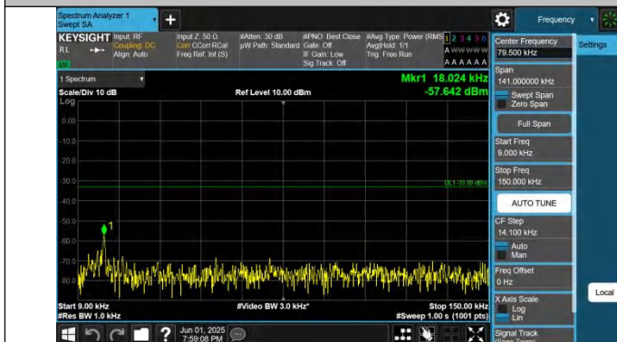
Band26(824-849)-1.4MHz-QPSK-27033-1RB#0-0.009~0.15-PASS
