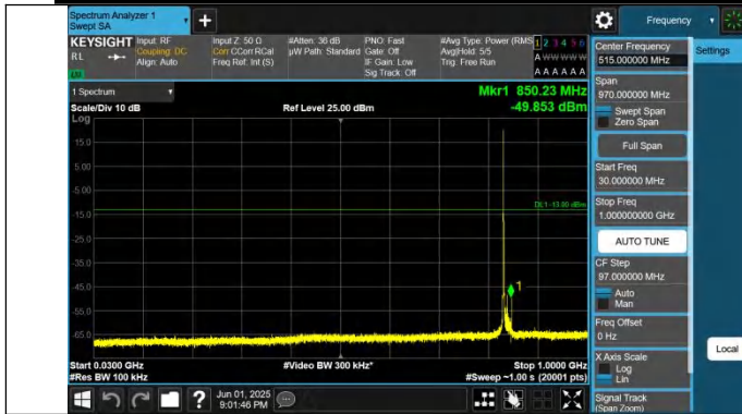
Band26(824-849)-15MHz-QPSK-26965-1RB#0-30~1000-PASS
