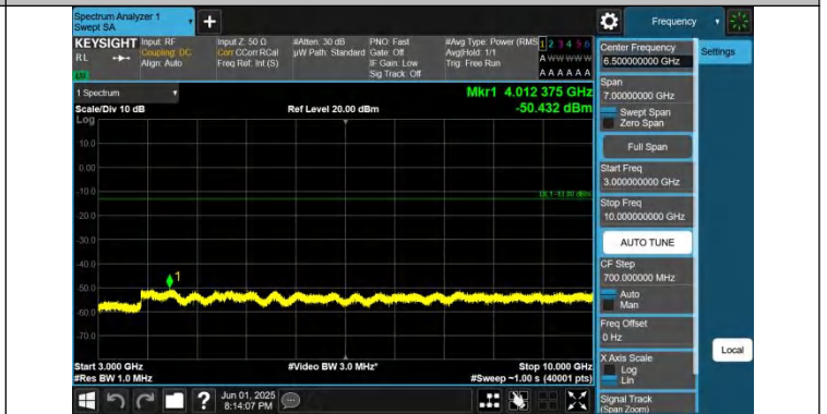
Band26(824-849)-3MHz-QPSK-26915-1RB#14-3000~10000-PASS
