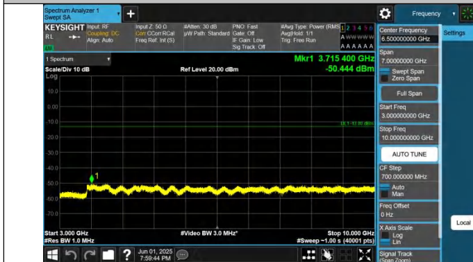
Band26(824-849)-1.4MHz-QPSK-27033-1RB#0-3000~10000-PASS
