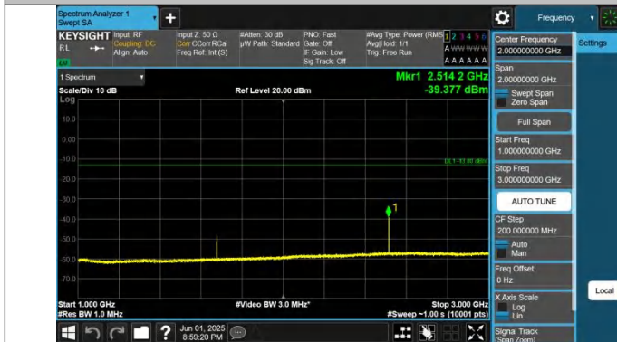
Band26(824-849)-15MHz-QPSK-26865-1RB#74-1000~3000-PAS
