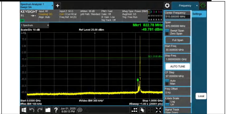
Band26(824-849)-15MHz-QPSK-26865-1RB#74-30~1000-PASS
