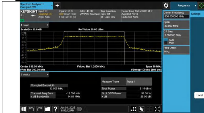
Band26(824-849)-15MHz-QPSK-26915-75RB#0-PASS
