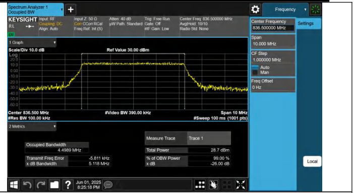
Band26(824-849)-5MHz-64QAM-26915-25RB#0-PASS
