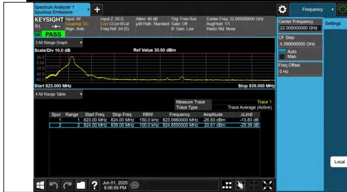
Band26(824-849)-15MHz-QPSK-26865-1RB#0-PASS
