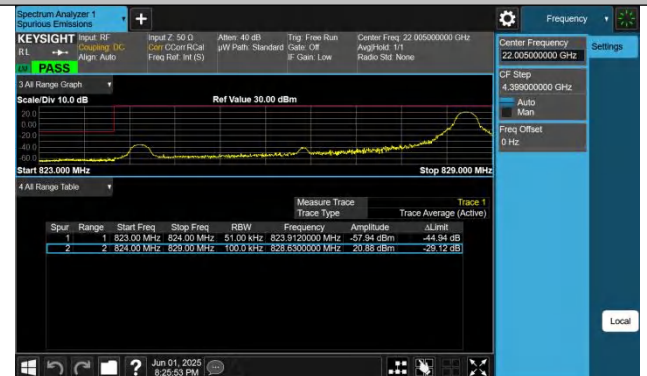
Band26(824-849)-5MHz-QPSK-26815-1RB#24-PASS
