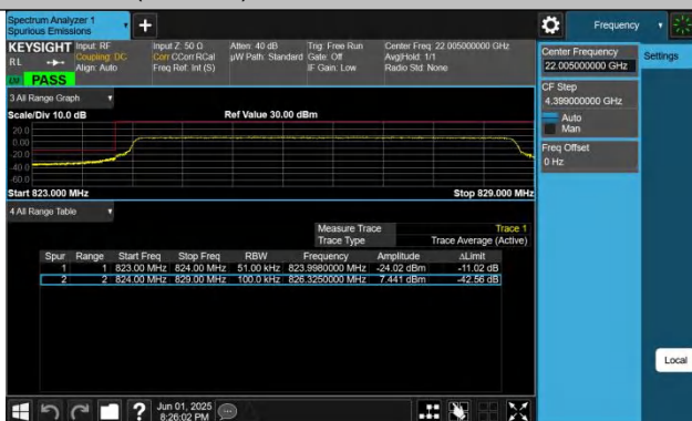
Band26(824-849)-5MHz-QPSK-26815-25RB#0-PASS
