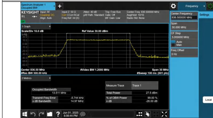
Band26(824-849)-15MHz-256QAM-26915-75RB#0-PASS
