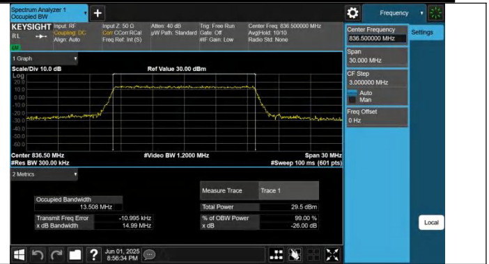
Band26(824-849)-15MHz-64QAM-26915-75RB#0-PASS
