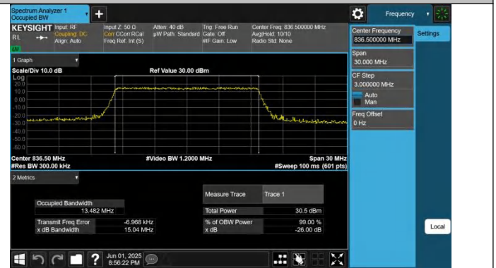
Band26(824-849)-15MHz-16QAM-26915-75RB#0-PASS
