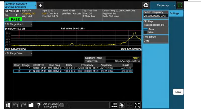
Band26(824-849)-15MHz-QPSK-26865-1RB#74-PASS
