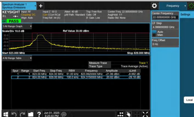
Band26(824-849)-5MHz-QPSK-26815-1RB#0-PASS
