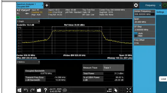
Band26(824-849)-10MHz-QPSK-26915-50RB#0-PASS
