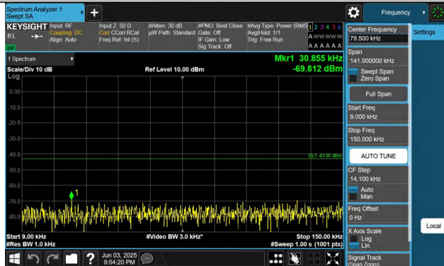
Band25-20MHz-QPSK-26590-1RB#0-0.009~0.15-PASS
