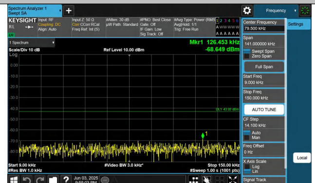
Band25-20MHz-QPSK-26590-1RB#99-0.009~0.15-PASS
