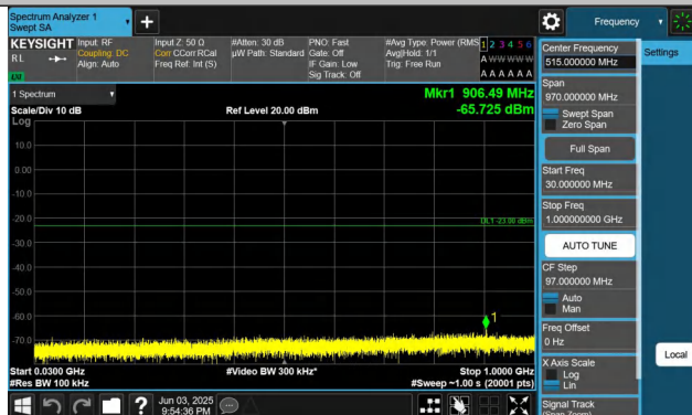
Band25-20MHz-QPSK-26590-1RB#0-30~1000-PASS
