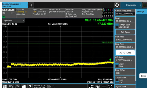
Band25-20MHz-QPSK-26590-1RB#0-3000~20000-PASS
