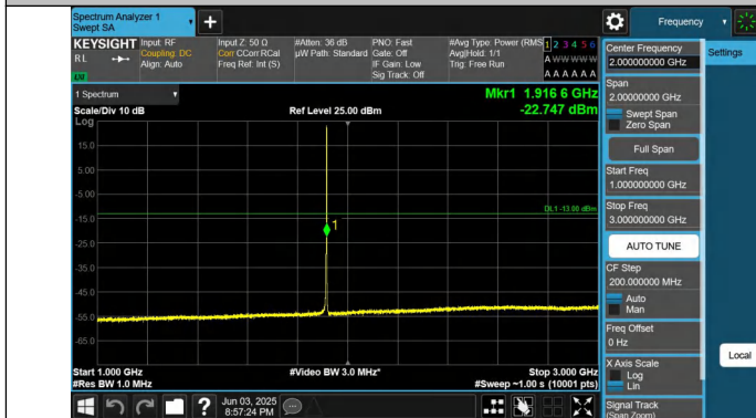
Band25-3MHz-QPSK-26675-1RB#14-1000~3000-PASS
