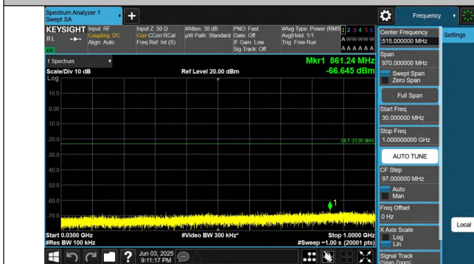
Band25-5MHz-QPSK-26665-1RB#0-30~1000-PASS
