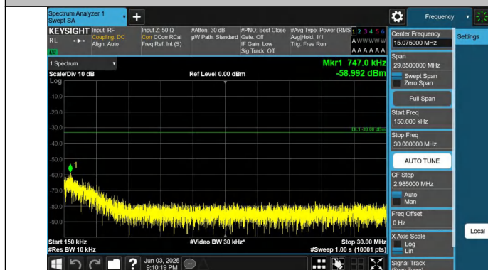
Band25-5MHz-QPSK-26365-1RB#24-0.15~30-PASS
