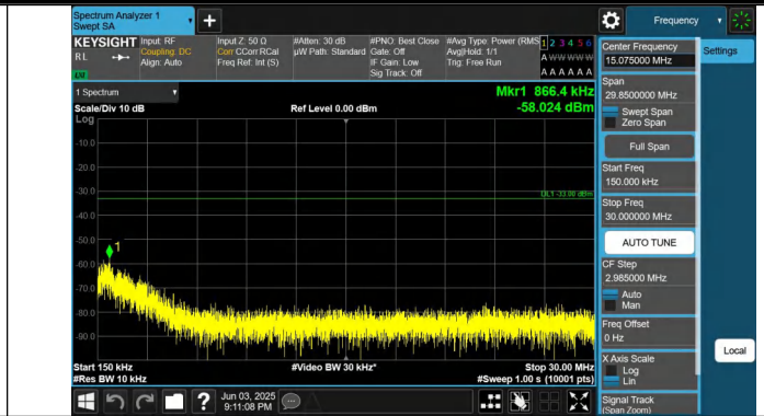
Band25-5MHz-QPSK-26665-1RB#0-0.15~30-PASS
