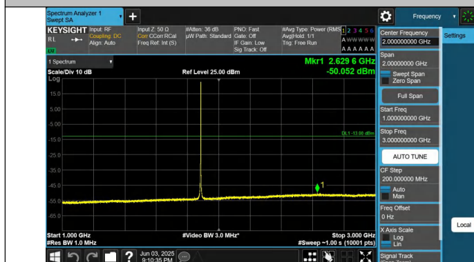
Band25-5MHz-QPSK-26365-1RB#24-1000~3000-PASS
