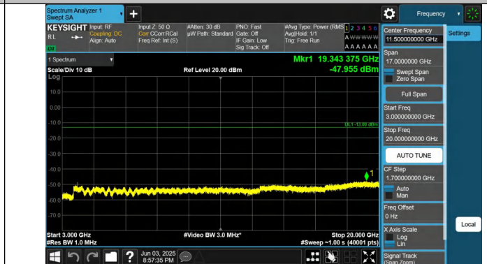
Band25-3MHz-QPSK-26675-1RB#14-3000~20000-PASS
