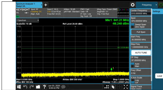
Band25-5MHz-QPSK-26365-1RB#0-30~1000-PASS
