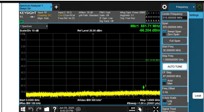
Band25-1.4MHz-QPSK-26365-1RB#5-30~1000-PASS
