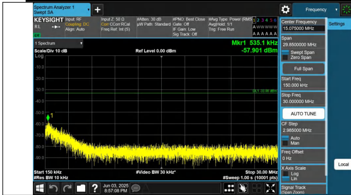
Band25-3MHz-QPSK-26675-1RB#14-0.15~30-PASS
