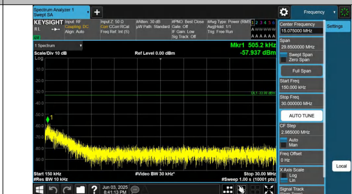
Band25-1.4MHz-QPSK-26683-1RB#0-0.15~30-PASS
