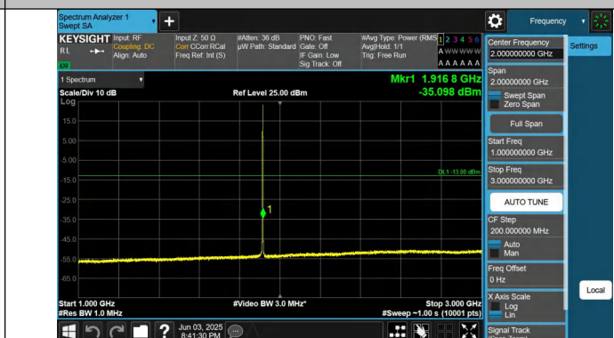
Band25-1.4MHz-QPSK-26683-1RB#0-1000~3000-PASS
