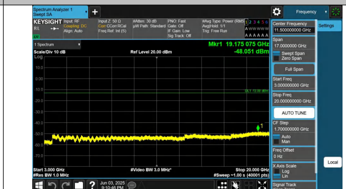
Band25-5MHz-QPSK-26365-1RB#24-3000~20000-PASS
