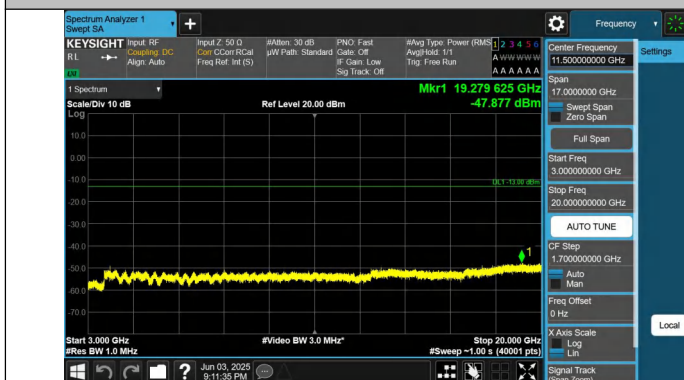
Band25-5MHz-QPSK-26665-1RB#0-3000~20000-PASS
