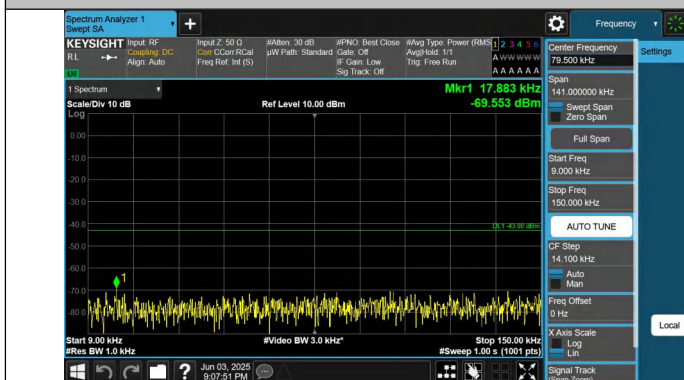
Band25-5MHz-QPSK-26065-1RB#0-0.009~0.15-PASS
