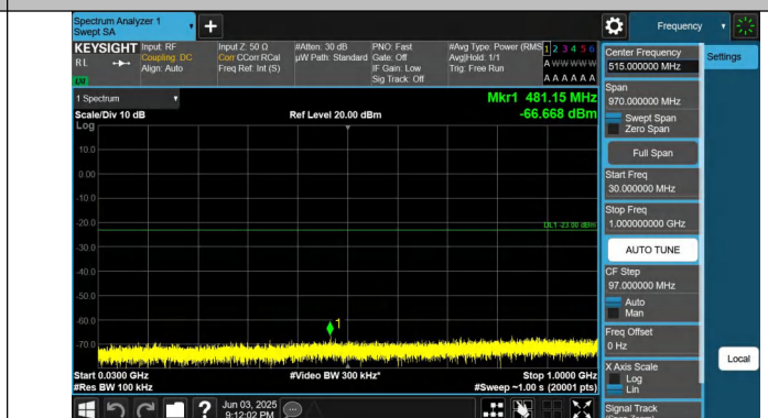
Band25-5MHz-QPSK-26665-1RB#24-30~1000-PASS
