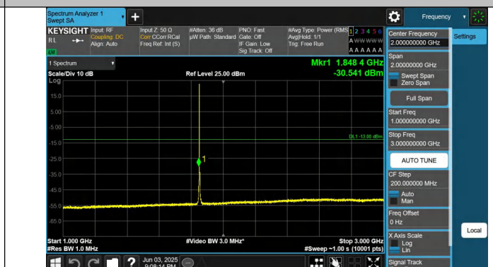
Band25-5MHz-QPSK-26065-1RB#0-1000~3000-PASS
