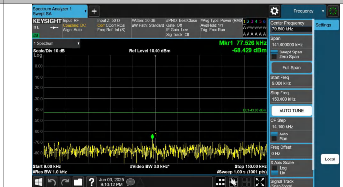
Band25-5MHz-QPSK-26365-1RB#24-0.009~0.15-PASS
