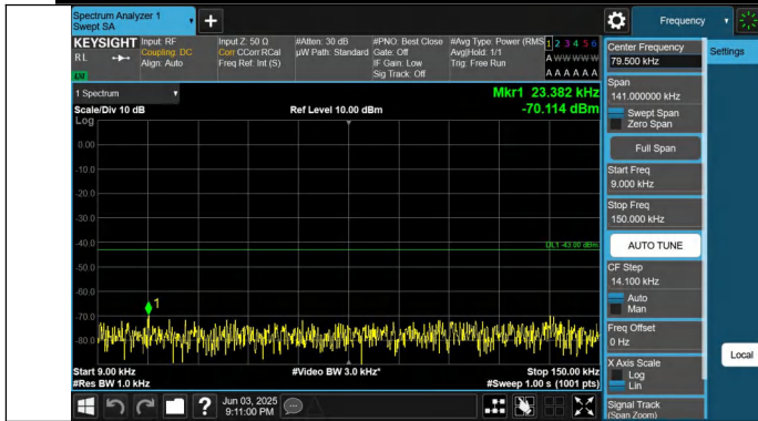
Band25-5MHz-QPSK-26665-1RB#0-0.009~0.15-PASS
