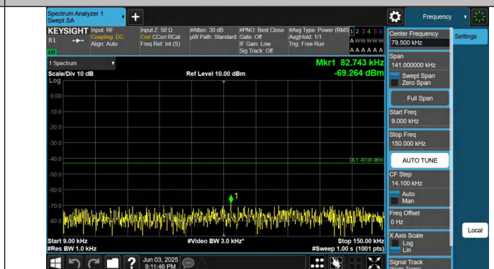
Band25-5MHz-QPSK-26665-1RB#24-0.009~0.15-PASS
