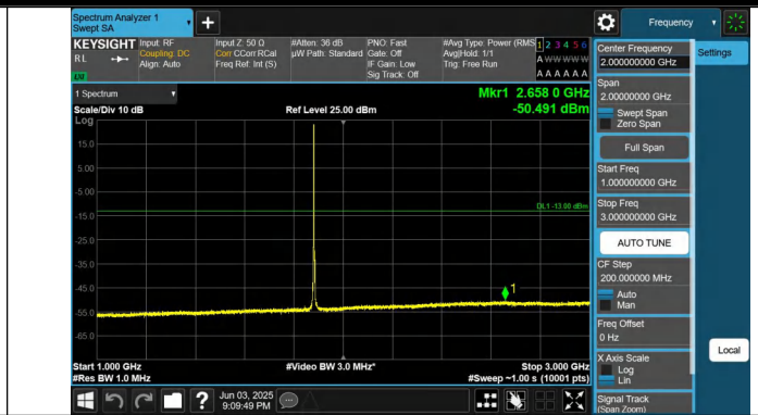
Band25-5MHz-QPSK-26365-1RB#0-1000~3000-PASS
