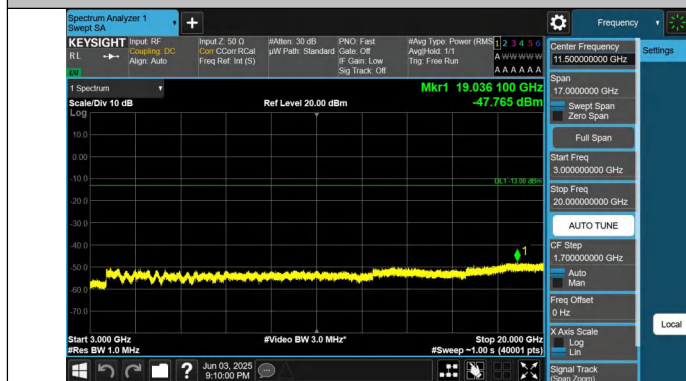
Band25-5MHz-QPSK-26365-1RB#0-3000~20000-PASS
