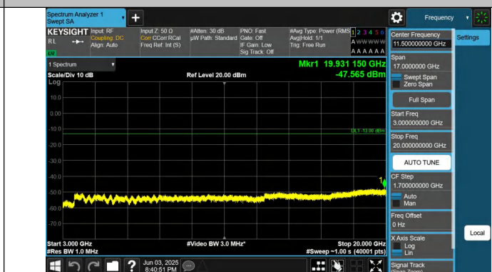
Band25-1.4MHz-QPSK-26365-1RB#5-3000~20000-PASS
