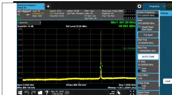
Band12-3MHz-QPSK-23025-1RB#0-30~1000-PASS
