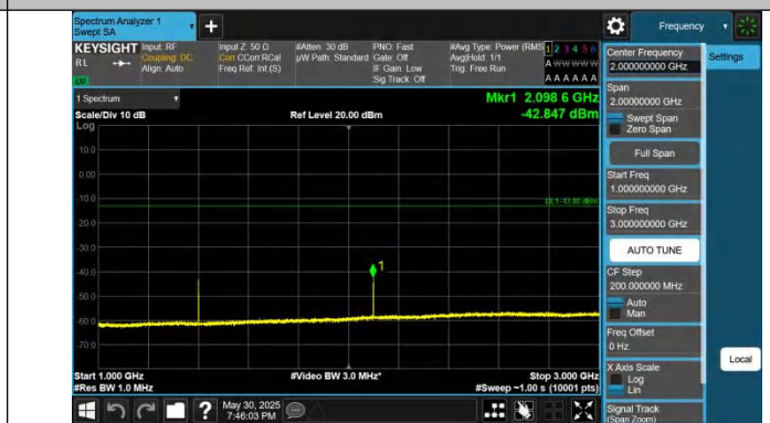
Band12-10MHz-QPSK-23060-1RB#0-1000~3000-PASS
