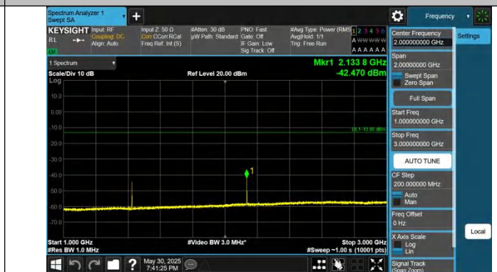
Band12-5MHz-QPSK-23155-1RB#0-1000~3000-PASS
