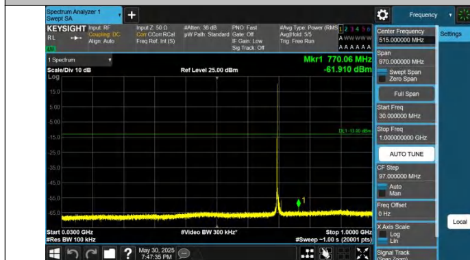
Band12-10MHz-QPSK-23095-1RB#0-30~1000-PASS
