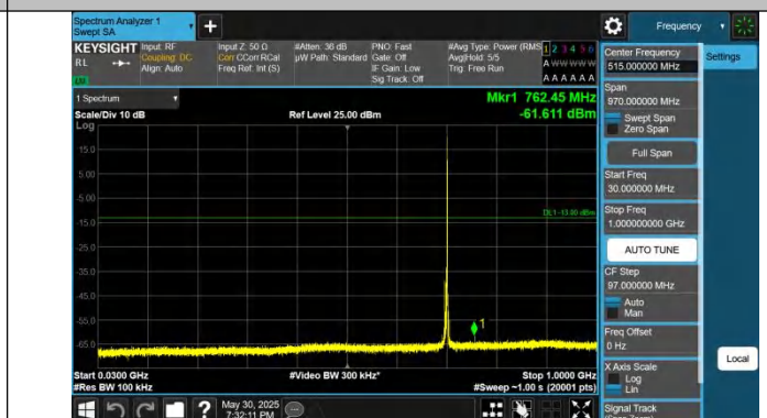
Band12-3MHz-QPSK-23095-1RB#14-30~1000-PASS
