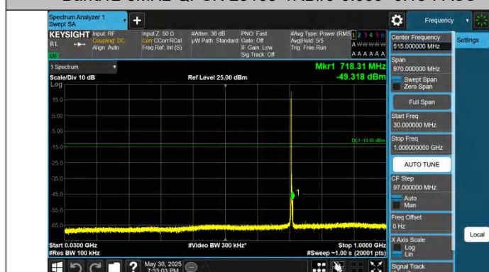
Band12-3MHz-QPSK-23165-1RB#0-30~1000-PASS
