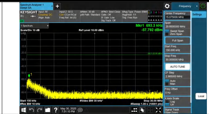
Band12-3MHz-QPSK-23095-1RB#0-0.15~30-PASS
