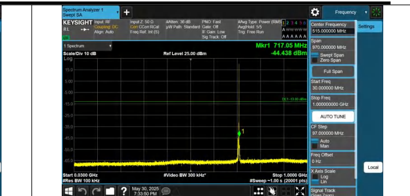
Band12-3MHz-QPSK-23165-1RB#14-30~1000-PASS
