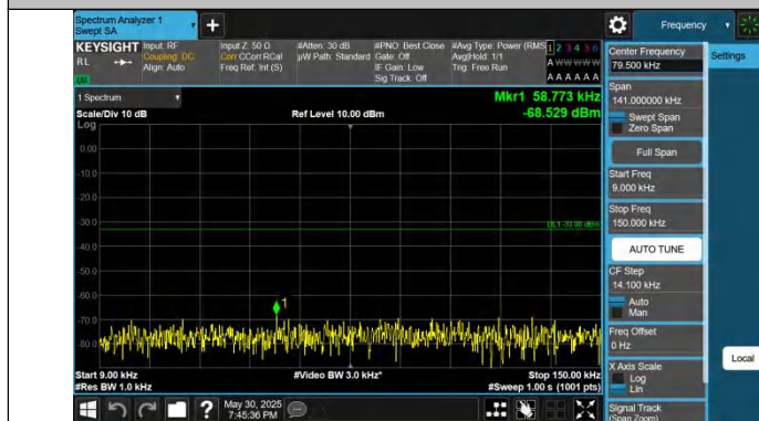
Band12-10MHz-QPSK-23060-1RB#0-0.009~0.15-PASS
