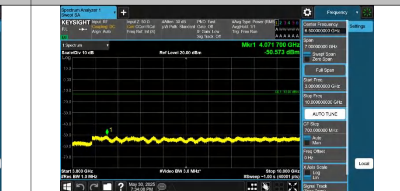
Band12-3MHz-QPSK-23165-1RB#14-3000~10000-PASS
