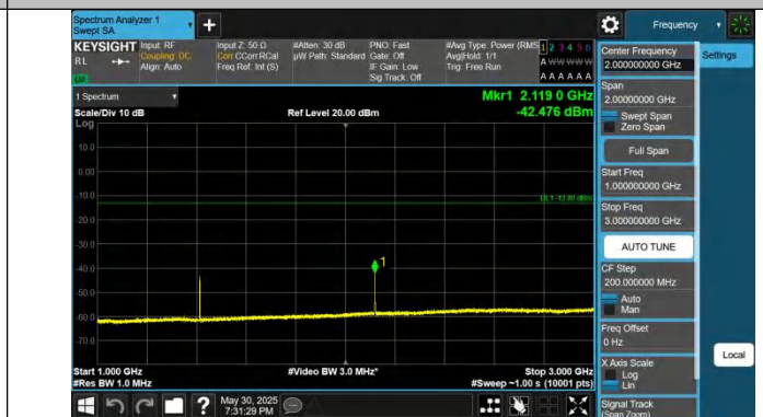
Band12-3MHz-QPSK-23095-1RB#0-1000~3000-PASS
