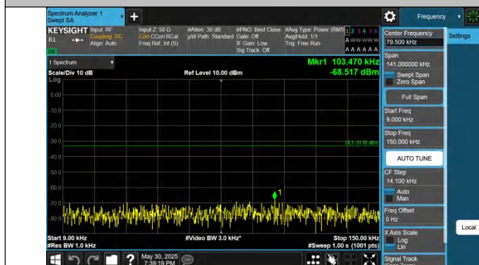
Band12-5MHz-QPSK-23095-1RB#0-0.009~0.15-PASS
