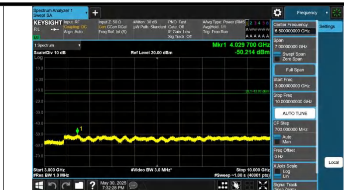
Band12-3MHz-QPSK-23095-1RB#14-3000~10000-PASS
