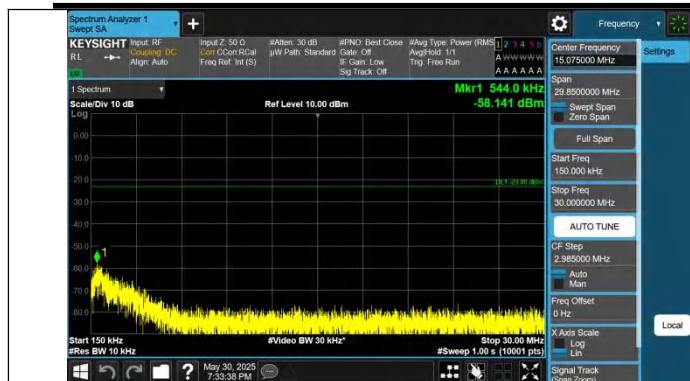
Band12-3MHz-QPSK-23165-1RB#14-0.15~30-PASS
