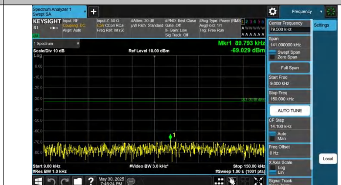
Band12-10MHz-QPSK-23060-1RB#49-0.009~0.15-PASS
