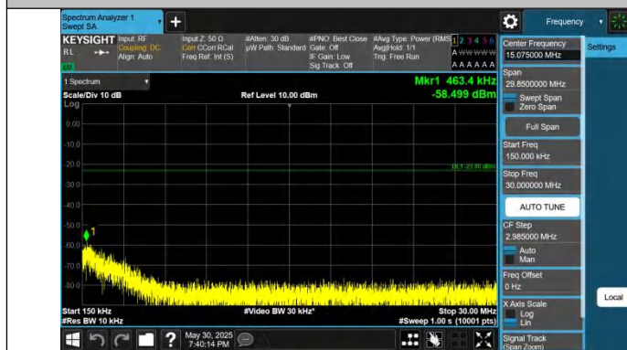
Band12-5MHz-QPSK-23095-1RB#24-0.15~30-PASS
