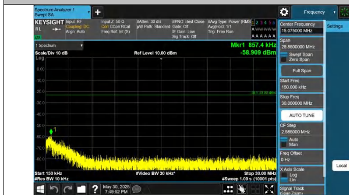
Band12-10MHz-QPSK-23130-1RB#49-0.15~30-PASS
