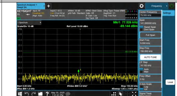
Band12-3MHz-QPSK-23095-1RB#14-0.009~0.15-PASS
