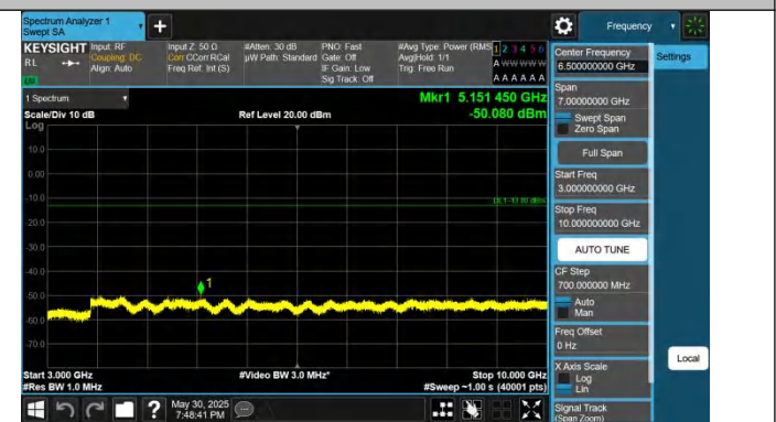
Band12-10MHz-QPSK-23095-1RB#49-3000~10000-PASS
