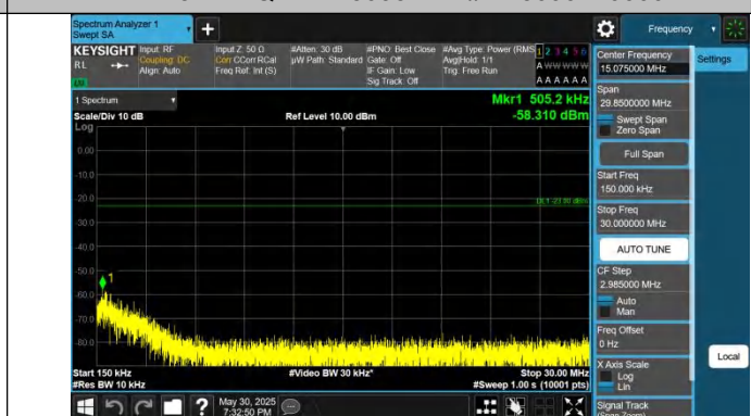
Band12-3MHz-QPSK-23165-1RB#0-0.15~30-PASS
