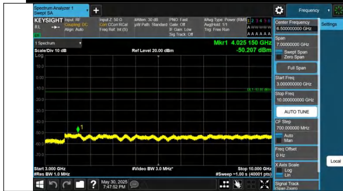
Band12-10MHz-QPSK-23095-1RB#0-3000~10000-PASS
