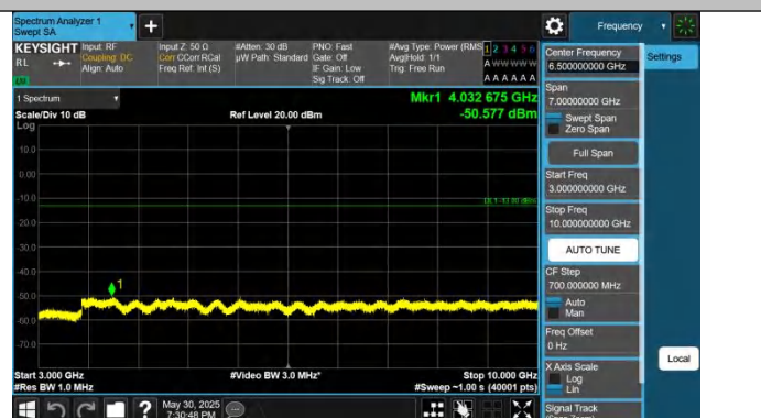
Band12-3MHz-QPSK-23025-1RB#14-3000~10000-PASS
