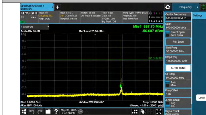
Band12-10MHz-QPSK-23060-1RB#0-30~1000-PASS
