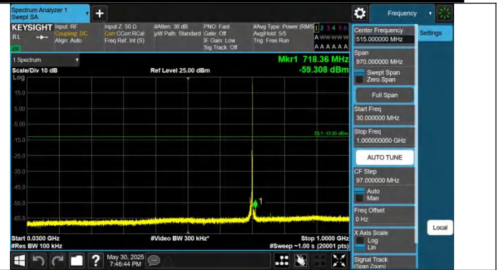
Band12-10MHz-QPSK-23060-1RB#49-30~1000-PASS
