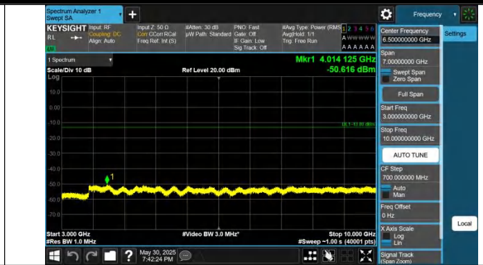
Band12-5MHz-QPSK-23155-1RB#24-3000~10000-PASS
