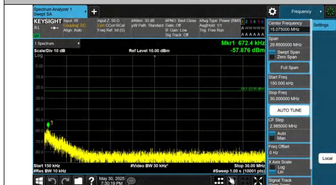
Band12-3MHz-QPSK-23025-1RB#14-0.15~30-PASS
