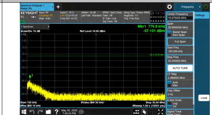
Band12-10MHz-QPSK-23060-1RB#0-0.15~30-PASS
