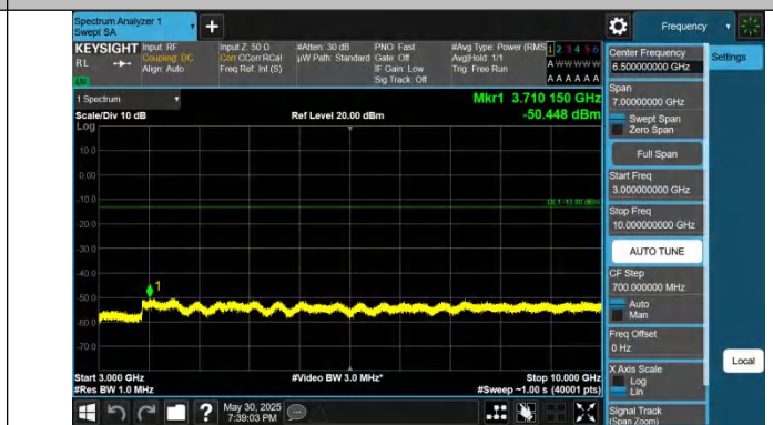
Band12-5MHz-QPSK-23035-1RB#24-3000~10000-PASS
