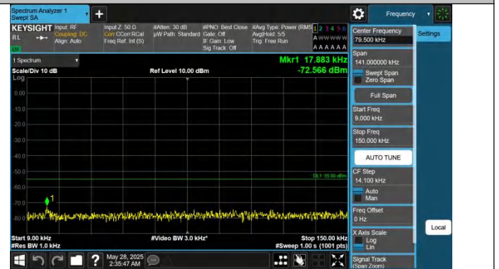
Band7-15MHz-QPSK-21100-1RB#74-0.009~0.15-PASS
