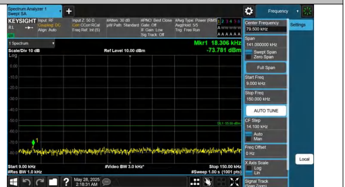
Band7-10MHz-QPSK-20800-1RB#49-0.009~0.15-PASS
