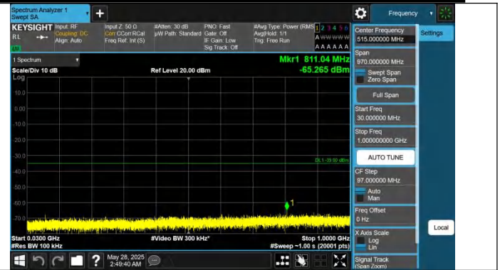
Band7-20MHz-QPSK-20850-1RB#99-30~1000-PASS
