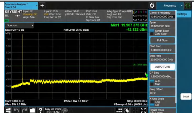
Band7-5MHz-QPSK-21100-1RB#0-1000~20000-PASS
