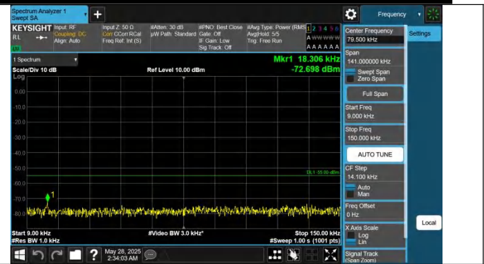
Band7-15MHz-QPSK-20825-1RB#74.0.009~0.15-PASS
