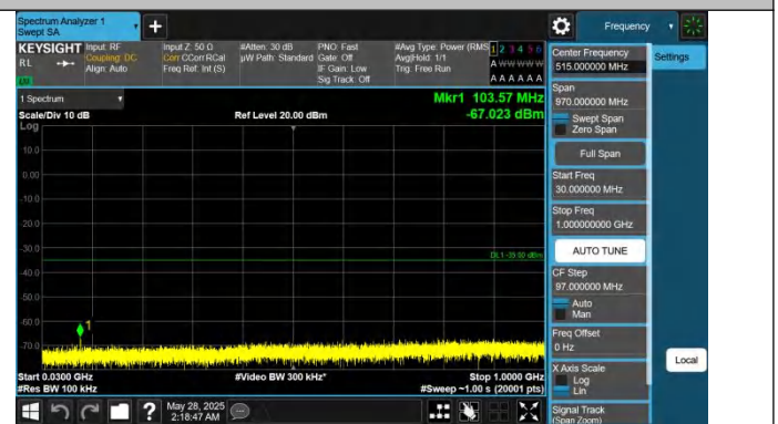
Band7-10MHz-QPSK-20800-1RB#49-30~1000-PASS
