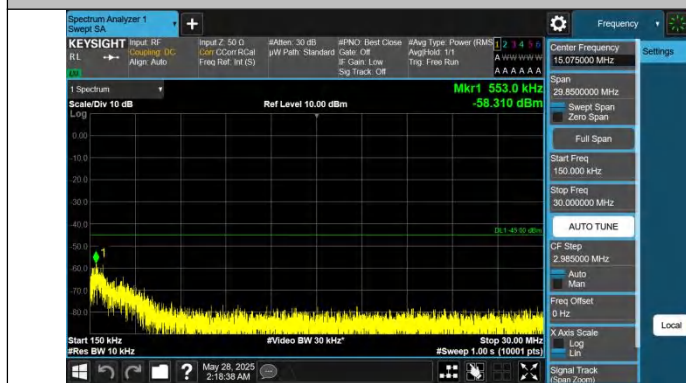
Band7-10MHz-QPSK-20800-1RB#49-0.15~30-PASS
