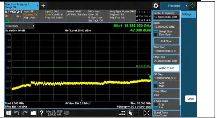
Band7-15MHz-QPSK-21100-1RB#0-1000~20000-PASS
