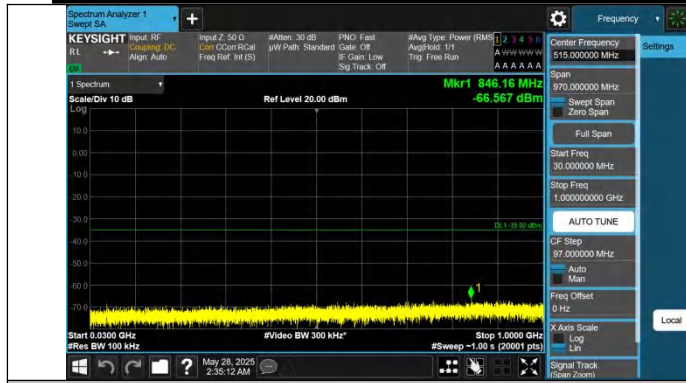
Band7-15MHz-QPSK-21100-1RB#0-30~1000-PASS
