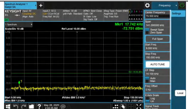
Band7-5MHz-QPSK-21100-1RB#24-0.009~0.15-PASS
