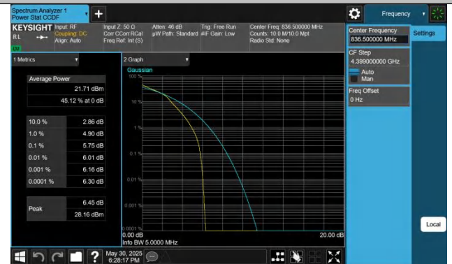
Band5-5MHz-16QAM-20525-25RB#0-PASS
