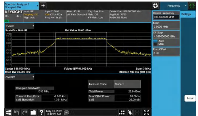
Band5-1.4MHz-64QAM-20525-6RB#0-PASS
