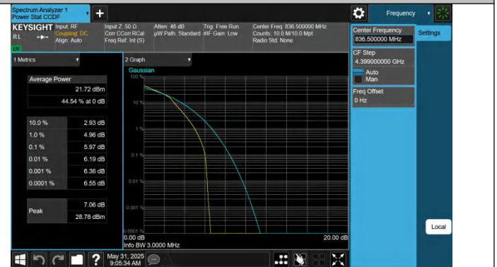
Band5-3MHz-16QAM-20525-15RB#0-PASS
