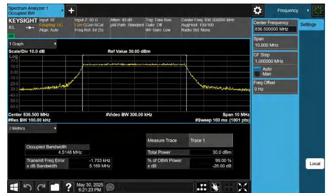
Band5-5MHz-64QAM-20525-25RB#0-PASS
