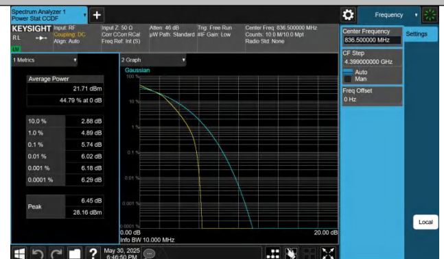
Band5-10MHz-16QAM-20525-50RB#0-PASS
