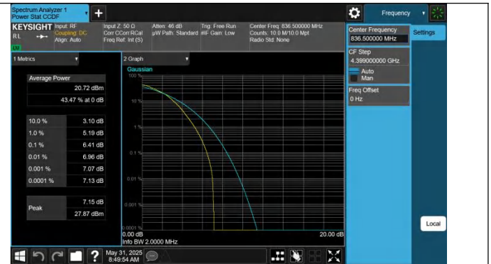
Band5-1.4MHz-64QAM-20525-6RB#0-PASS
