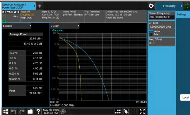
Band5-10MHz-QPSK-20525-50RB#0-PASS
