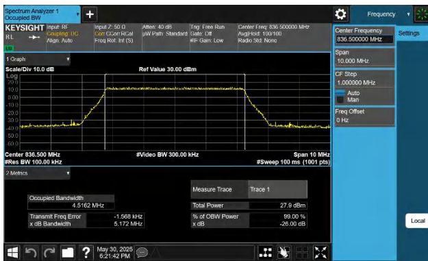
Band5-5MHz-256QAM-20525-25RB#0-PASS
