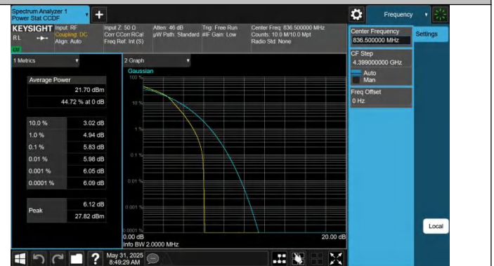
Band5-1.4MHz-16QAM-20525-6RB#0-PASS
