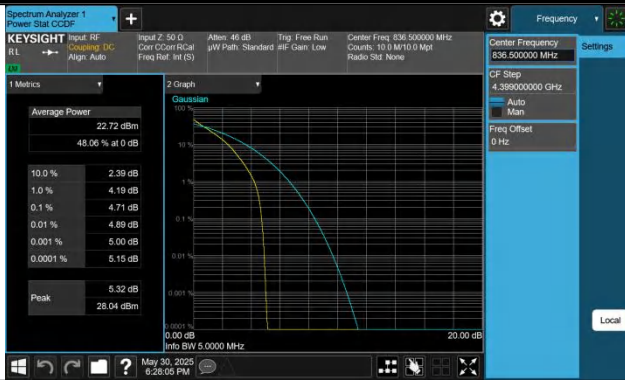
Band5-5MHz-QPSK-20525-25RB#0-PASS
