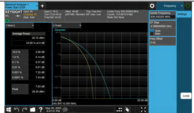
Band5-10MHz-64QAM-20525-50RB#0-PASS
